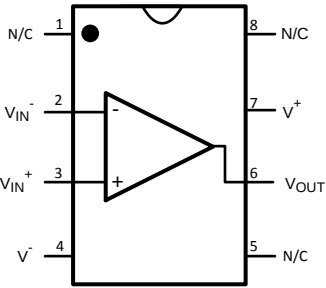
Figure 3. 8-Pin SOIC (Top View) See Package Number D0008A
