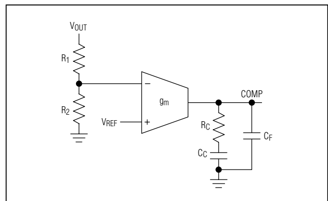
Figure 3. Compensation Network
