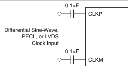
Figure 57. Differential Clock Driving Circuit
