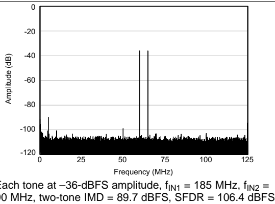
Figure 5. FFT for Two-Tone Input Signal
