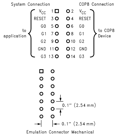
Figure 4-5. Emulation Connection
