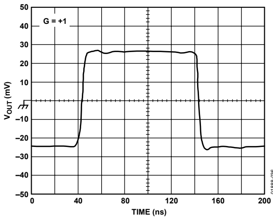
Figure 36. Small Signal Transient Response, V_O = 50\text{ mV p-p} , G = +1 (See Figure 48)
