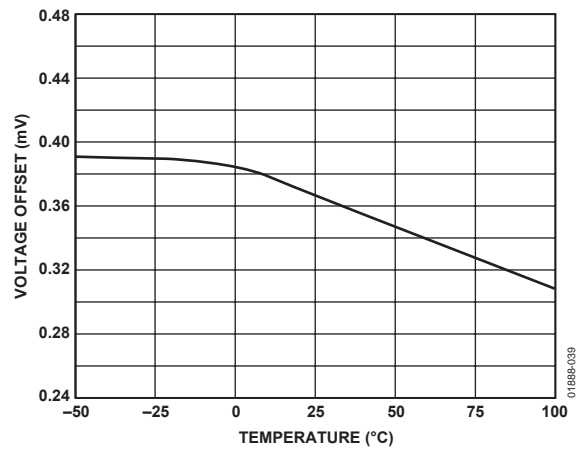
Figure 39. V_{OS} vs. Temperature
