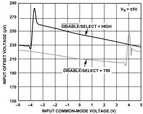
Figure 44. Input Offset Voltage vs. Input Common-Mode Voltage, V_S = \pm 5V
