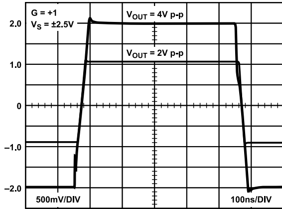
Figure 33. Large Signal Transient Response, G = +1
