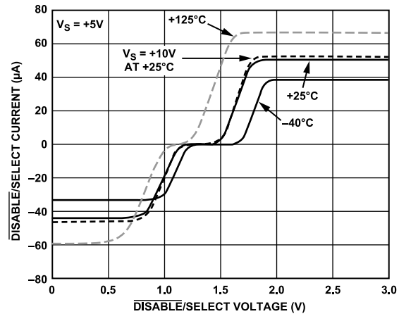
Figure 55. \overline{\text{DISABLE}}/\overline{\text{SELECT}} Current vs. \overline{\text{DISABLE}}/\overline{\text{SELECT}} Voltage and Temperature
