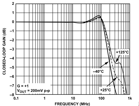
Figure 19. AD8028 Small Signal Frequency Response vs. Frequency for Various Temperatures
