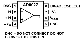
Figure 4. 8-Lead SOIC, AD8027 Pin Configuration
