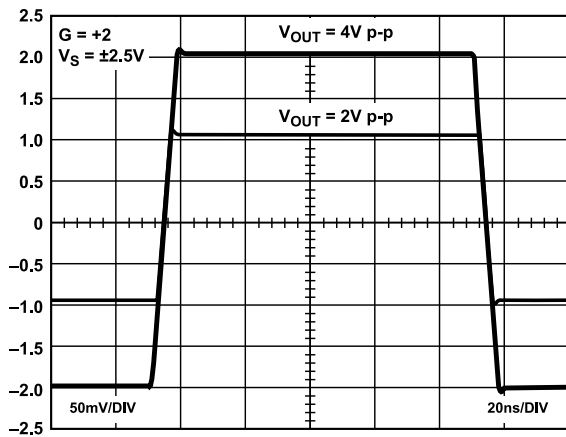
Figure 34. Large Signal Transient Response, G = +2
