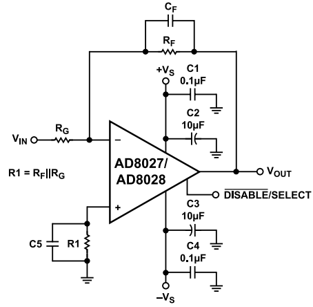
Figure 63. Wideband Inverting Gain Configuration
