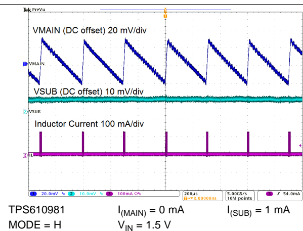
Figure 62. Switching Waveforms
