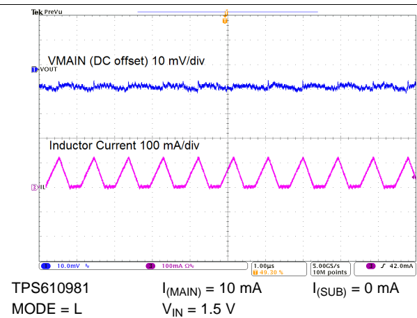
Figure 60. Switching Waveforms
