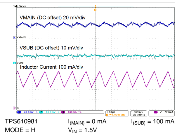
Figure 64. Switching Waveforms
