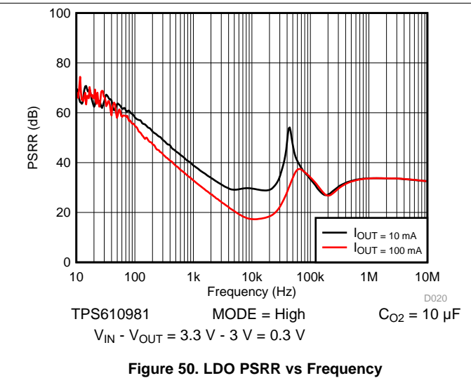
Figure 50. LDO PSRR vs Frequency
