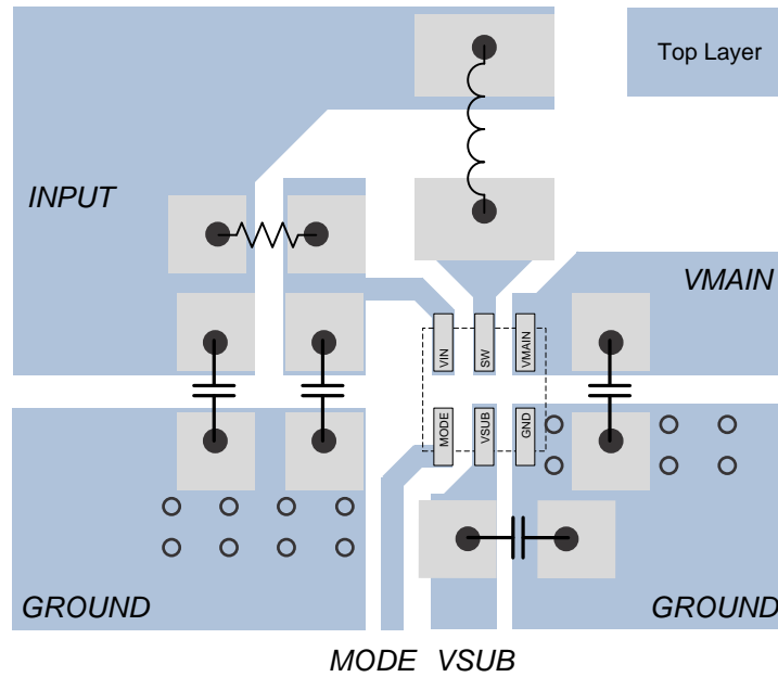
Figure 96. Layout
