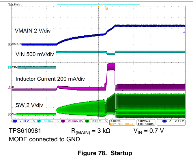
Figure 78. Startup
