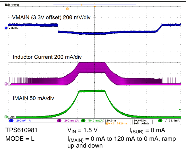
Figure 74. Load Regulation
