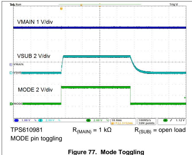
Figure 77. Mode Toggling
