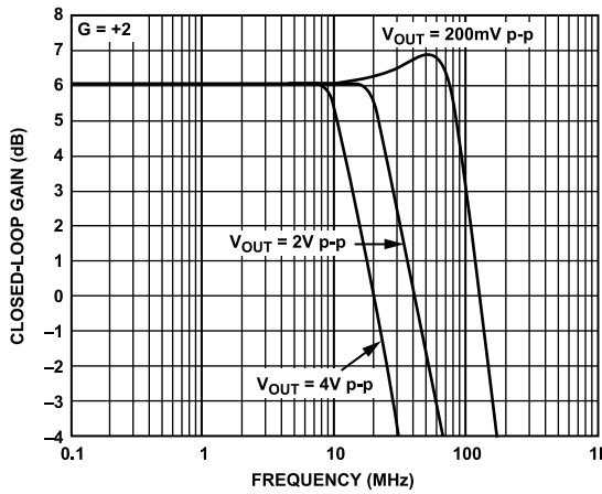
Figure 15. Frequency Response for Various Output Amplitudes
