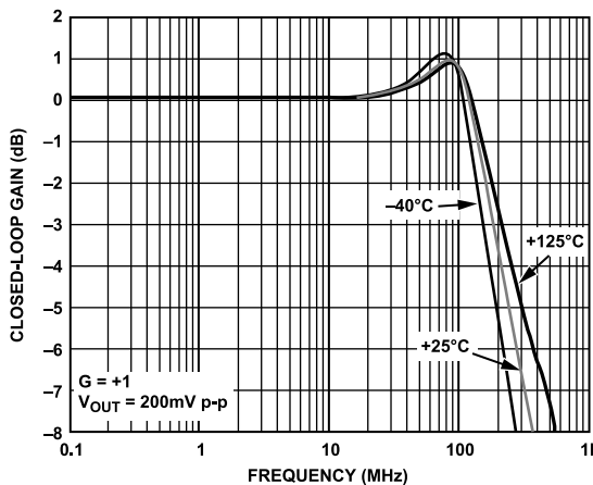
Figure 16. AD8027 Small Signal Frequency Response vs. Frequency for Various Temperatures
