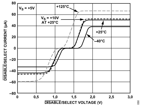
Figure 55. \overline{\text{DISABLE}}/\overline{\text{SELECT}} Current vs. \overline{\text{DISABLE}}/\overline{\text{SELECT}} Voltage and Temperature
