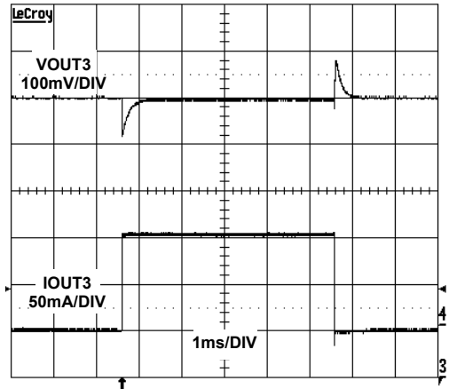
FIGURE 6. LDO3 TRANSIENT RESPONSE (10mA to 100mA)
