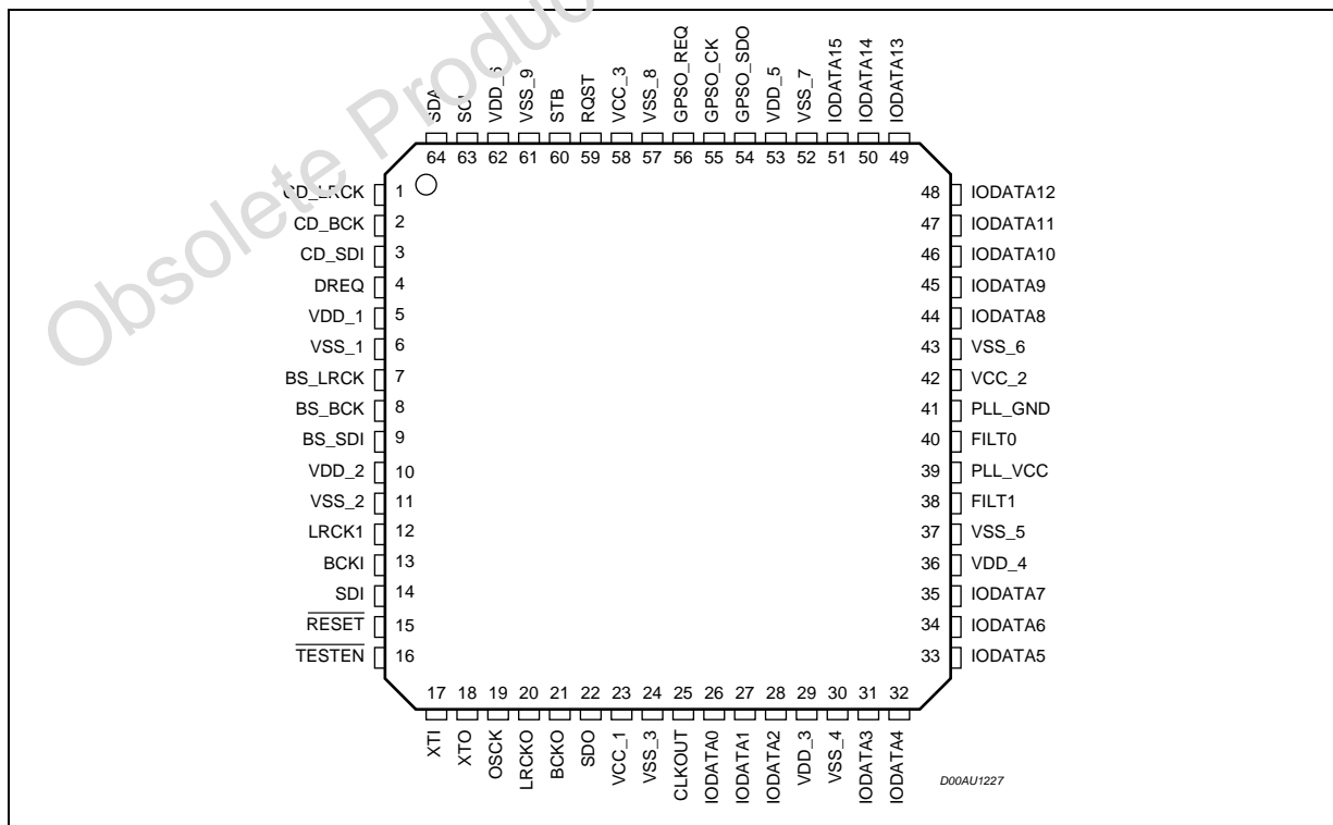
Figure 5. PIN CONNECTION
