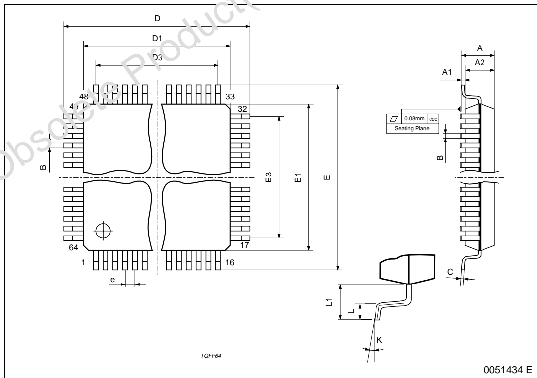
TQFP64 (10 x 10 x 1.4mm)
