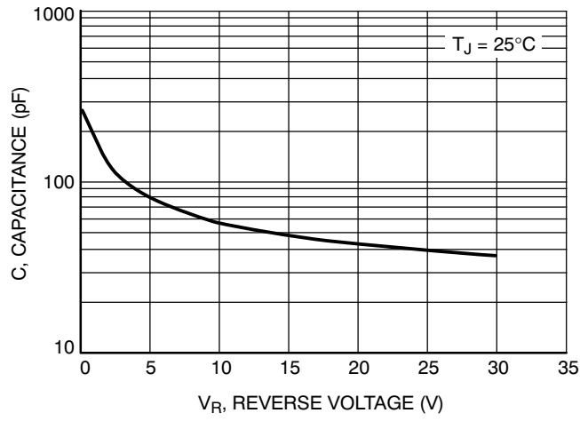
Figure 17. Capacitance
