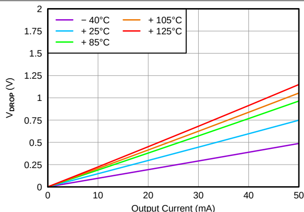
Figure 7. Dropout Voltage
