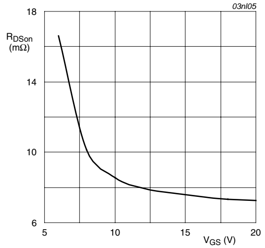
T_j = 25^\circ\text{C}; V_{DS} = 25\text{V}
