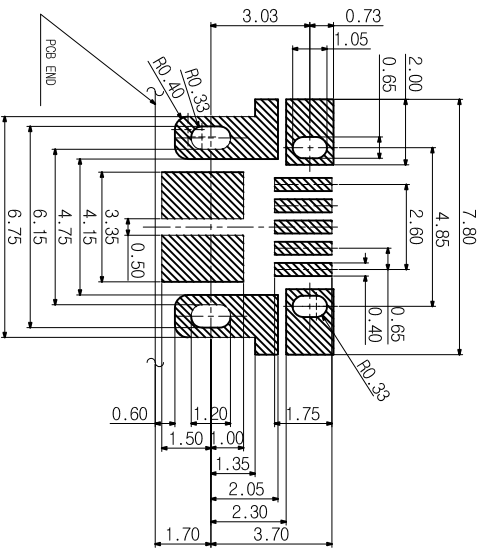
RECOMMENDED PCB Pattern (Tolerance : ±0.05)
