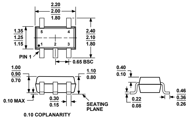
COMPLIANT TO JEDEC STANDARDS MO-203-AA Figure 47. 5-Lead Thin Shrink Small Outline Transistor Package [SC70] (KS-5) Dimensions shown in millimeters
