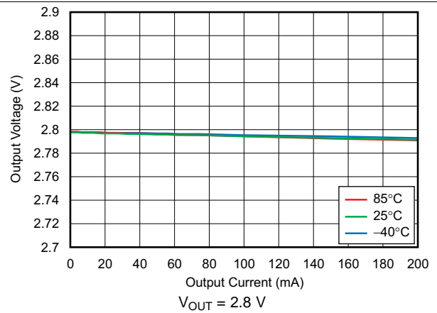
Figure 2. Load Regulation
