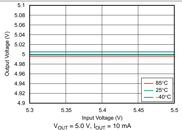
Figure 6. Line Regulation
