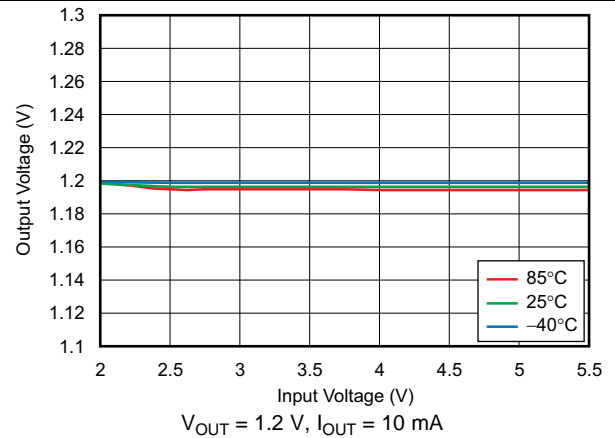
Figure 4. Line Regulation
