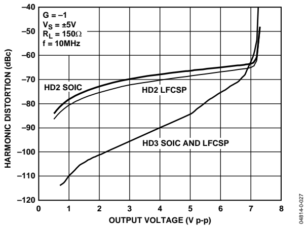
Figure 27. Harmonic Distortion vs. Output Voltage
