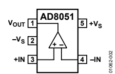
Figure 2. SOT-23-5 (R)
