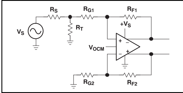
Figure 98. Application Circuit for the THS4500 and THS4501, Featuring Single-Supply Operation With a Ground-Reference Input Signal
