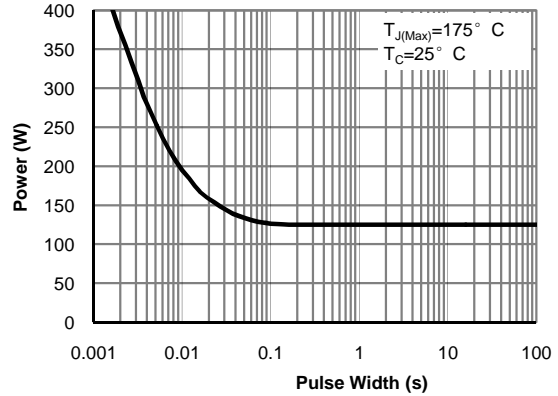
Figure 10: Single Pulse Power Rating Junction-to-C a (Note F)
