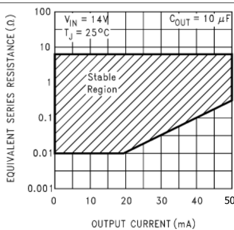
Figure 8. 3-V LM2936Q C OUT ESR
