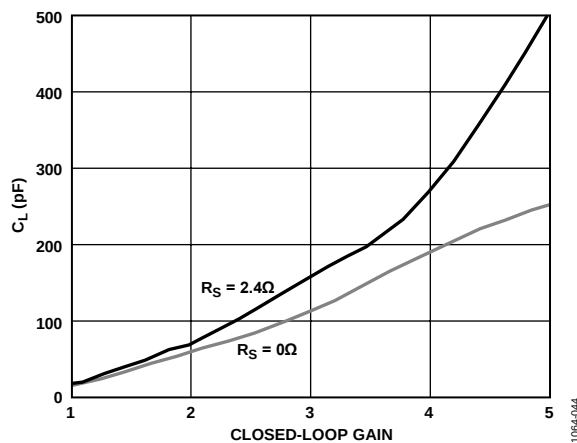
Figure 43. Capacitive Load Drive vs. Closed-Loop Gain
