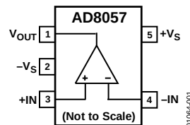
Figure 1. RT-5 (SOT-23)
