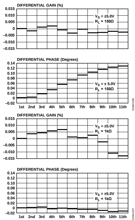
Figure 34. Differential Gain and Differential Phase One Back Terminated Load ( 150\Omega ) (Video Op Amps Only)
