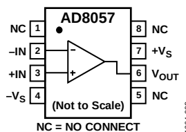
Figure 2. R-8 (SOIC)
