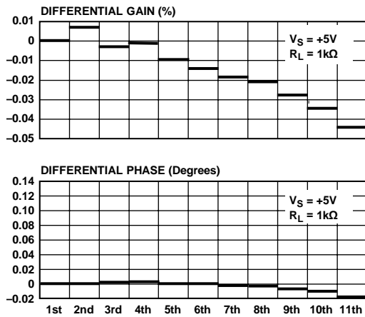
Figure 37. Differential Gain and Differential Phase, R_L = 1k\Omega
