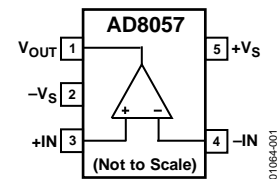
Figure 1. RT-5 (SOT-23)
