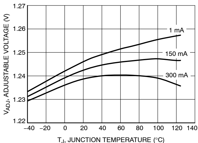
Figure 6. Adjustable Voltage vs. Temperature
