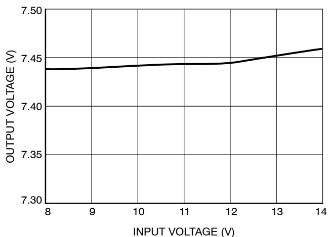
Figure 4. Line Regulation
