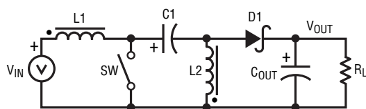
20a. SEPIC Topology
