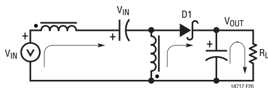
20c. Current Flow During Switch Off-Time
