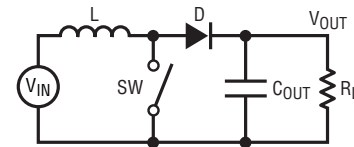
13a. Circuit Diagram
