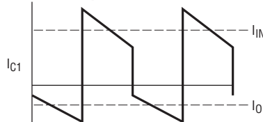
21c. DC Coupling Capacitor Current
