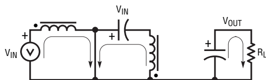
20b. Current Flow During Switch On-Time
