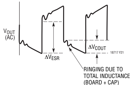
21e. Output Ripple Voltage
