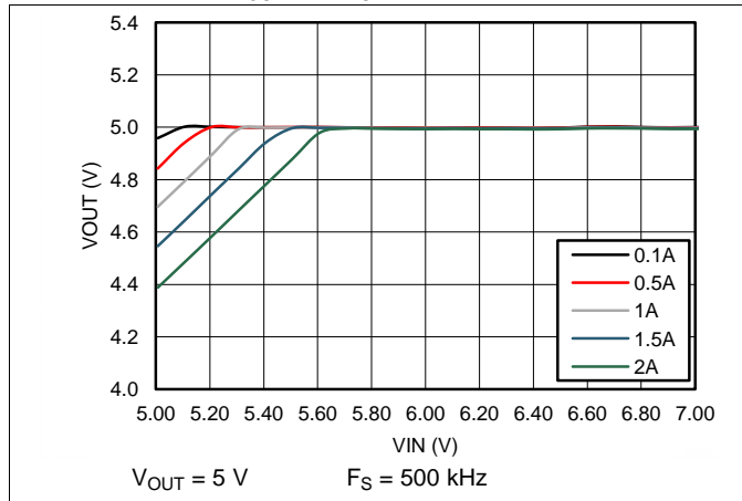
Figure 57. Dropout Voltage
