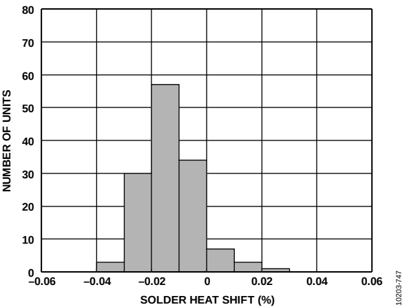
Figure 43. ADR4530 Solder Heat Resistance Shift (3 \times Reflow)
