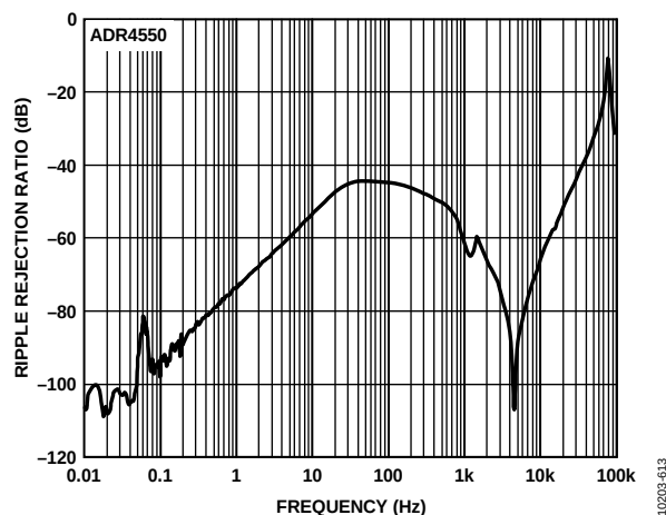
Figure 79. ADR4550 Ripple Rejection Ratio vs. Frequency
