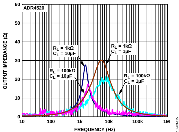
Figure 14. ADR4520 Output Impedance vs. Frequency
