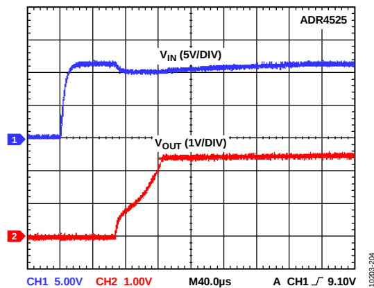
Figure 18. ADR4525 Output Voltage Start-Up Response
