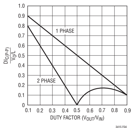
Figure 4. Normalized Output Ripple Current [ I_{RMS} \approx 0.3 (DI_C(PP)) ]
