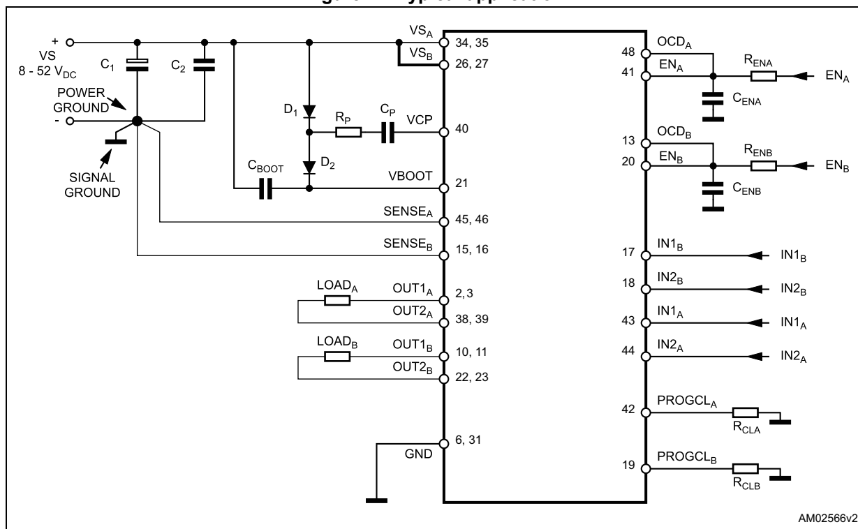
Figure 14. Typical application
