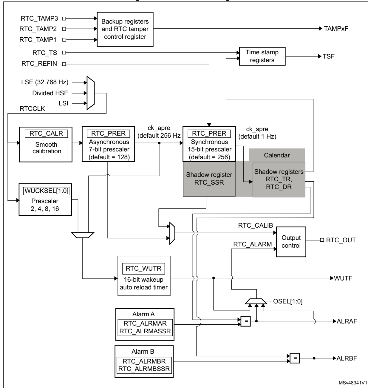
Figure 348. RTC block diagram
