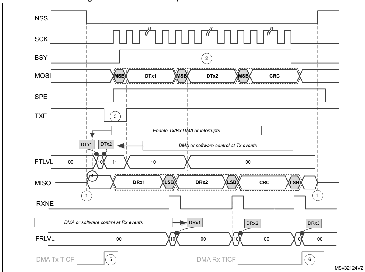
Figure 417. Master full-duplex communication with CRC
