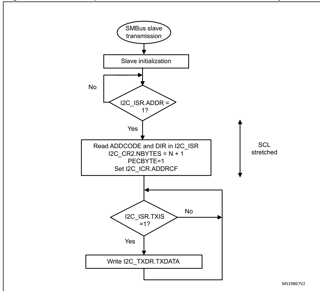
Figure 373. Transfer sequence flowchart for SMBus slave transmitter N bytes + PEC
