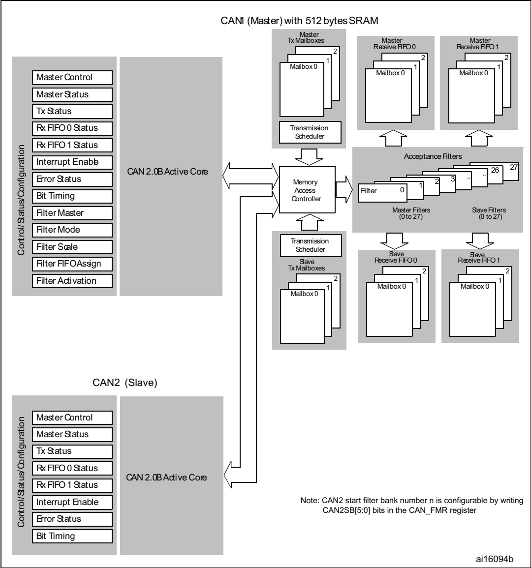
Figure 493. Dual-CAN block diagram
