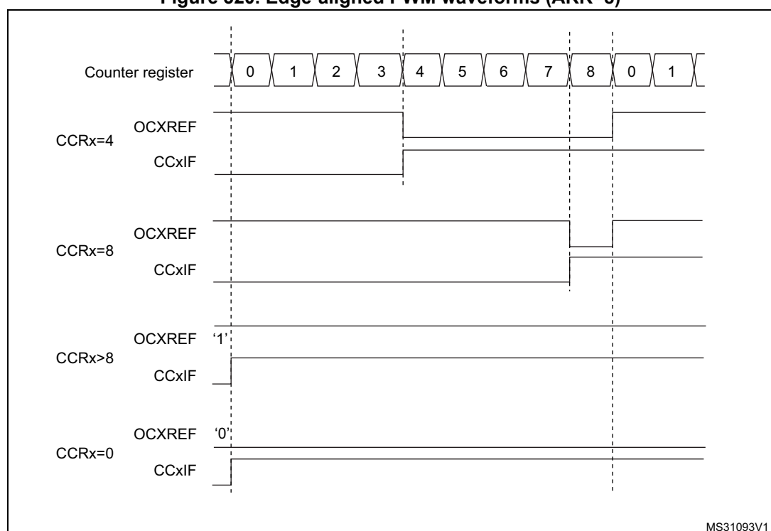
Figure 320. Edge-aligned PWM waveforms (ARR=8)
