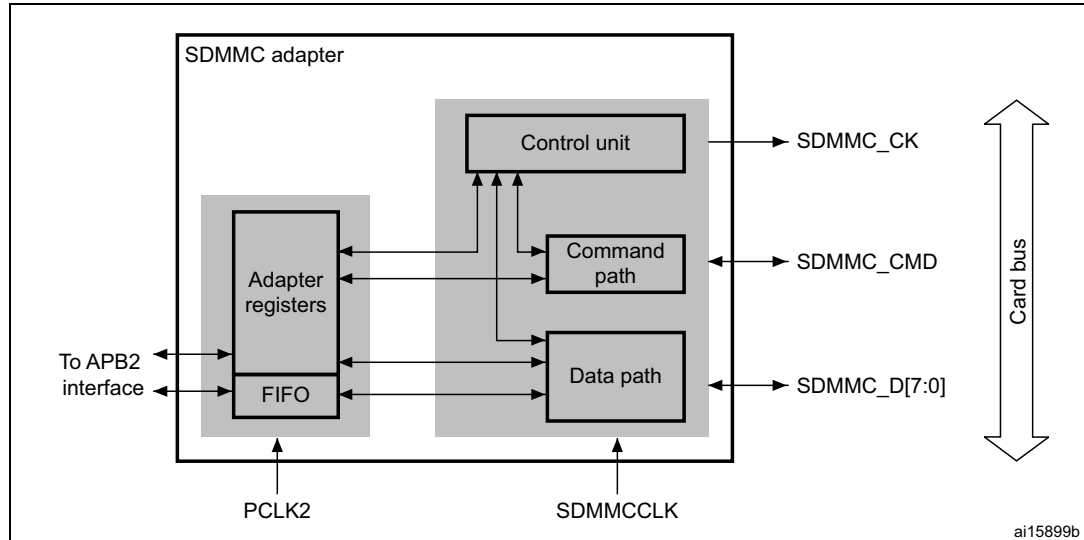
Figure 484. SDMMC adapter
