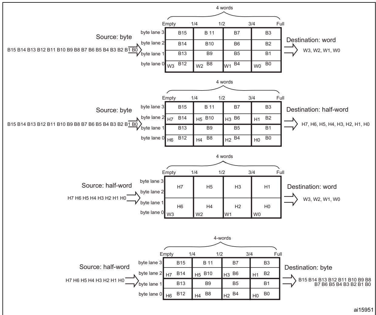
Figure 28. FIFO structure
