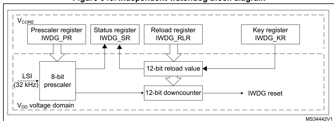
Figure 345. Independent watchdog block diagram
