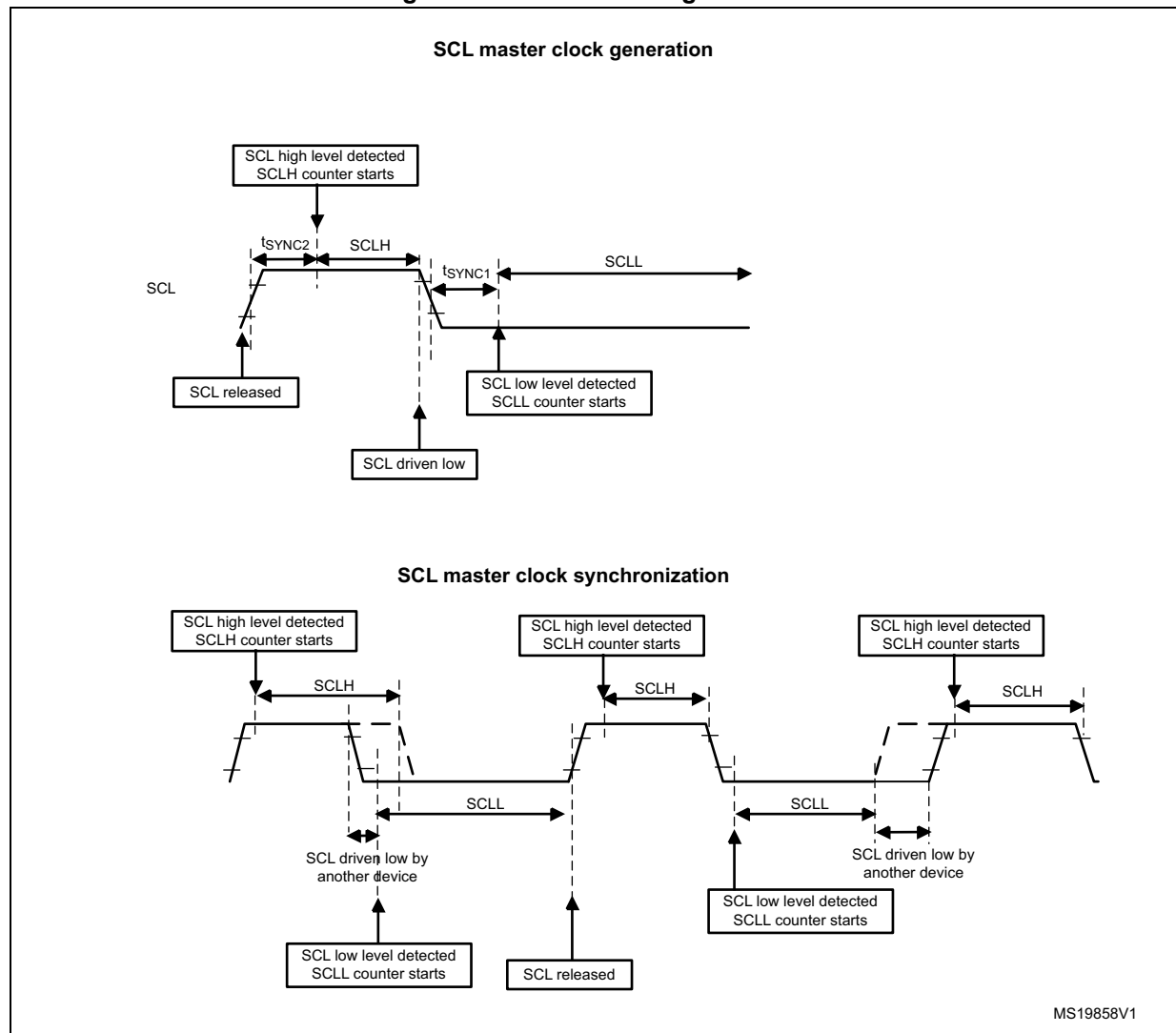
Figure 362. Master clock generation
