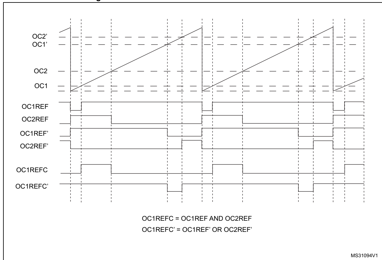
Figure 232. Combined PWM mode on channel 1 and 3
