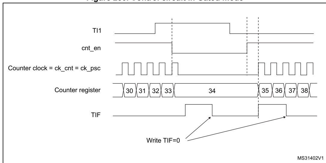
Figure 250. Control circuit in Gated mode
