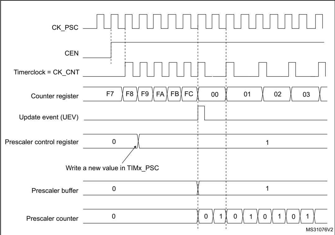
Figure 304. Counter timing diagram with prescaler division change from 1 to 2
