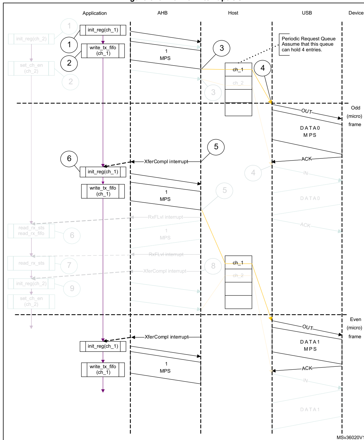
Figure 523. Normal interrupt OUT
