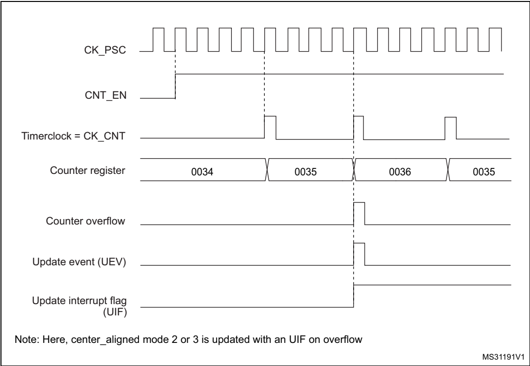
Figure 211. Counter timing diagram, internal clock divided by 4, TIMx_ARR=0x36
