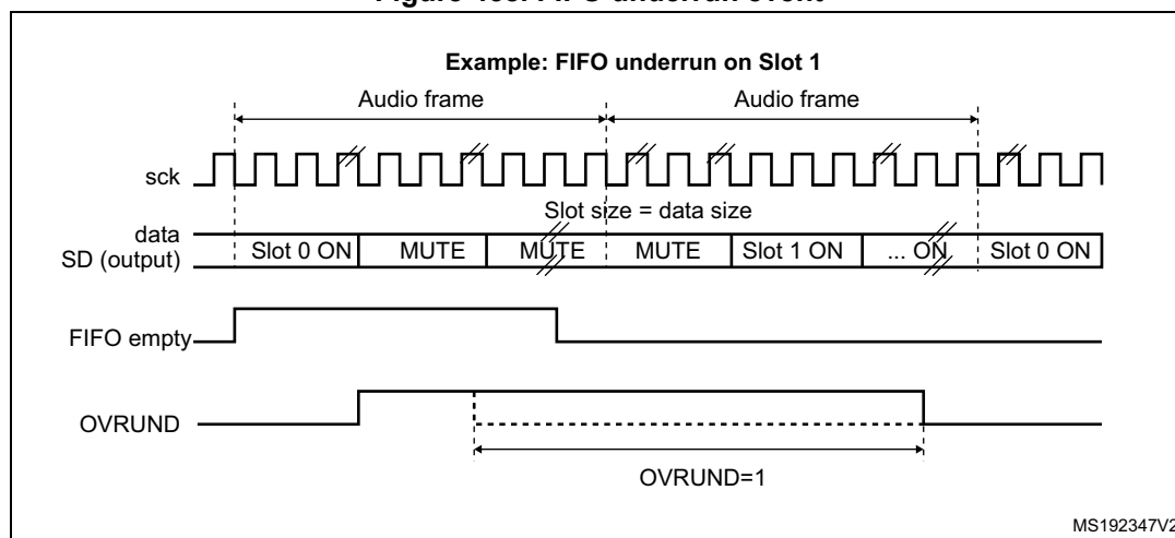
Figure 458. FIFO underrun event
