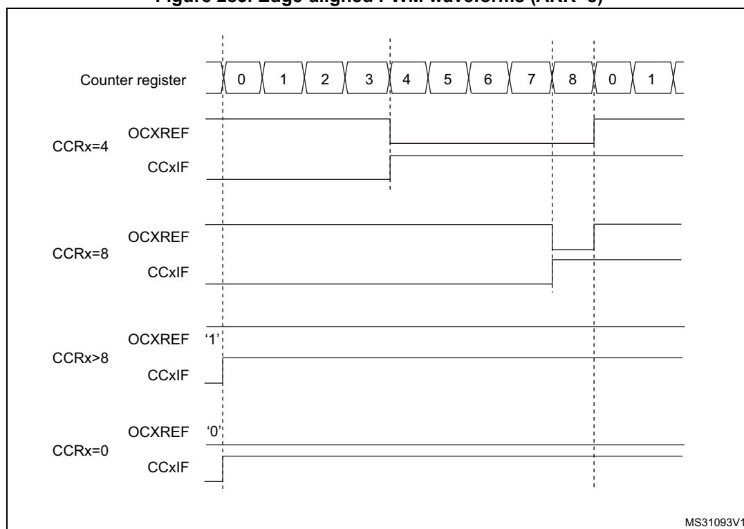
Figure 283. Edge-aligned PWM waveforms (ARR=8)
