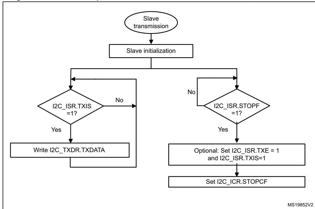
Figure 357. Transfer sequence flowchart for I2C slave transmitter, NOSTRETCH=1
