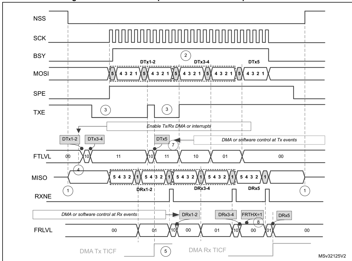
Figure 418. Master full-duplex communication in packed mode
