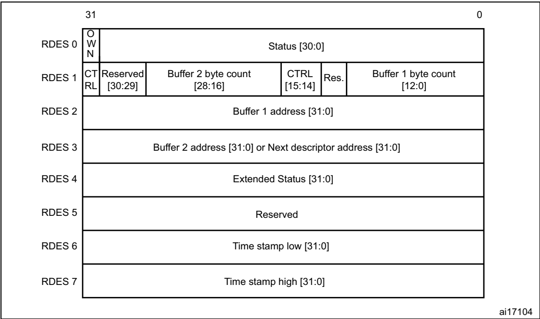
Figure 574. Enhanced receive descriptor field format with IEEE1588 time stamp enabled
