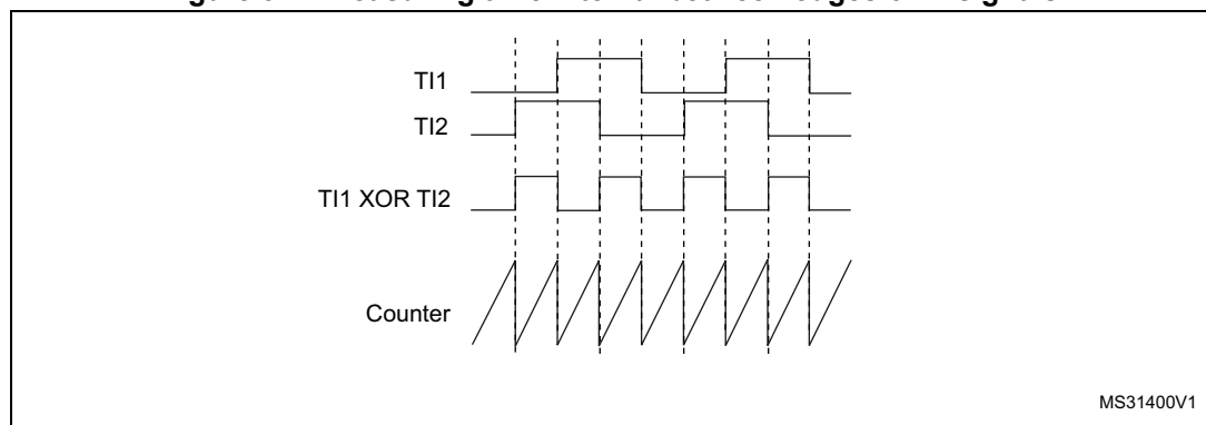
Figure 324. Measuring time interval between edges on 2 signals
