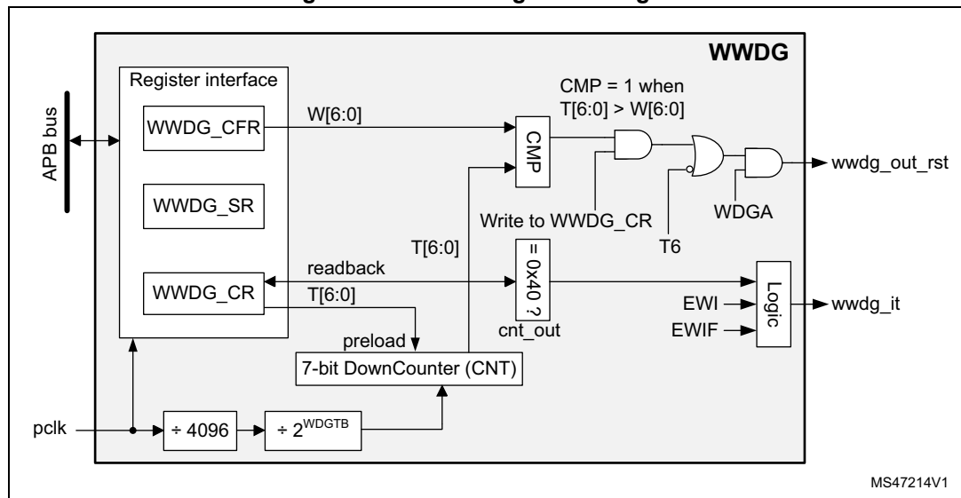
Figure 346. Watchdog block diagram
