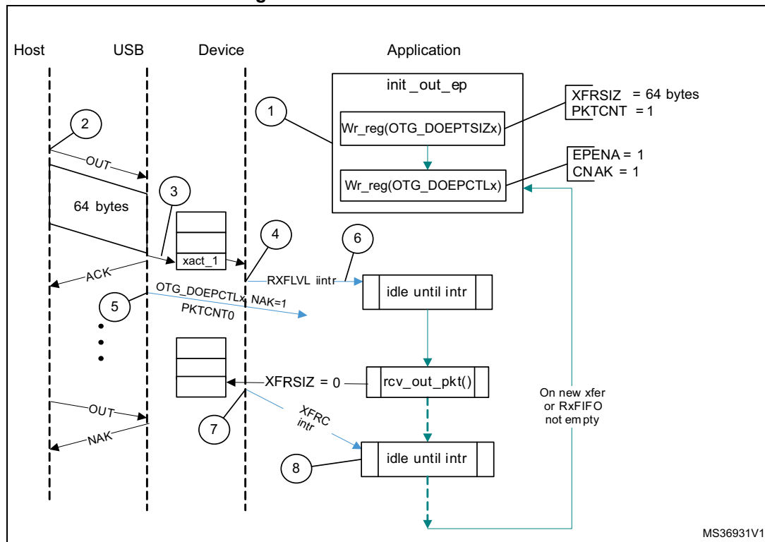
Figure 535. Bulk OUT transaction
