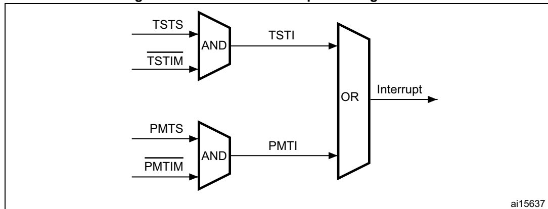
Figure 561. MAC core interrupt masking scheme
