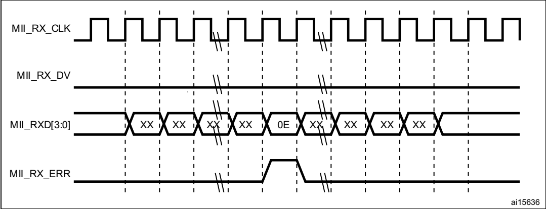
Figure 560. Reception with false carrier indication
