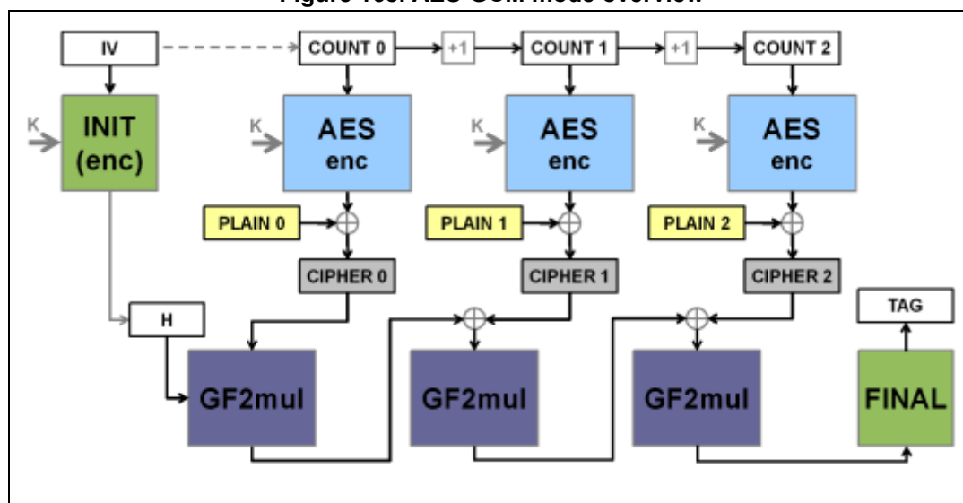
Figure 168. AES-GCM mode overview
