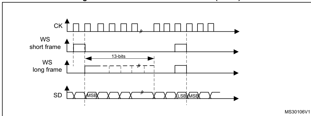
Figure 438. PCM standard waveforms (16-bit)
