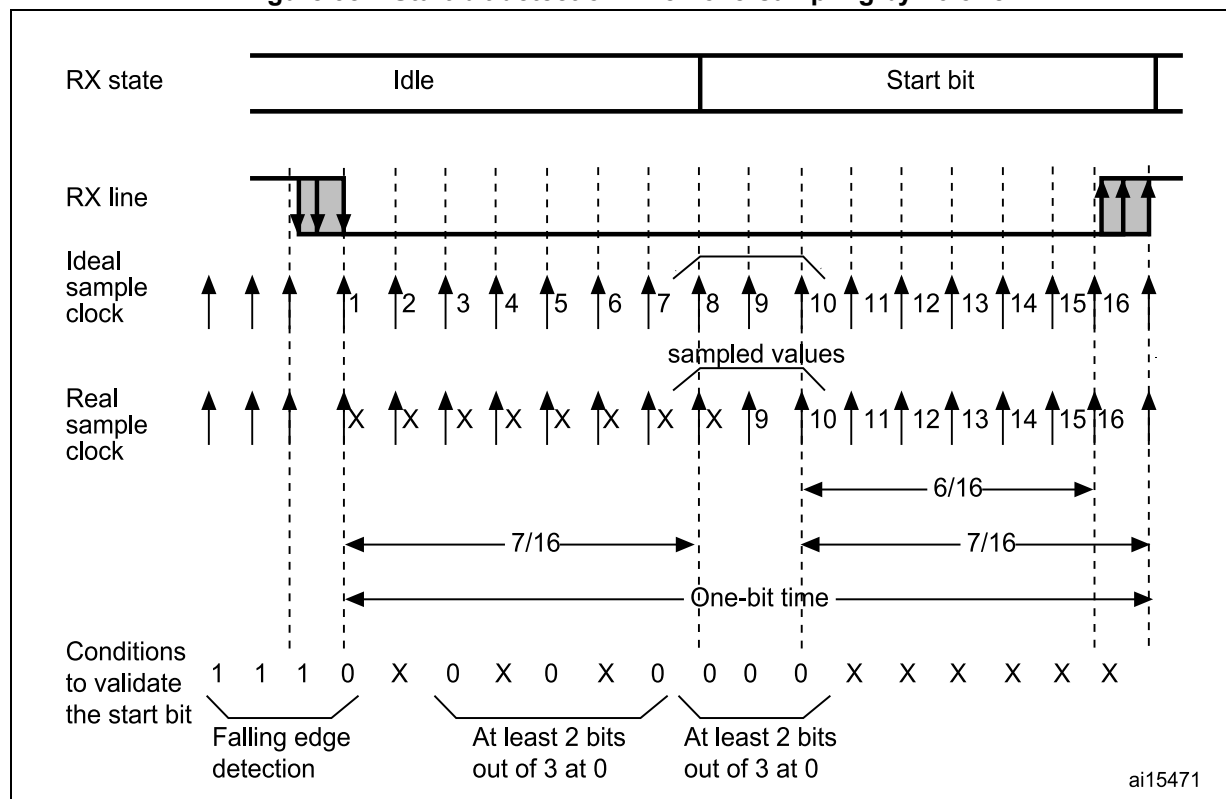
Figure 384. Start bit detection when oversampling by 16 or 8
