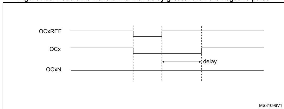
Figure 235. Dead-time waveforms with delay greater than the negative pulse
