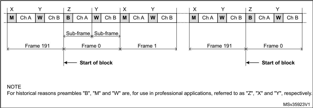
Figure 461. S/PDIF block format
