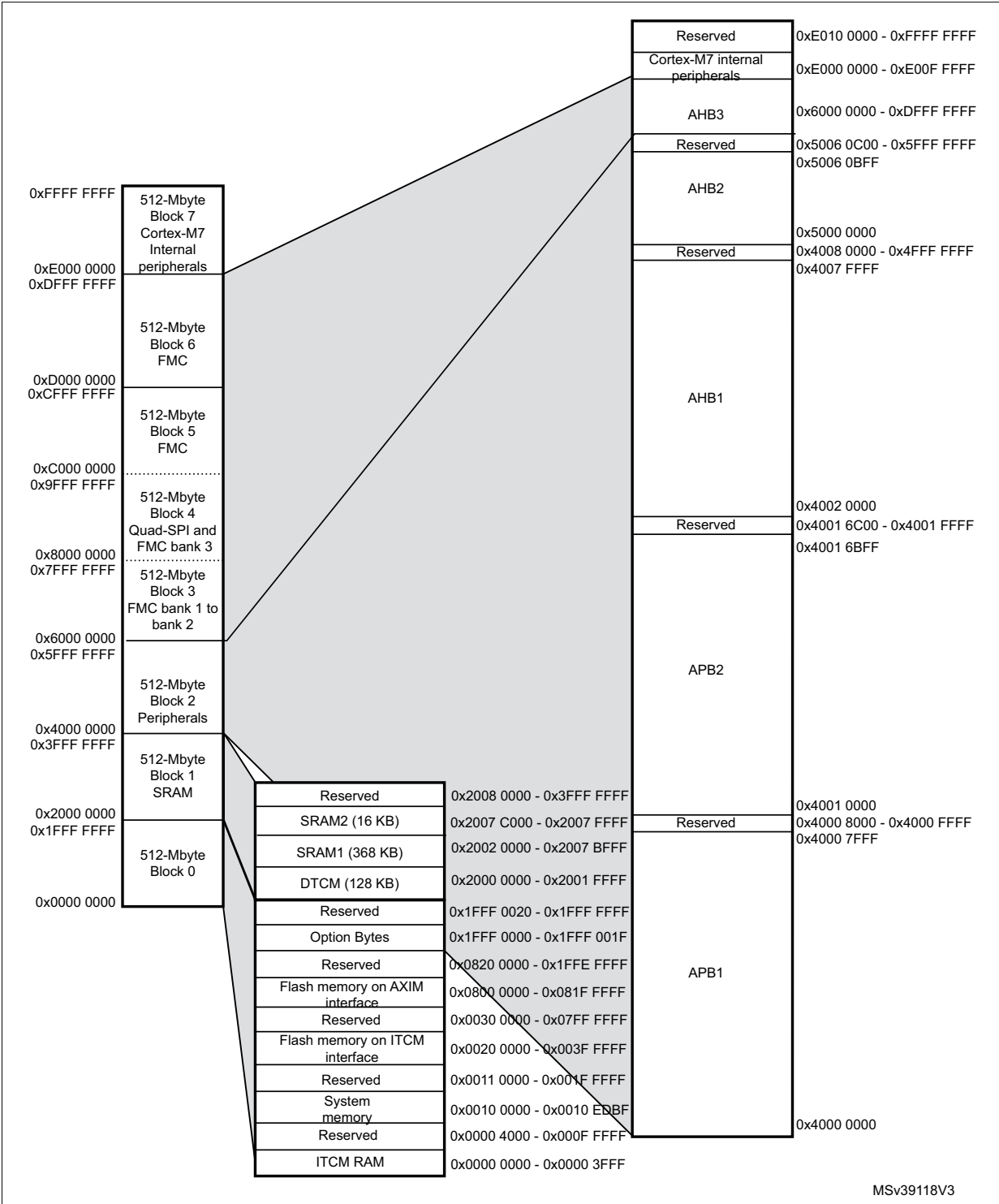
Figure 2. Memory map
