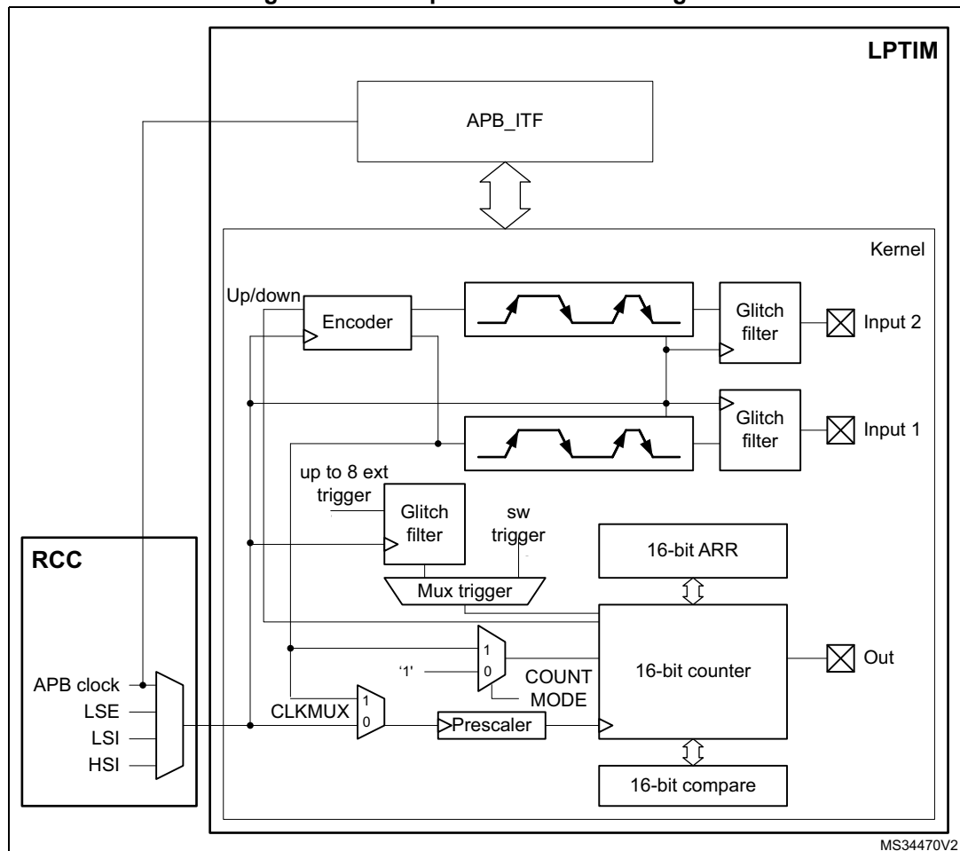
Figure 338. Low-power timer block diagram
