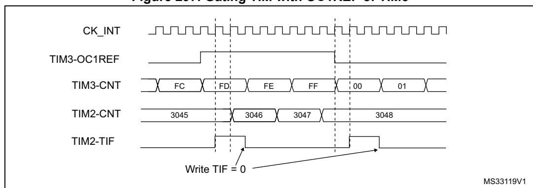
Figure 297. Gating TIM with OC1REF of TIM3
