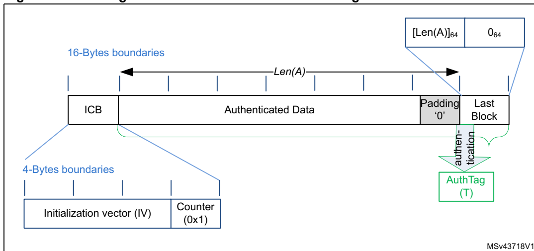
Figure 186. Message construction for the Galois Message Authentication Code mode
