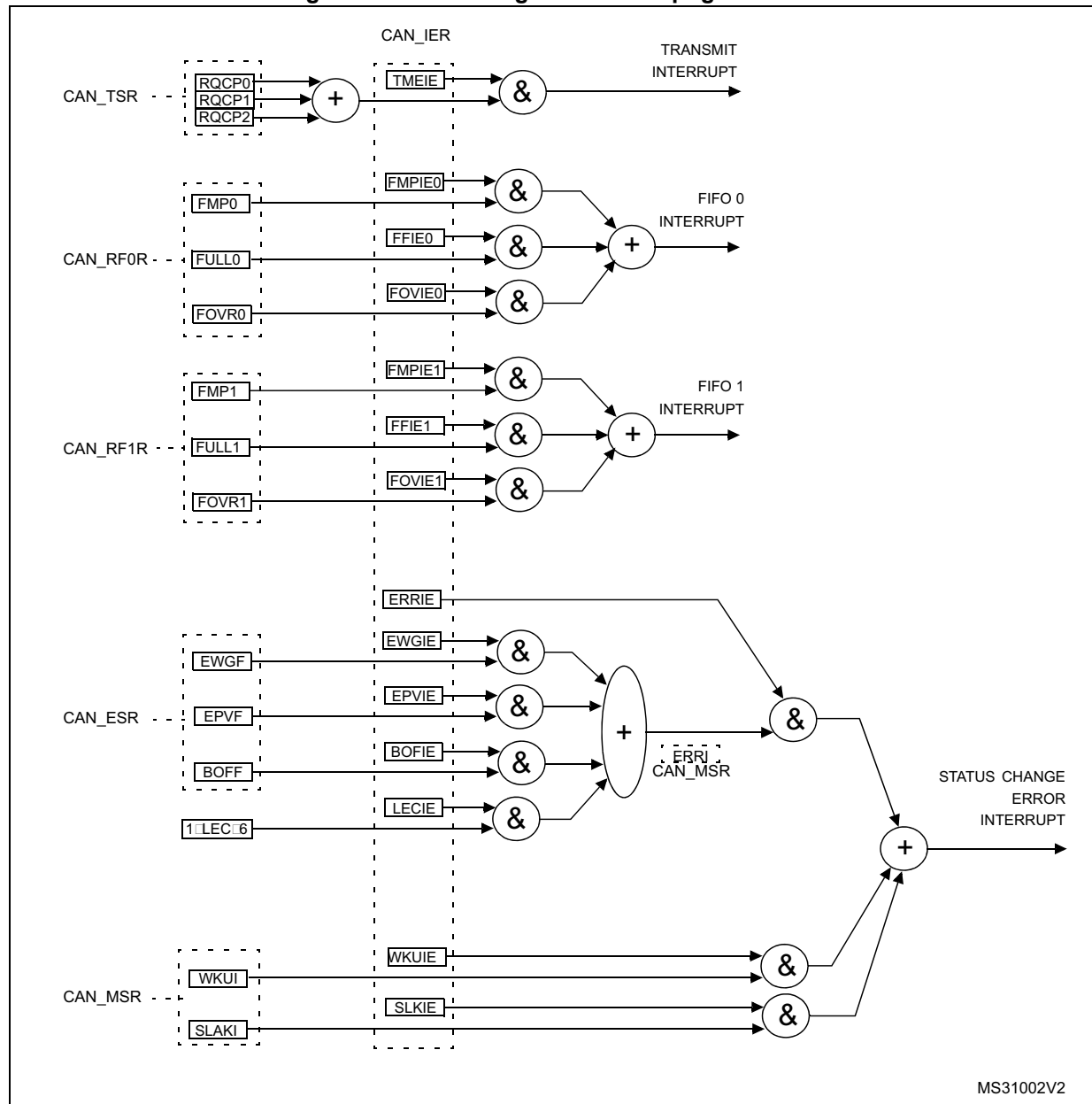
Figure 507. Event flags and interrupt generation
