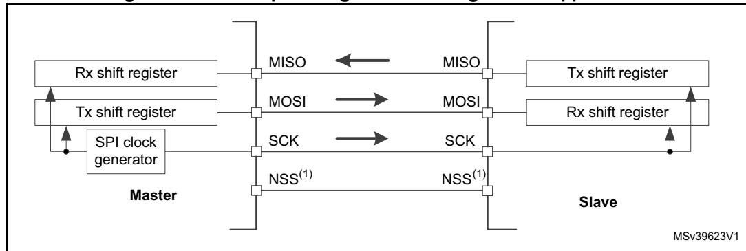
Figure 406. Full-duplex single master/ single slave application
