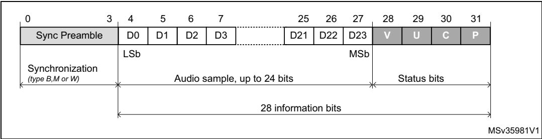
Figure 460. S/PDIF Sub-Frame Format
