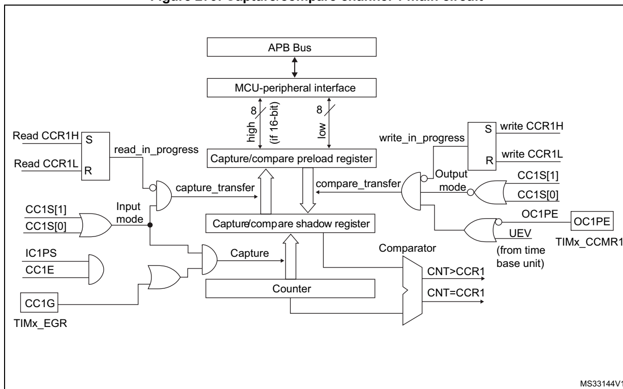
Figure 279. Capture/compare channel 1 main circuit
