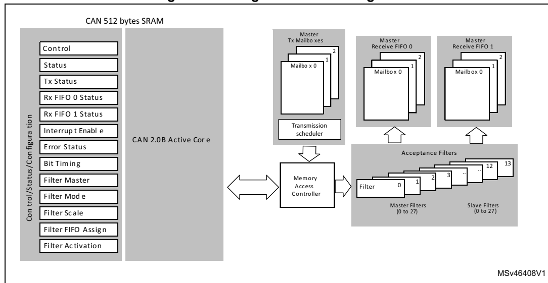
Figure 494. Single-CAN block diagram
