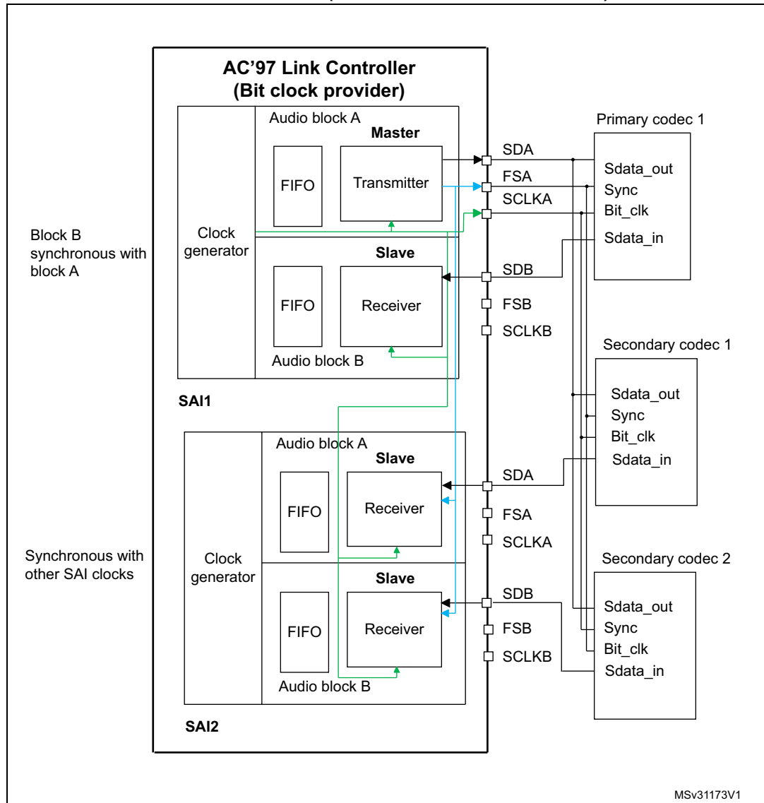
Figure 451. Example of typical AC'97 configuration on devices featuring at least 2 embedded SAIs (three external AC'97 decoders)
