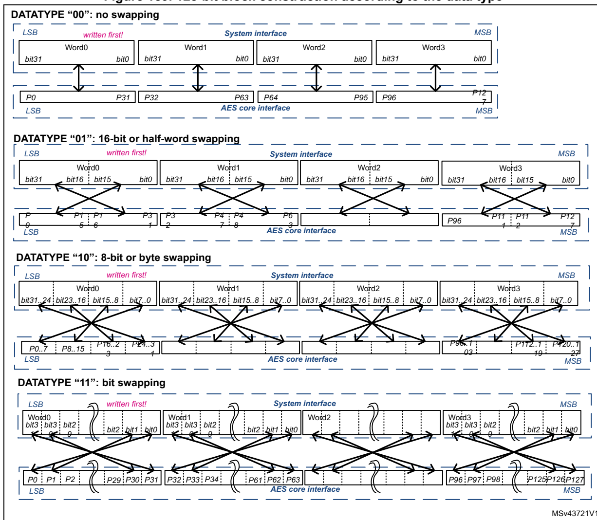
Figure 189. 128-bit block construction according to the data type
