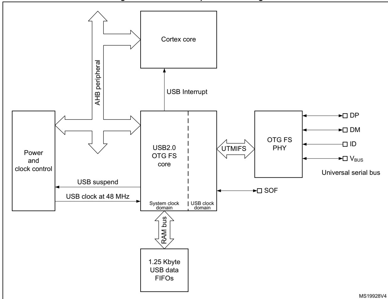
Figure 509. OTG full-speed block diagram
