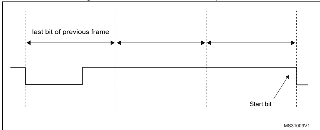
Figure 583. SFT of three nominal bit periods
