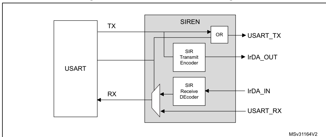
Figure 397. IrDA SIR ENDEC- block diagram
