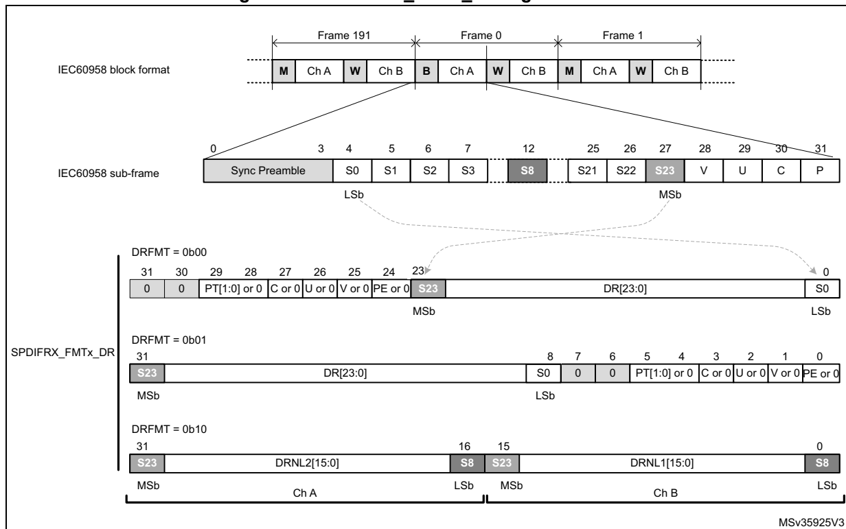
Figure 470. SPDIFRX_FMTx_DR register format
