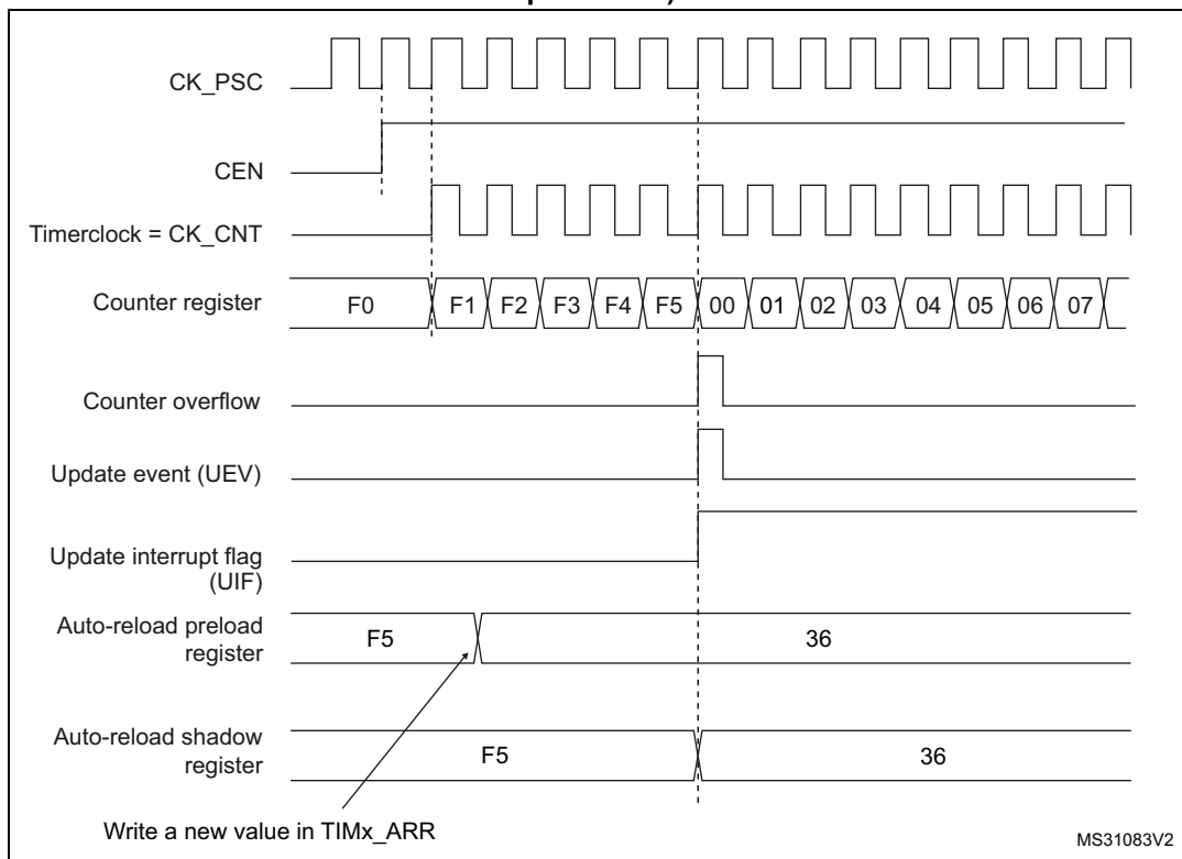
Figure 336. Counter timing diagram, update event when ARPE=1 (TIMx_ARR preloaded)
