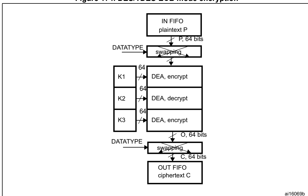
Figure 174. DES/TDES-ECB mode encryption
