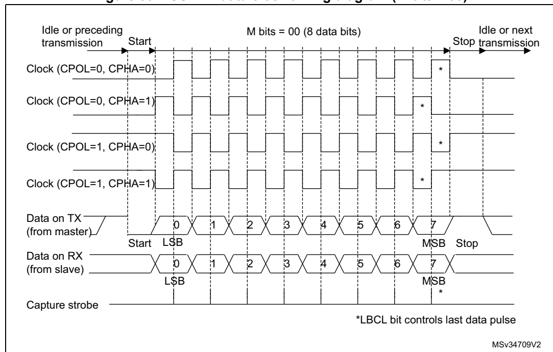
Figure 392. USART data clock timing diagram (M bits = 00)
