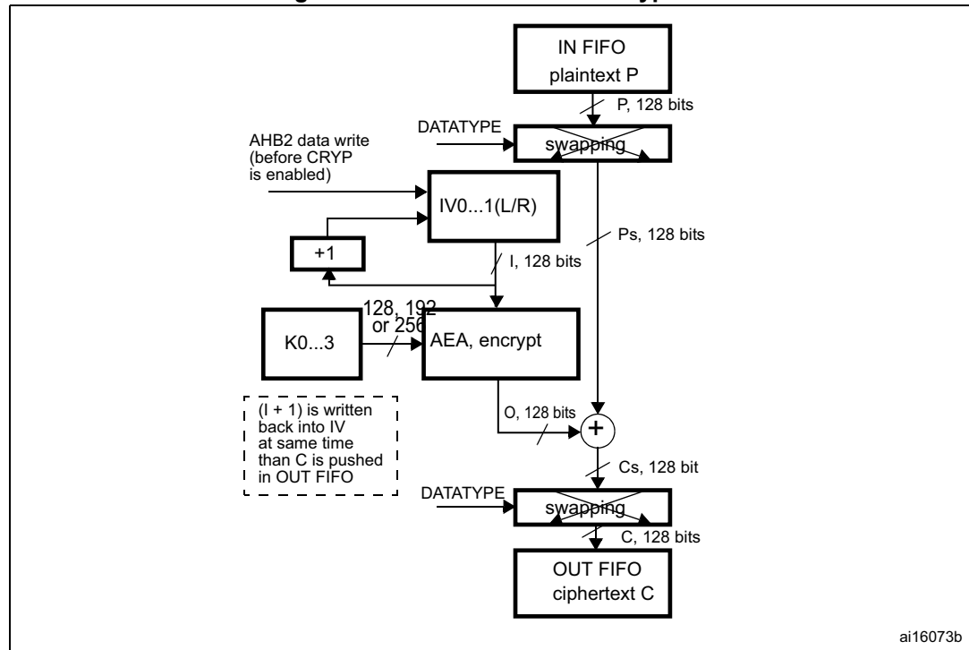
Figure 183. AES-CTR mode encryption
