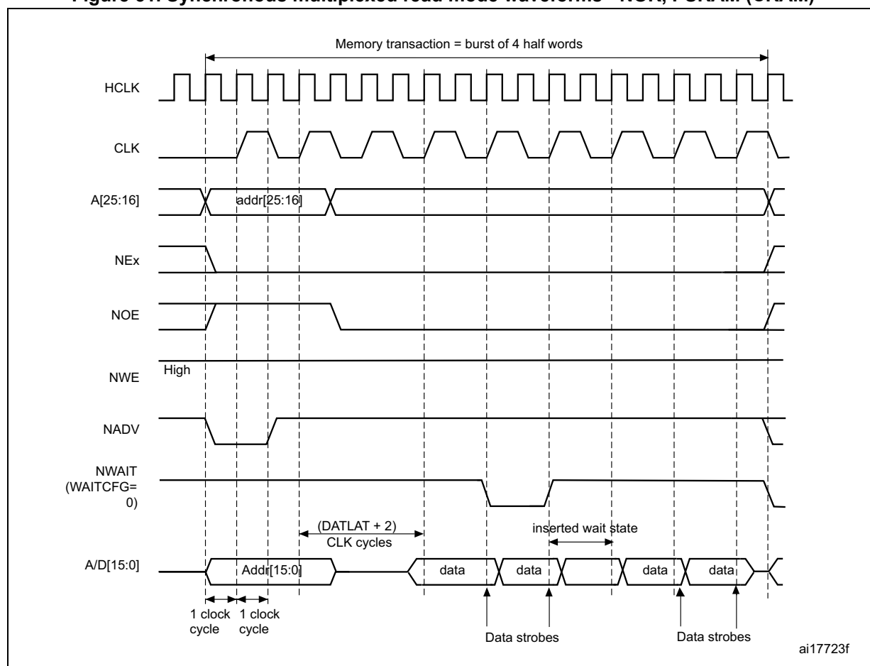
Figure 51. Synchronous multiplexed read mode waveforms - NOR, PSRAM (CRAM)
