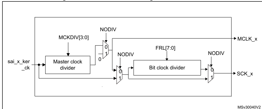
Figure 449. Audio block clock generator overview
