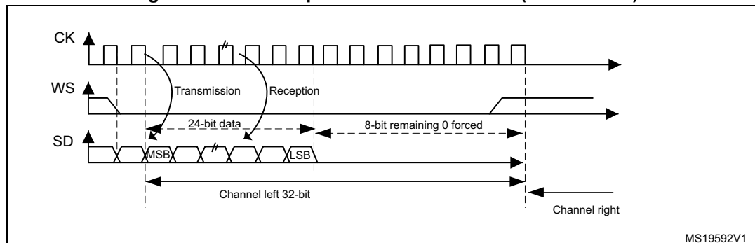
Figure 424. I 2 S Philips standard waveforms (24-bit frame)
