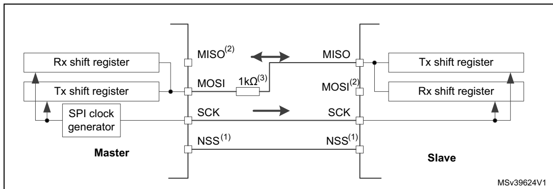
Figure 407. Half-duplex single master/ single slave application
