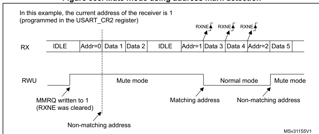
Figure 388. Mute mode using address mark detection
