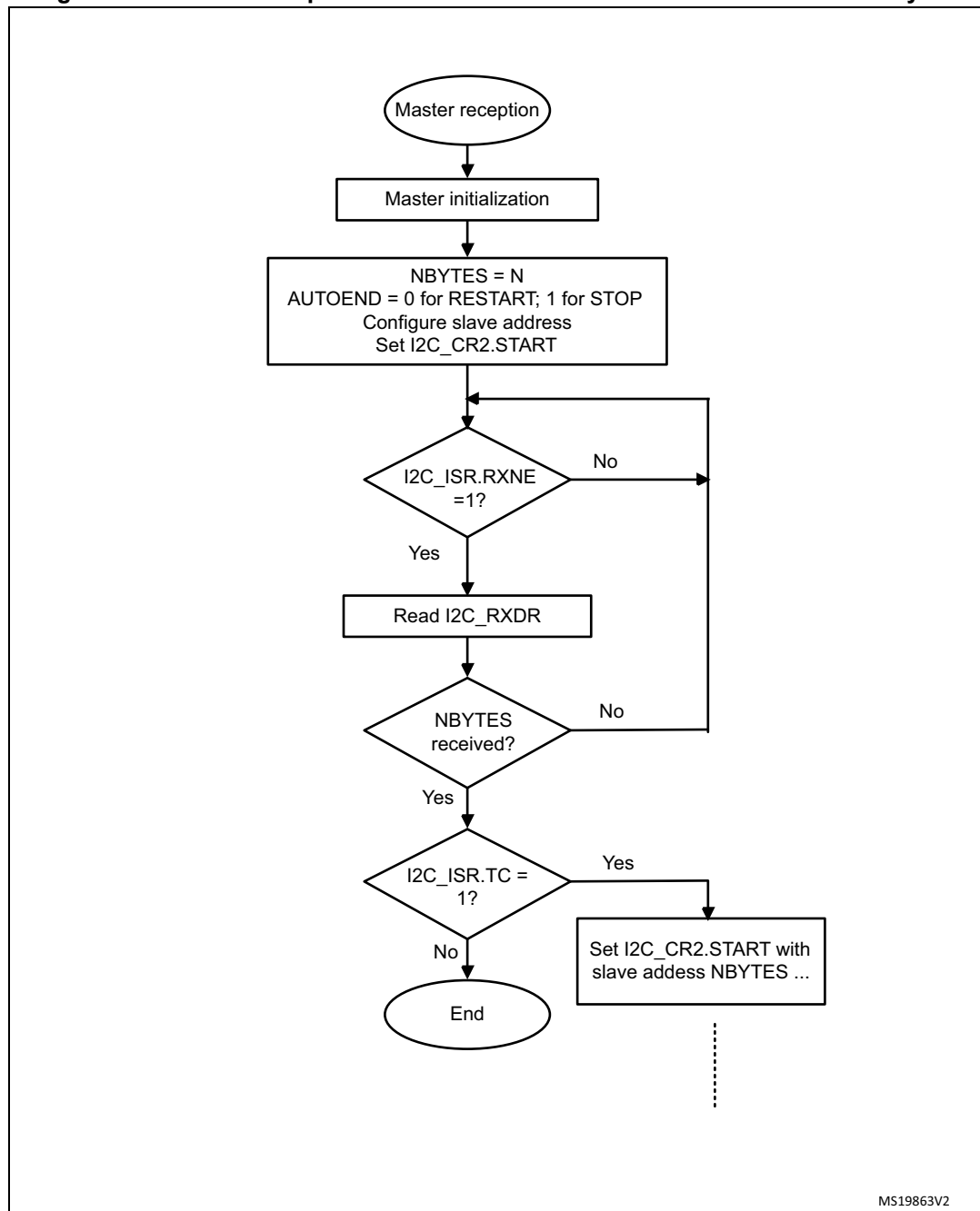
Figure 369. Transfer sequence flowchart for I2C master receiver for N \leq 255 bytes
