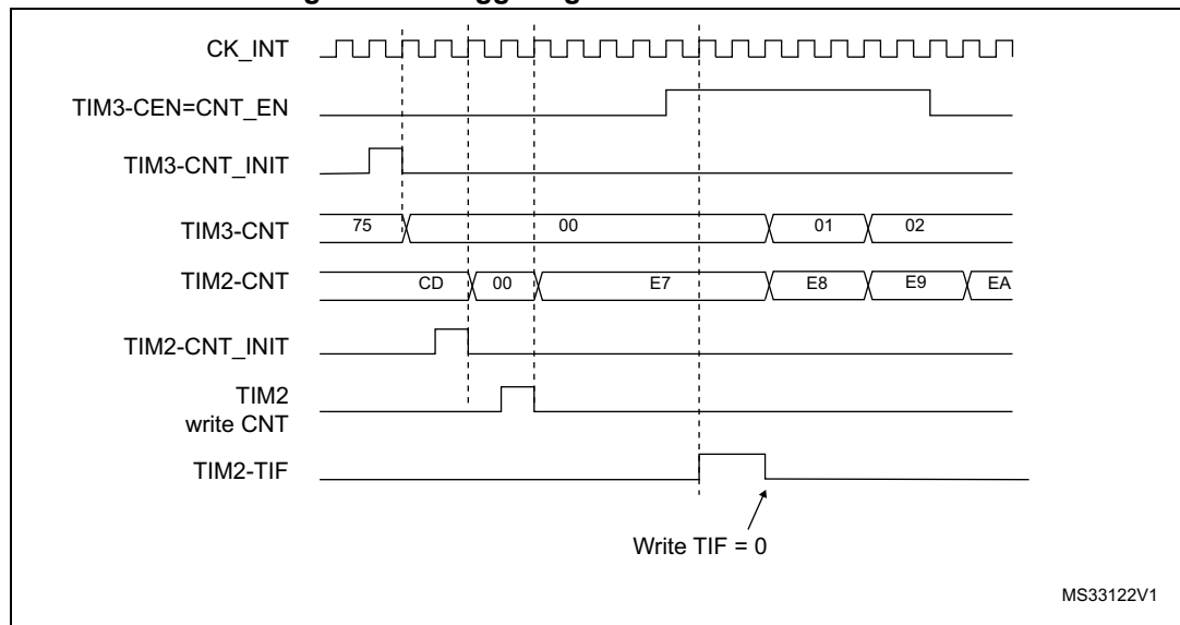
Figure 300. Triggering TIM with Enable of TIM3
