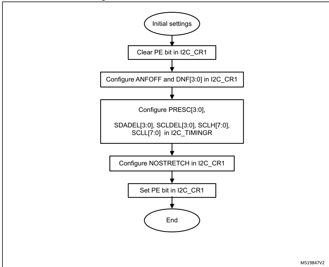
Figure 352. I2C initialization flowchart
