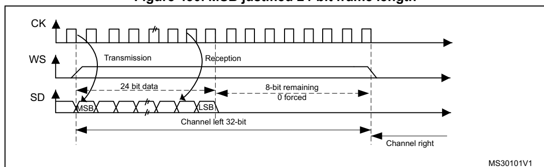
Figure 430. MSB justified 24-bit frame length
