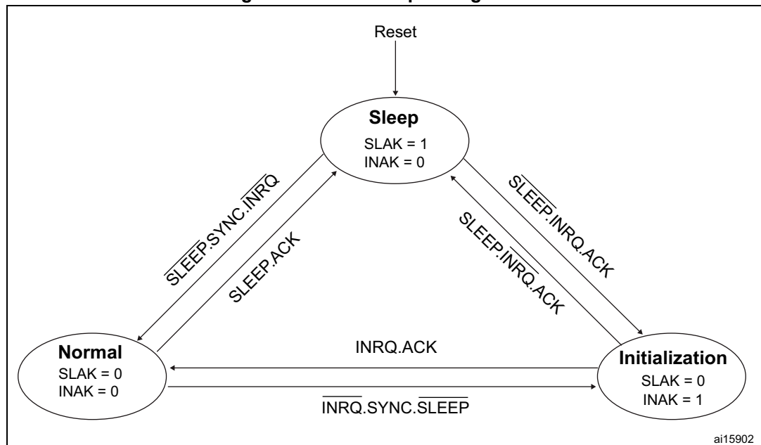
Figure 495. bxCAN operating modes
