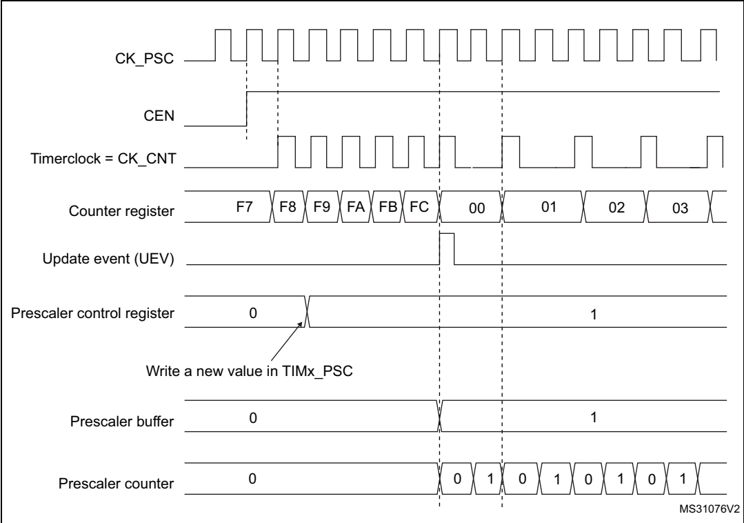
Figure 196. Counter timing diagram with prescaler division change from 1 to 2
