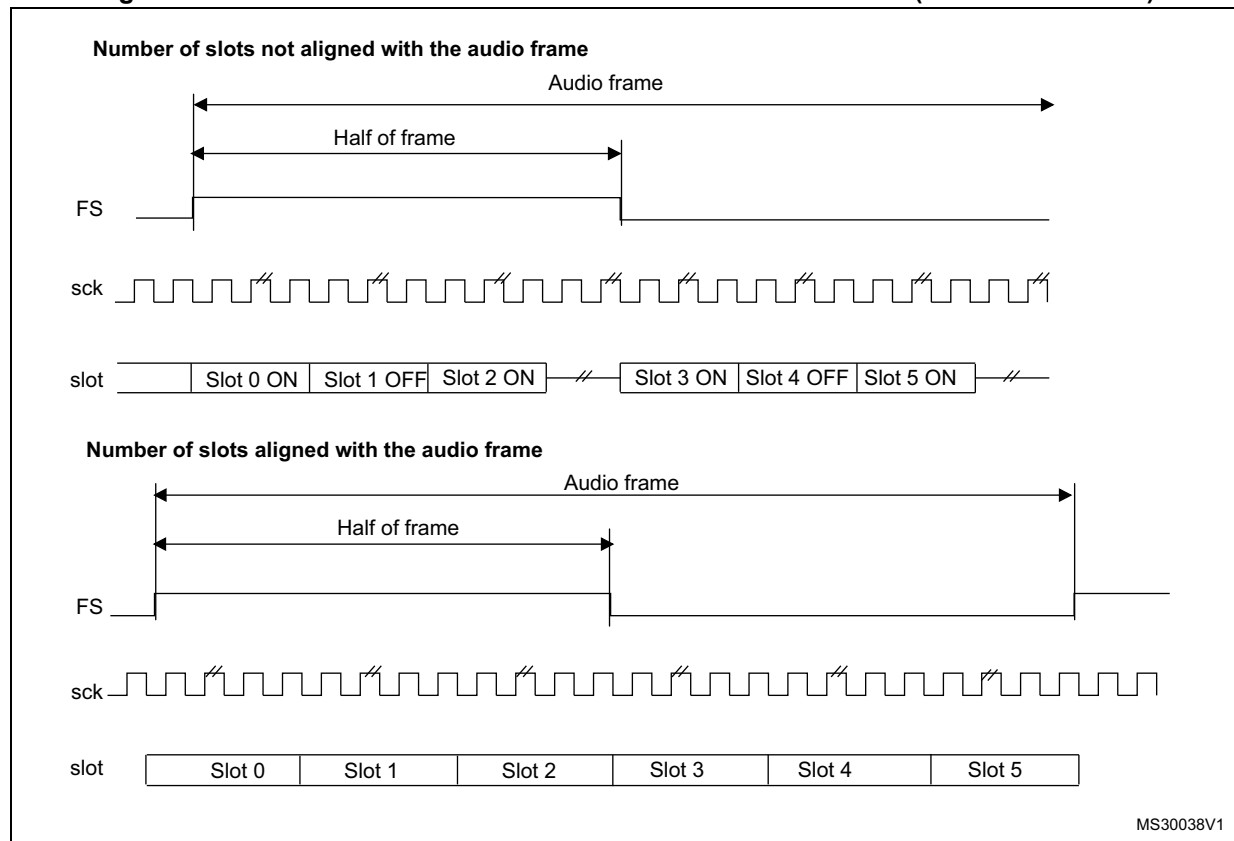
Figure 445. FS role is start of frame + channel side identification (FSDEF = TRIS = 1)
