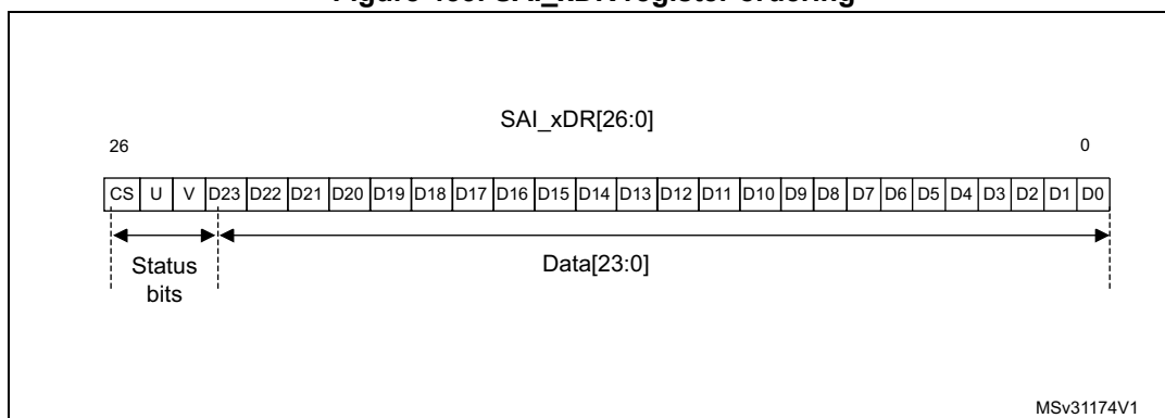
Figure 453. SAI_xDR register ordering
