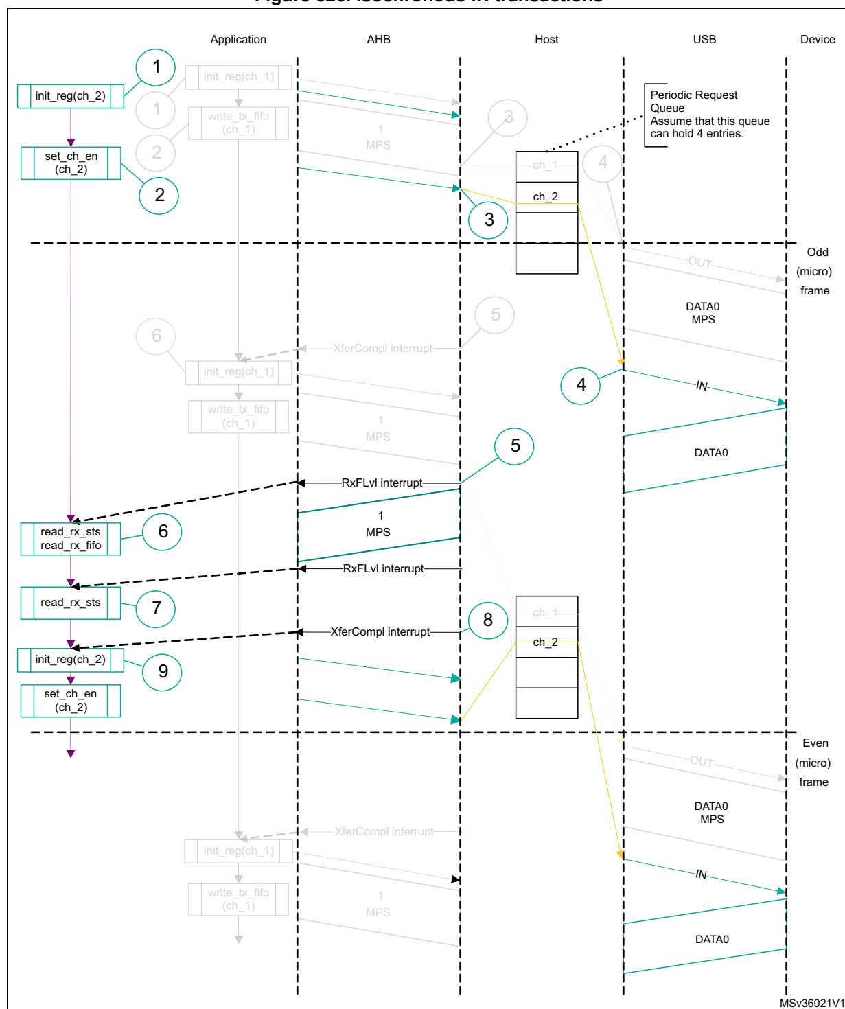
Figure 526. Isochronous IN transactions
