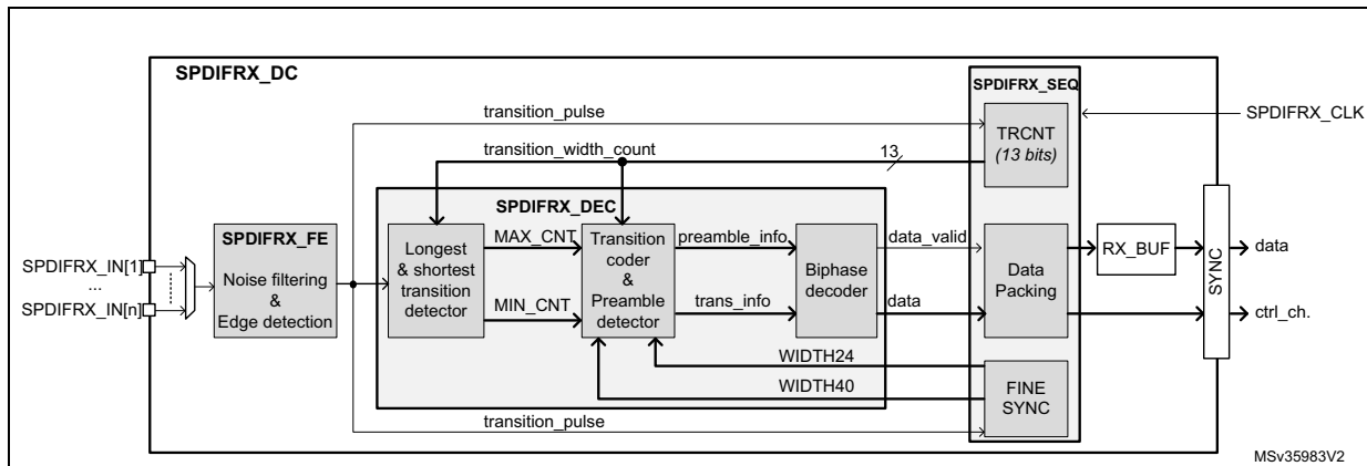
Figure 464. SPDIFRX decoder
