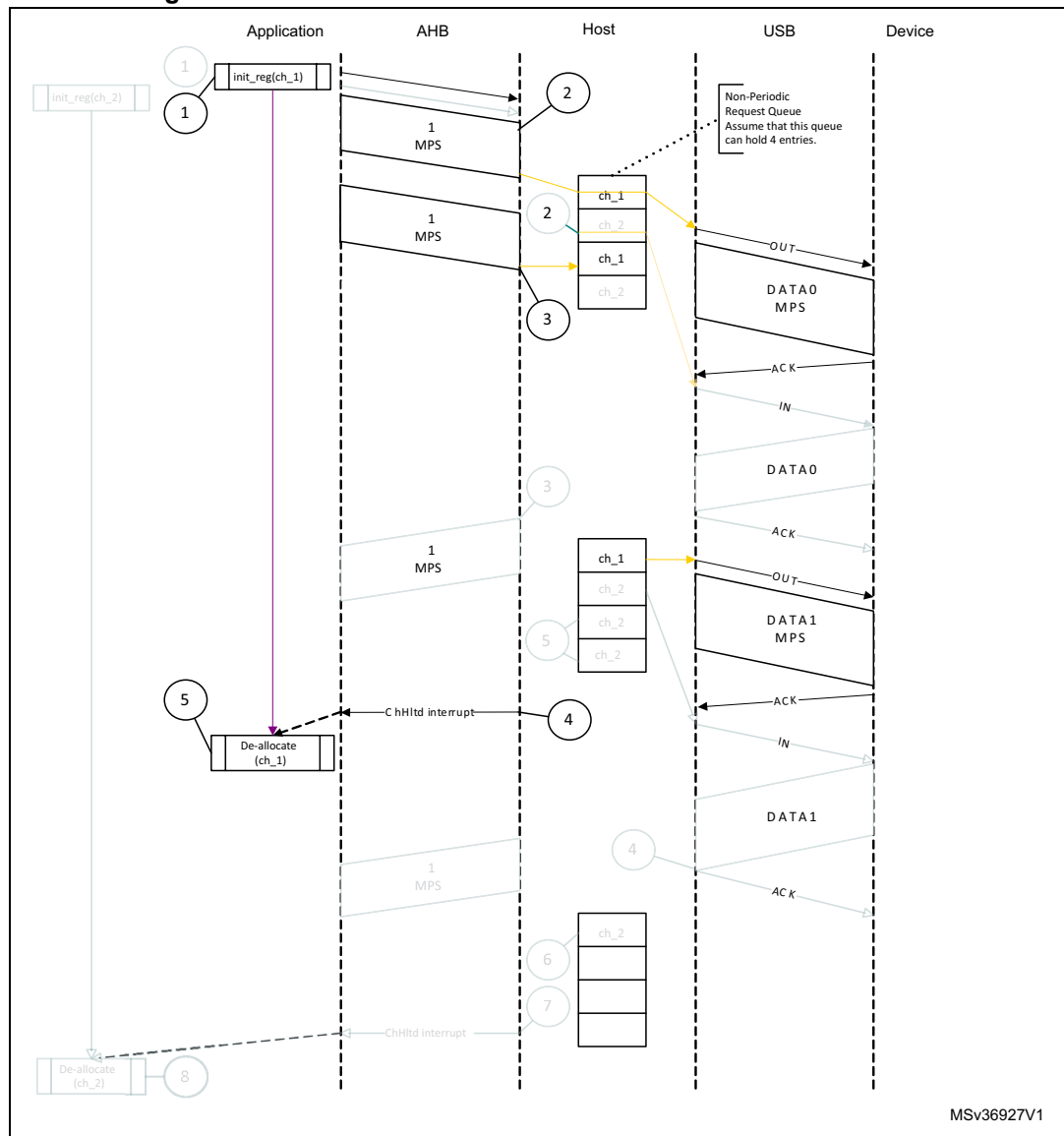
Figure 527. Normal bulk/control OUT/SETUP transactions - DMA
