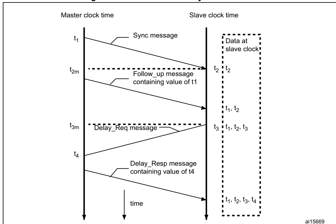
Figure 563. Networked time synchronization
