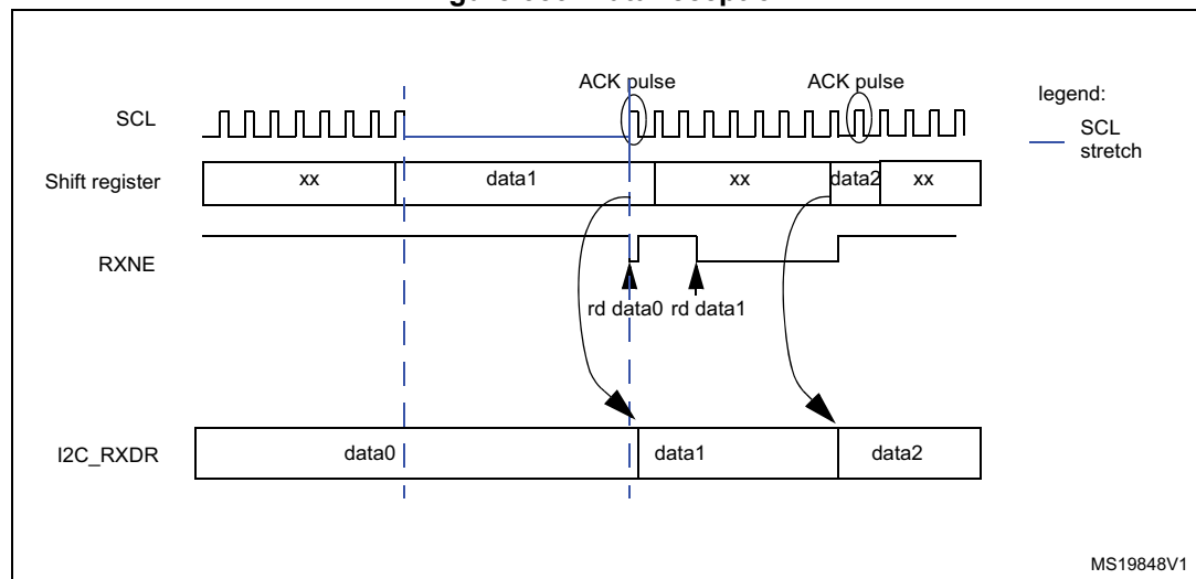
Figure 353. Data reception
