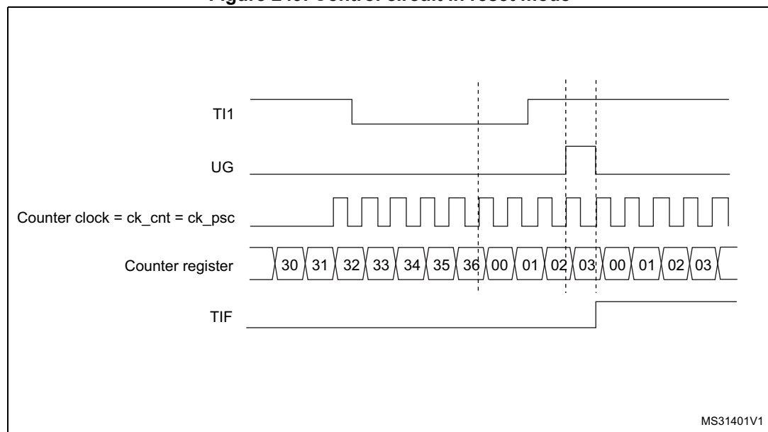
Figure 249. Control circuit in reset mode
