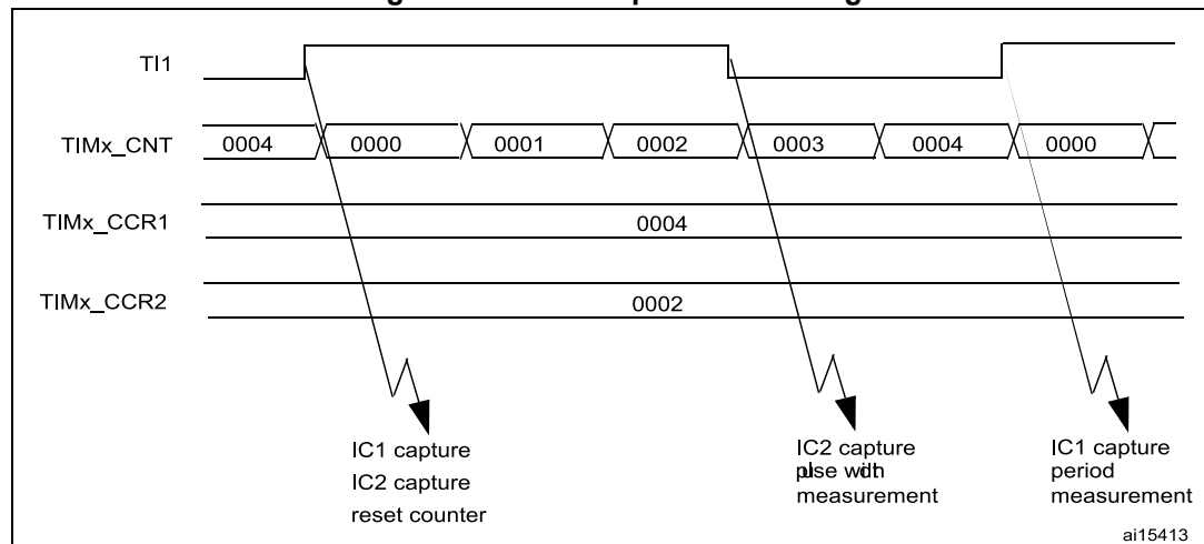
Figure 281. PWM input mode timing
