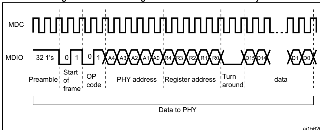
Figure 543. MDIO timing and frame structure - Write cycle
