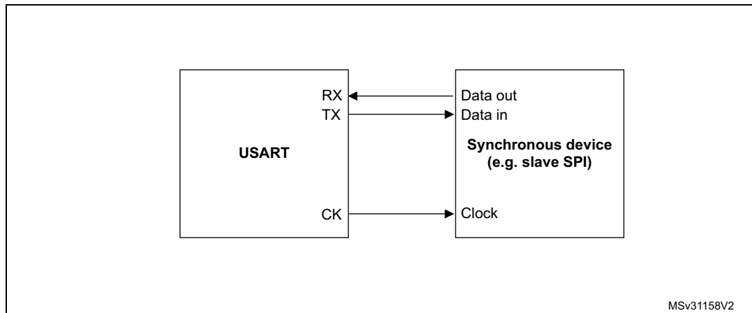
Figure 391. USART example of synchronous transmission
