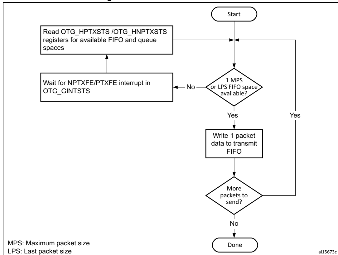
Figure 519. Transmit FIFO write task
