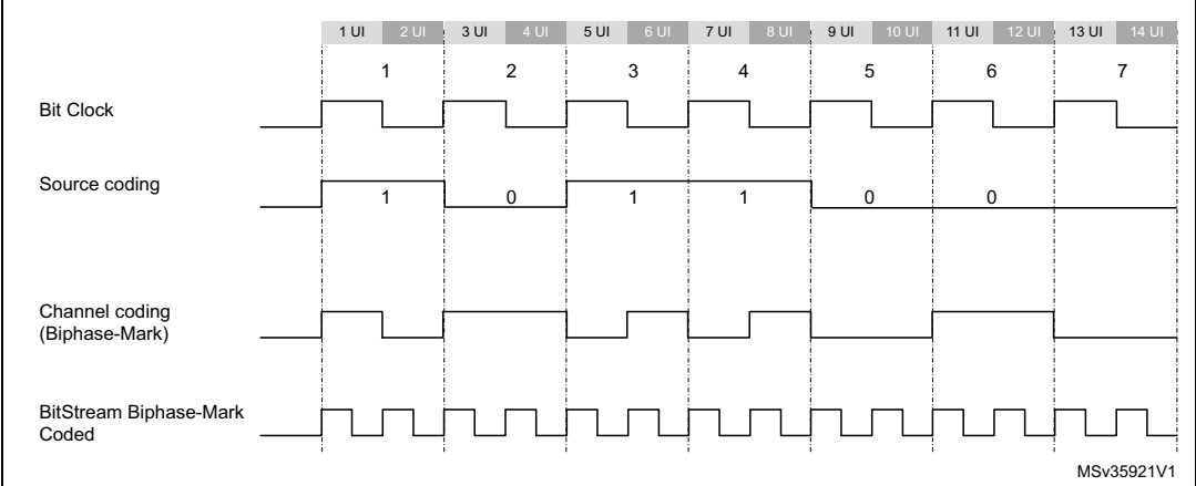
Figure 463. Channel coding example
