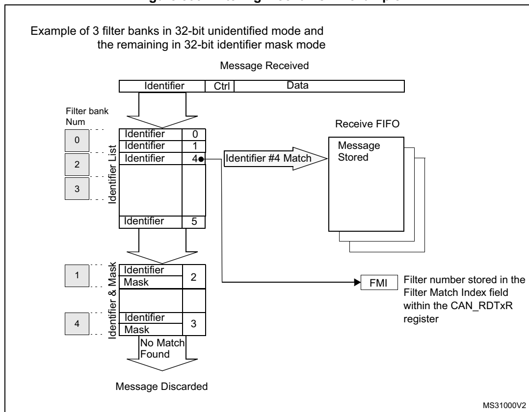
Figure 503. Filtering mechanism - example
