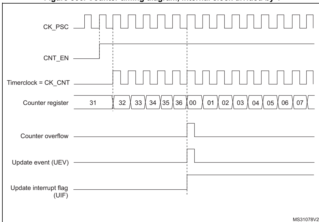
Figure 306. Counter timing diagram, internal clock divided by 1
