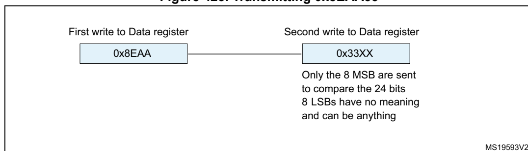
Figure 425. Transmitting 0x8EAA33
