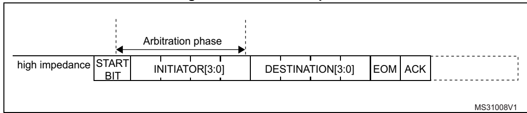
Figure 582. Arbitration phase
