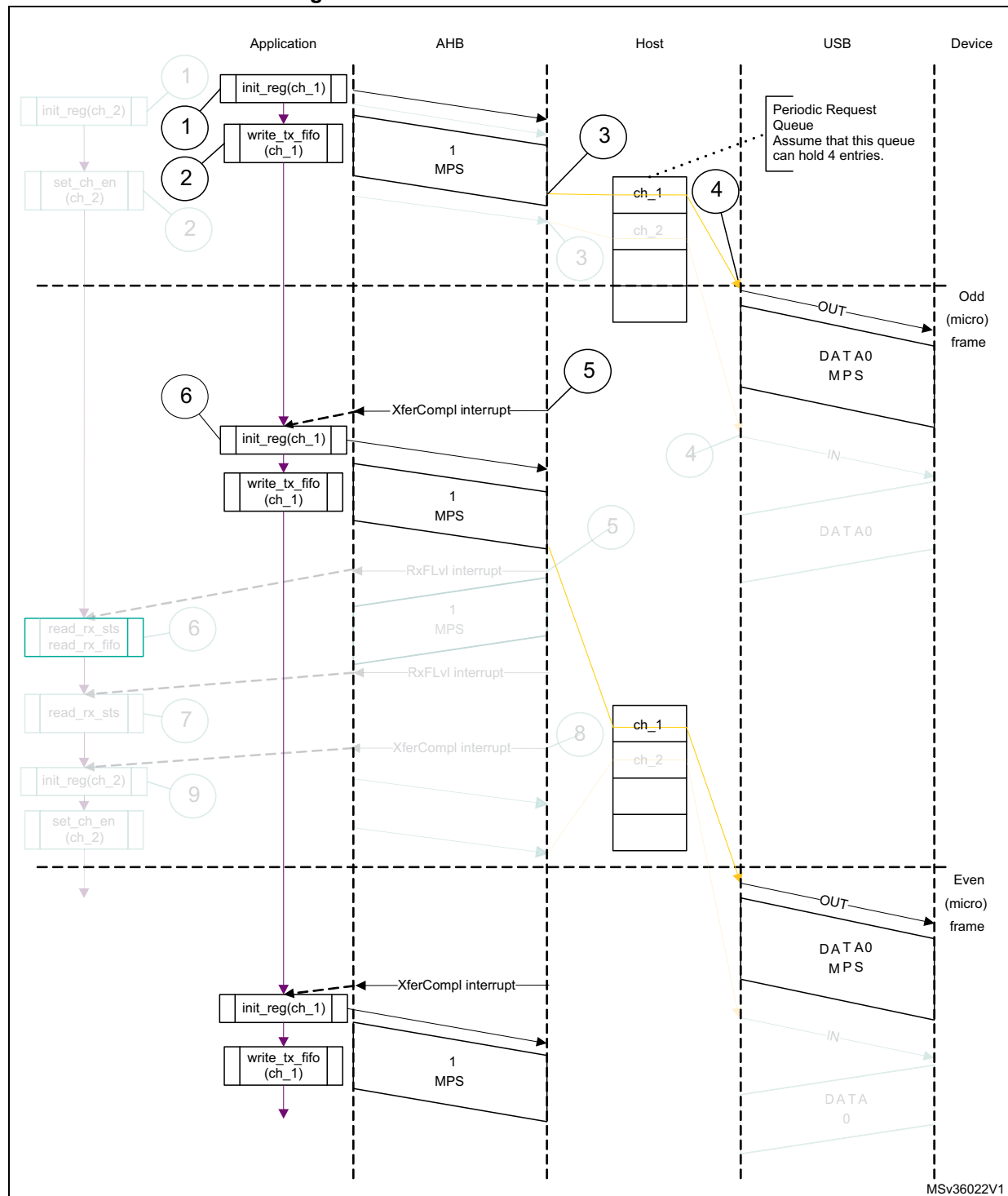
Figure 525. Isochronous OUT transactions
