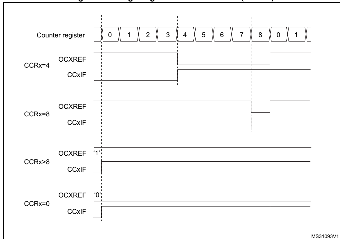
Figure 229. Edge-aligned PWM waveforms (ARR=8)
