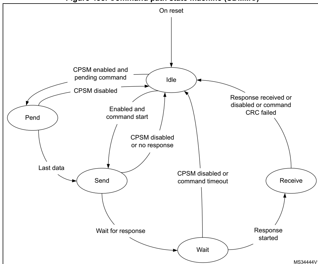
Figure 488. Command path state machine (SDMMC)
