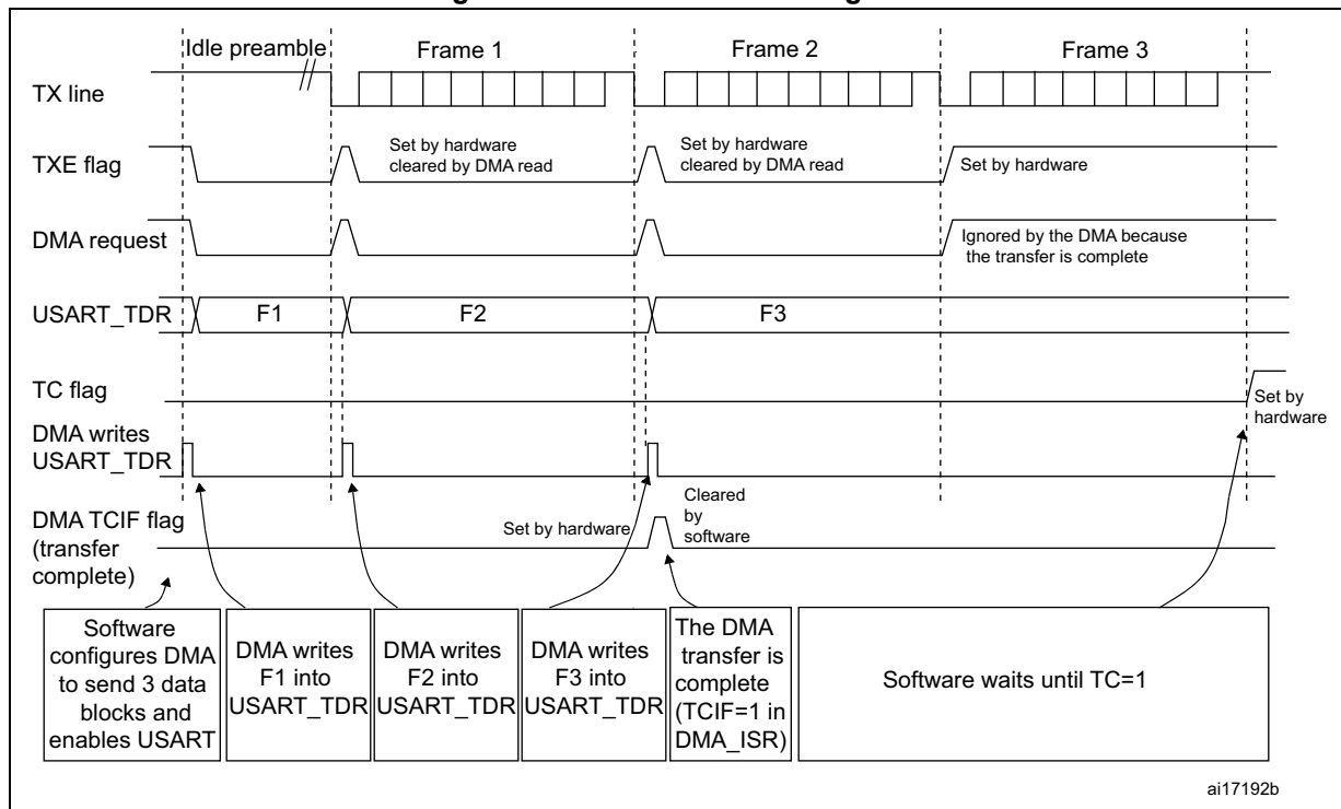
Figure 399. Transmission using DMA
