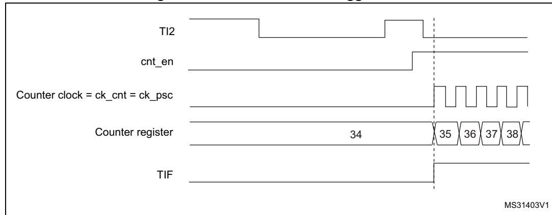
Figure 294. Control circuit in trigger mode
