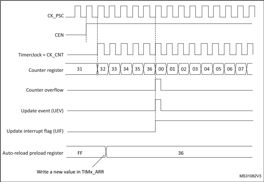
Figure 202. Counter timing diagram, update event when ARPE=0 (TIMx_ARR not preloaded)
