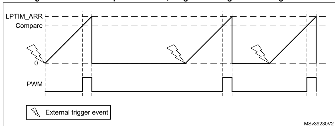
Figure 340. LPTIM output waveform, single counting mode configuration
