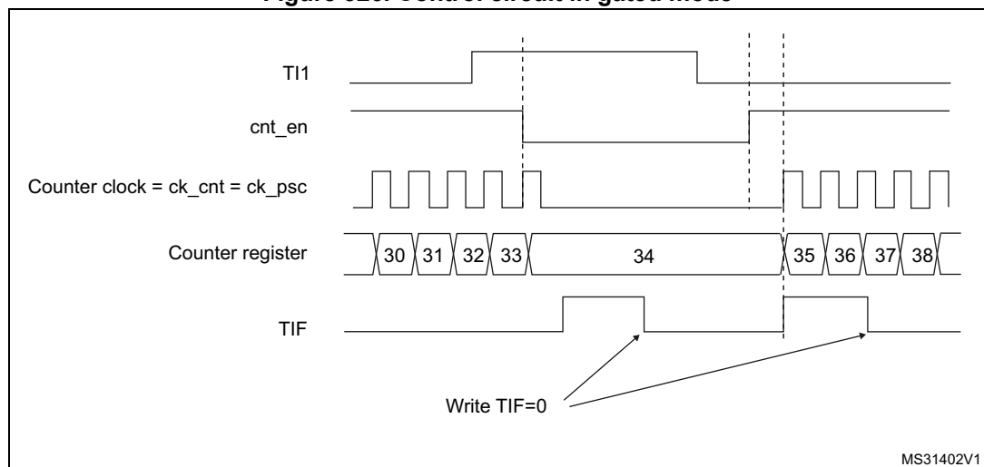
Figure 326. Control circuit in gated mode
