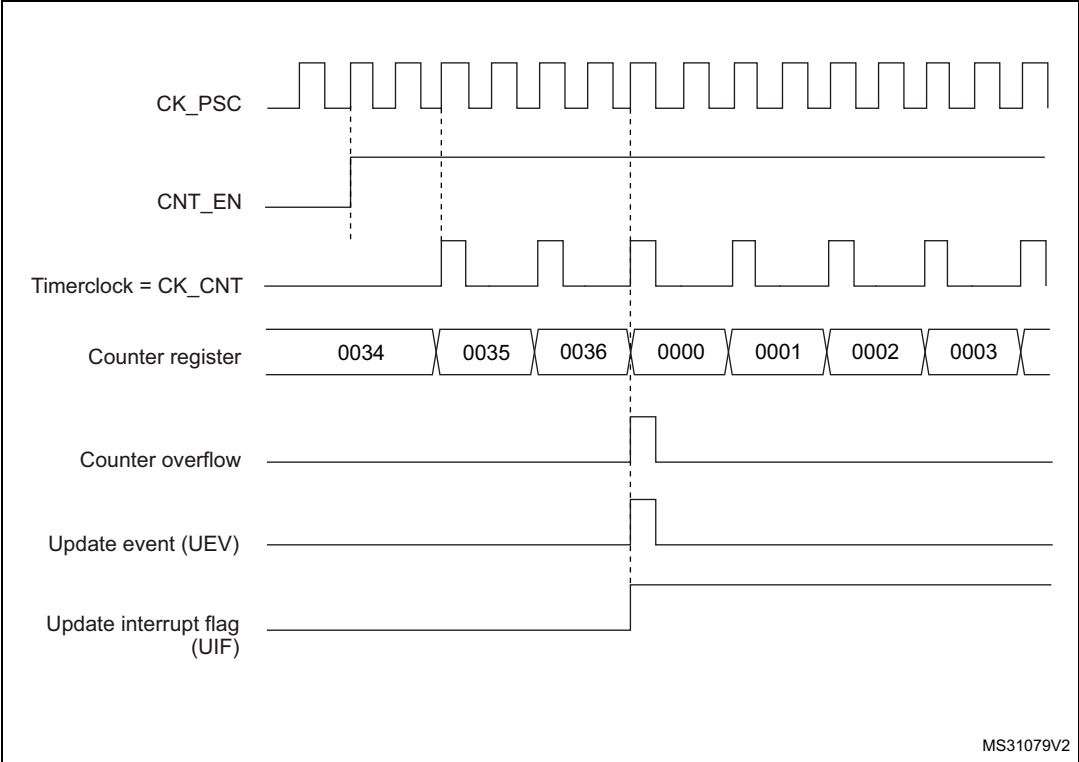
Figure 332. Counter timing diagram, internal clock divided by 2
