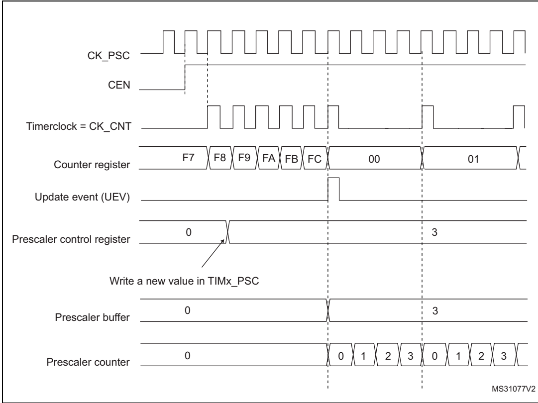
Figure 330. Counter timing diagram with prescaler division change from 1 to 4
