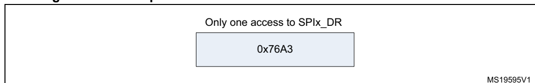
Figure 428. Example of 16-bit data frame extended to 32-bit channel frame
