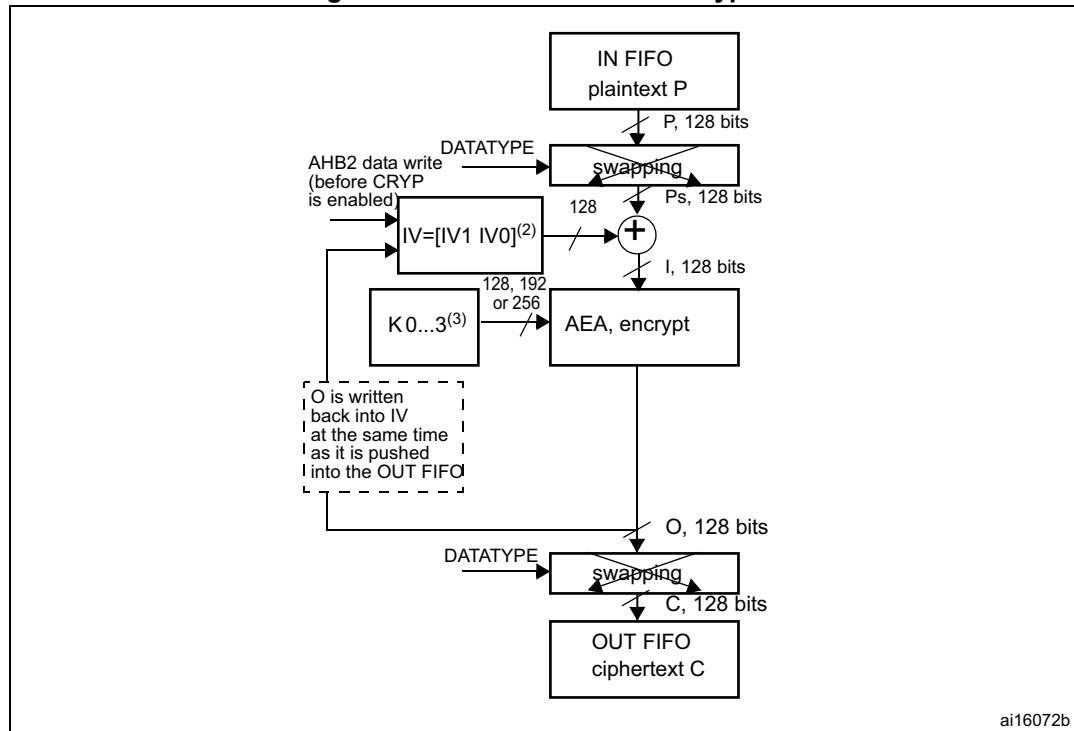
Figure 180. AES-CBC mode encryption
