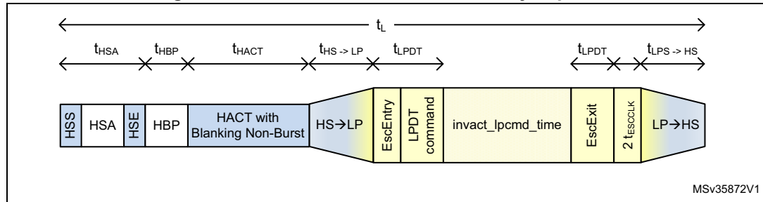
Figure 143. VLPSIZE for non-burst with sync pulses
