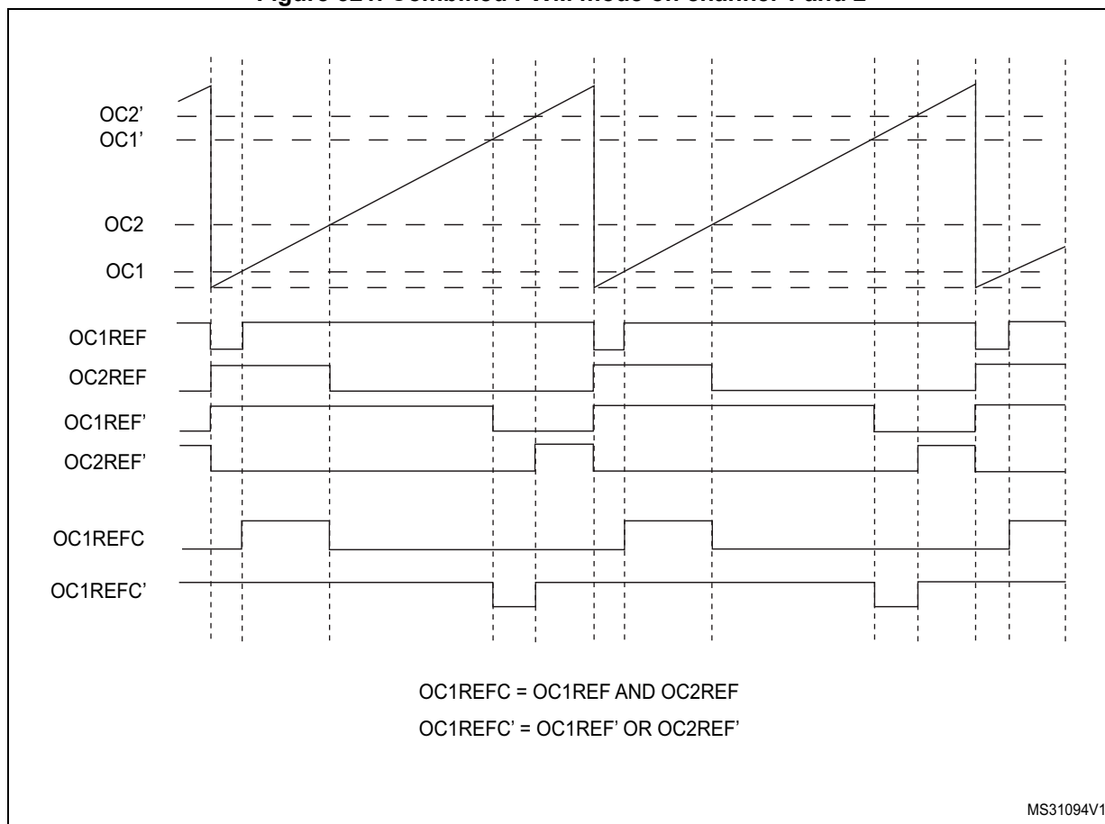
Figure 321. Combined PWM mode on channel 1 and 2
