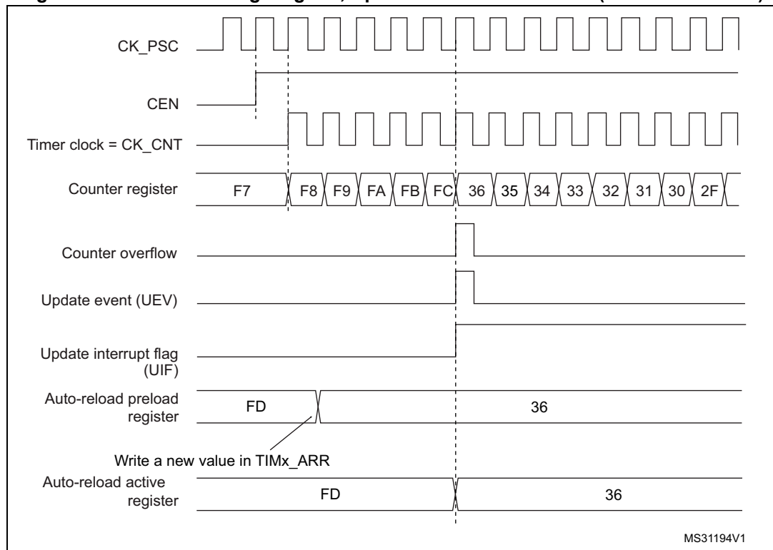
Figure 214. Counter timing diagram, Update event with ARPE=1 (counter overflow)
