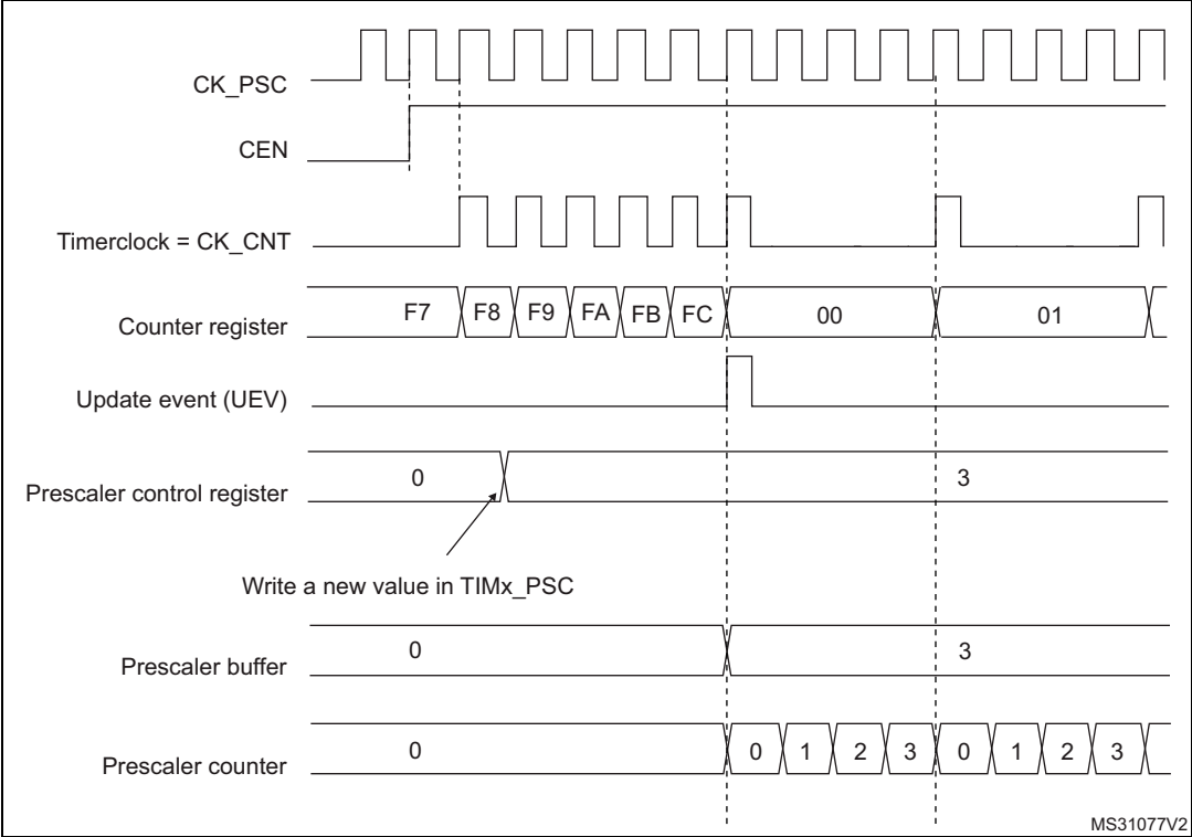
Figure 305. Counter timing diagram with prescaler division change from 1 to 4
