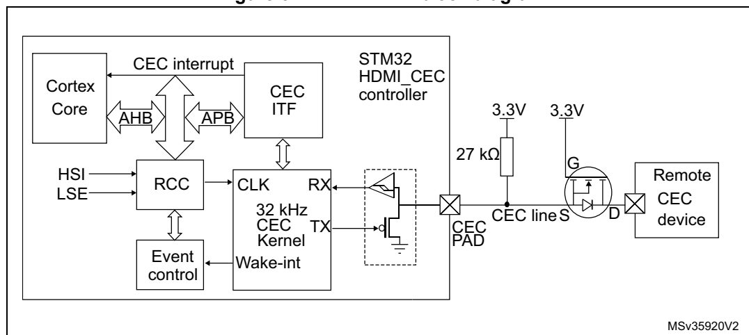
Figure 577. HDMI-CEC block diagram
