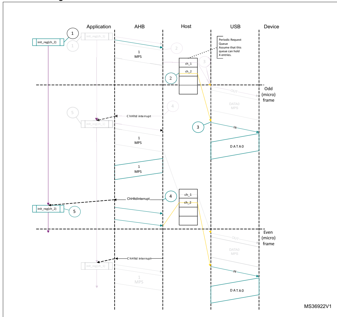
Figure 532. Normal isochronous IN transactions - DMA mode
