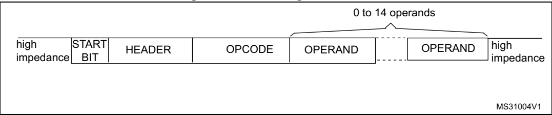
Figure 578. Message structure
