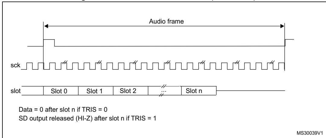
Figure 446. FS role is start of frame (FSDEF = 0)
