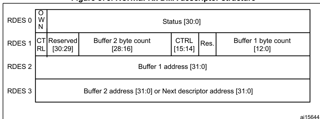
Figure 573. Normal Rx DMA descriptor structure
