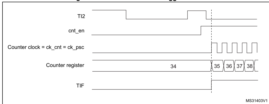
Figure 251. Control circuit in trigger mode
