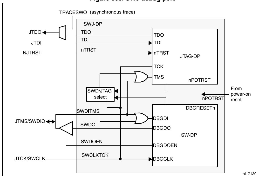
Figure 588. SWJ debug port
