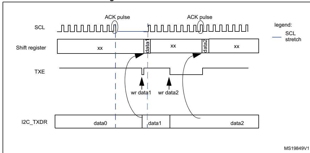
Figure 354. Data transmission
