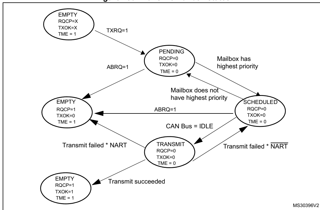
Figure 499. Transmit mailbox states
