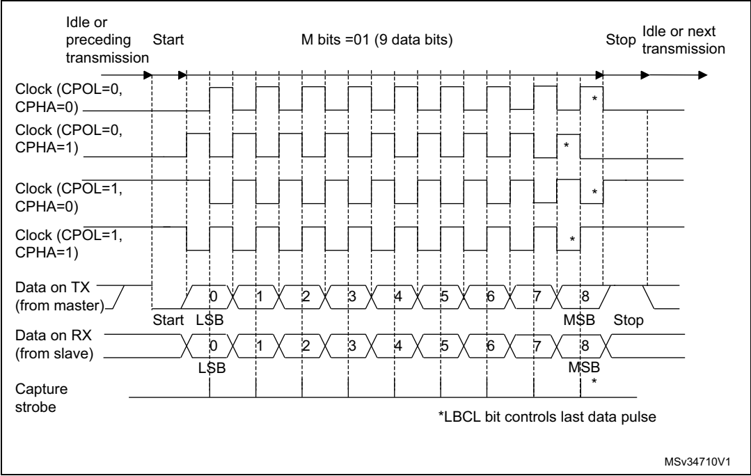
Figure 393. USART data clock timing diagram (M bits = 01)
