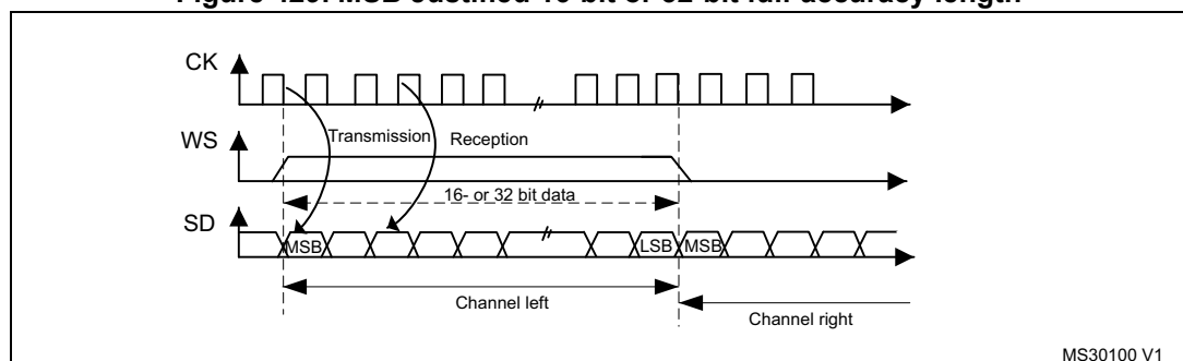
Figure 429. MSB Justified 16-bit or 32-bit full-accuracy length
