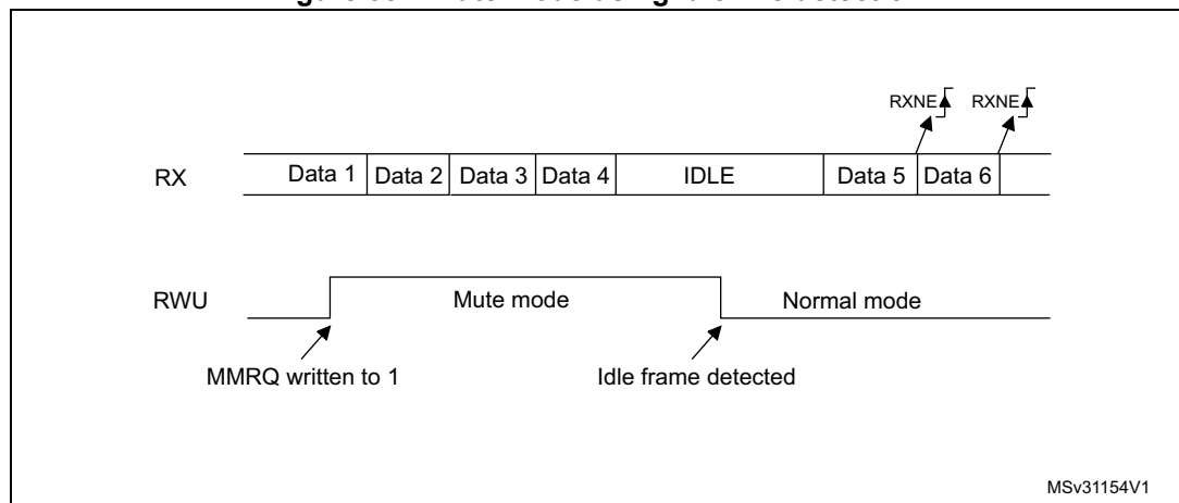
Figure 387. Mute mode using Idle line detection
