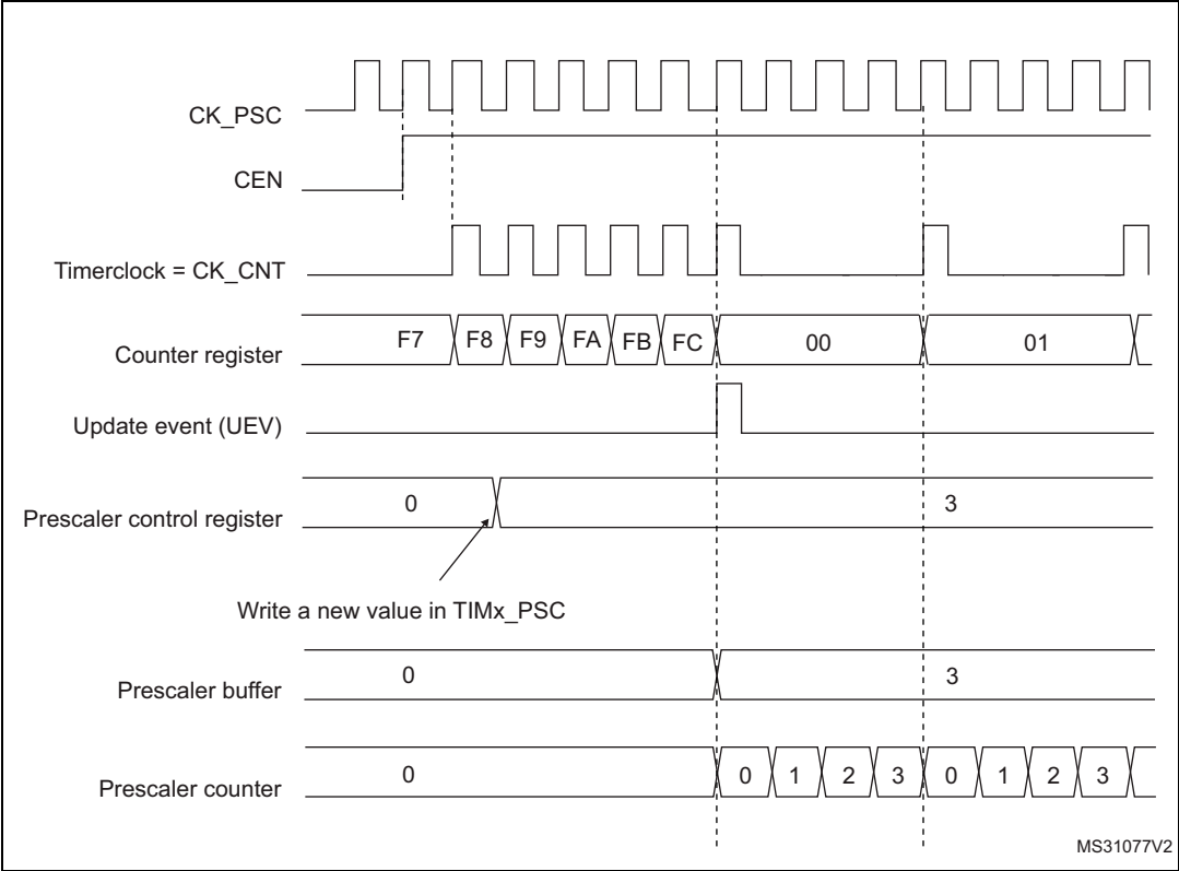
Figure 197. Counter timing diagram with prescaler division change from 1 to 4
