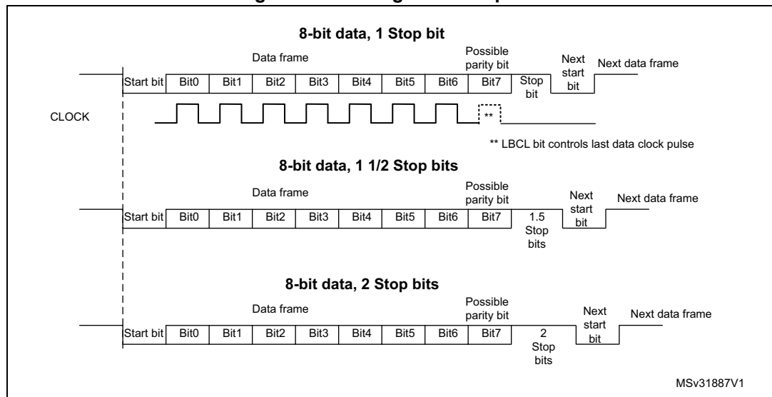
Figure 382. Configurable stop bits
