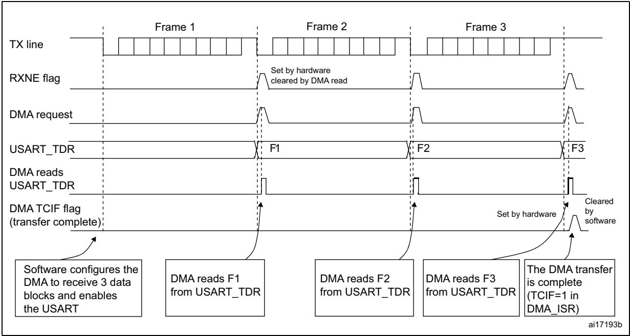
Figure 400. Reception using DMA
