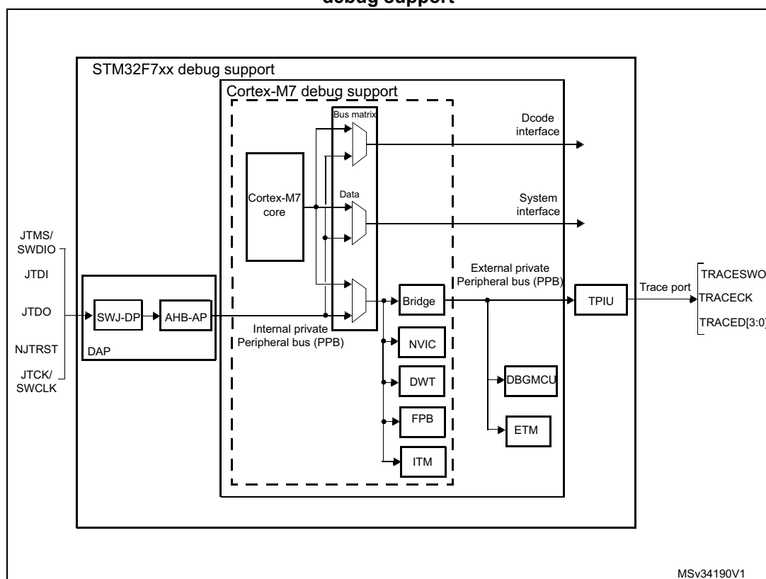
Figure 587. Block diagram of STM32 MCU and Cortex®-M7 with FPU -level debug support
