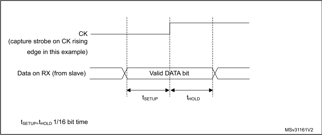
Figure 394. RX data setup/hold time
