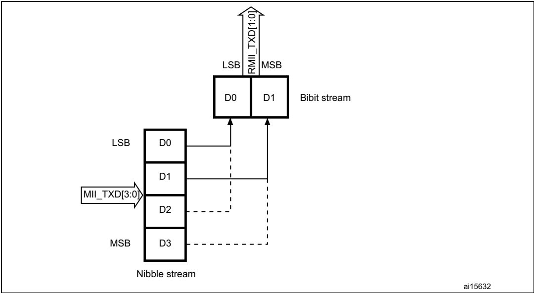
Figure 553. Transmission bit order
