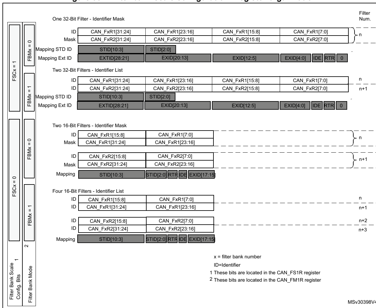
Figure 501. Filter bank scale configuration - register organization
