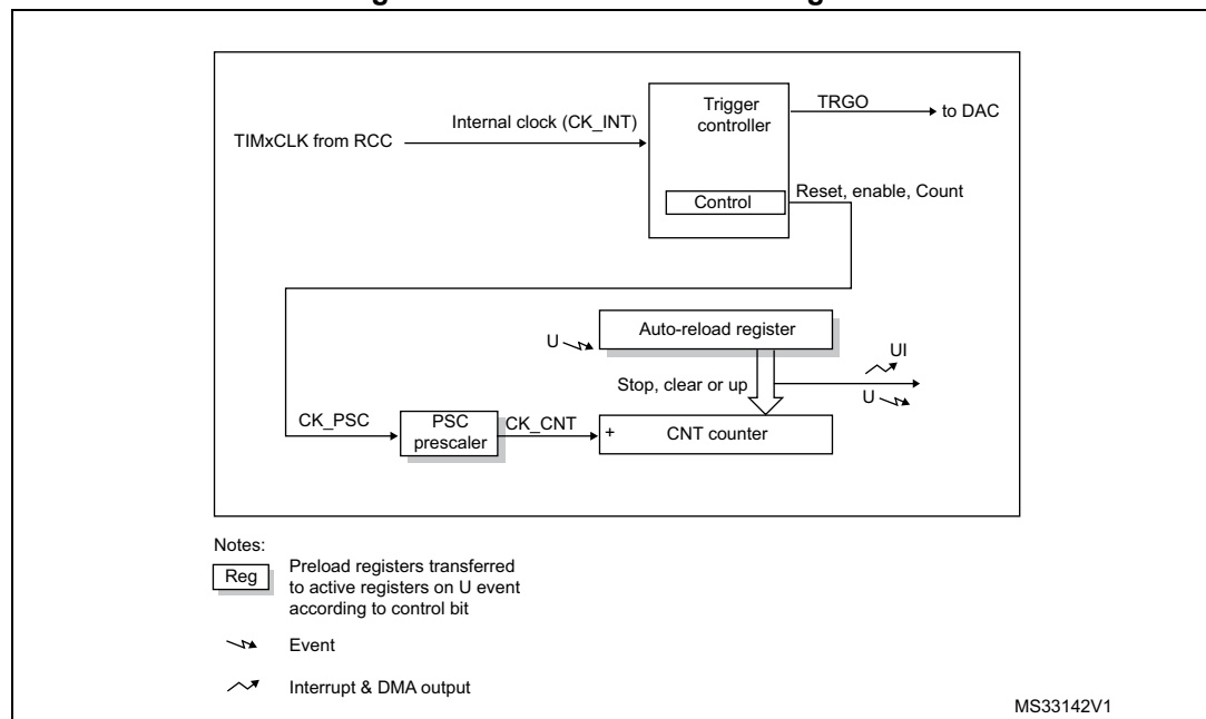
Figure 328. Basic timer block diagram
