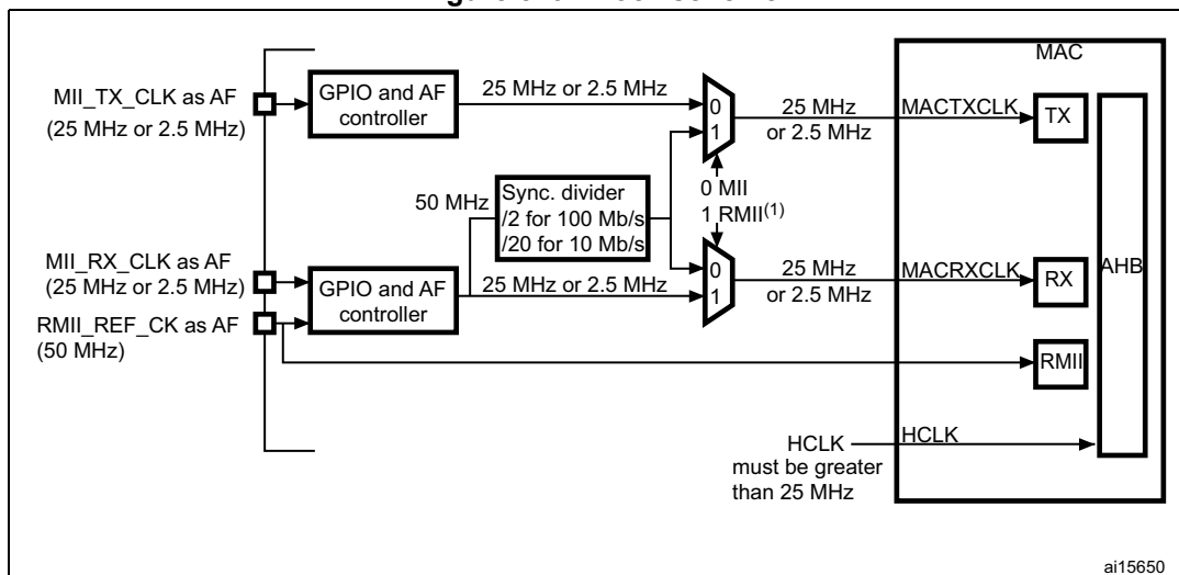
Figure 549. Clock scheme
