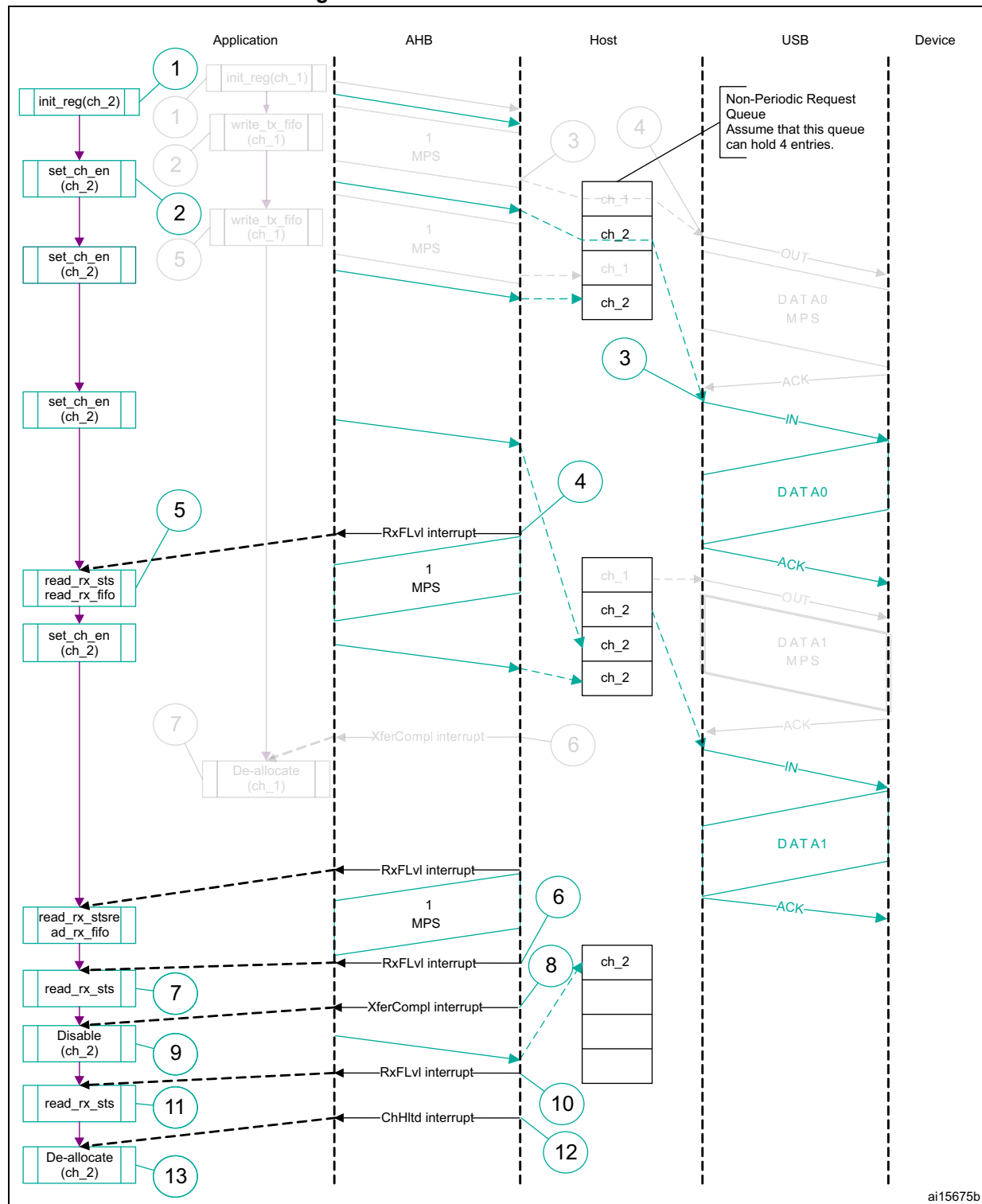
Figure 522. Bulk/control IN transactions
