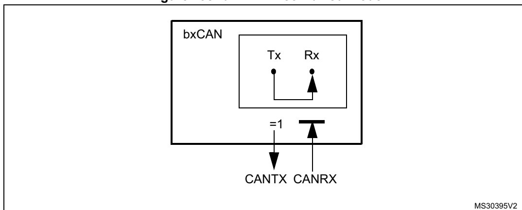
Figure 498. bxCAN in combined mode
