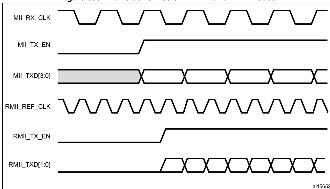
Figure 556. Frame transmission in MII and RMII modes
