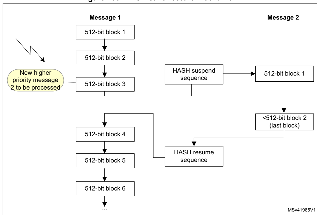
Figure 193. HASH save/restore mechanism
