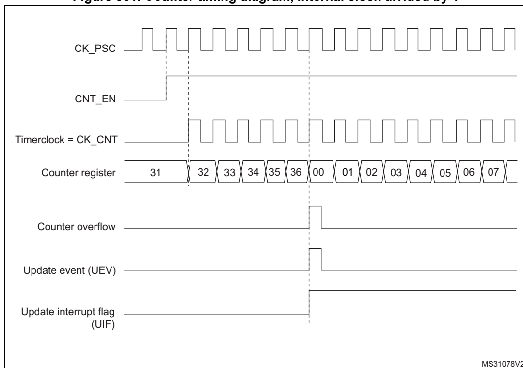
Figure 331. Counter timing diagram, internal clock divided by 1
