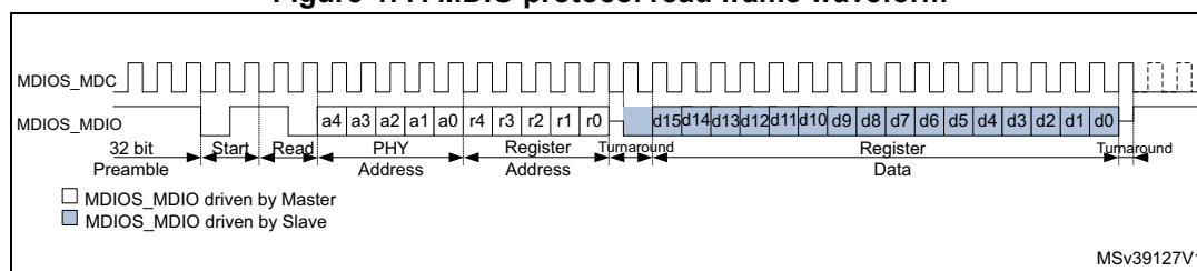
Figure 477. MDIO protocol read frame waveform
