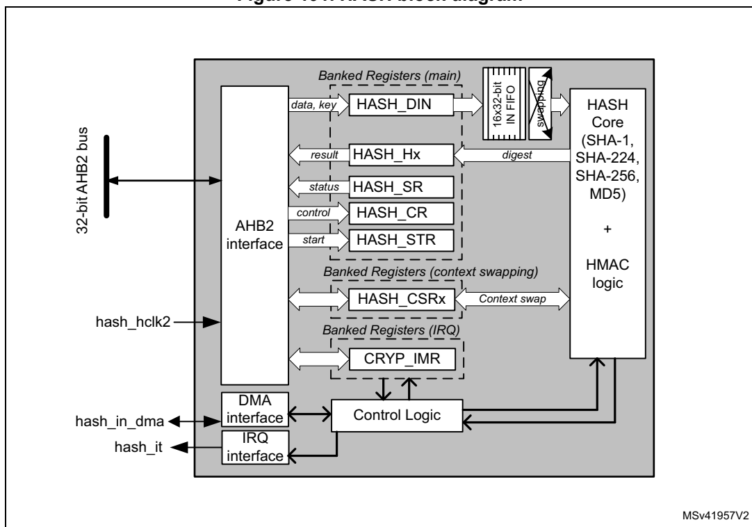
Figure 191. HASH block diagram
