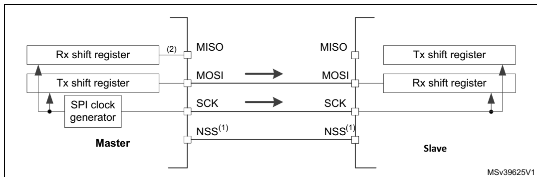
Figure 408. Simplex single master/single slave application (master in transmit-only/ slave in receive-only mode)
