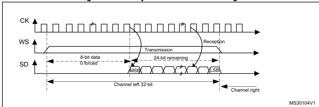
Figure 433. LSB justified 24-bit frame length
