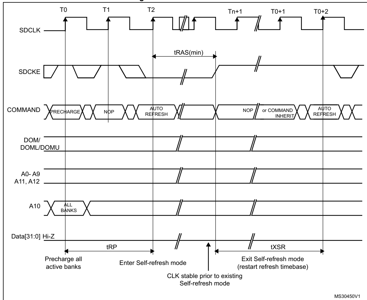
Figure 60. Self-refresh mode
