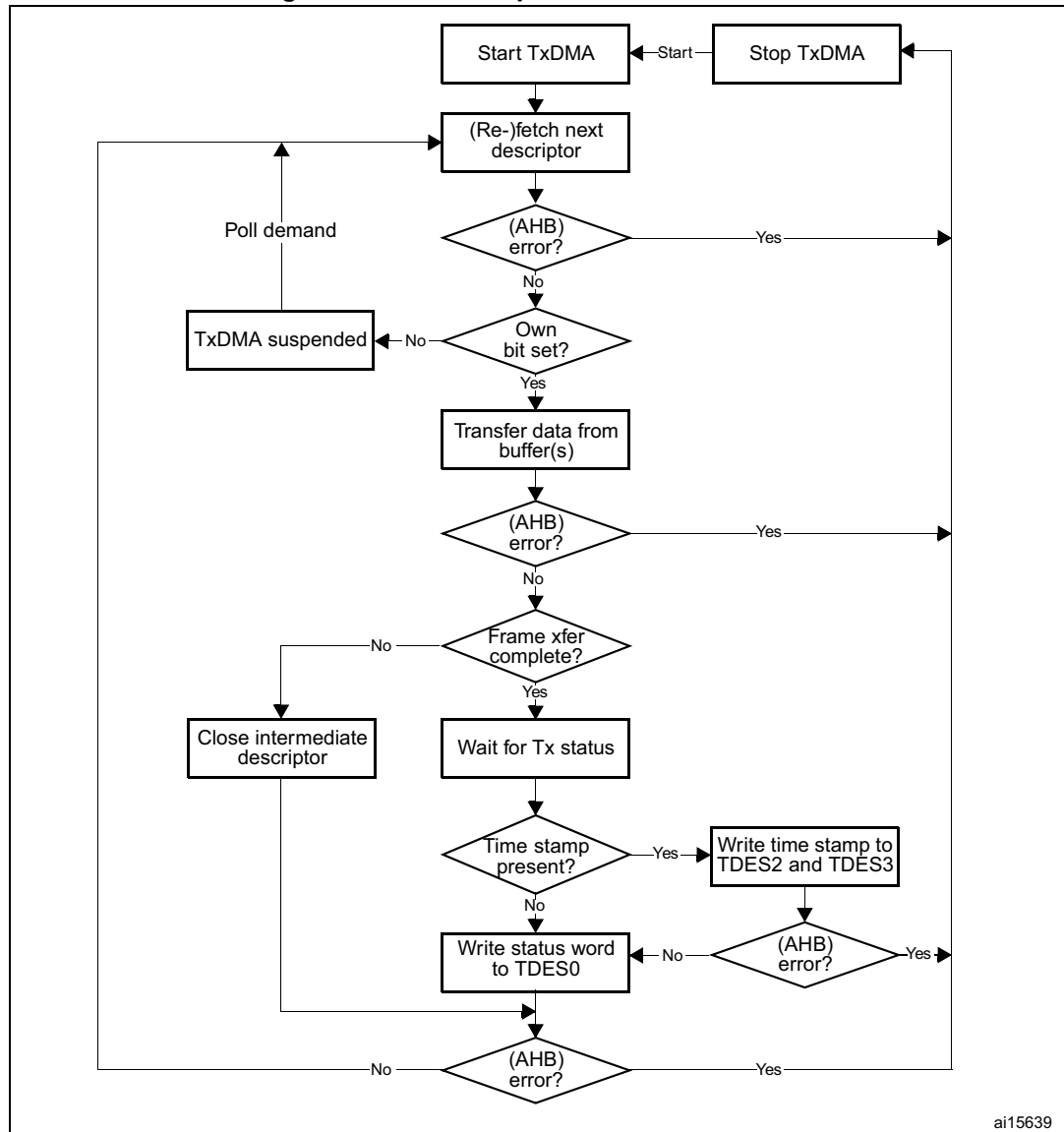
Figure 568. TxDMA operation in default mode
