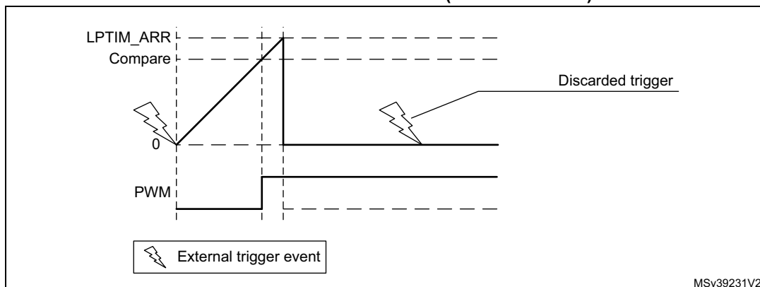
Figure 341. LPTIM output waveform, Single counting mode configuration and Set-once mode activated (WAVE bit is set)
