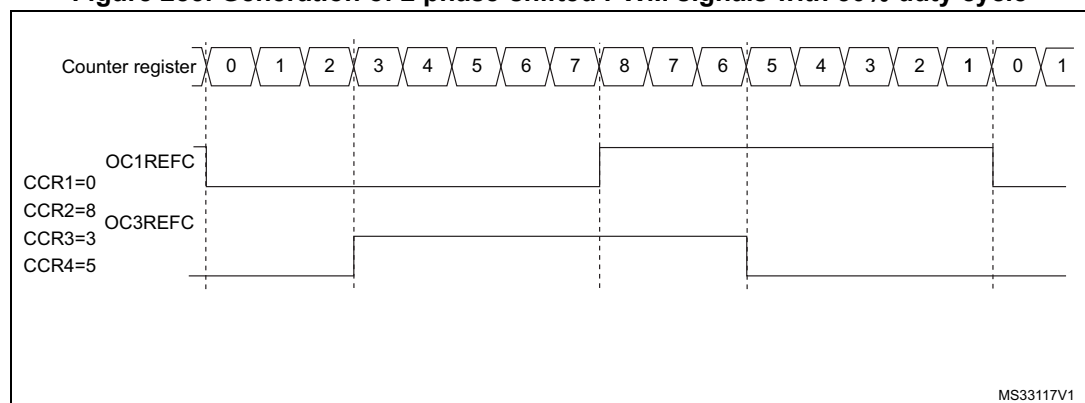
Figure 285. Generation of 2 phase-shifted PWM signals with 50% duty cycle
