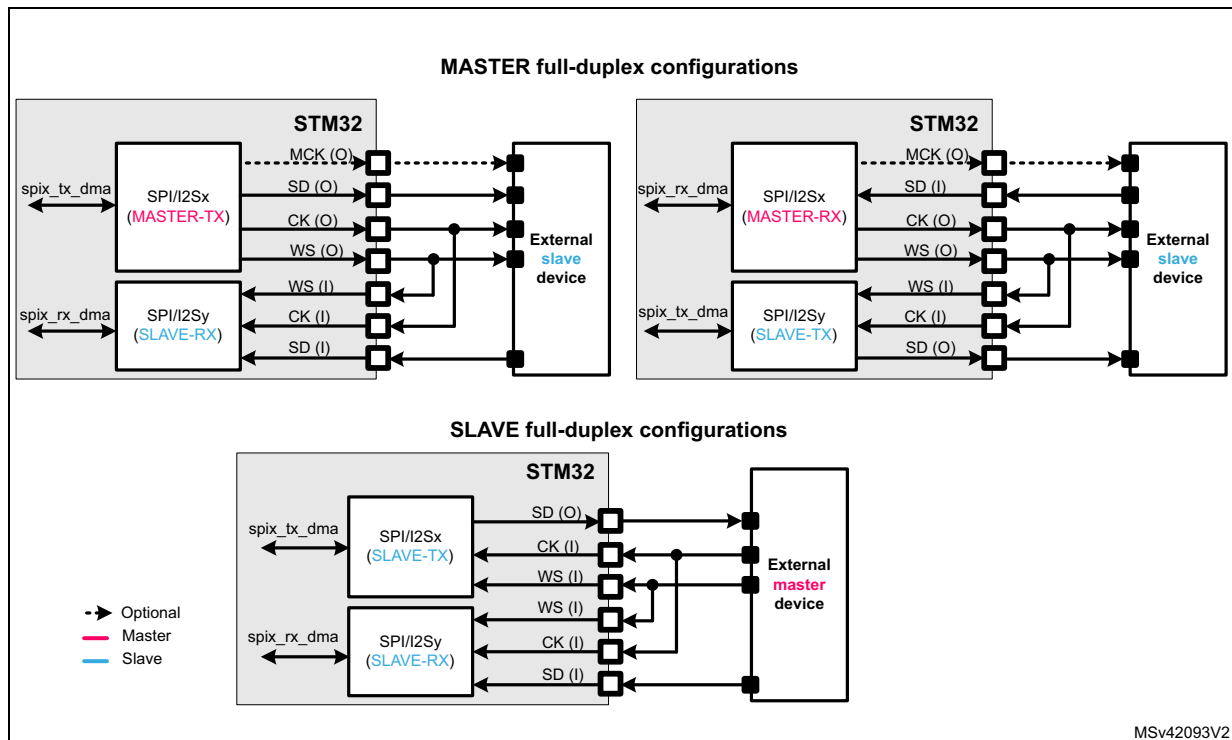
Figure 422. Full-duplex communication
