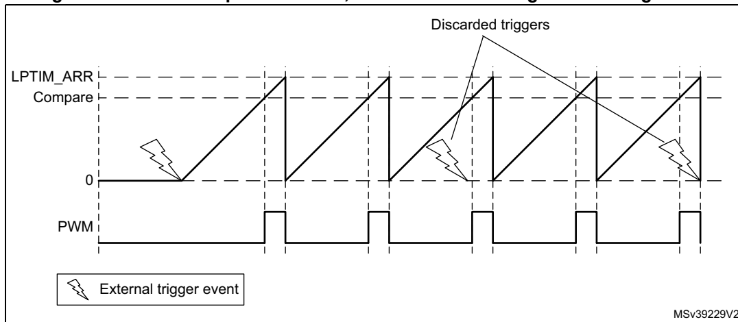
Figure 342. LPTIM output waveform, Continuous counting mode configuration
