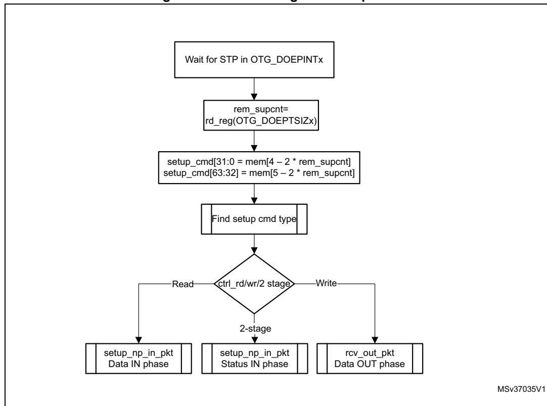
Figure 534. Processing a SETUP packet
