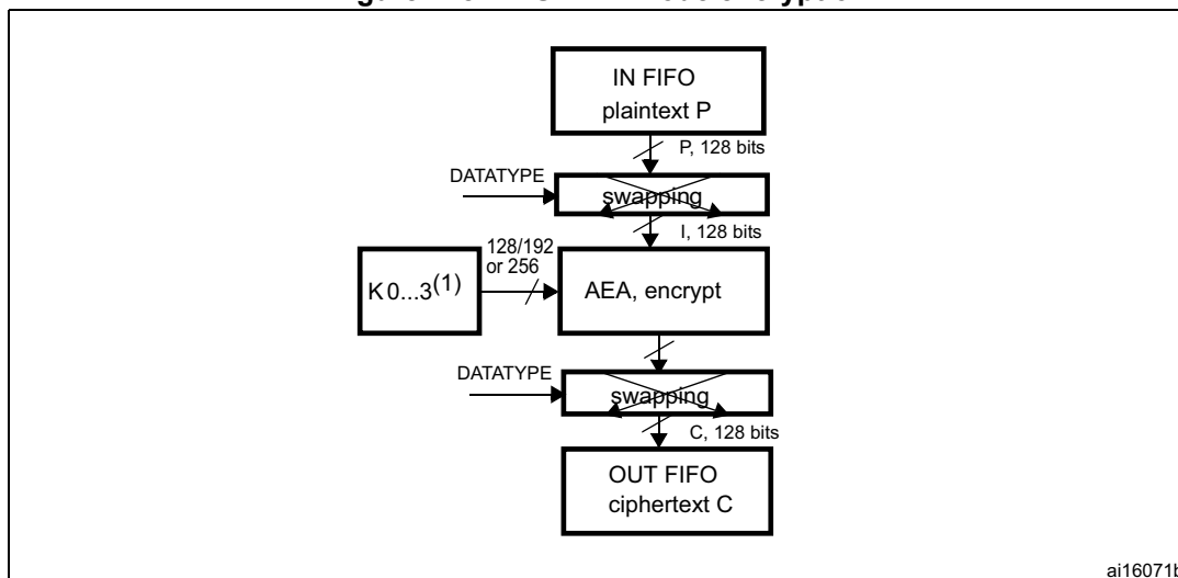
Figure 178. AES-ECB mode encryption
