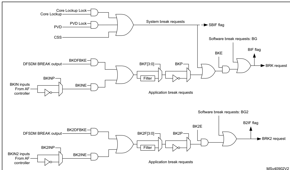
Figure 237. Break and Break2 circuitry overview
