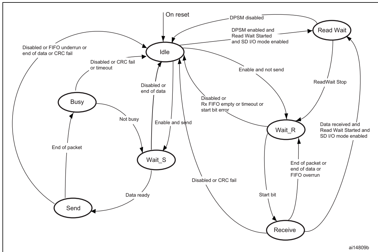
Figure 491. Data path state machine (DPSM)
