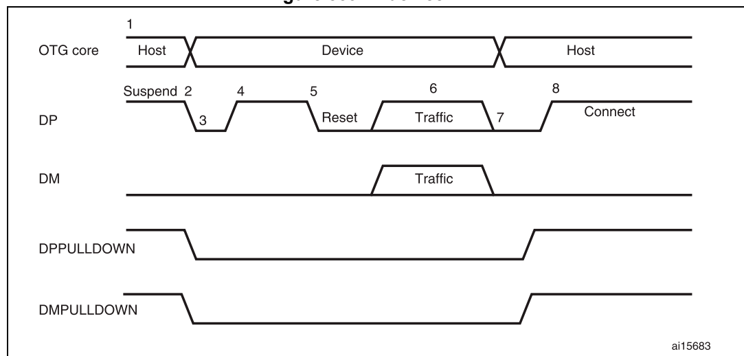
Figure 539. A-device HNP
