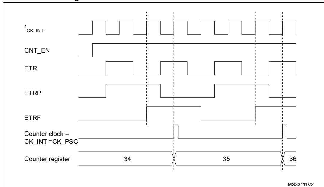
Figure 277. Control circuit in external clock mode 2
