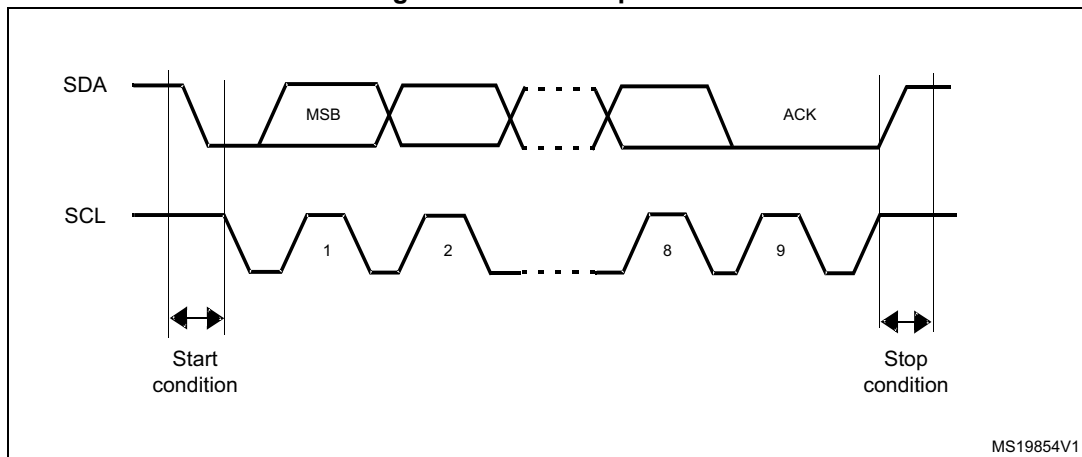
Figure 350. I 2 C bus protocol
