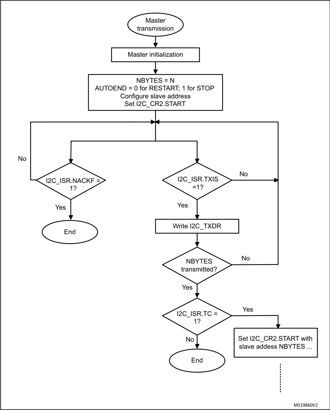
Figure 366. Transfer sequence flowchart for I2C master transmitter for N≤255 bytes
