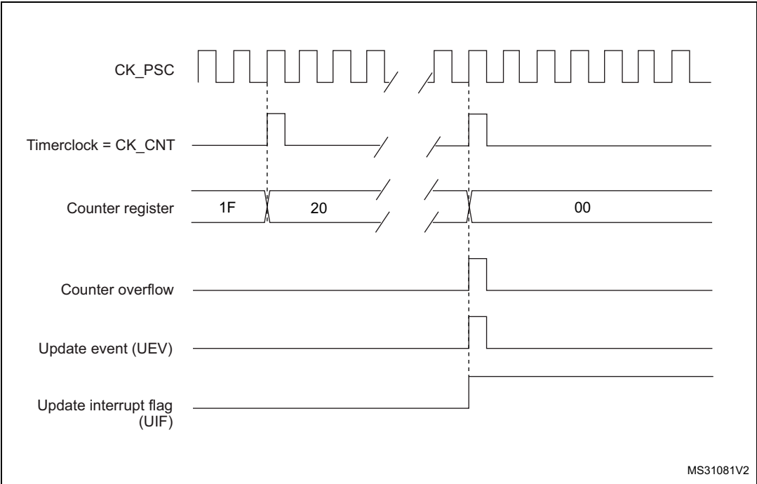
Figure 334. Counter timing diagram, internal clock divided by N
