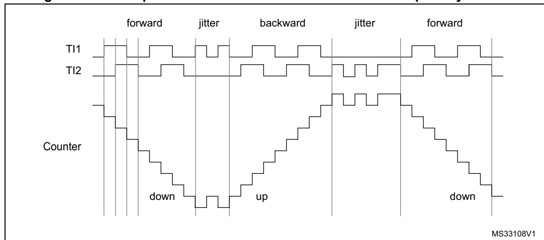
Figure 291. Example of encoder interface mode with TI1FP1 polarity inverted
