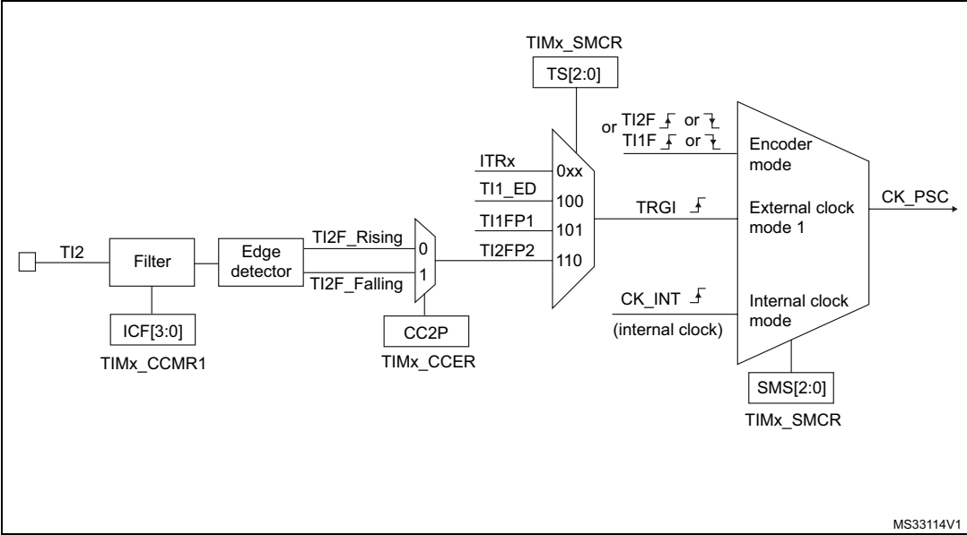
Figure 313. TI2 external clock connection example
