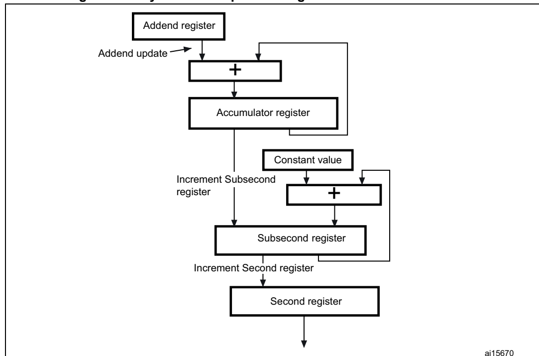
Figure 564. System time update using the Fine correction method
