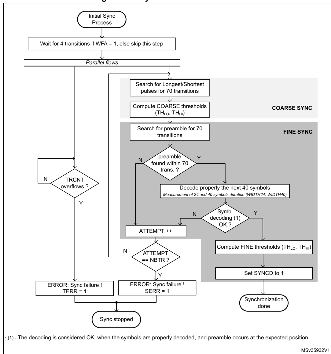
Figure 467. Synchronization flowchart
