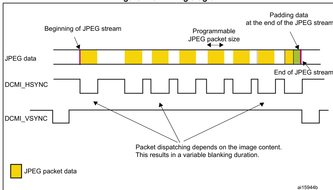
Figure 113. Timing diagram
