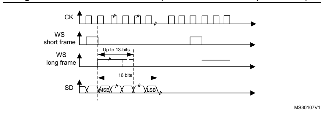
Figure 439. PCM standard waveforms (16-bit extended to 32-bit packet frame)
