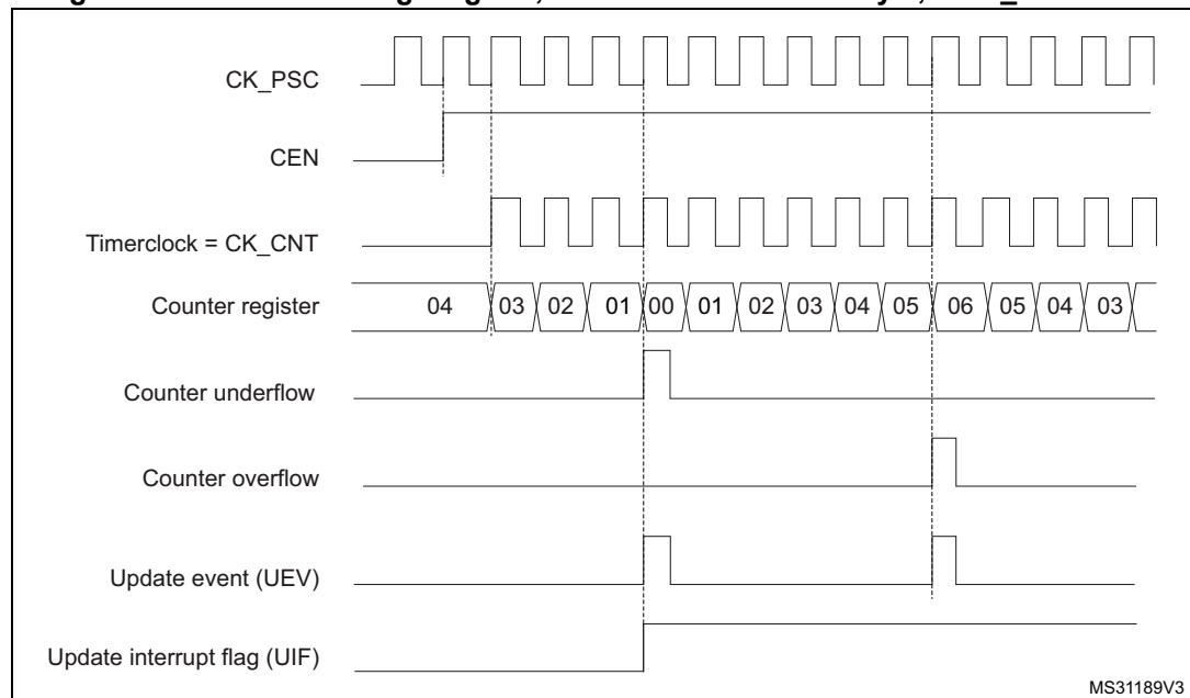
Figure 209. Counter timing diagram, internal clock divided by 1, TIMx_ARR = 0x6
