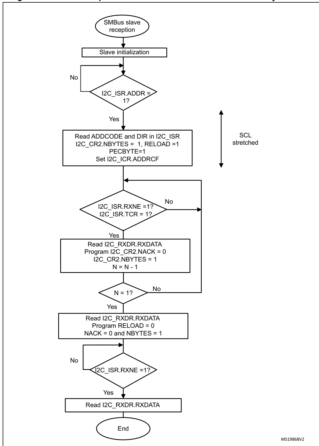
Figure 375. Transfer sequence flowchart for SMBus slave receiver N Bytes + PEC
