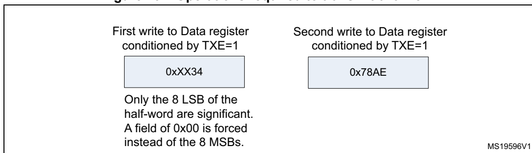
Figure 434. Operations required to transmit 0x3478AE
