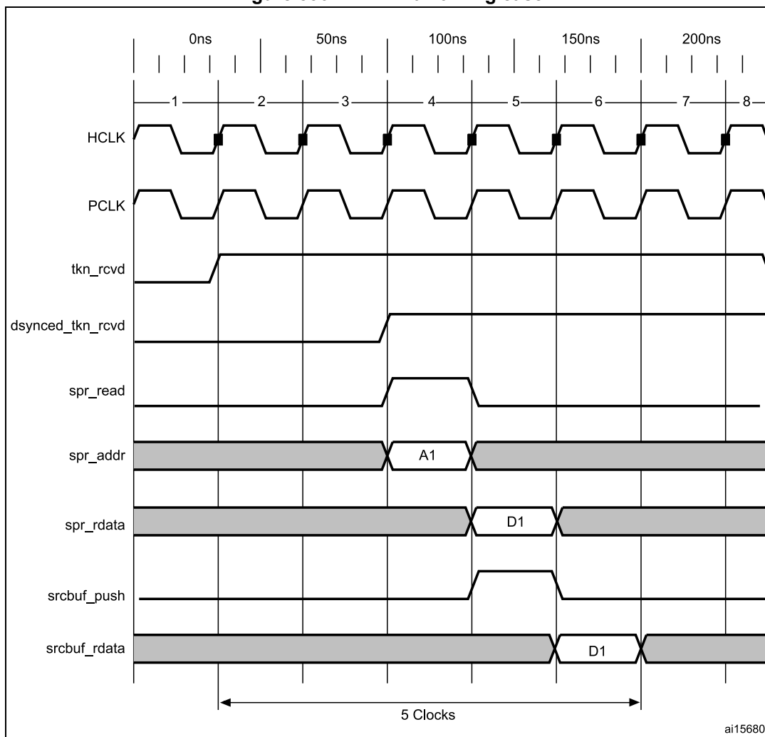
Figure 536. TRDT max timing case
