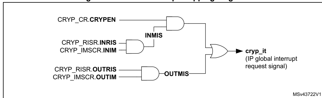
Figure 190. CRYP interrupt mapping diagram
