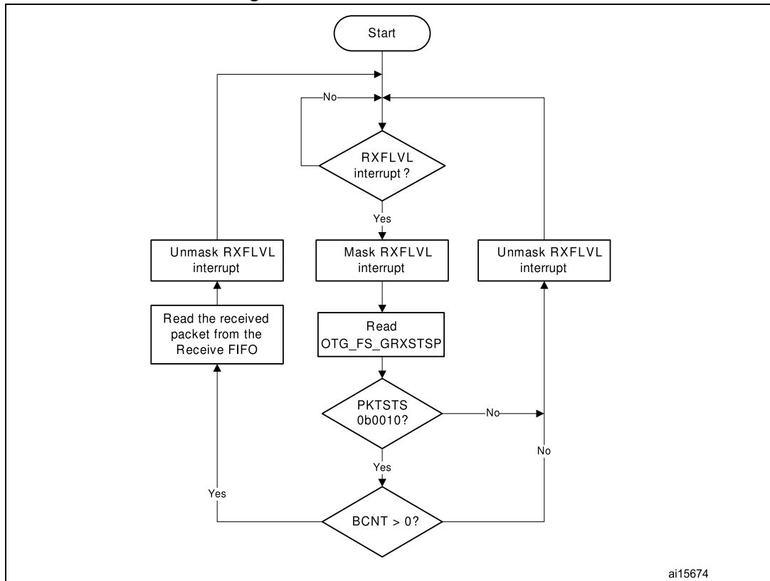
Figure 520. Receive FIFO read task
