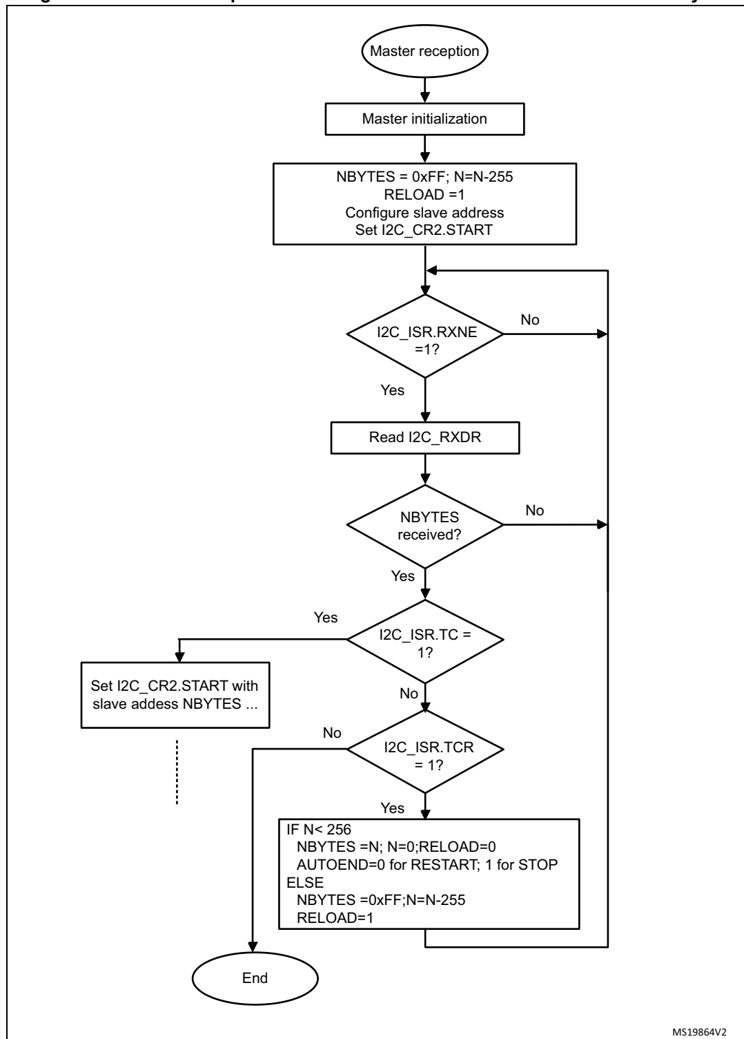
Figure 370. Transfer sequence flowchart for I2C master receiver for N &gt; 255 bytes
