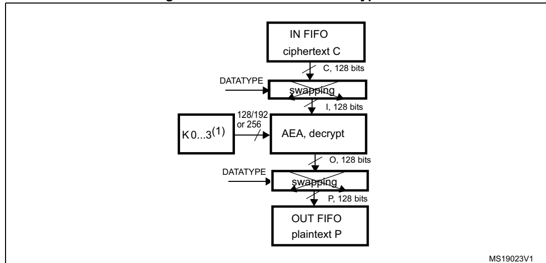
Figure 179. AES-ECB mode decryption
