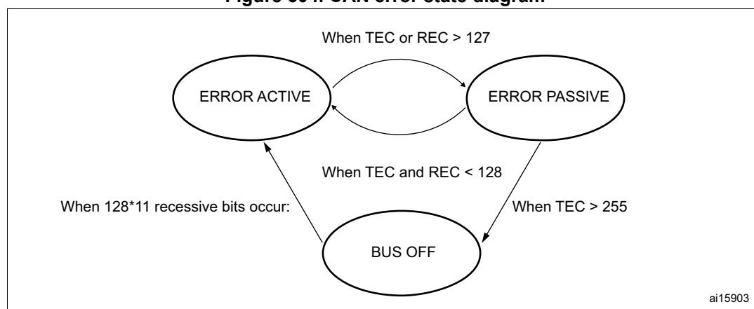
Figure 504. CAN error state diagram
