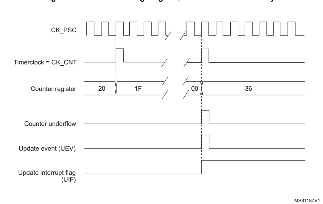
Figure 265. Counter timing diagram, internal clock divided by N
