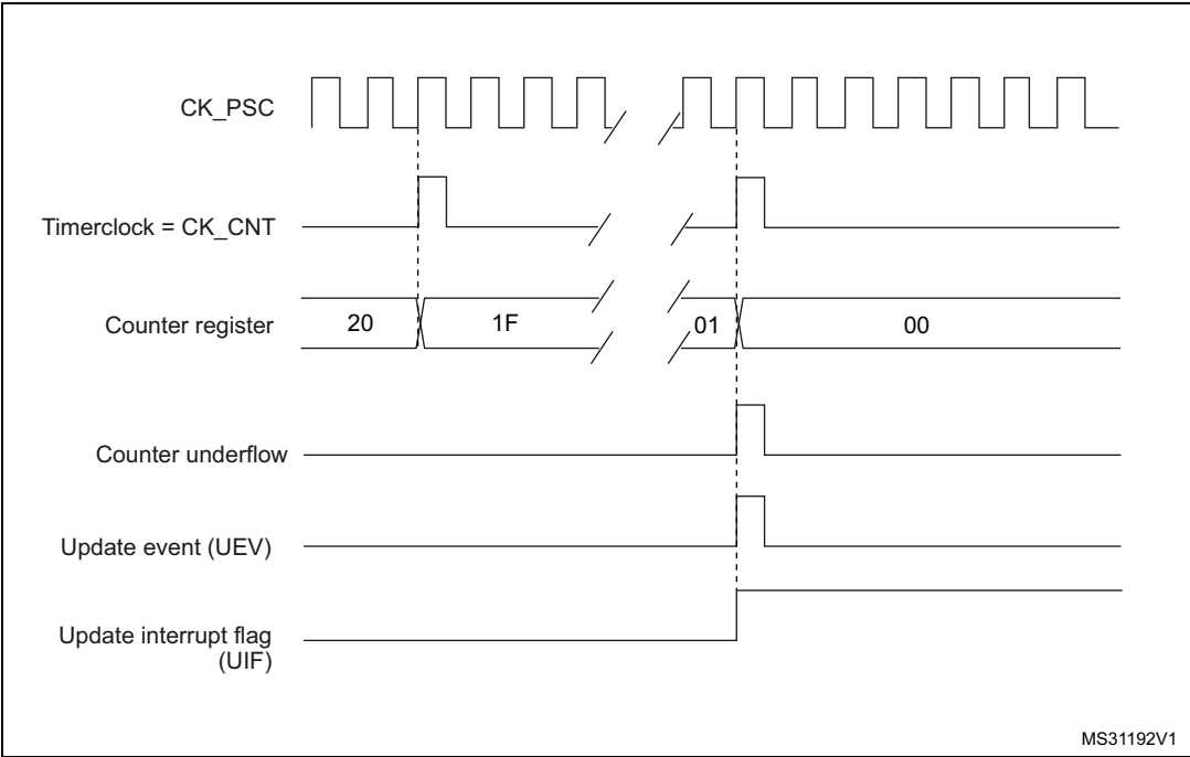
Figure 212. Counter timing diagram, internal clock divided by N
