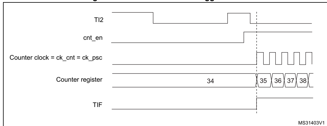
Figure 327. Control circuit in trigger mode
