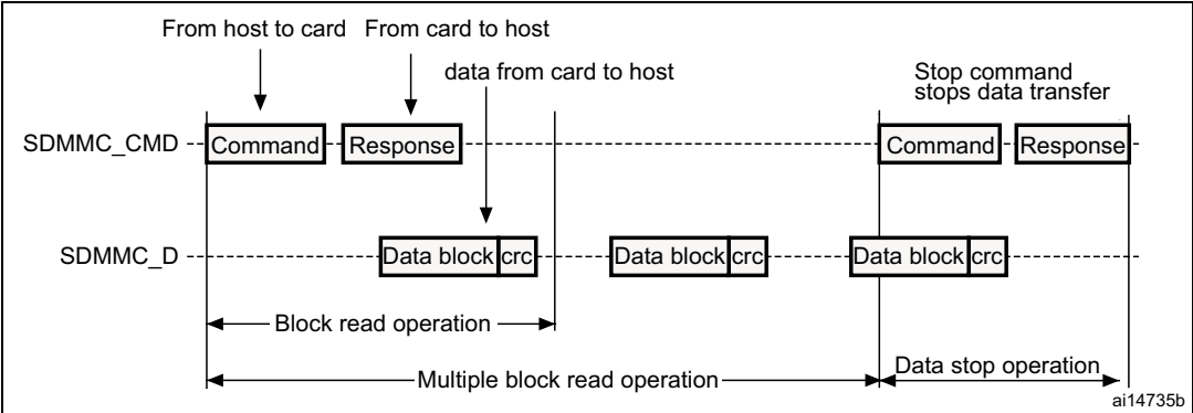
Figure 479. (Multiple) block read operation
