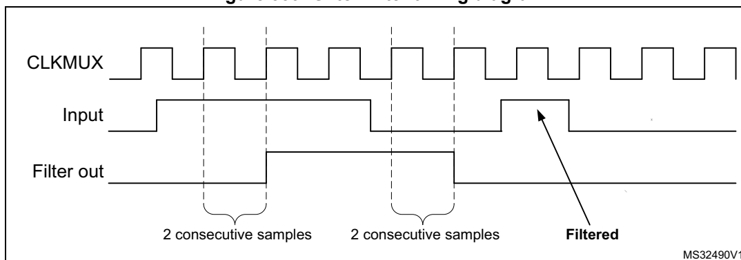
Figure 339. Glitch filter timing diagram
