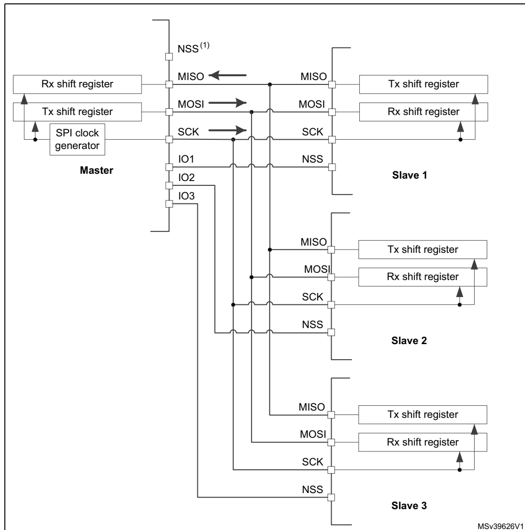
Figure 409. Master and three independent slaves
