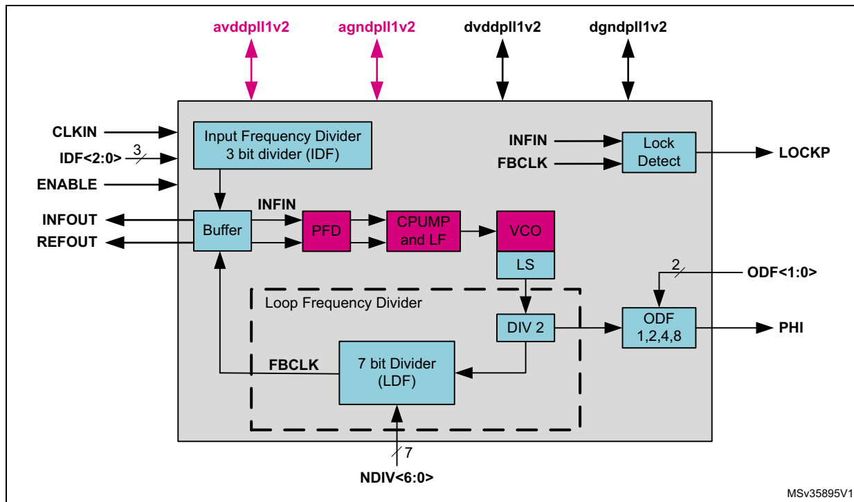
Figure 156. PLL block diagram
