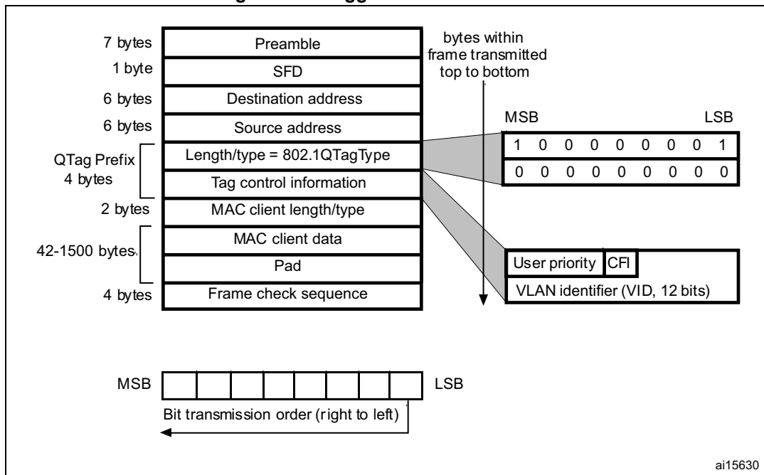
Figure 552. Tagged MAC frame format
