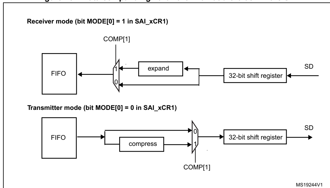
Figure 454. Data companding hardware in an audio block in the SAI
