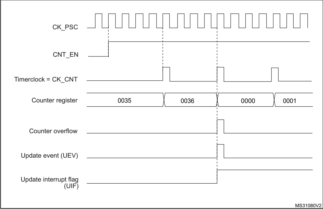
Figure 308. Counter timing diagram, internal clock divided by 4
