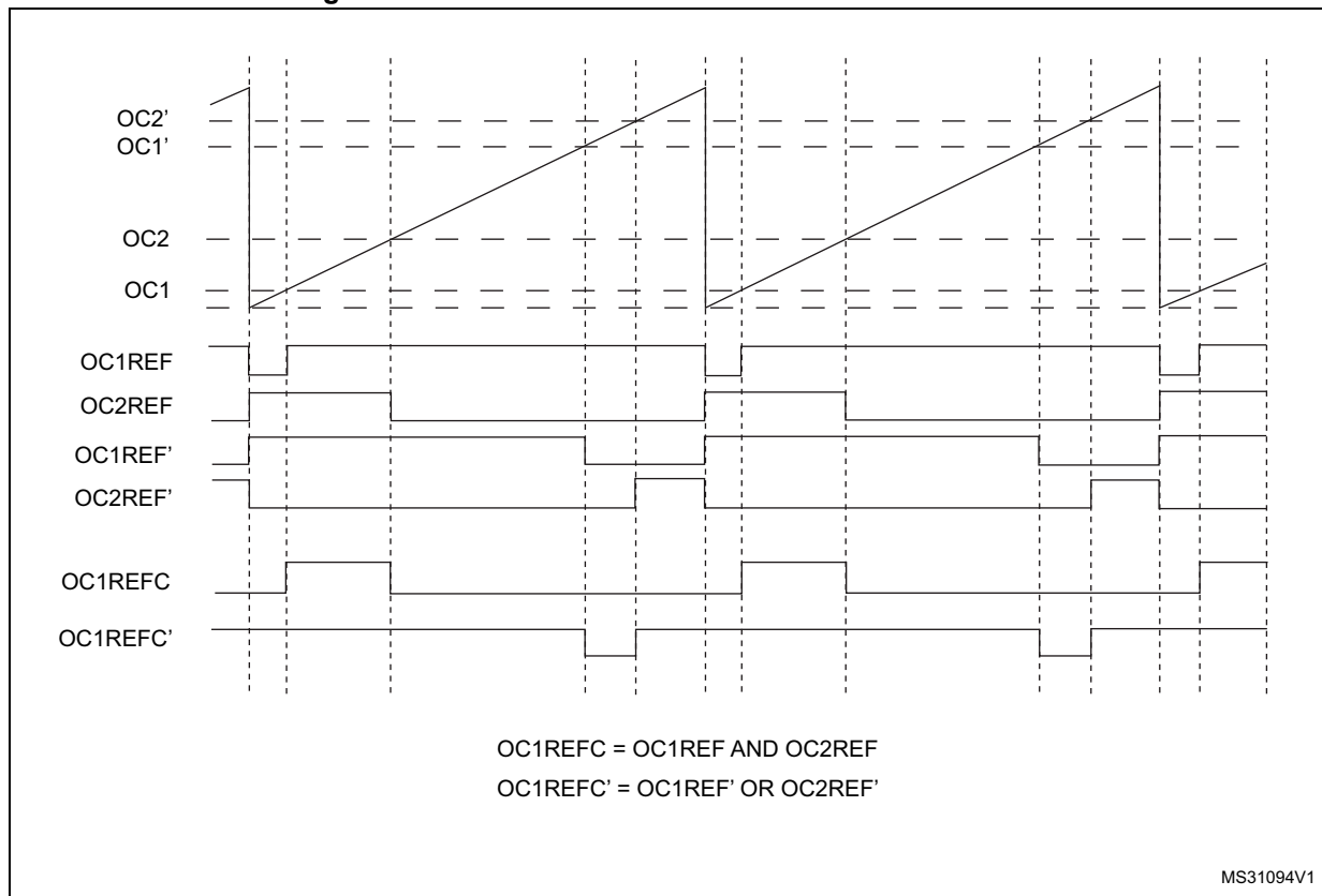
Figure 286. Combined PWM mode on channels 1 and 3
