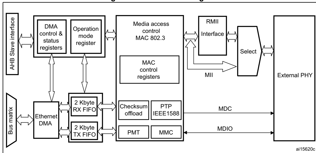
Figure 541. ETH block diagram
