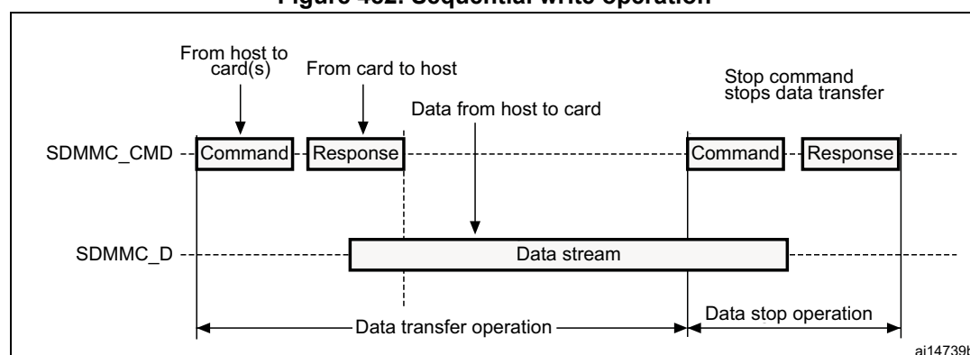
Figure 482. Sequential write operation
