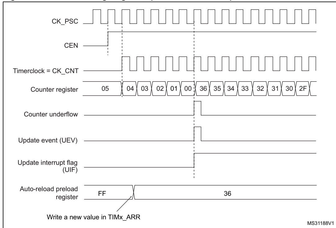
Figure 208. Counter timing diagram, update event when repetition counter is not used
