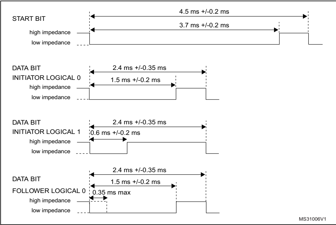
Figure 580. Bit timings
