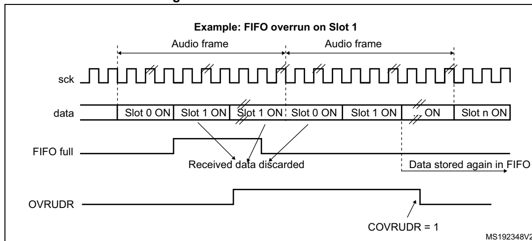
Figure 457. Overrun detection error
