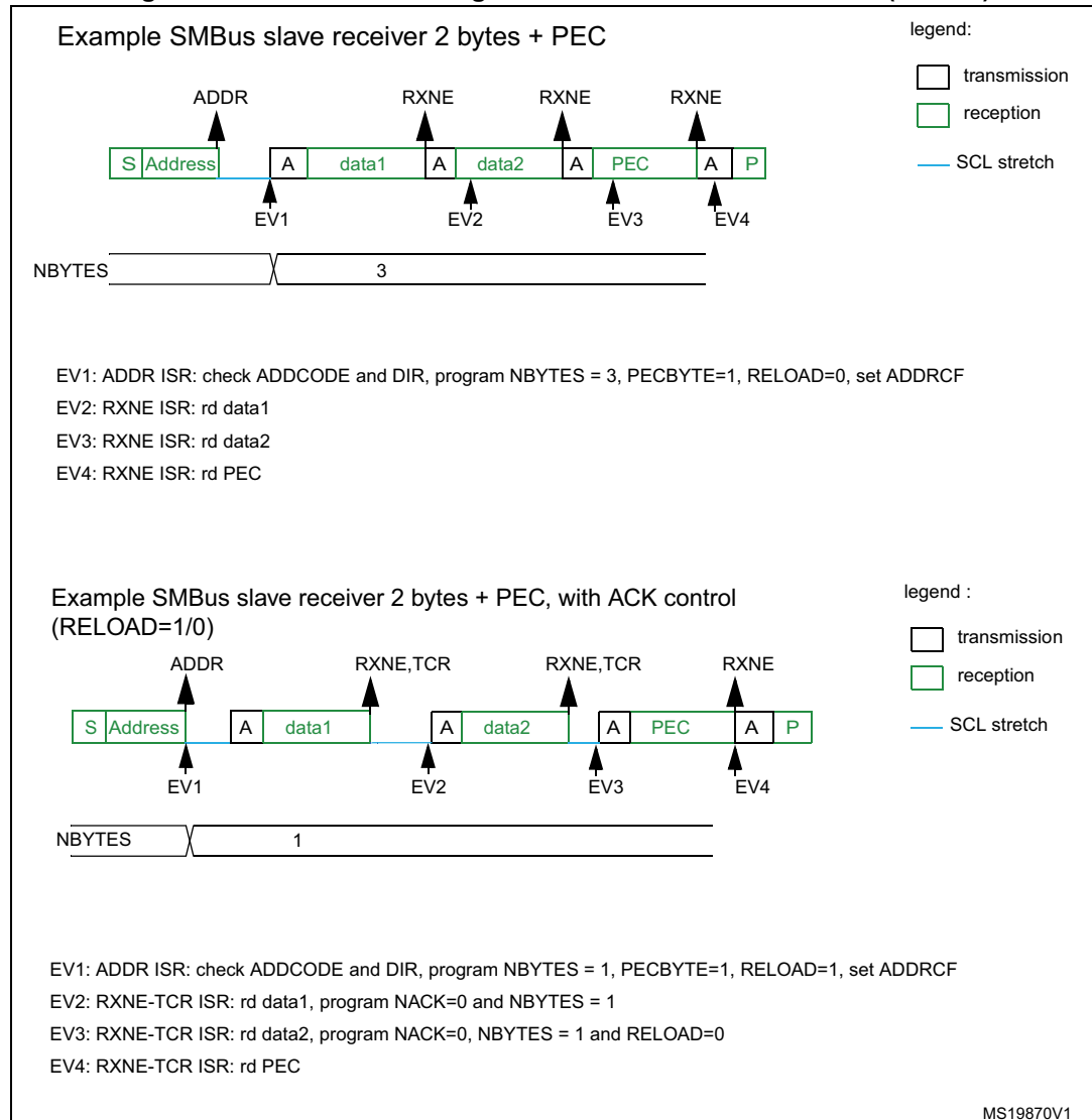
Figure 376. Bus transfer diagrams for SMBus slave receiver (SBC=1)
