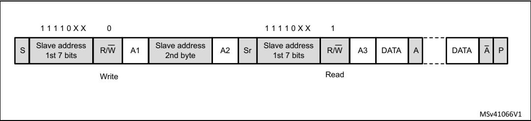
Figure 364. 10-bit address read access with HEAD10R=0
