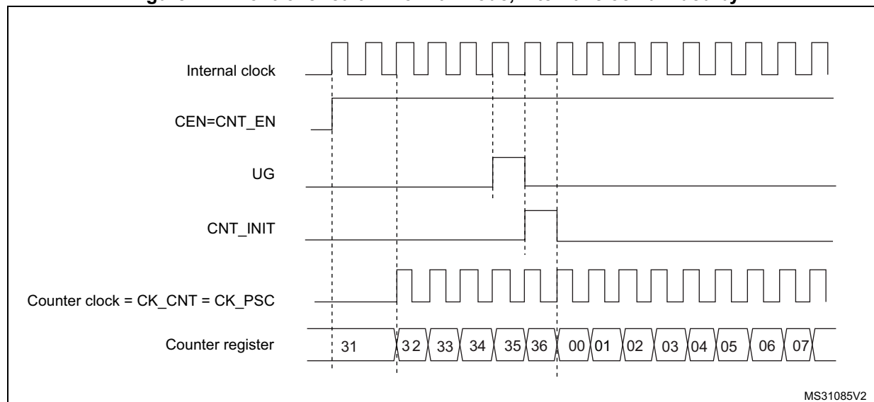
Figure 217. Control circuit in normal mode, internal clock divided by 1
