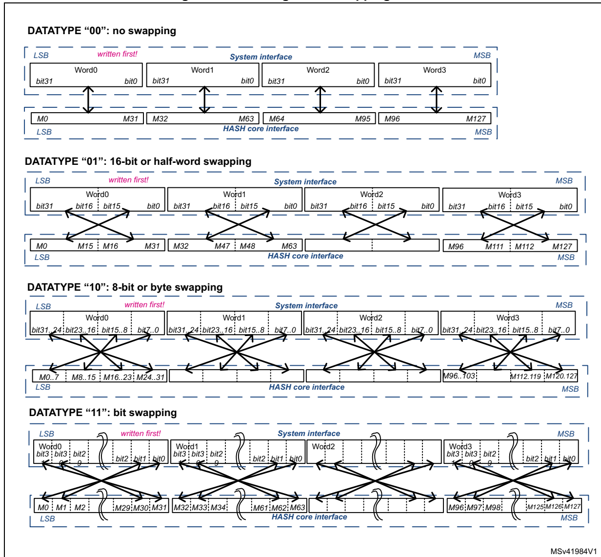
Figure 192. Message data swapping feature
