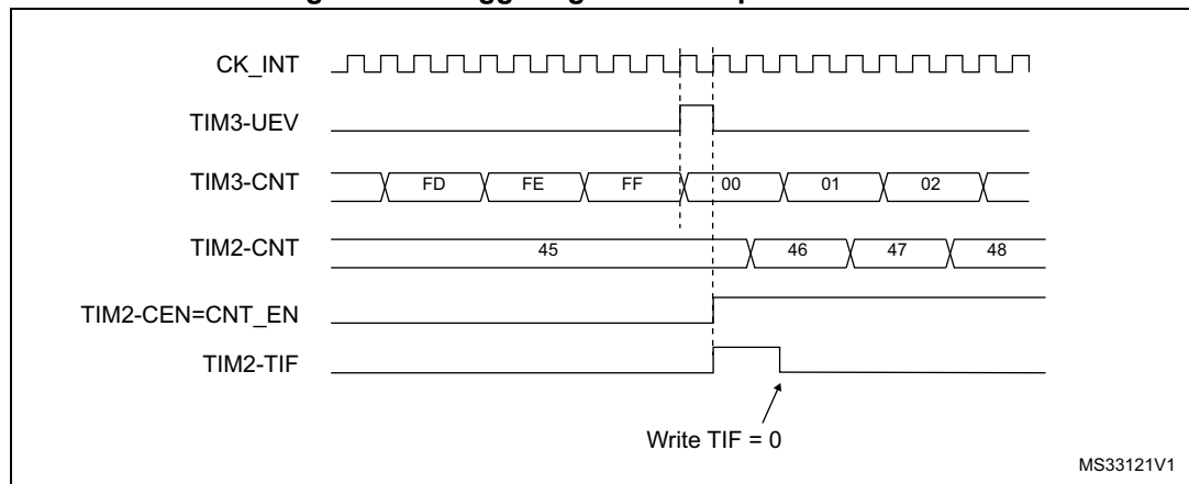
Figure 299. Triggering TIM with update of TIM3
