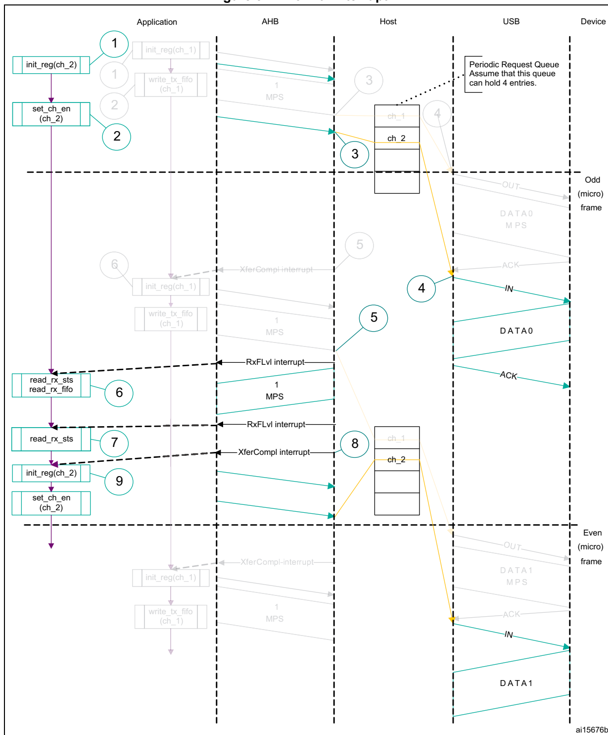
Figure 524. Normal interrupt IN
