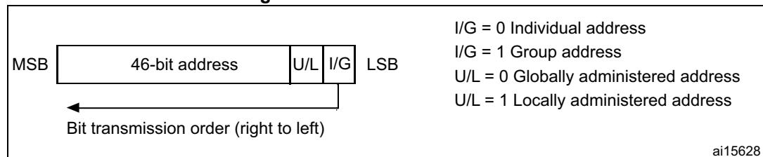
Figure 550. Address field format
