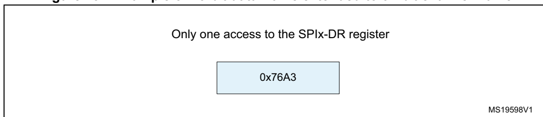
Figure 437. Example of 16-bit data frame extended to 32-bit channel frame
