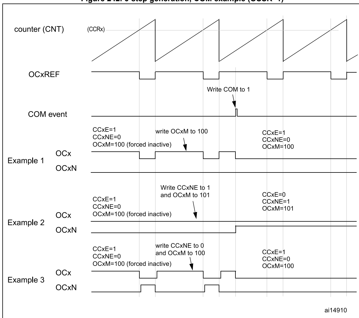
Figure 242. 6-step generation, COM example (OSSR=1)
