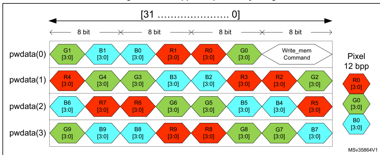
Figure 133. 12 bpp APB pixel to byte organization
