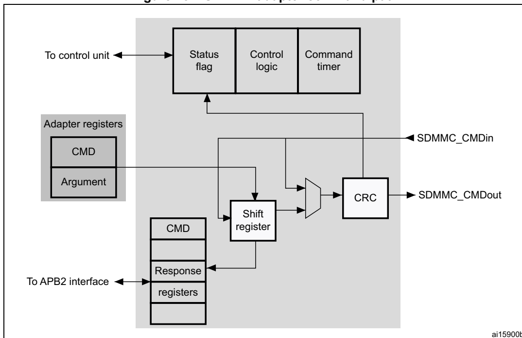
Figure 487. SDMMC adapter command path
