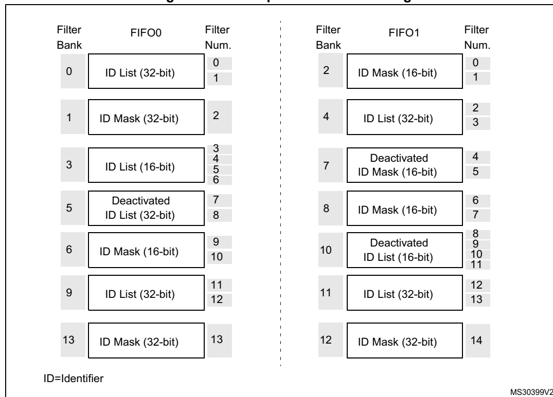
Figure 502. Example of filter numbering
