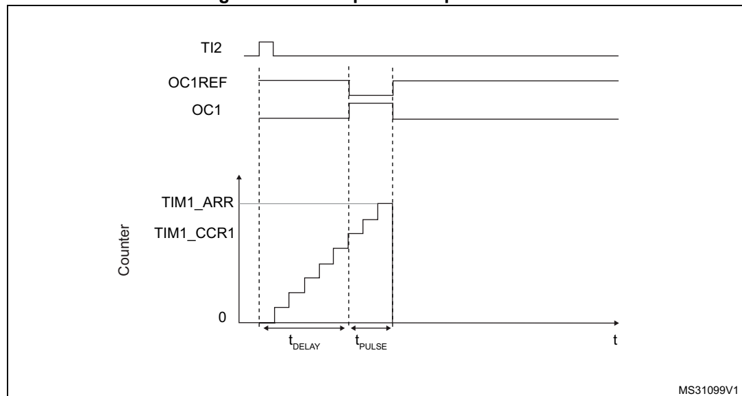
Figure 243. Example of one pulse mode.
