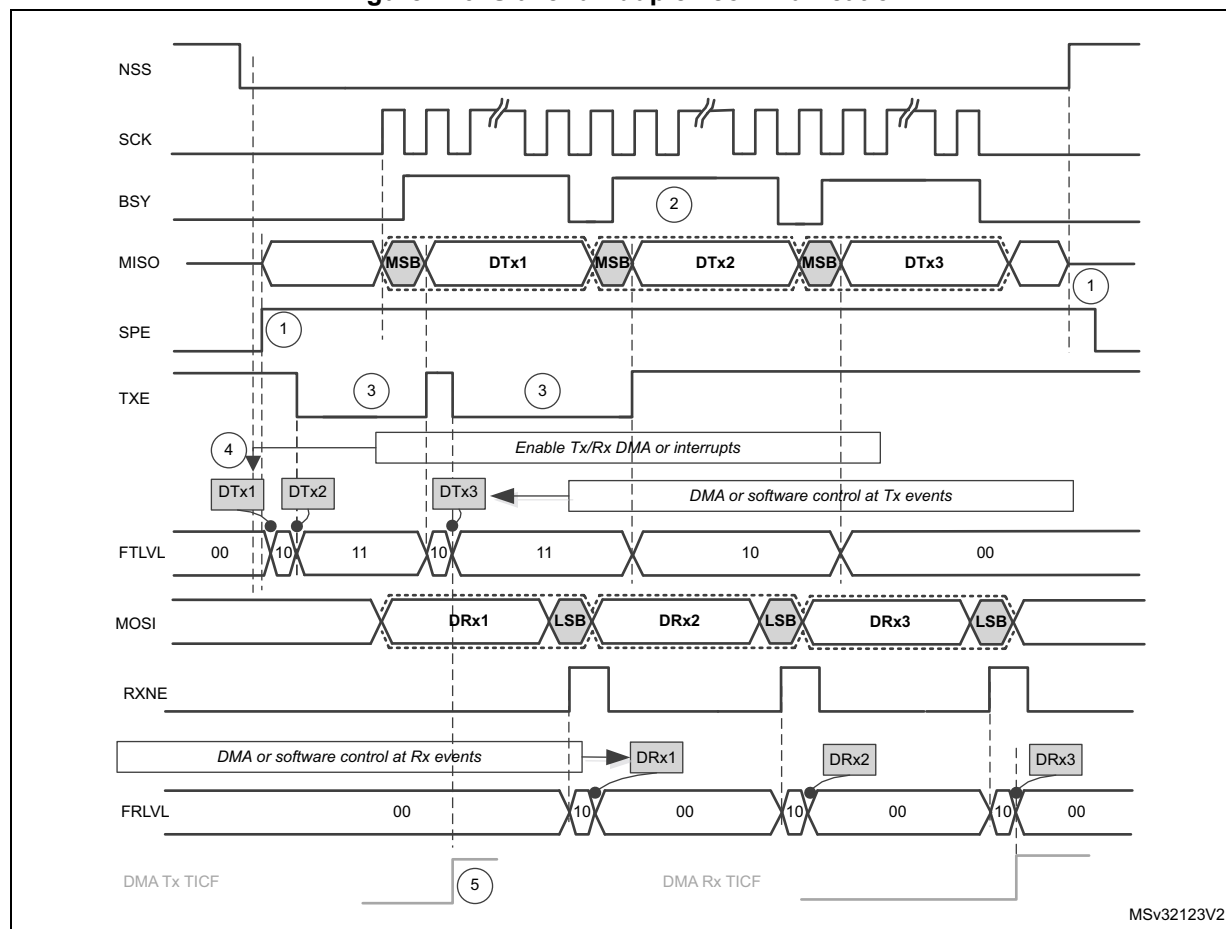
Figure 416. Slave full-duplex communication
