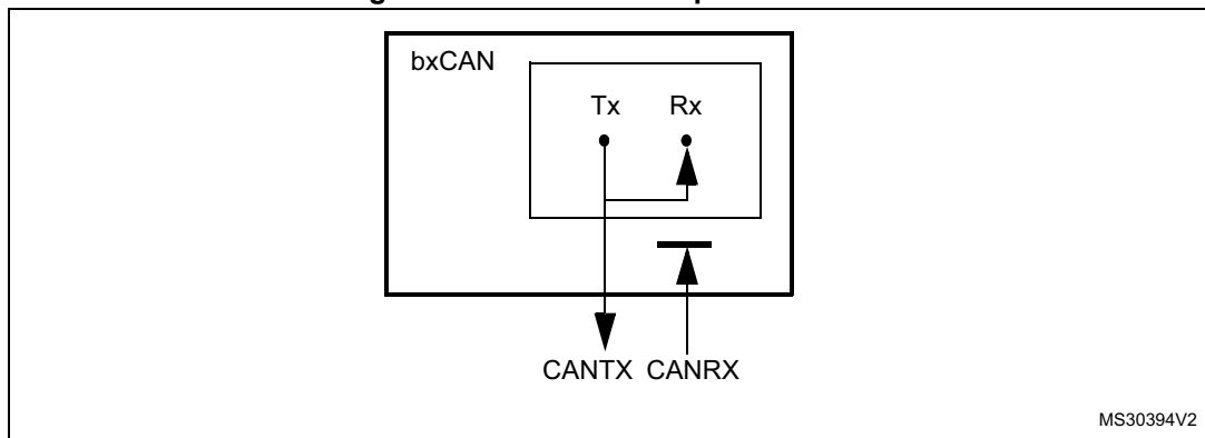
Figure 497. bxCAN in loop back mode
