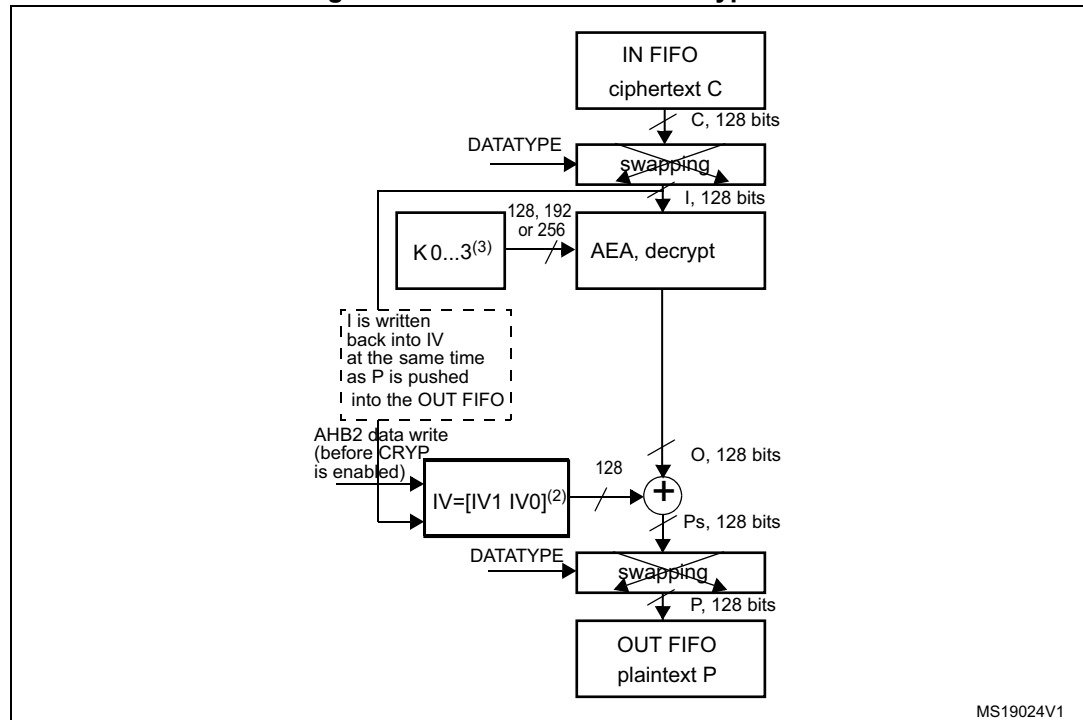
Figure 181. AES-CBC mode decryption
