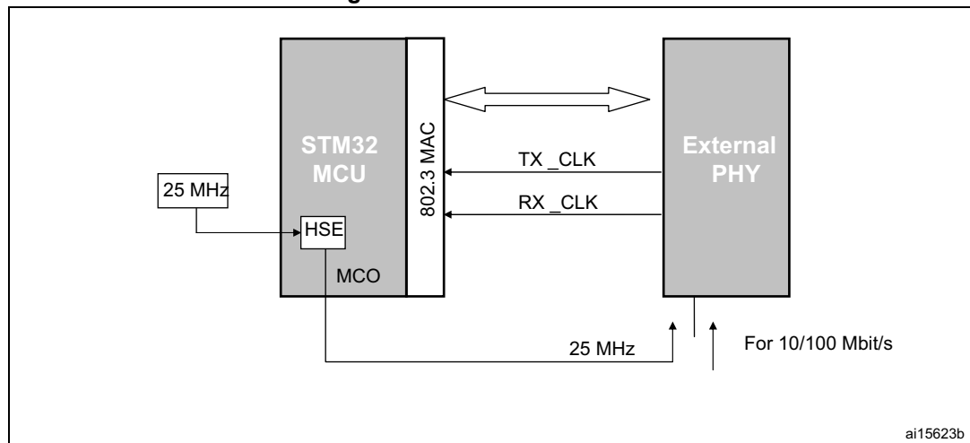
Figure 546. MII clock sources
