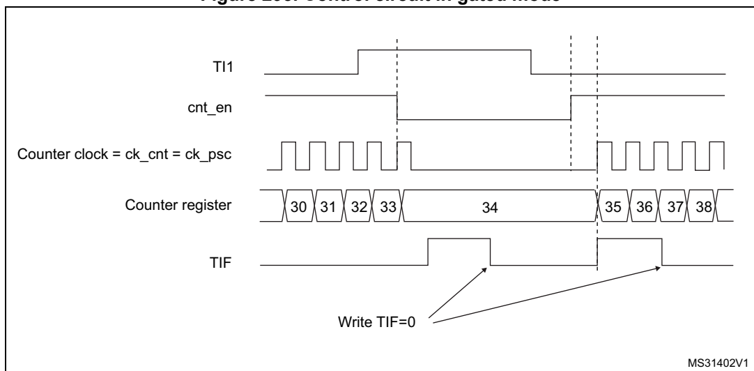
Figure 293. Control circuit in gated mode
