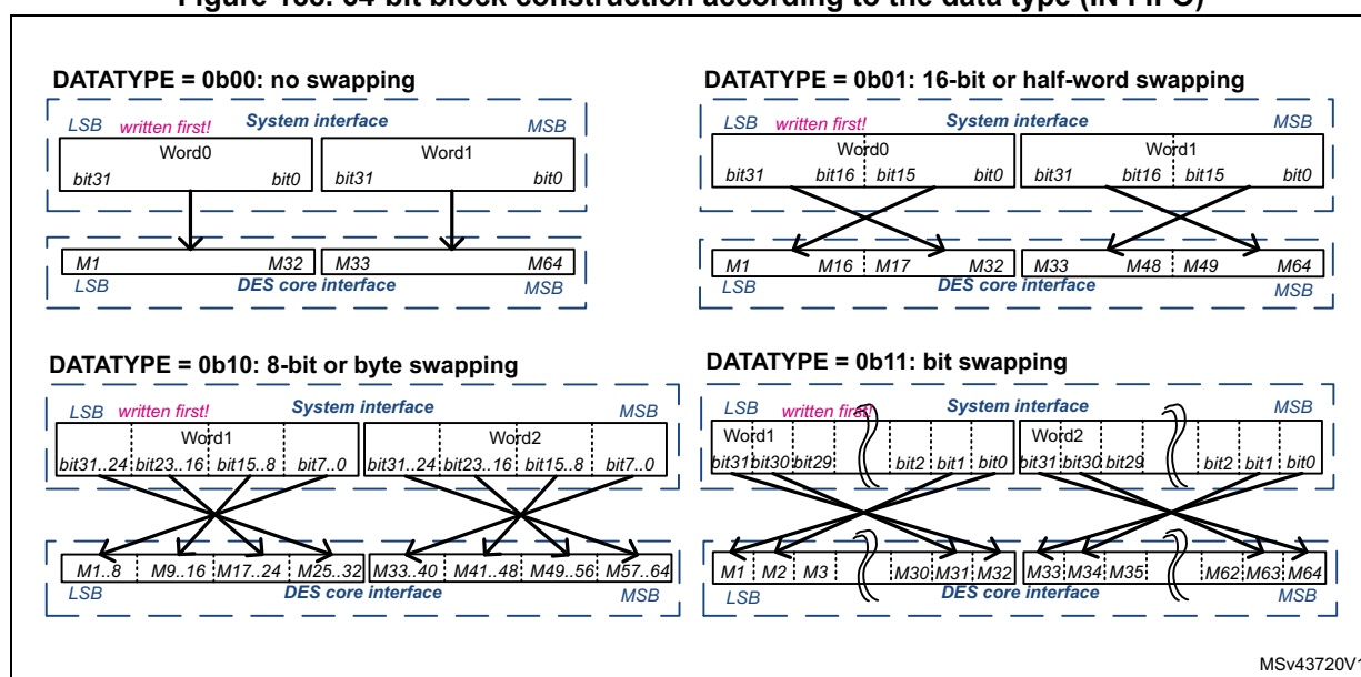
Figure 188. 64-bit block construction according to the data type (IN FIFO)
