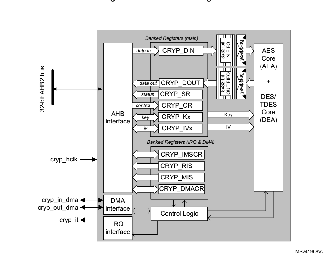
Figure 164. CRYP block diagram
