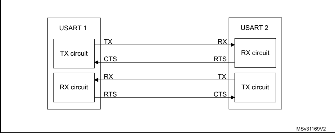
Figure 401. Hardware flow control between 2 USARTs
