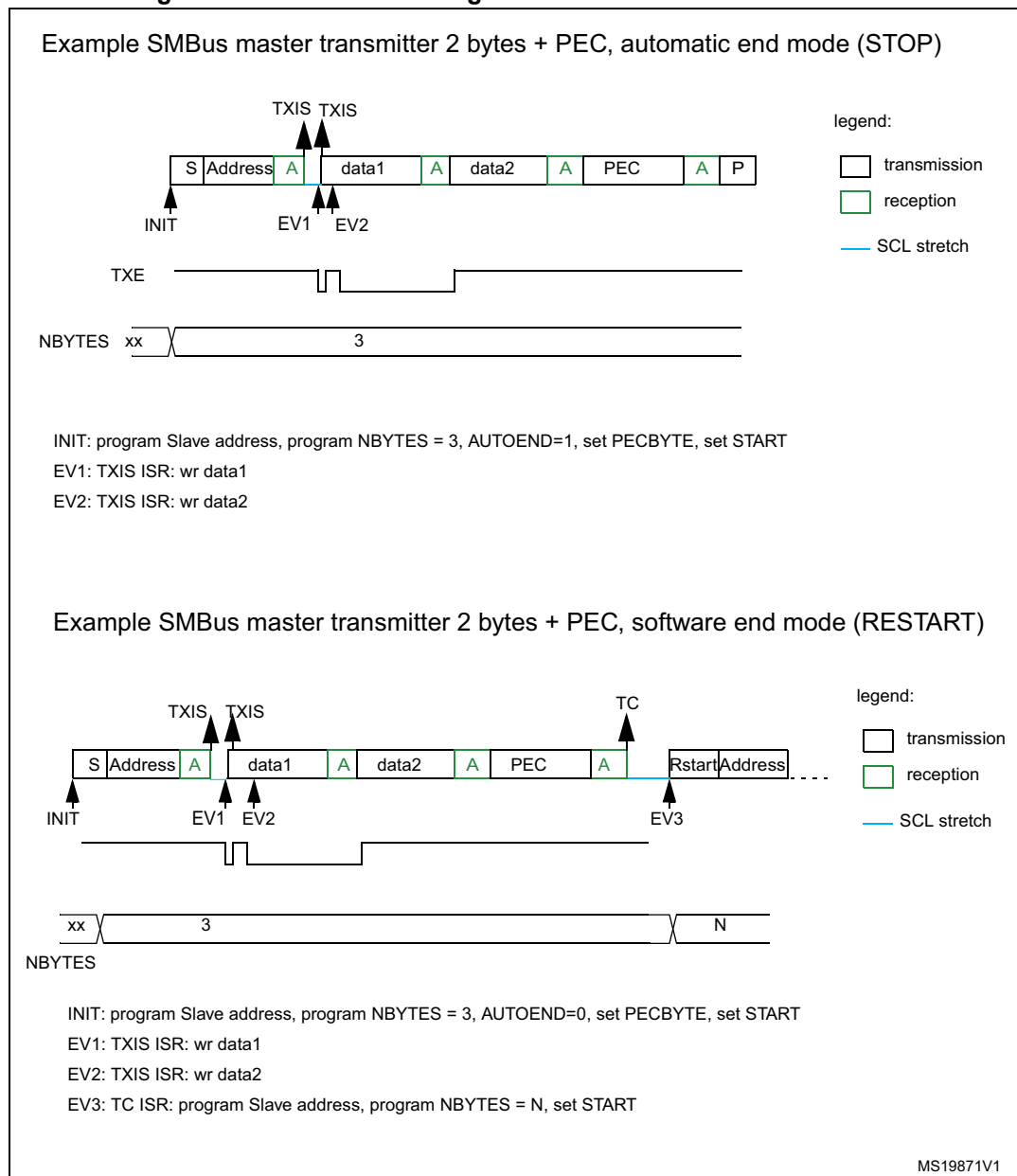
Figure 377. Bus transfer diagrams for SMBus master transmitter
