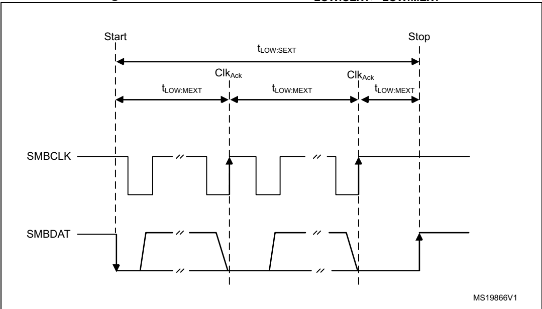
Figure 372. Timeout intervals for t_{\text{LOW:SEXT}} , t_{\text{LOW:MEXT}}
