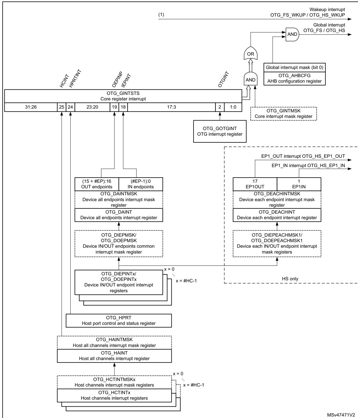
Figure 518. Interrupt hierarchy
