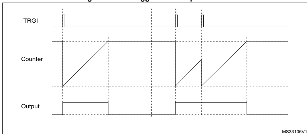
Figure 244. Retriggerable one pulse mode
