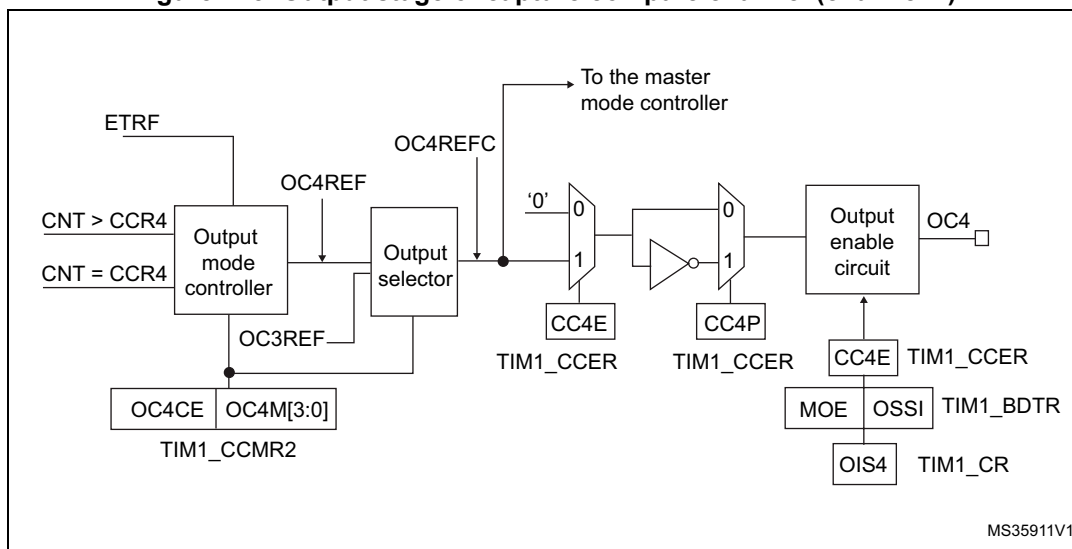
Figure 225. Output stage of capture/compare channel (channel 4)
