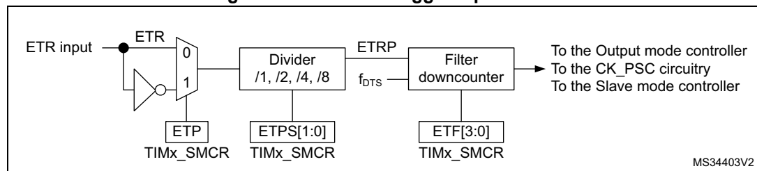
Figure 216. External trigger input block
