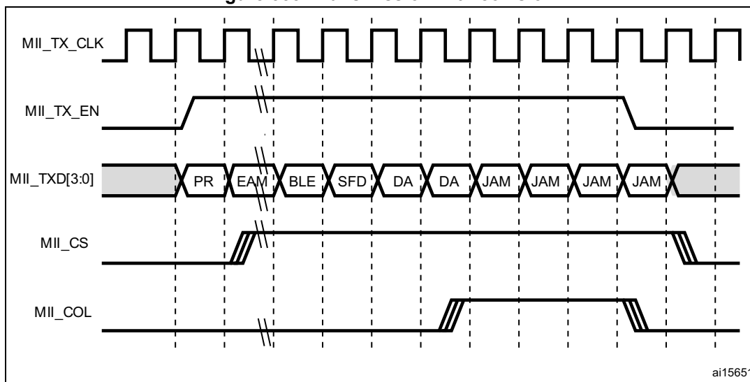
Figure 555. Transmission with collision
