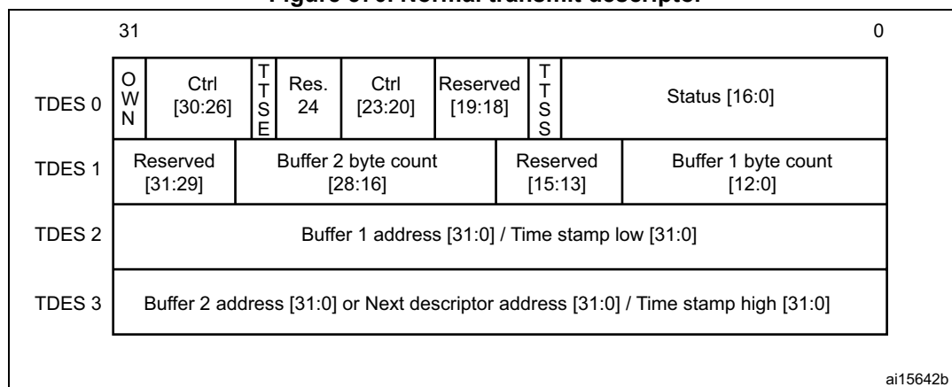
Figure 570. Normal transmit descriptor
