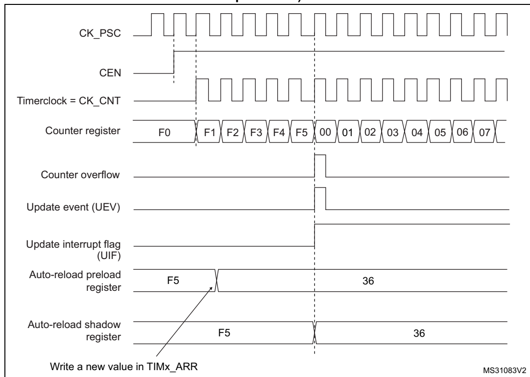
Figure 311. Counter timing diagram, update event when ARPE=1 (TIMx_ARR preloaded)
