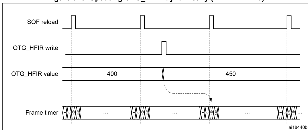
Figure 515. Updating OTG_HFIR dynamically (RLDCTRL = 0)
