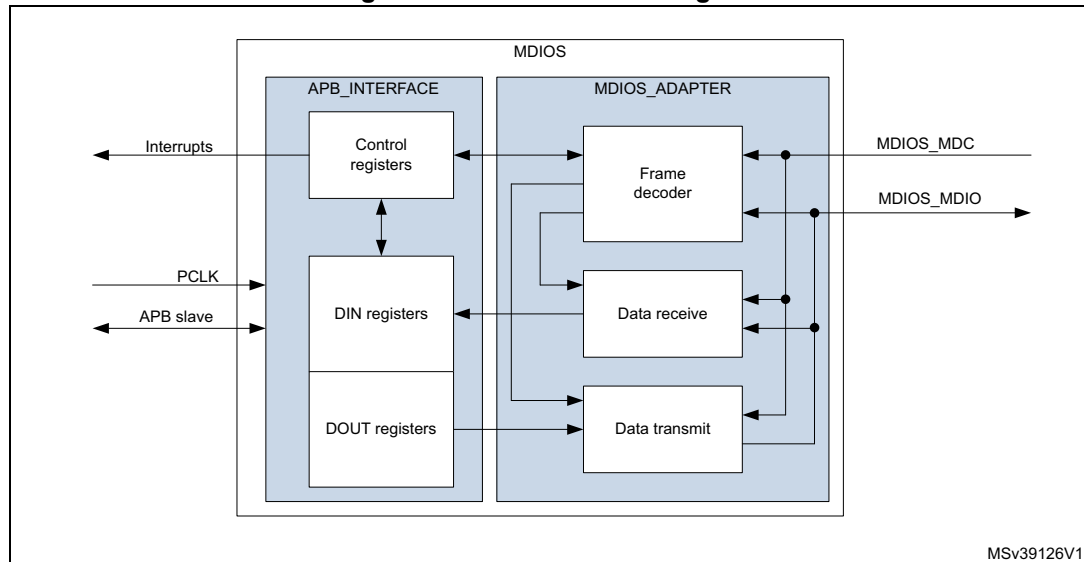
Figure 475. MDIOS block diagram
