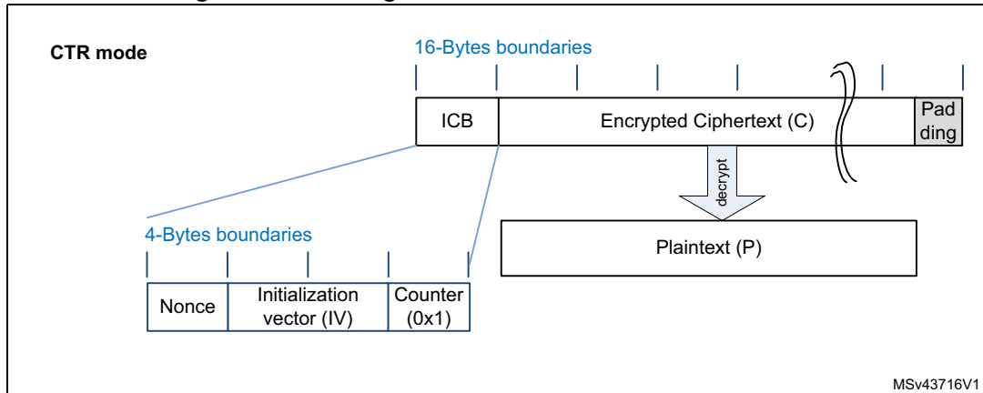
Figure 182. Message construction for the Counter mode
