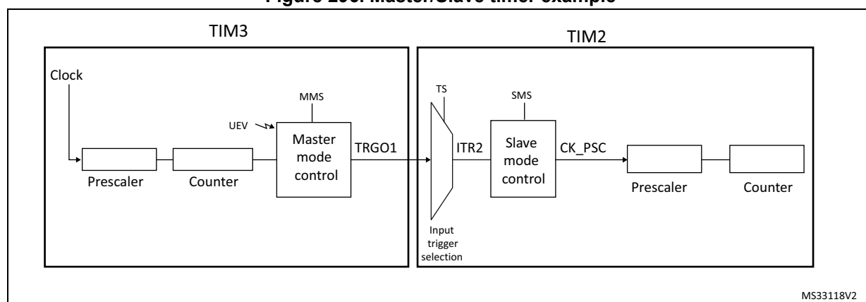
Figure 296. Master/Slave timer example
