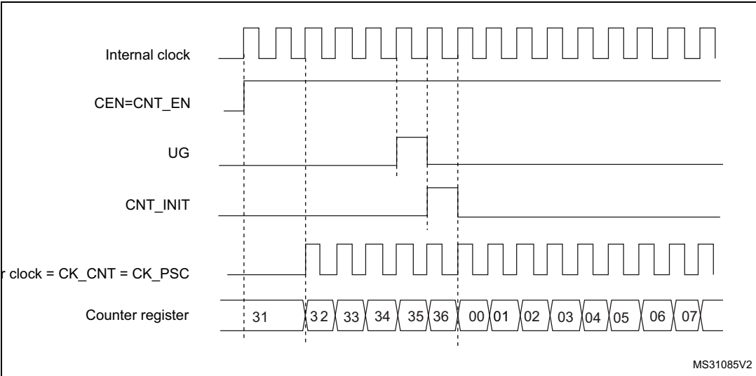
Figure 312. Control circuit in normal mode, internal clock divided by 1
