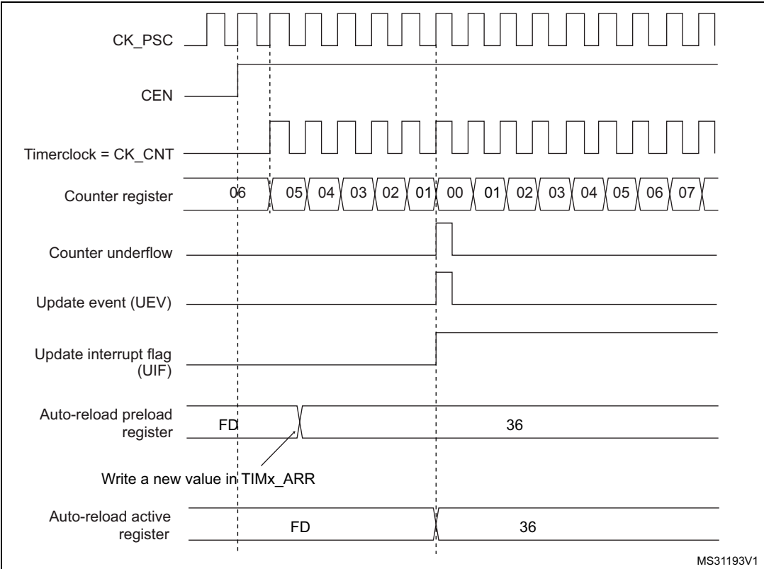
Figure 271. Counter timing diagram, Update event with ARPE=1 (counter underflow)
