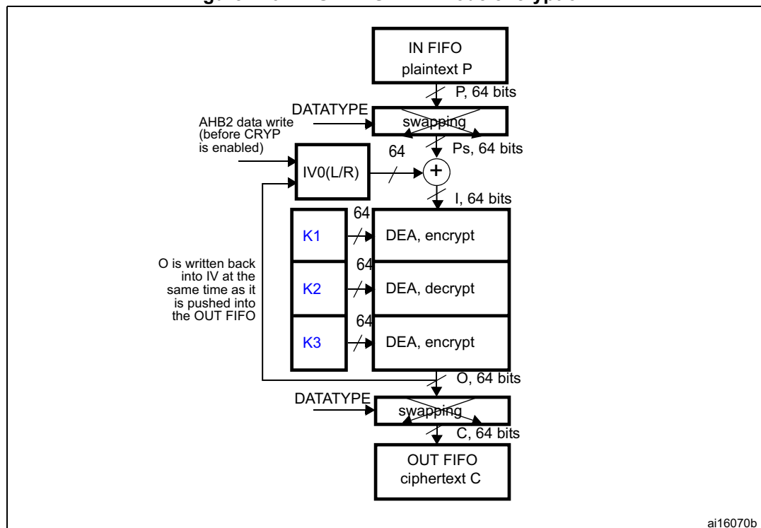
Figure 176. DES/TDES-CBC mode encryption
