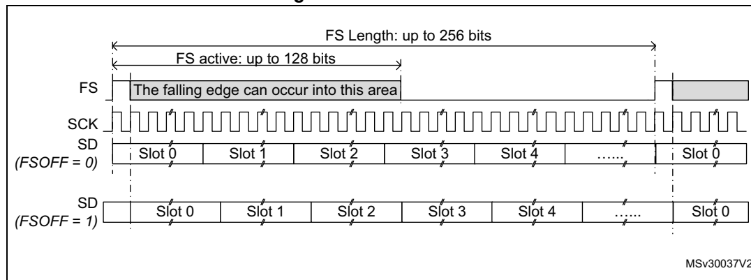
Figure 444. Audio frame
