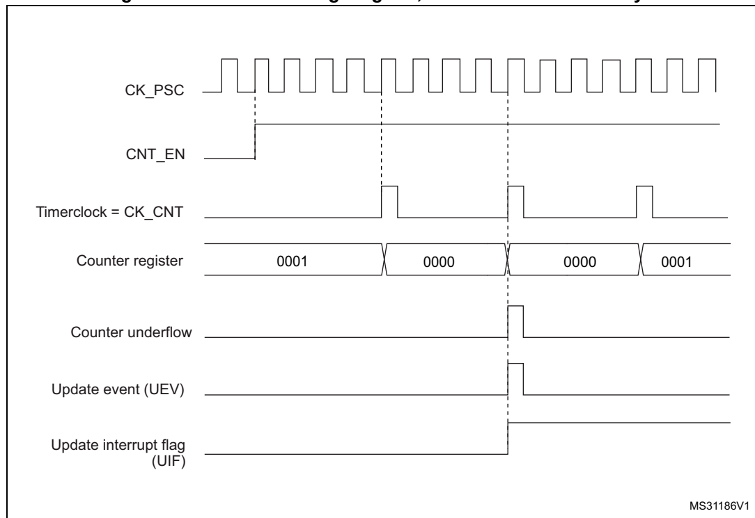
Figure 265. Counter timing diagram, internal clock divided by N
