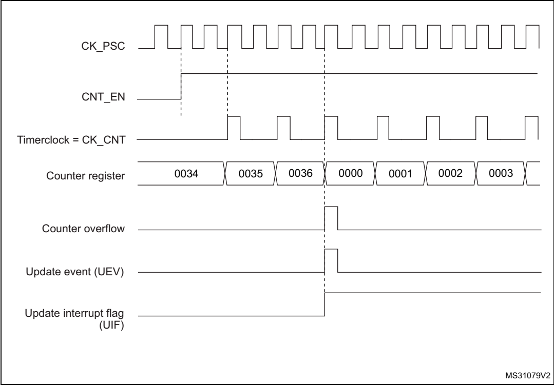
Figure 307. Counter timing diagram, internal clock divided by 2
