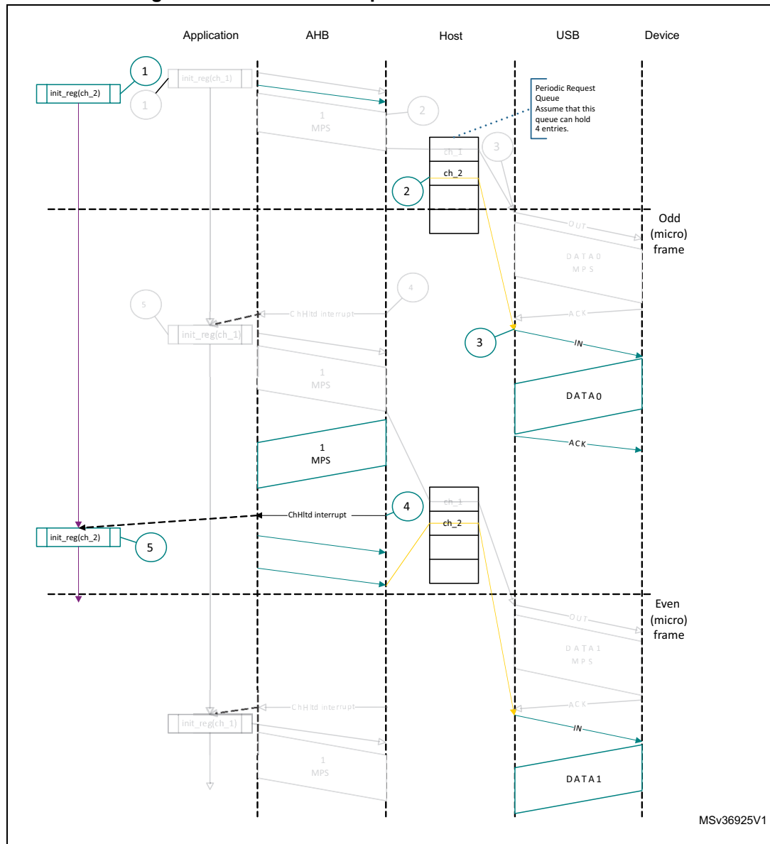
Figure 530. Normal interrupt IN transactions - DMA mode
