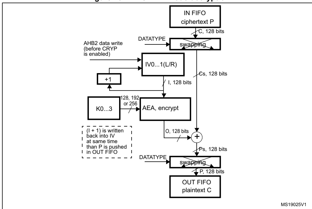
Figure 184. AES-CTR mode decryption
