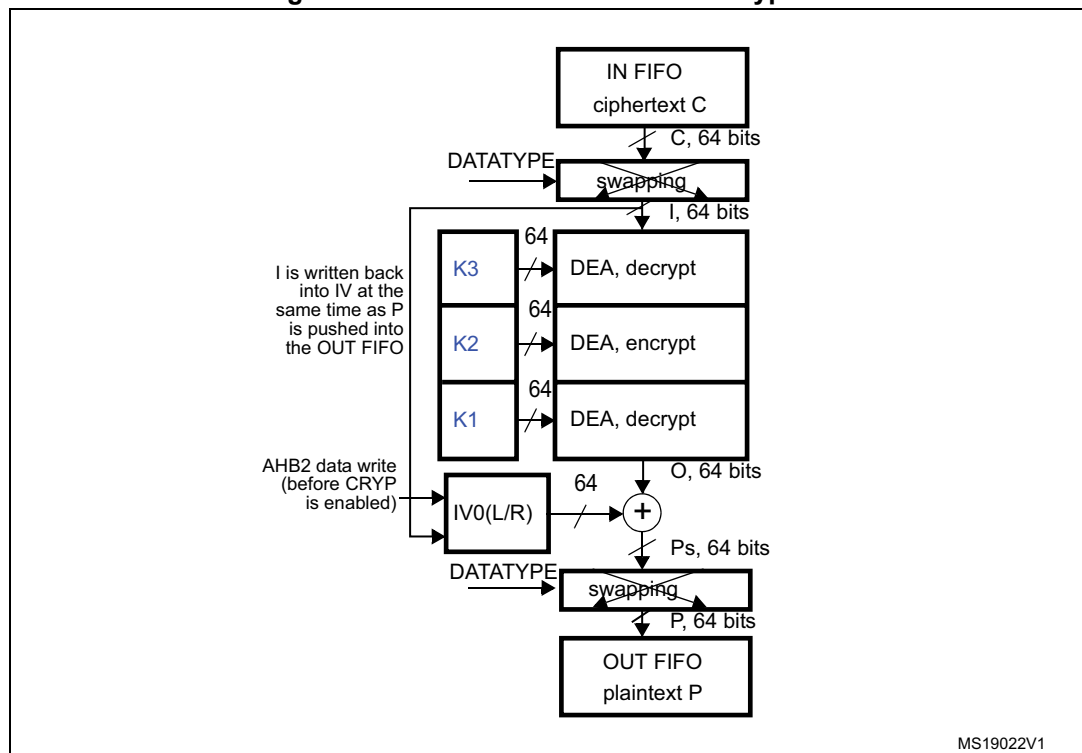
Figure 177. DES/TDES-CBC mode decryption
