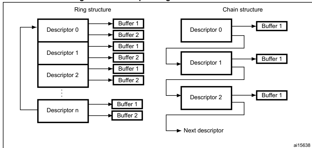
Figure 567. Descriptor ring and chain structure
