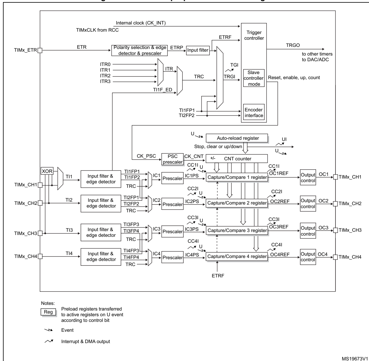
Figure 253. General-purpose timer block diagram
