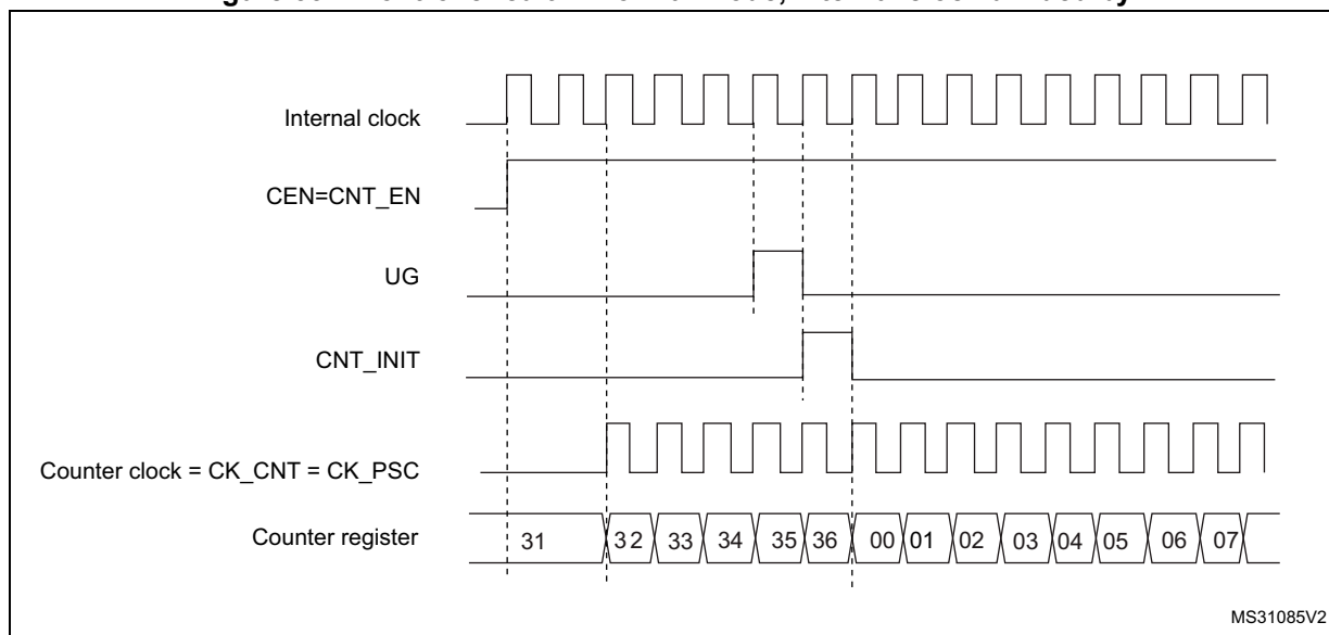
Figure 337. Control circuit in normal mode, internal clock divided by 1
