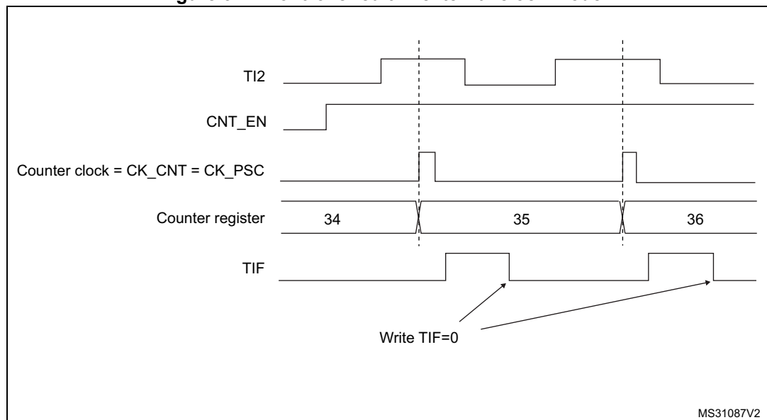
Figure 314. Control circuit in external clock mode 1
