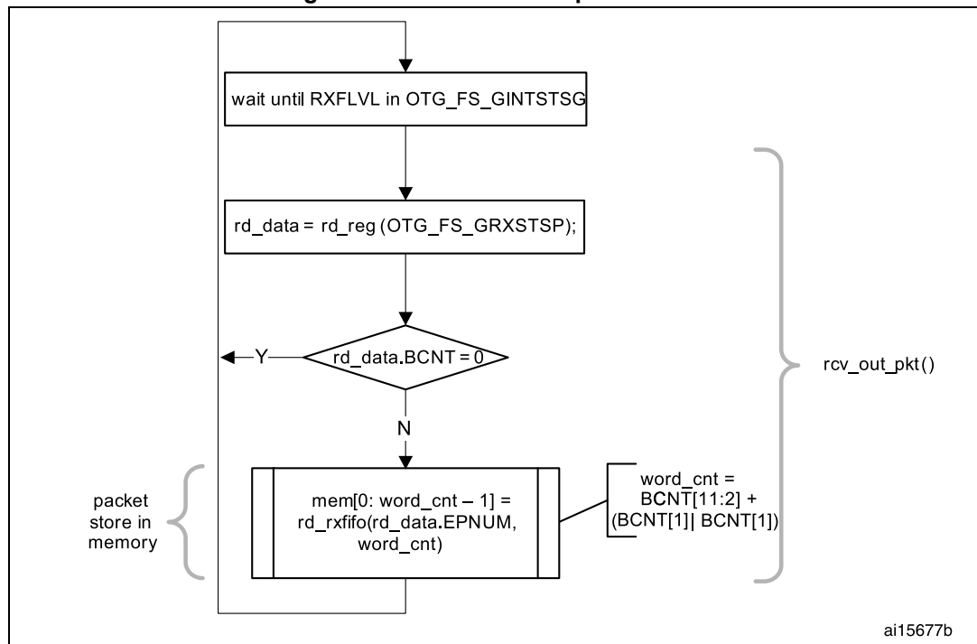
Figure 533. Receive FIFO packet read
