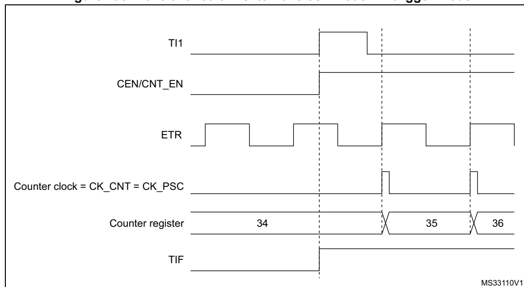
Figure 295. Control circuit in external clock mode 2 + trigger mode
