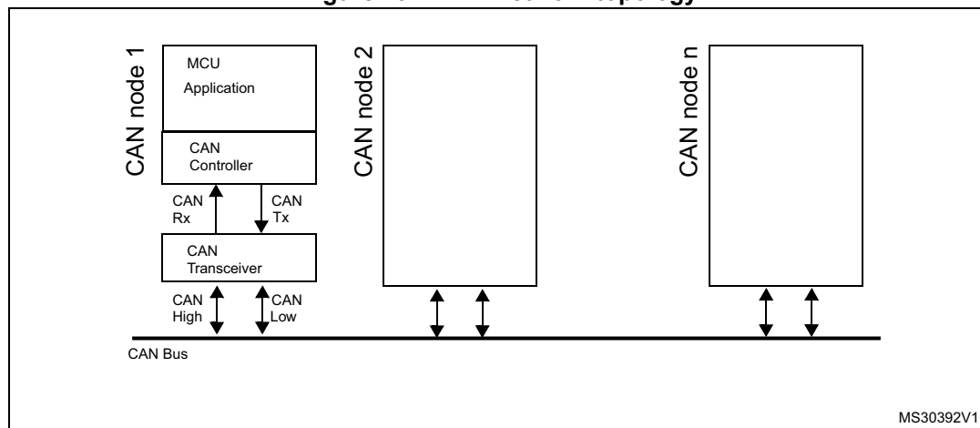
Figure 492. CAN network topology
