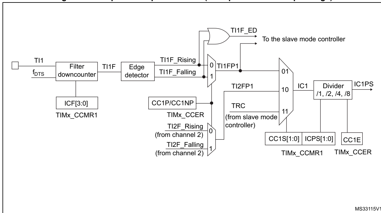
Figure 278. Capture/compare channel (example: channel 1 input stage)
