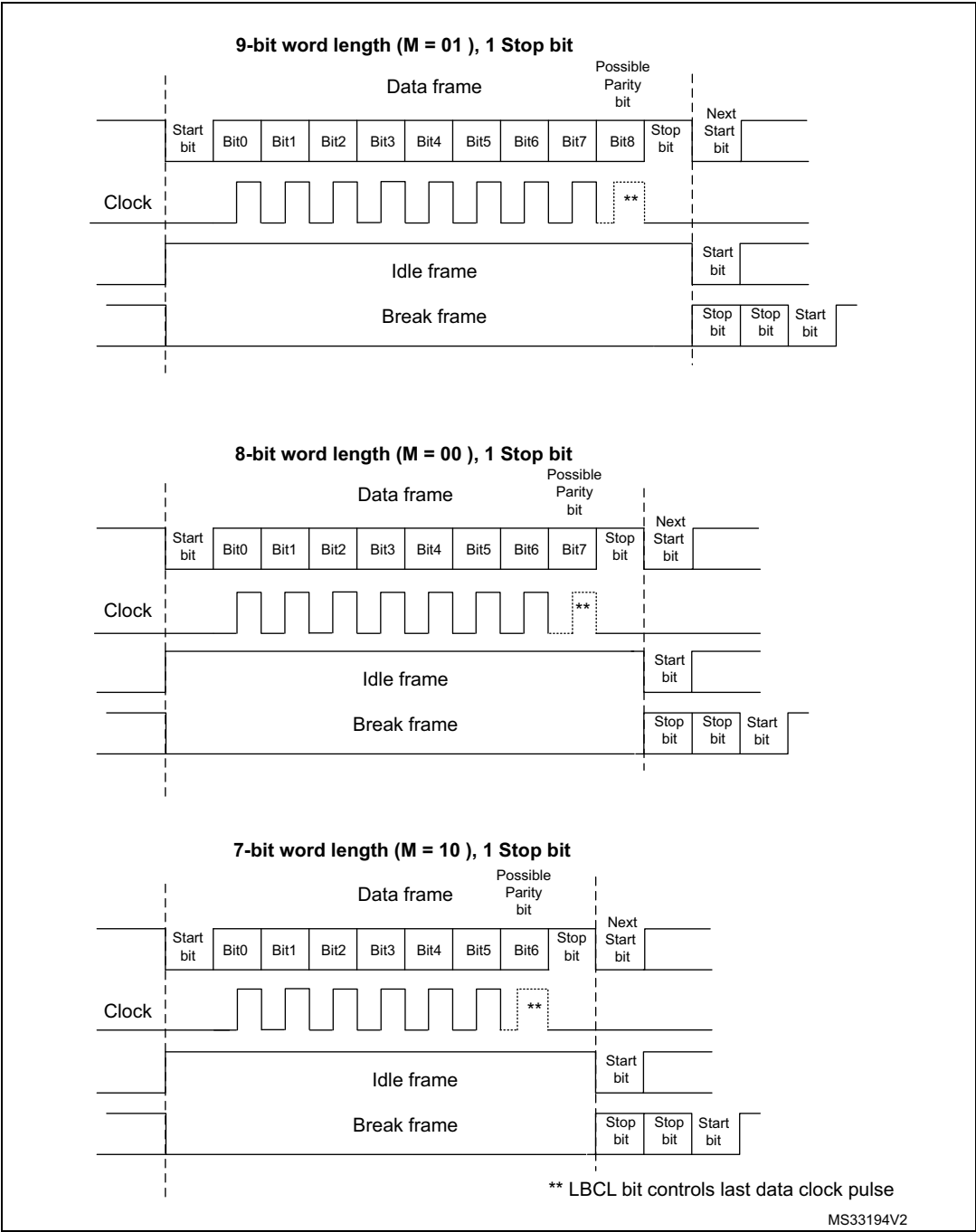
Figure 381. Word length programming
