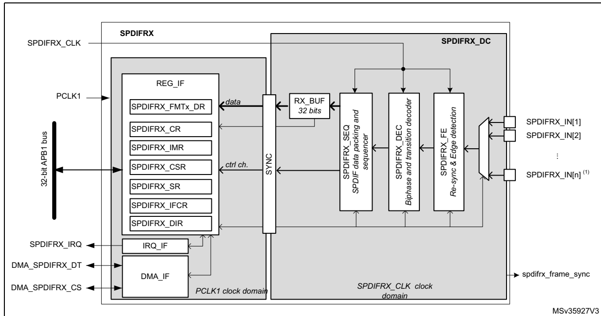
Figure 459. SPDIFRX block diagram
