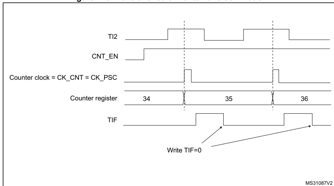
Figure 275. Control circuit in external clock mode 1
