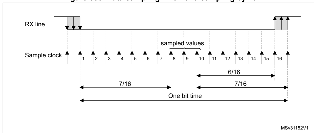
Figure 385. Data sampling when oversampling by 16
