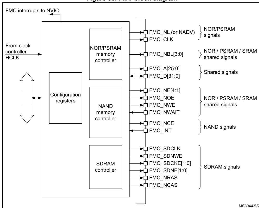
Figure 33. FMC block diagram
