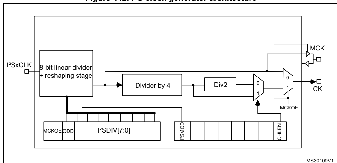
Figure 442. I 2 S clock generator architecture
