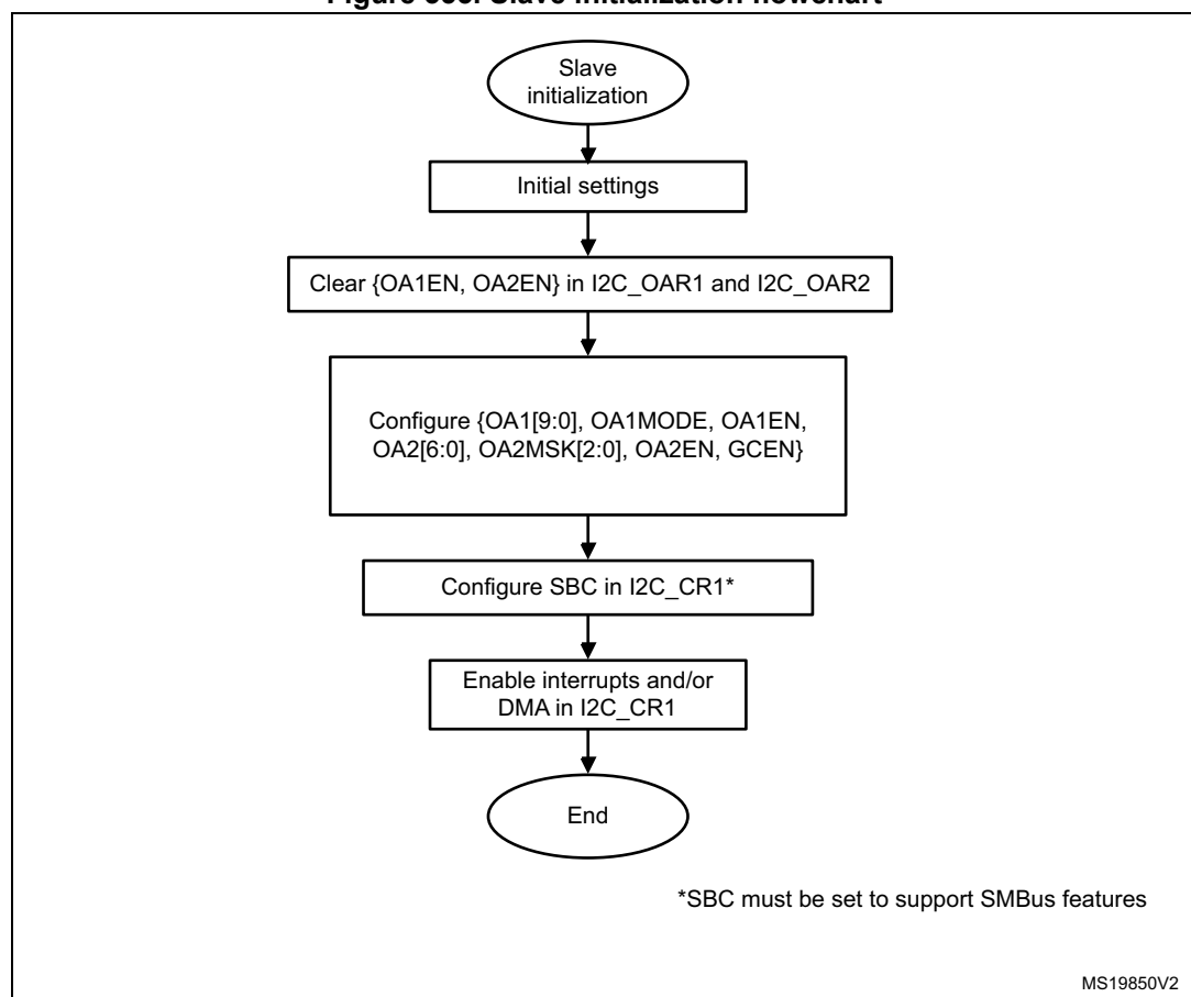
Figure 355. Slave initialization flowchart
