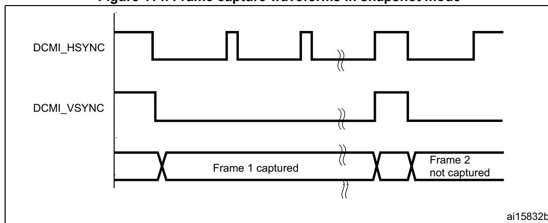
Figure 114. Frame capture waveforms in snapshot mode
