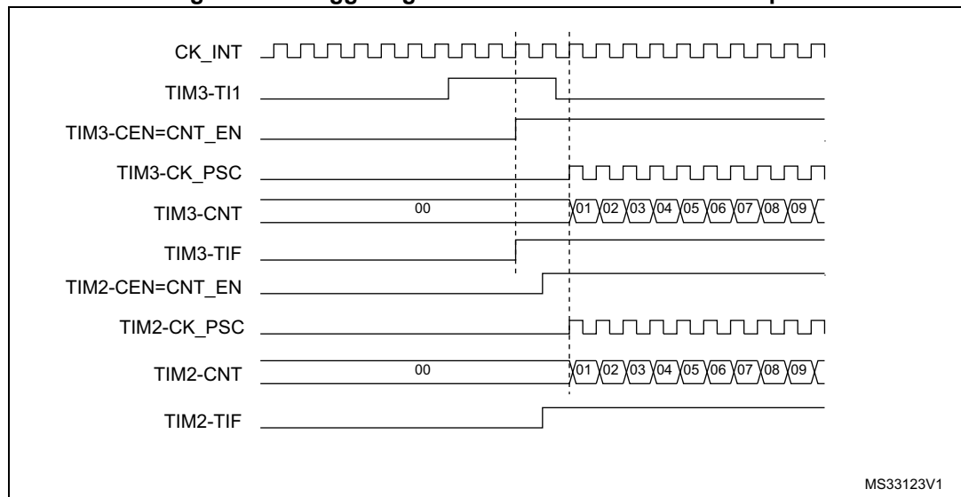
Figure 301. Triggering TIM3 and TIM2 with TIM3 TI1 input
