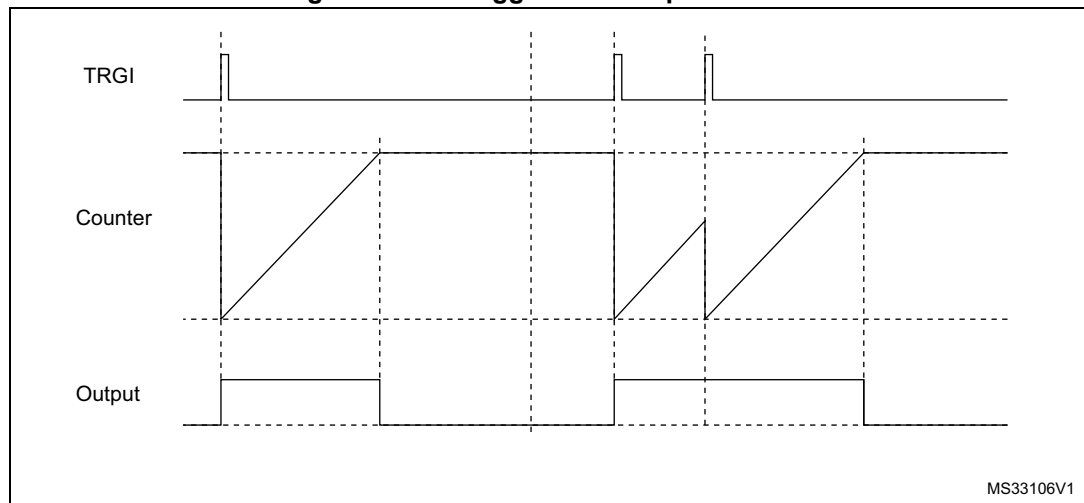
Figure 323. Retriggerable one pulse mode
