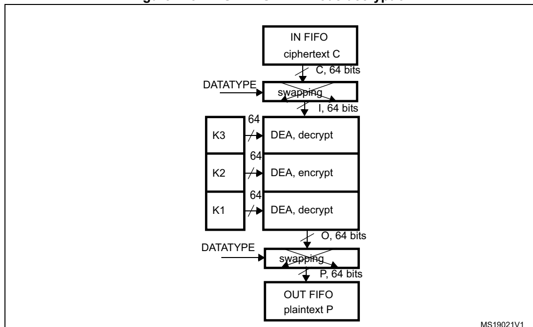
Figure 175. DES/TDES-ECB mode decryption
