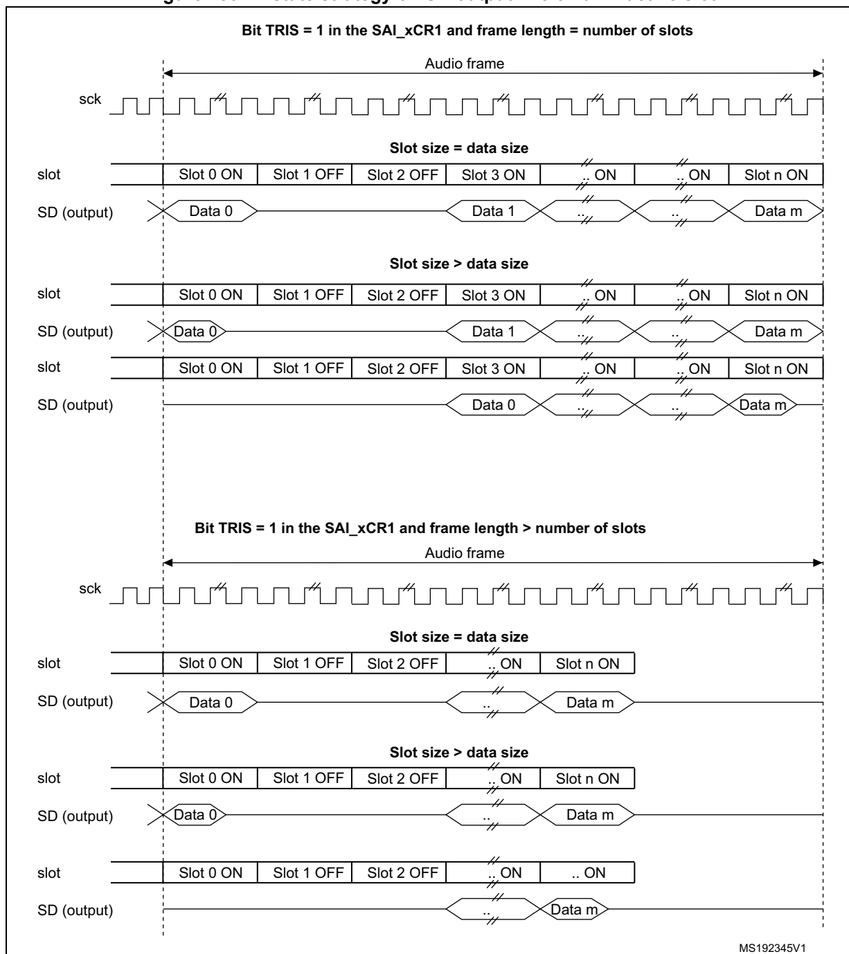
Figure 455. Tristate strategy on SD output line on an inactive slot
