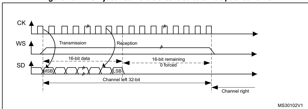
Figure 431. MSB justified 16-bit extended to 32-bit packet frame
