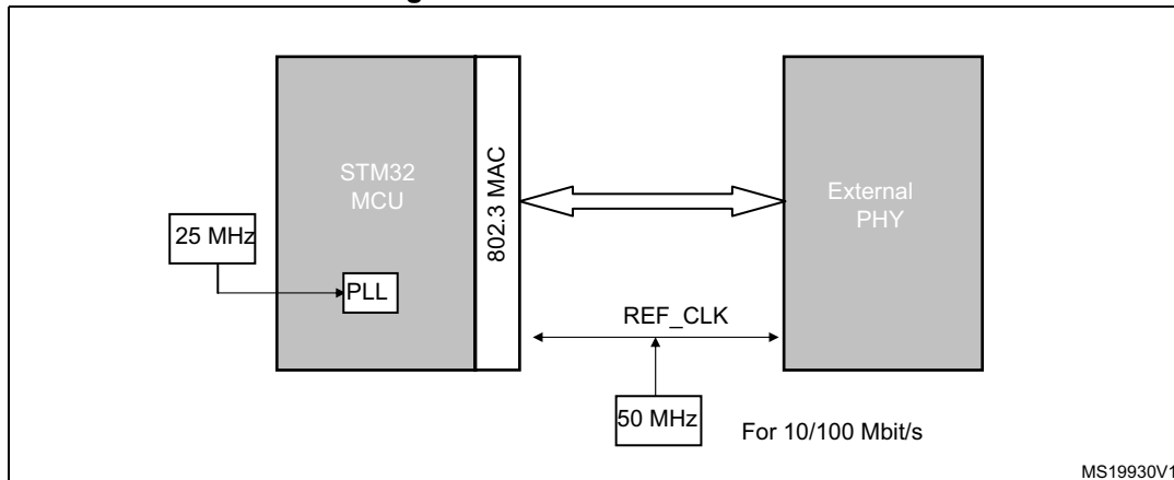
Figure 548. RMII clock sources-
