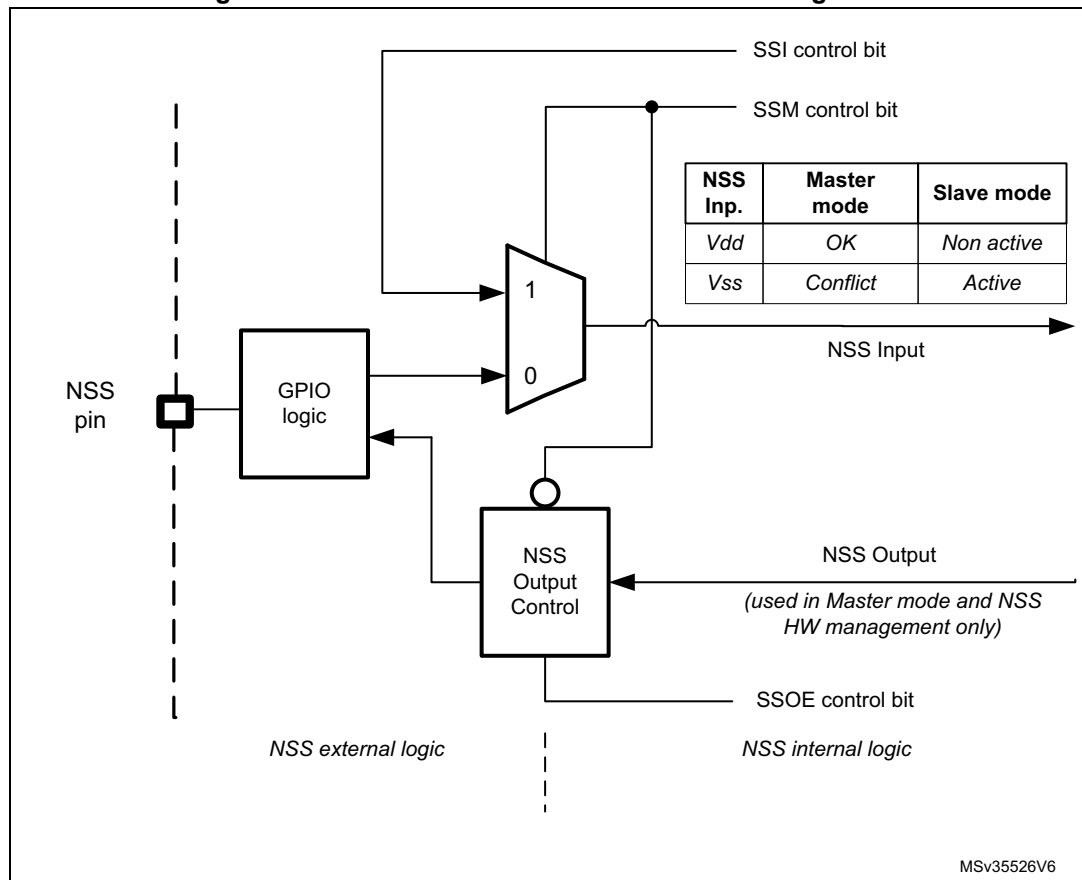
Figure 411. Hardware/software slave select management
