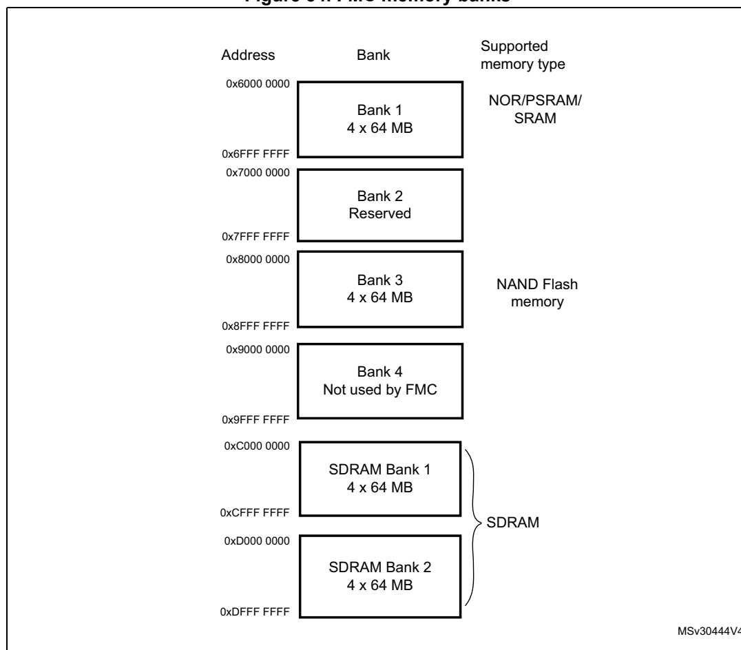
Figure 34. FMC memory banks
