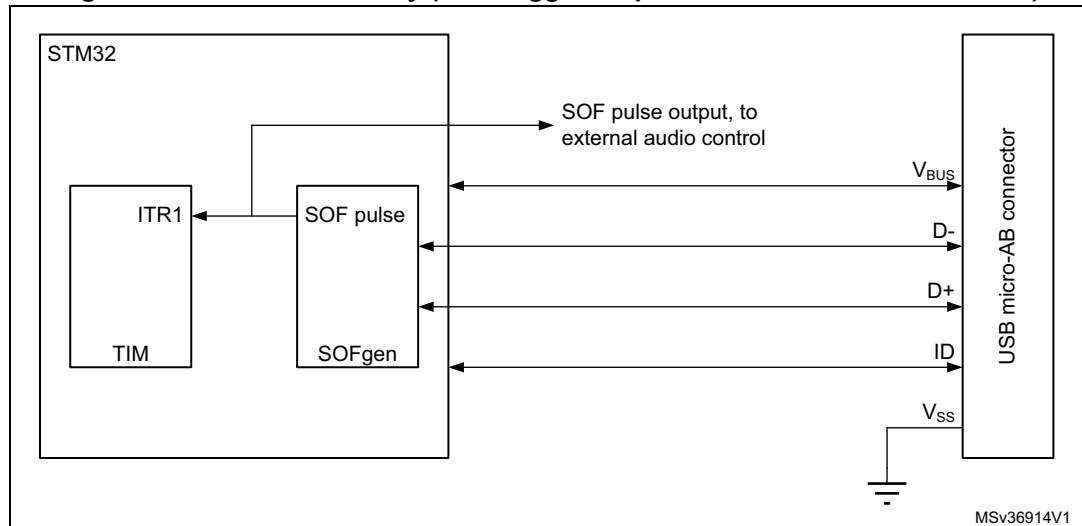
Figure 514. SOF connectivity (SOF trigger output to TIM and ITR1 connection)
