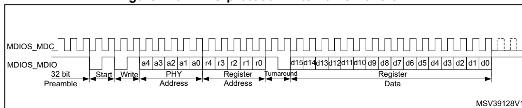
Figure 476. MDIO protocol write frame waveform
