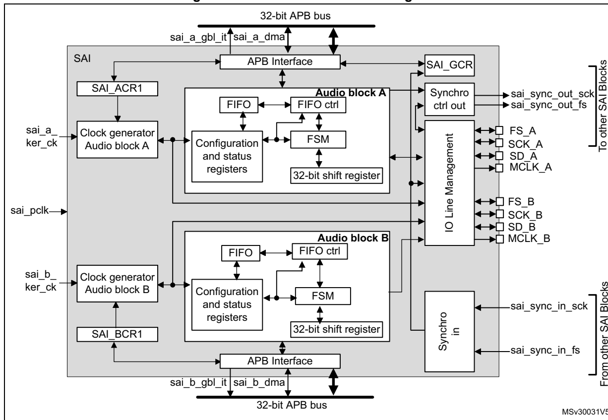
Figure 443. SAI functional block diagram
