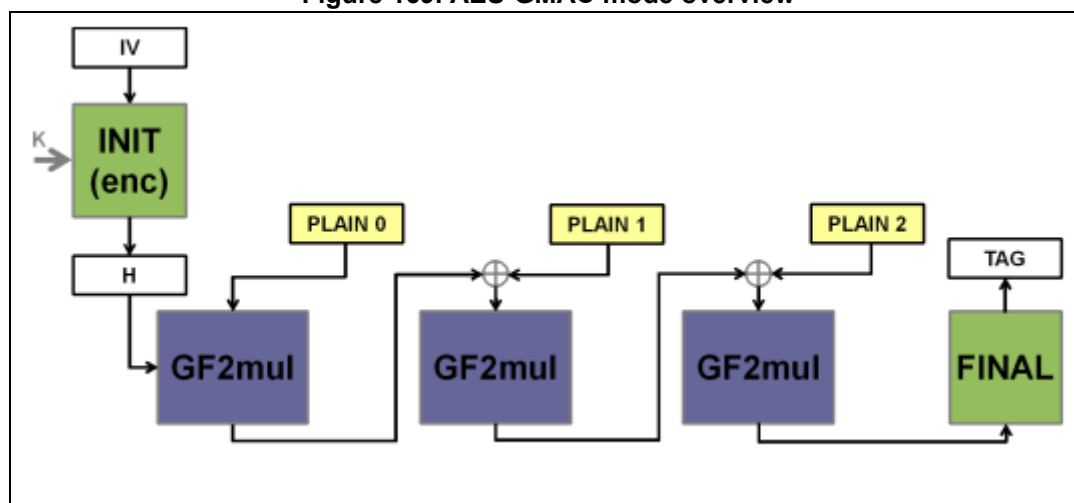
Figure 169. AES-GMAC mode overview
