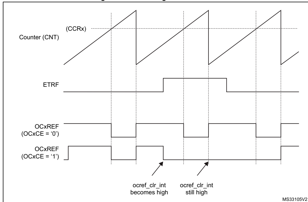
Figure 287. Clearing TIMx OCxREF
