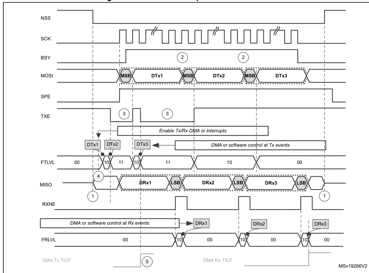
Figure 415. Master full-duplex communication
