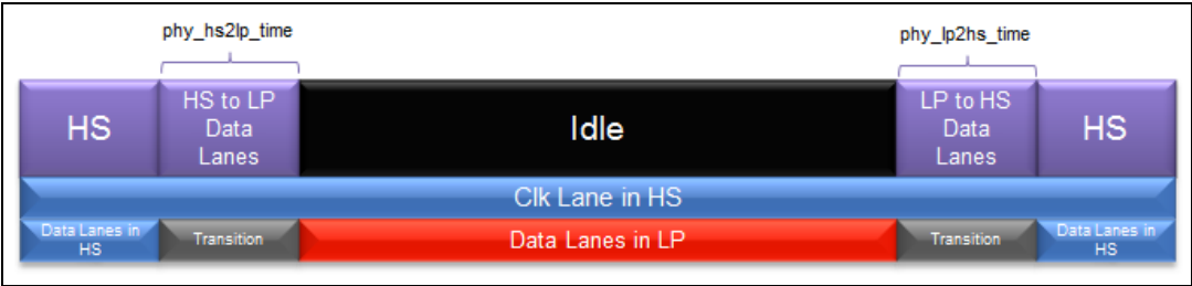
Figure 148. Clock lane in HS and data lanes in LP
