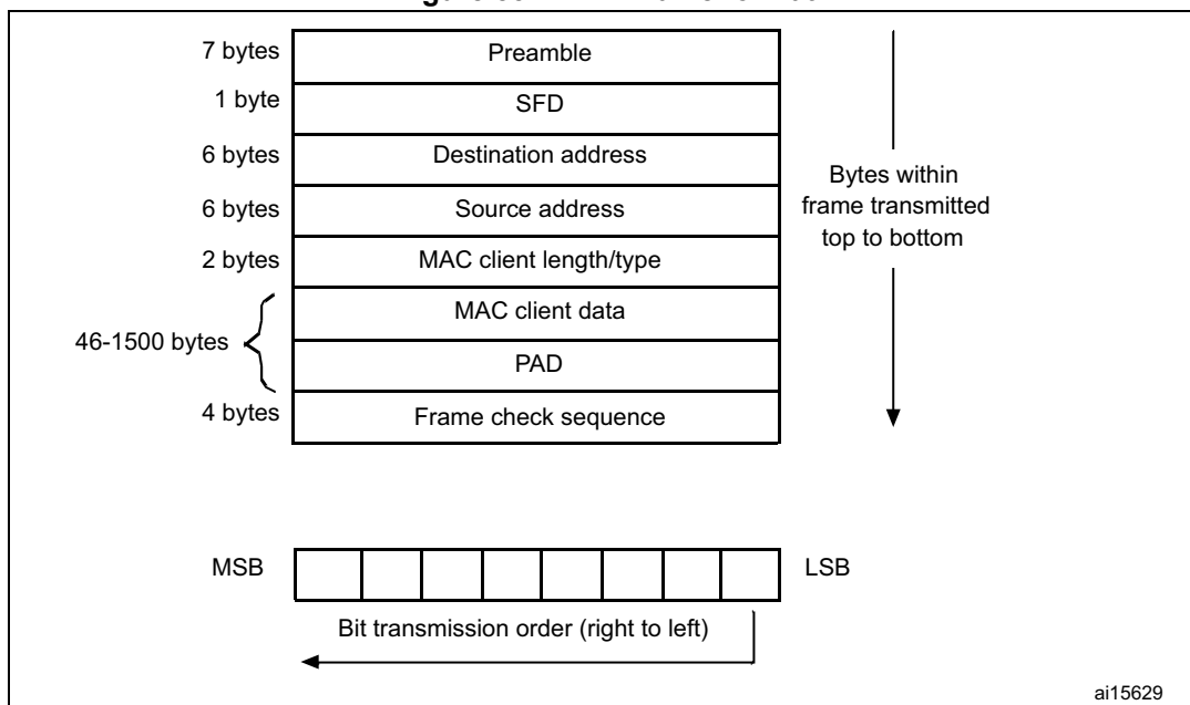
Figure 551. MAC frame format
