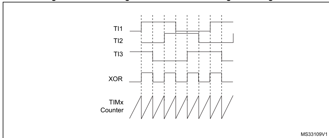
Figure 247. Measuring time interval between edges on 3 signals
