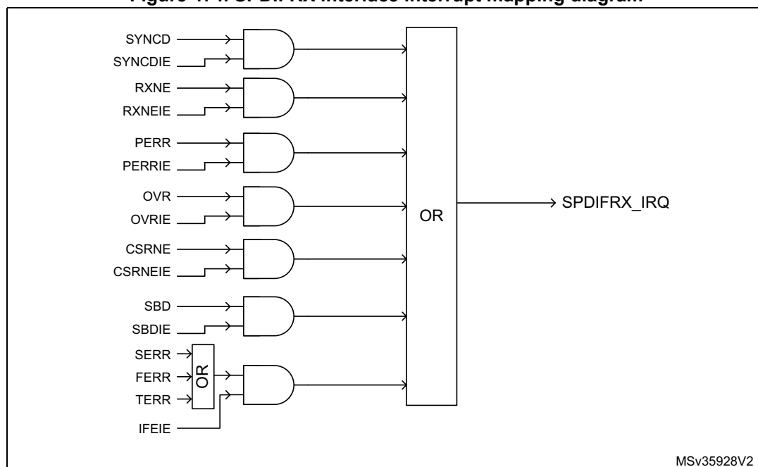
Figure 474. SPDIFRX interface interrupt mapping diagram
