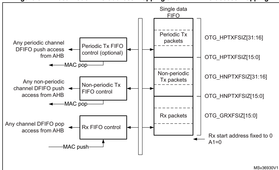
Figure 517. Host-mode FIFO address mapping and AHB FIFO access mapping
