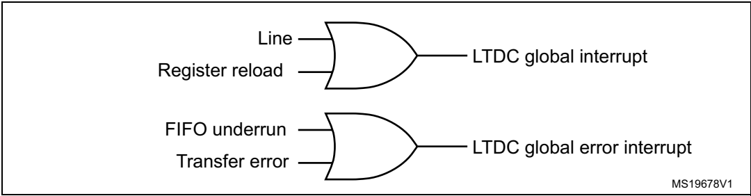
Figure 123. Interrupt events
