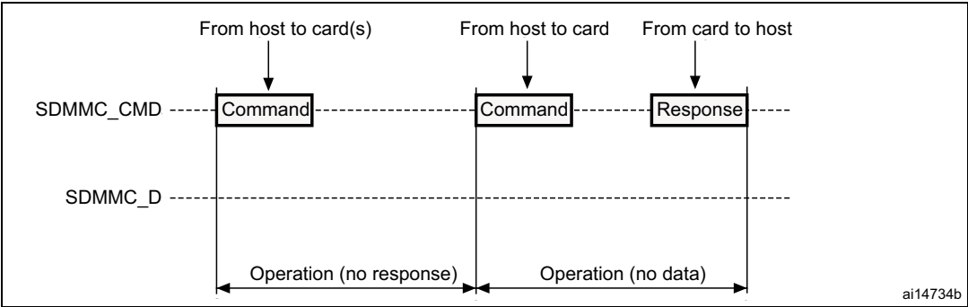
Figure 478. “No response” and “no data” operations
