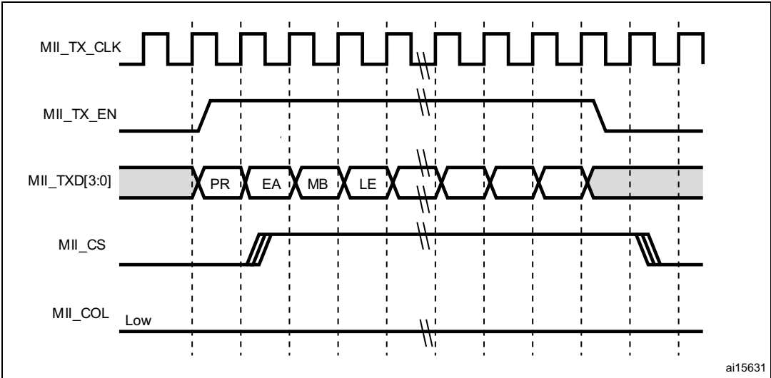
Figure 554. Transmission with no collision
