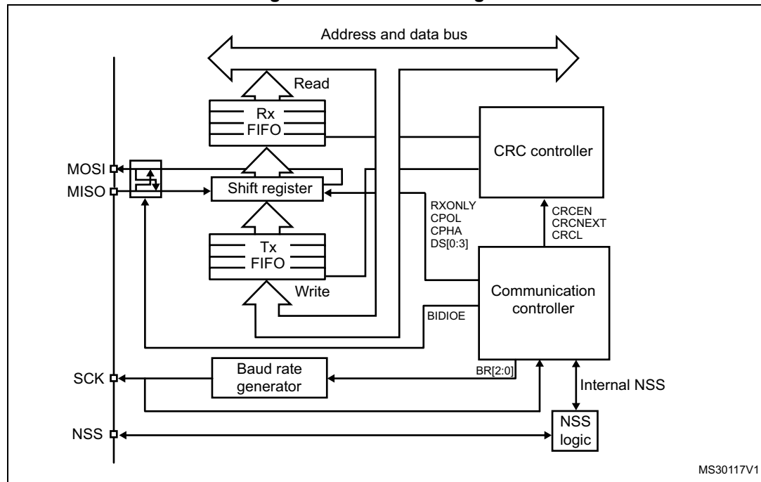
Figure 405. SPI block diagram
