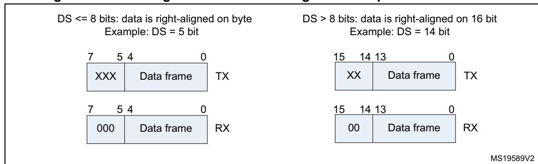
Figure 413. Data alignment when data length is not equal to 8-bit or 16-bit
