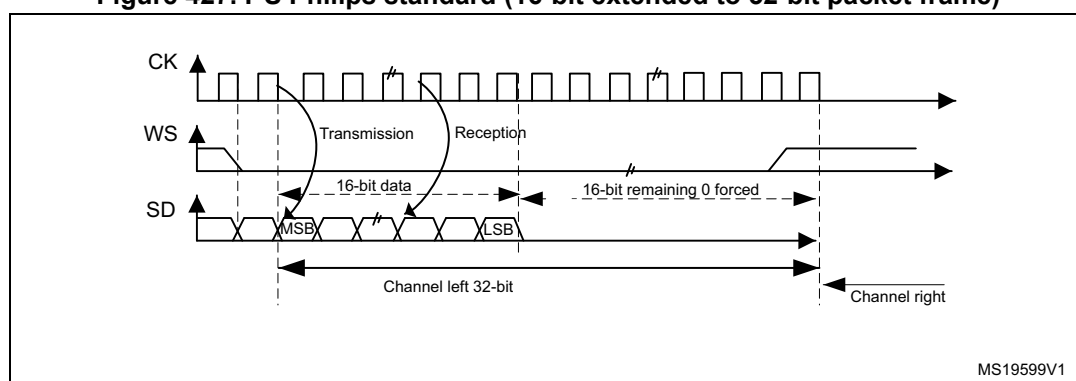
Figure 427. I 2 S Philips standard (16-bit extended to 32-bit packet frame)
