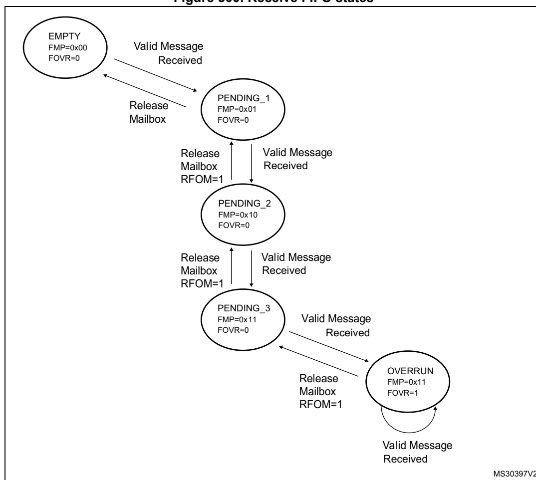
Figure 500. Receive FIFO states
