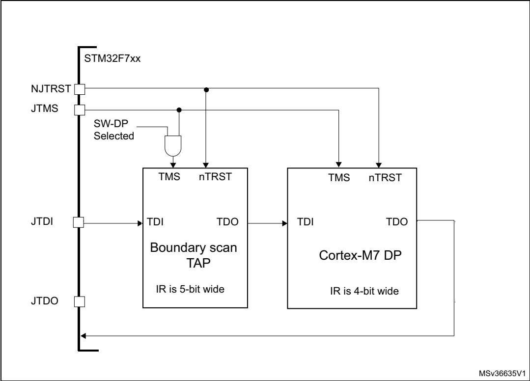
Figure 589. JTAG Debug Port connections
