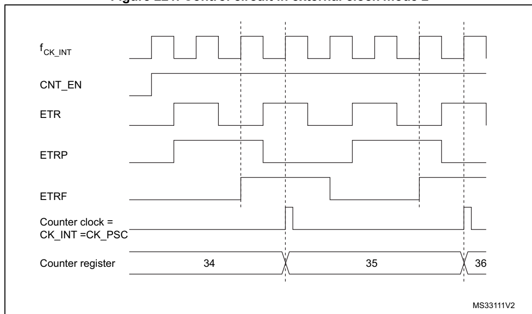
Figure 221. Control circuit in external clock mode 2
