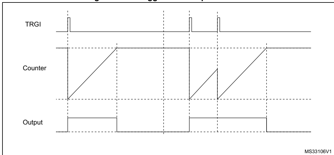
Figure 289 Retriggerable one pulse mode
