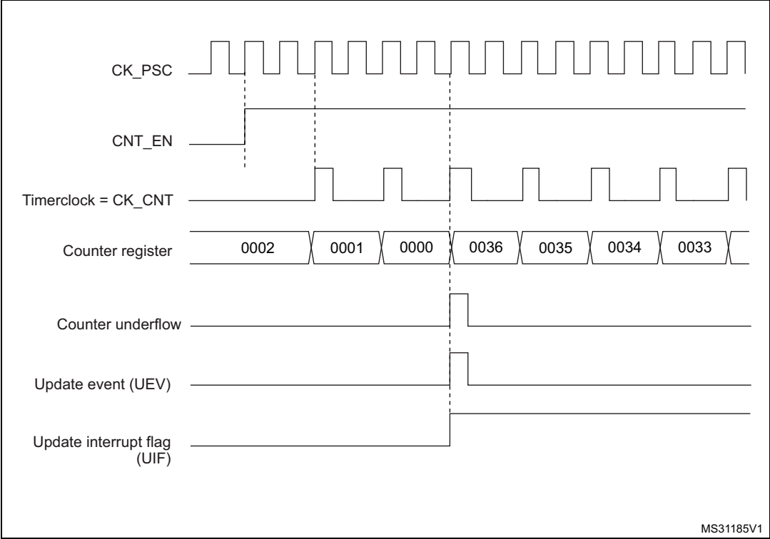
Figure 263. Counter timing diagram, internal clock divided by 2
