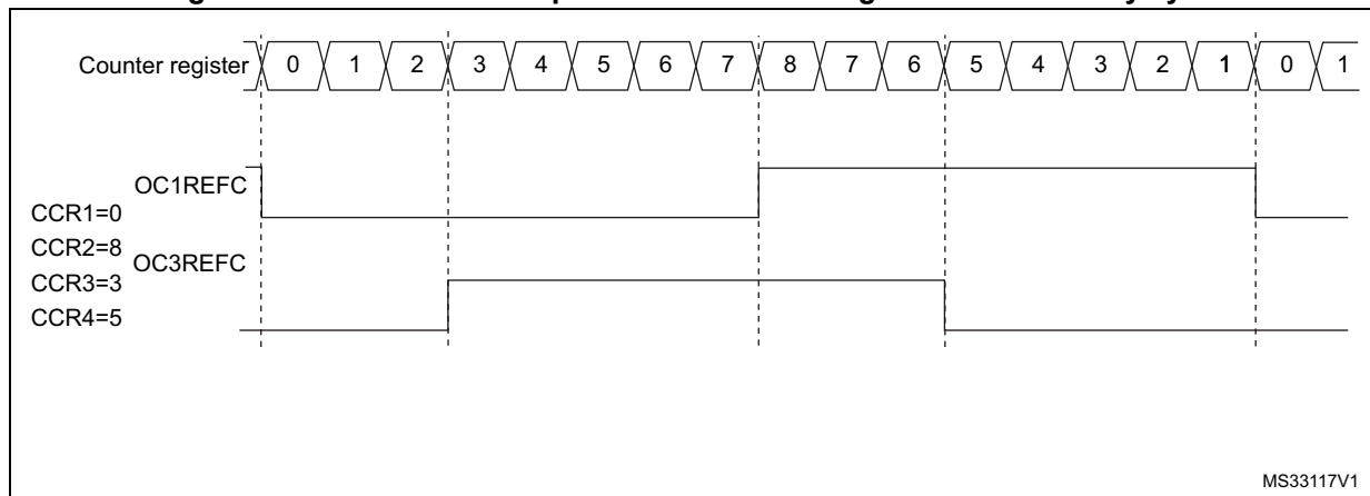
Figure 231. Generation of 2 phase-shifted PWM signals with 50% duty cycle
