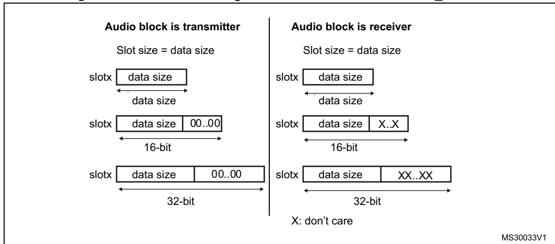
Figure 447. Slot size configuration with FBOFF = 0 in SAI_xSLOTR
