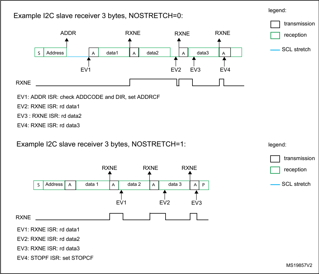
Figure 361. Transfer bus diagrams for I2C slave receiver
