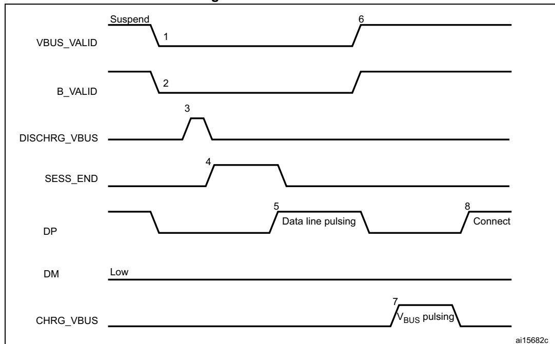
Figure 538. B-device SRP
