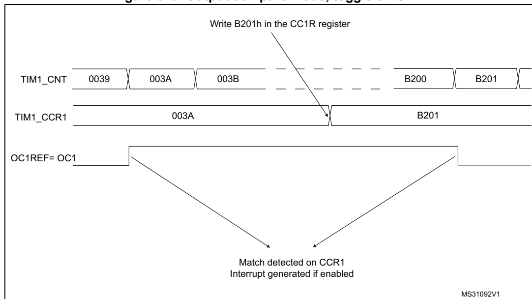
Figure 319. Output compare mode, toggle on OC1.
