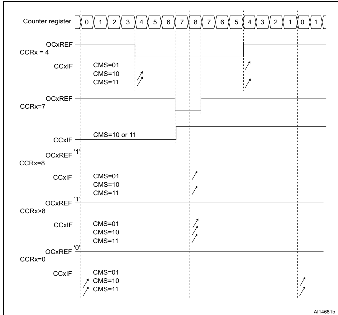
Figure 230. Center-aligned PWM waveforms (ARR=8)
