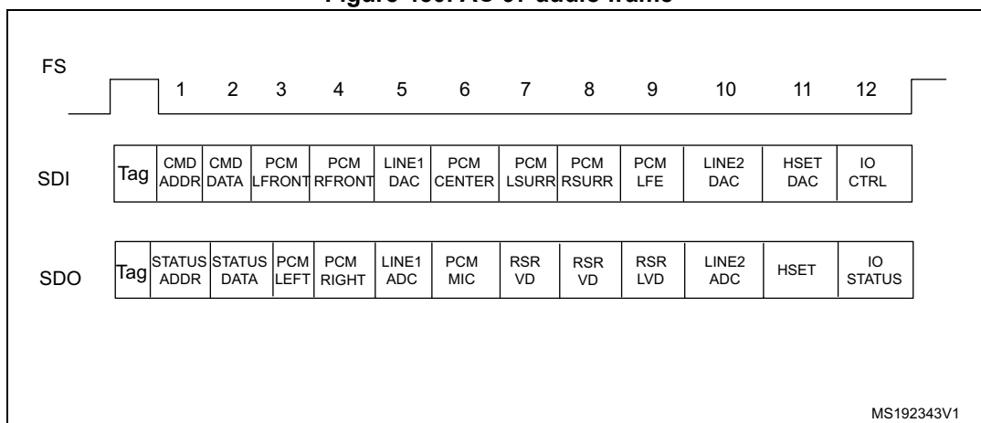
Figure 450. AC'97 audio frame
