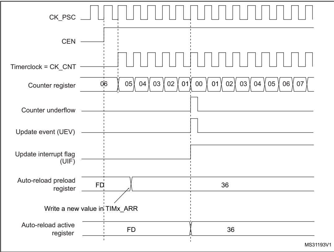
Figure 213. Counter timing diagram, update event with ARPE=1 (counter underflow)
