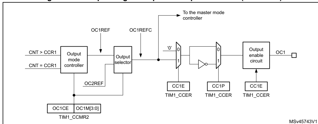
Figure 317. Output stage of capture/compare channel (channel 1)
