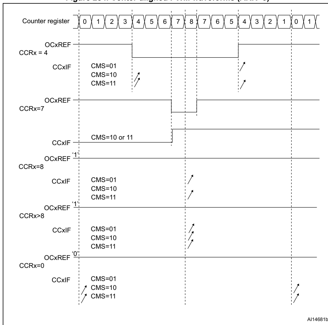
Figure 284. Center-aligned PWM waveforms (ARR=8)
