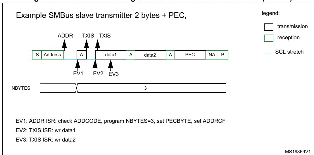
Figure 374. Transfer bus diagrams for SMBus slave transmitter (SBC=1)
