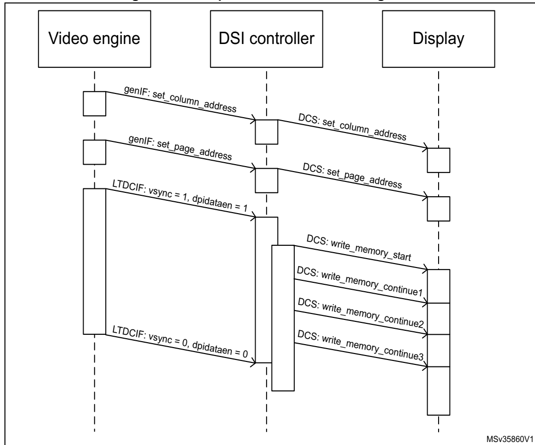
Figure 129. Adapted command mode usage flow
