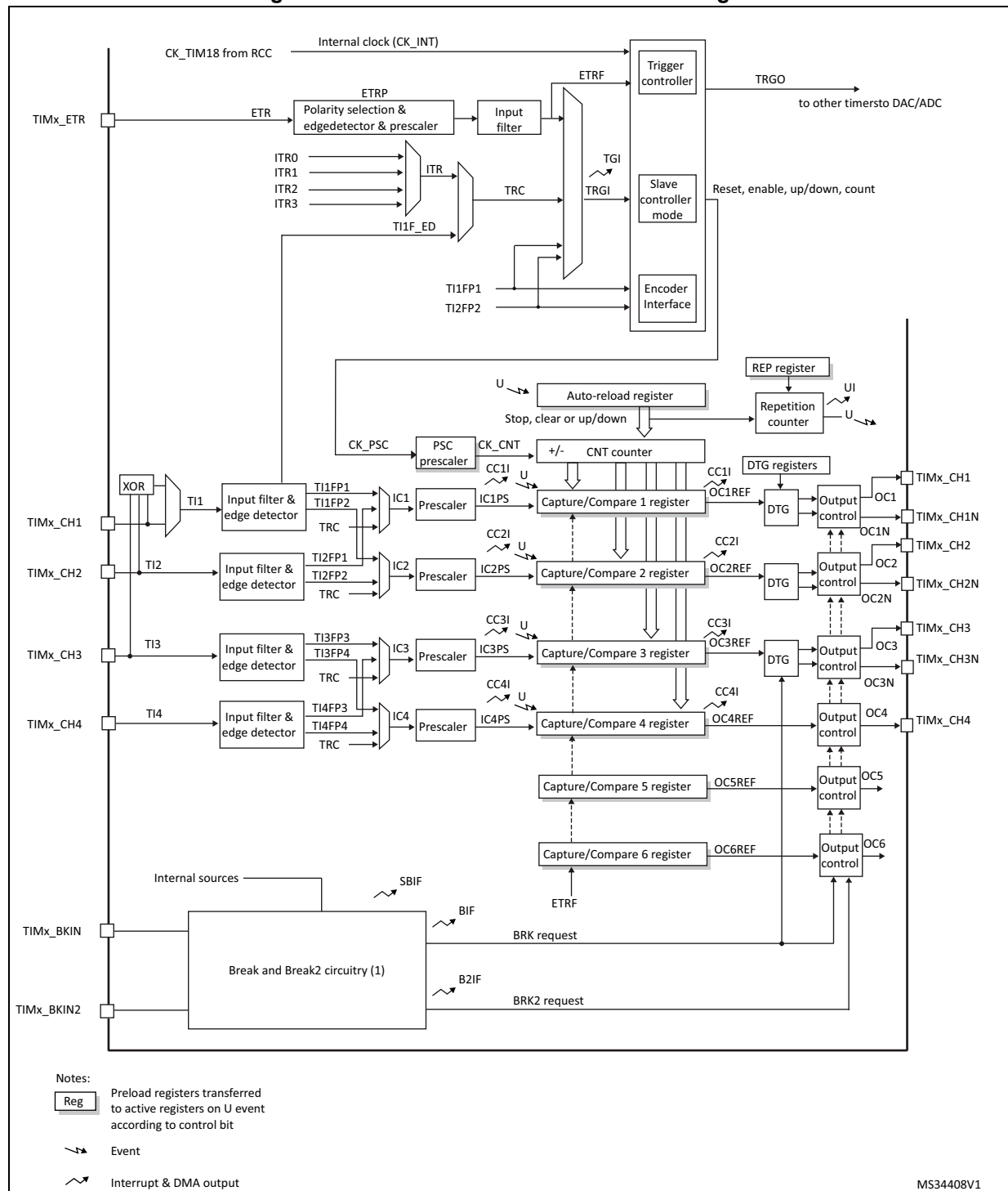
Figure 195. Advanced-control timer block diagram
