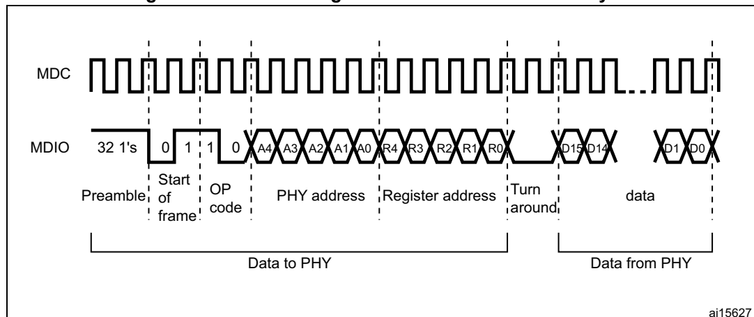
Figure 544. MDIO timing and frame structure - Read cycle
