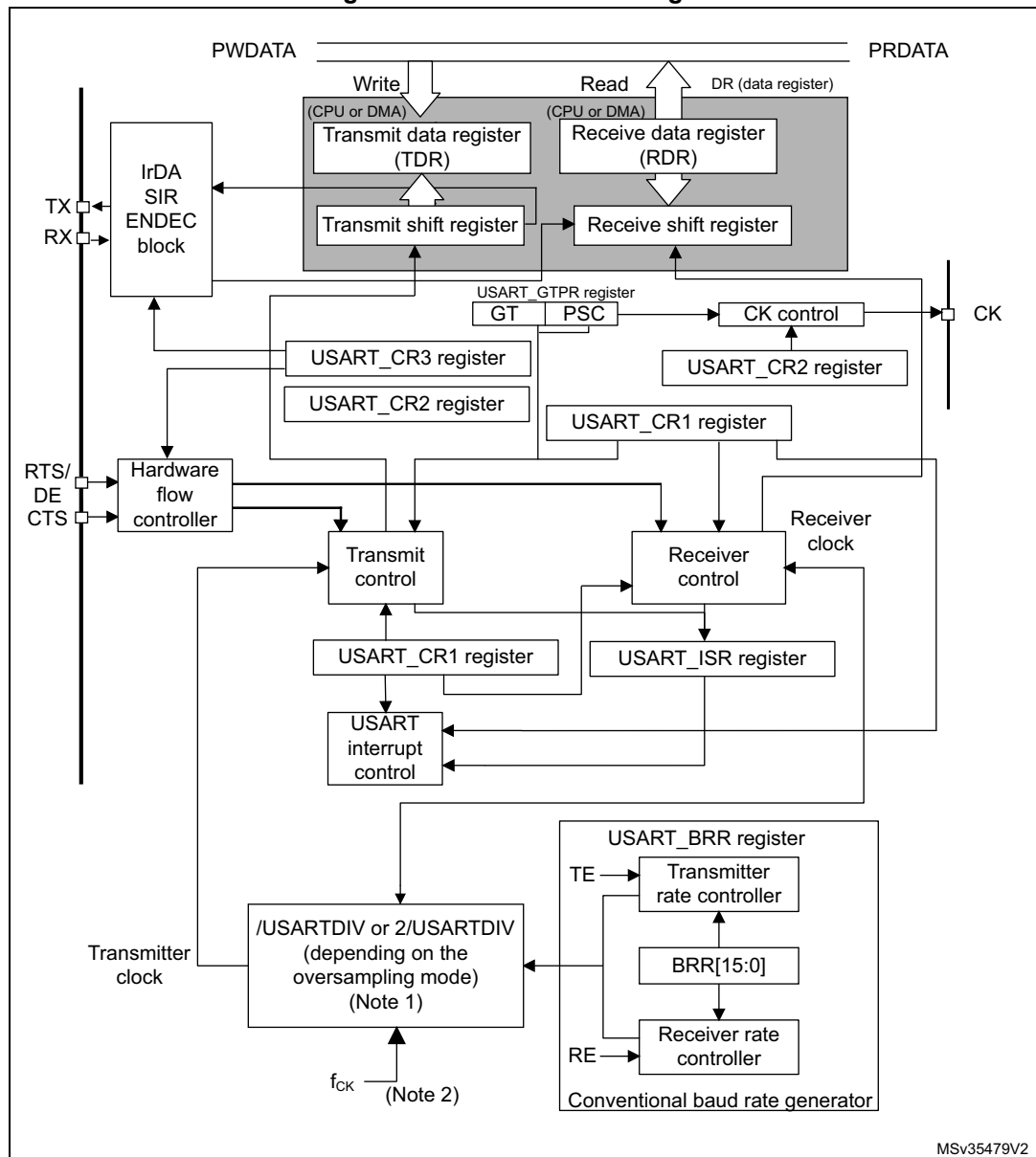
Figure 380. USART block diagram
