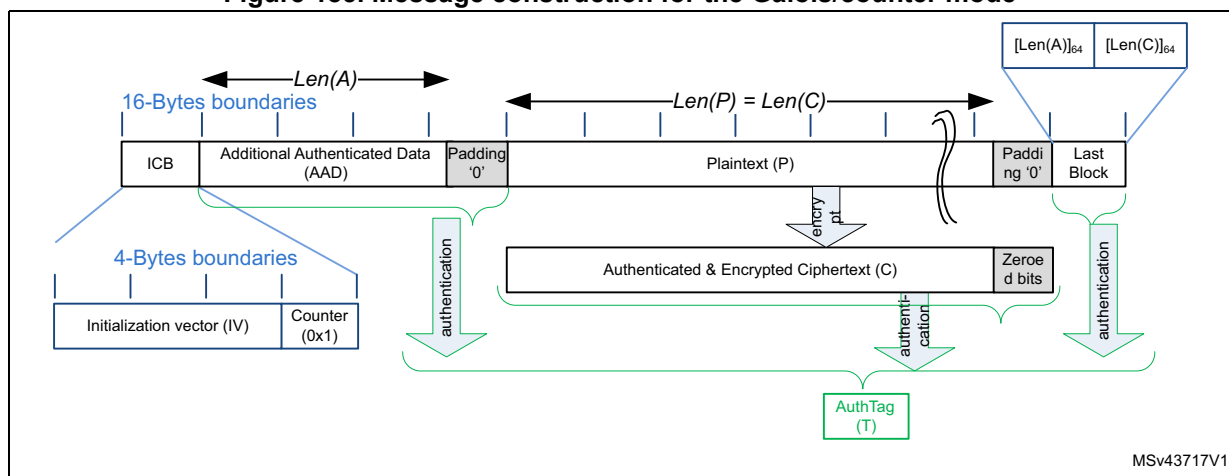
Figure 185. Message construction for the Galois/counter mode
