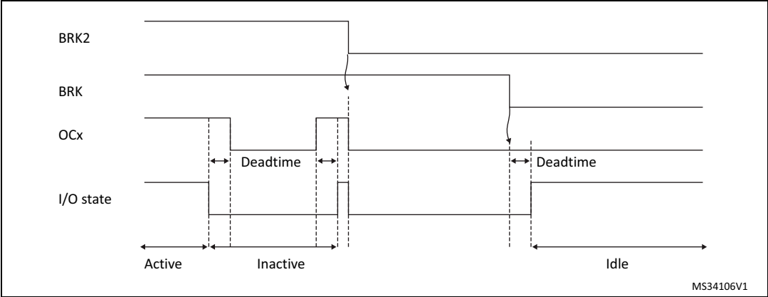
Figure 239. PWM output state following BRK and BRK2 pins assertion (OSSl=1)
