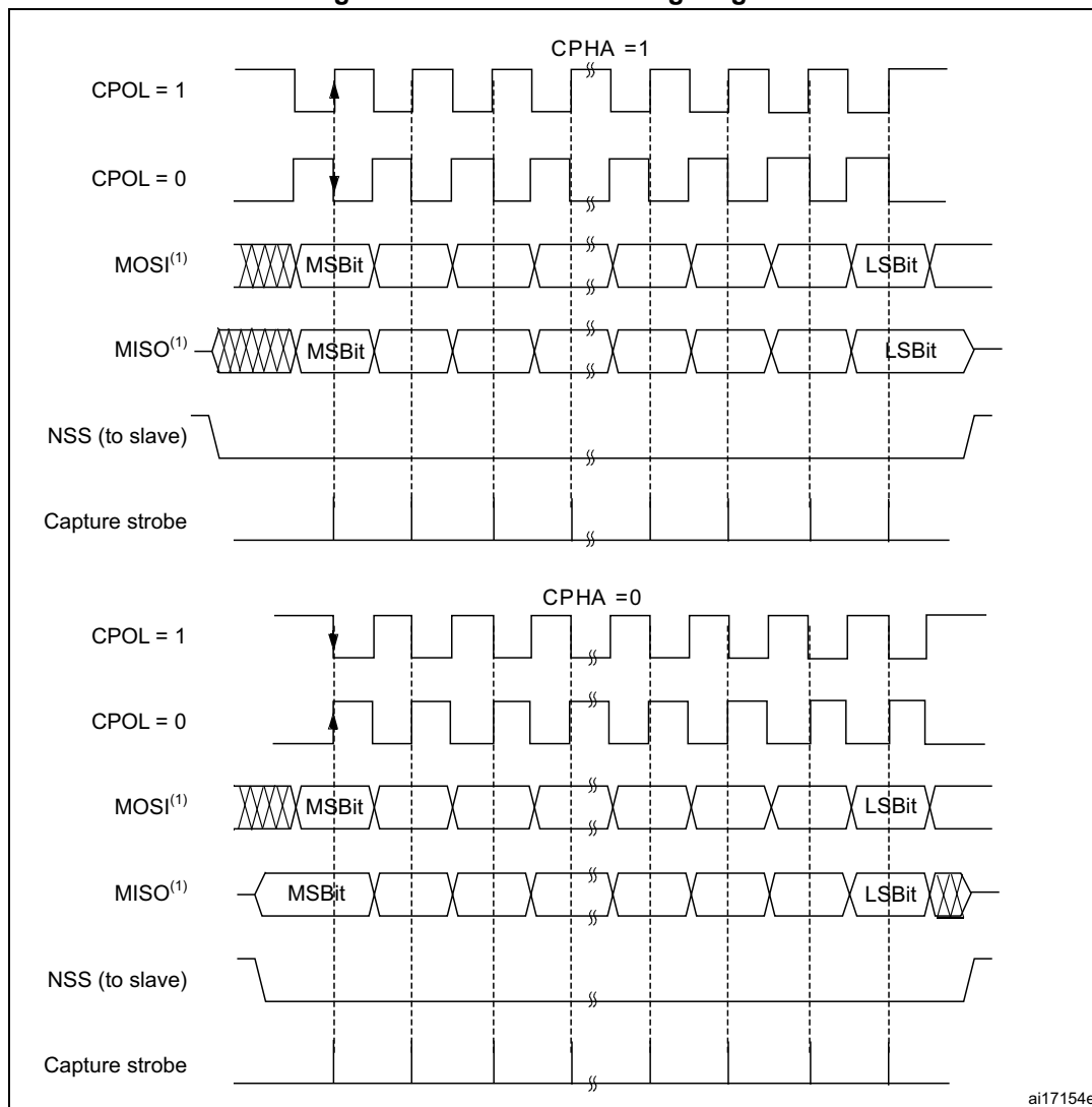
Figure 412. Data clock timing diagram
