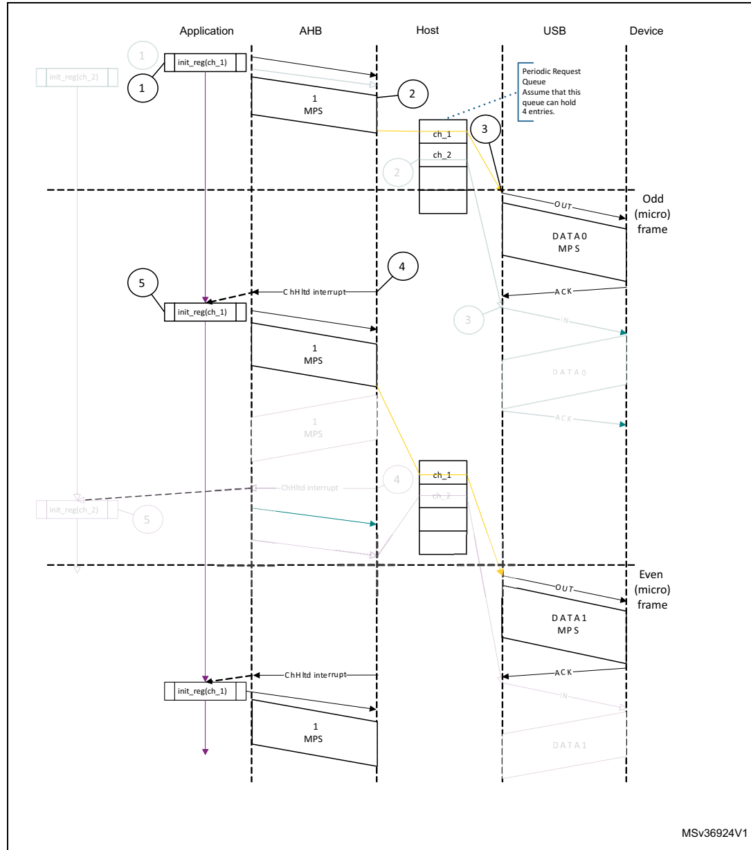
Figure 529. Normal interrupt OUT transactions - DMA mode
