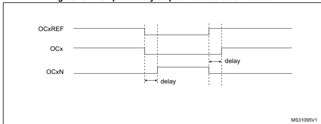
Figure 234. Complementary output with dead-time insertion
