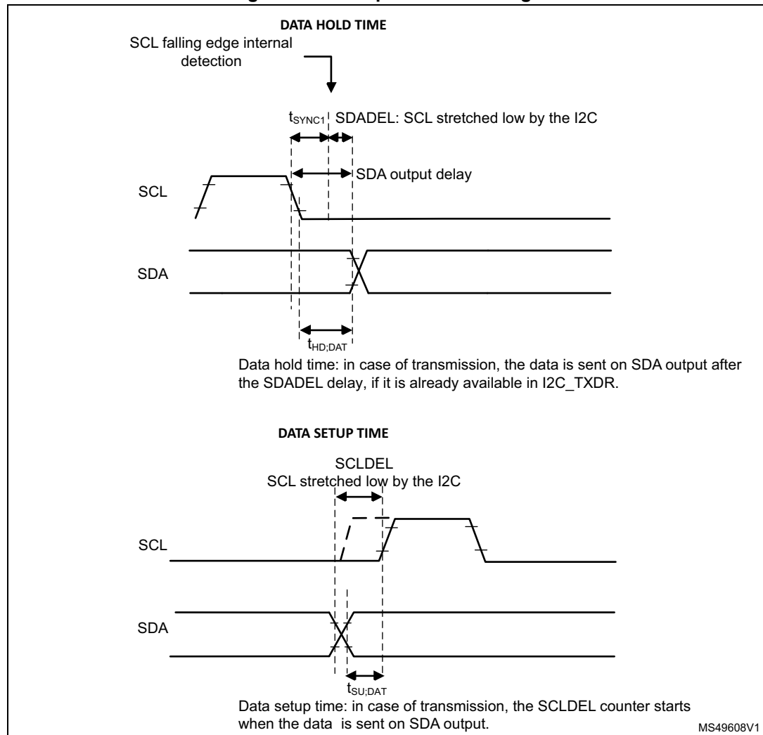
Figure 351. Setup and hold timings
