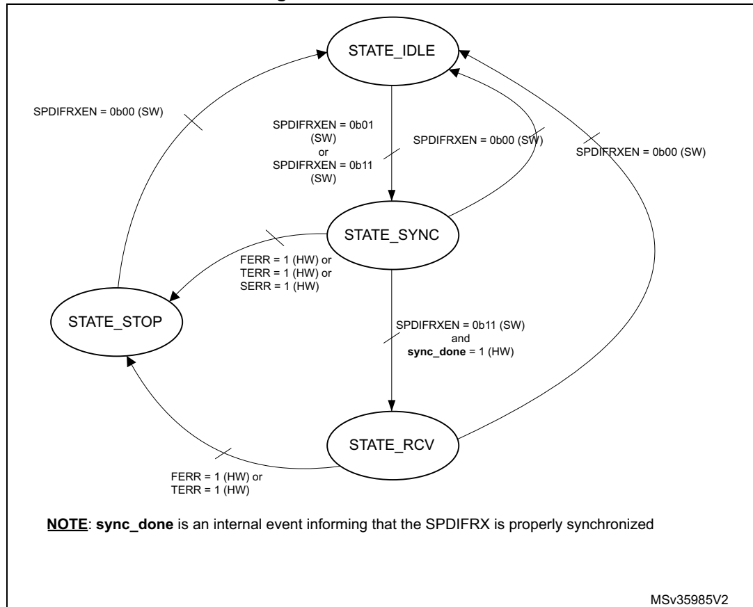
Figure 469. SPDIFRX States
