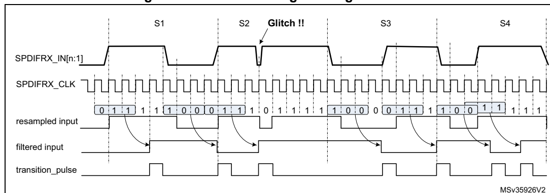
Figure 465. Noise filtering and edge detection
