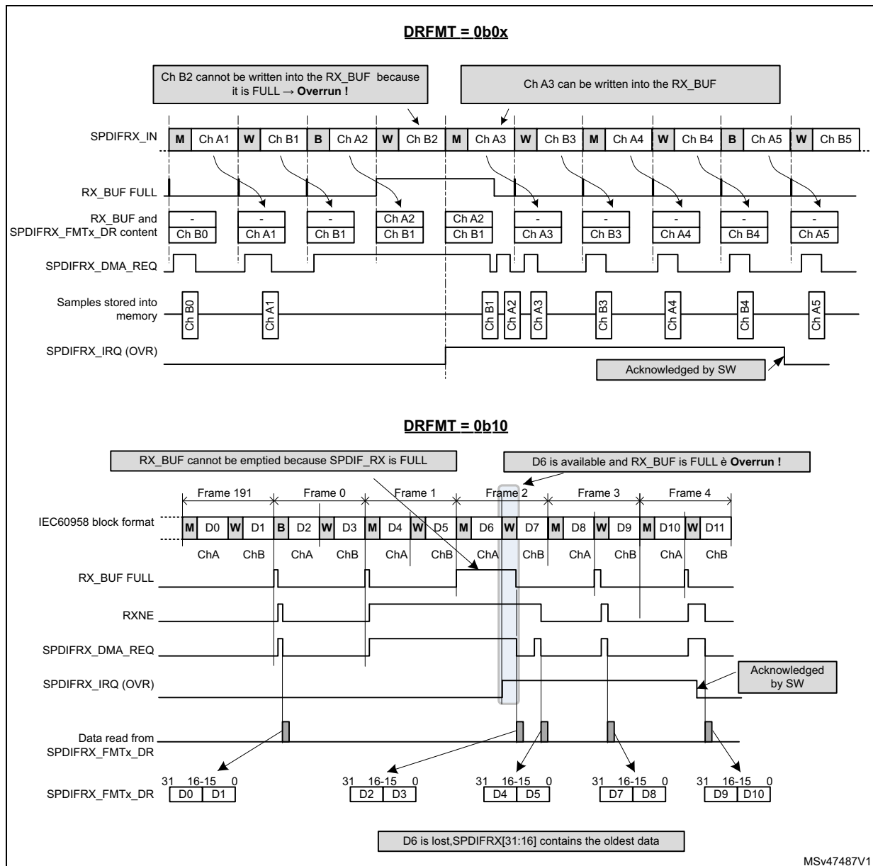
Figure 472. S/PDIF overrun error when RXSTEO = 0
