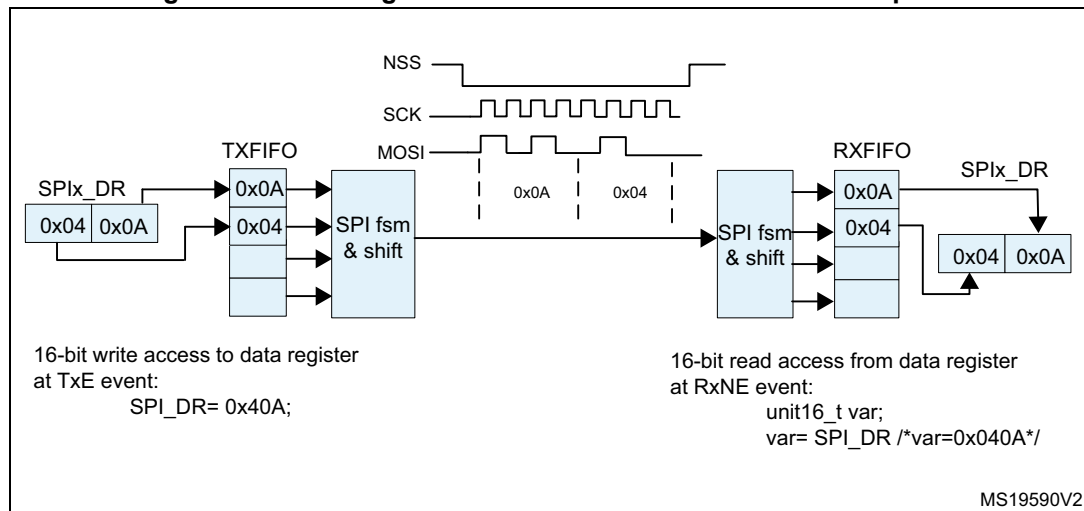
Figure 414. Packing data in FIFO for transmission and reception
