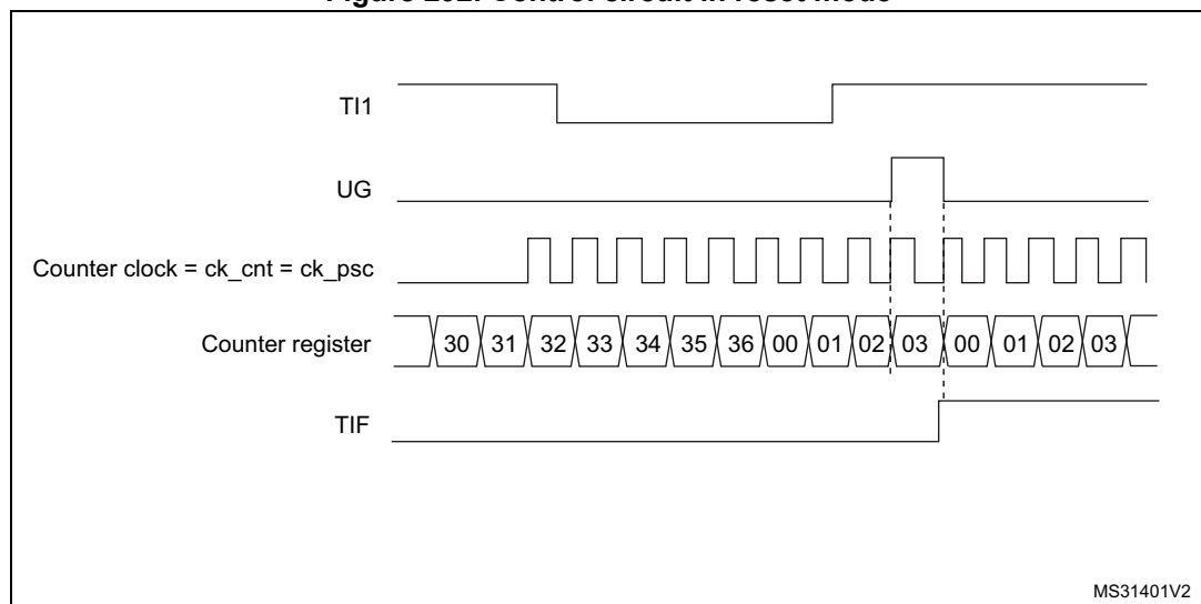
Figure 292. Control circuit in reset mode
