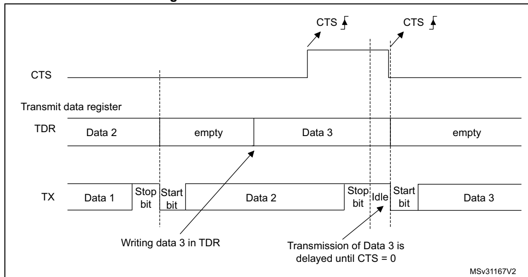
Figure 403. RS232 CTS flow control
