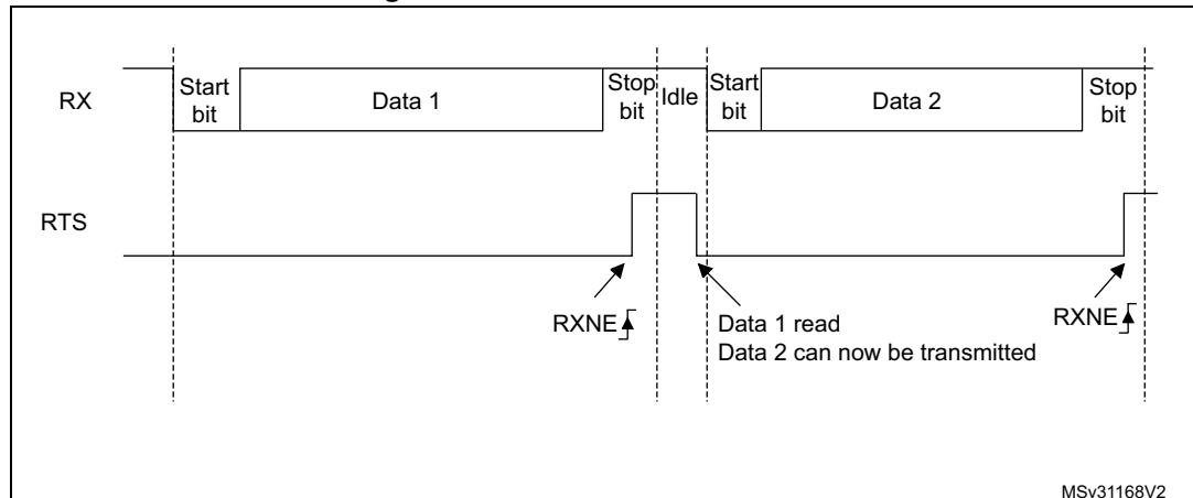
Figure 402. RS232 RTS flow control
