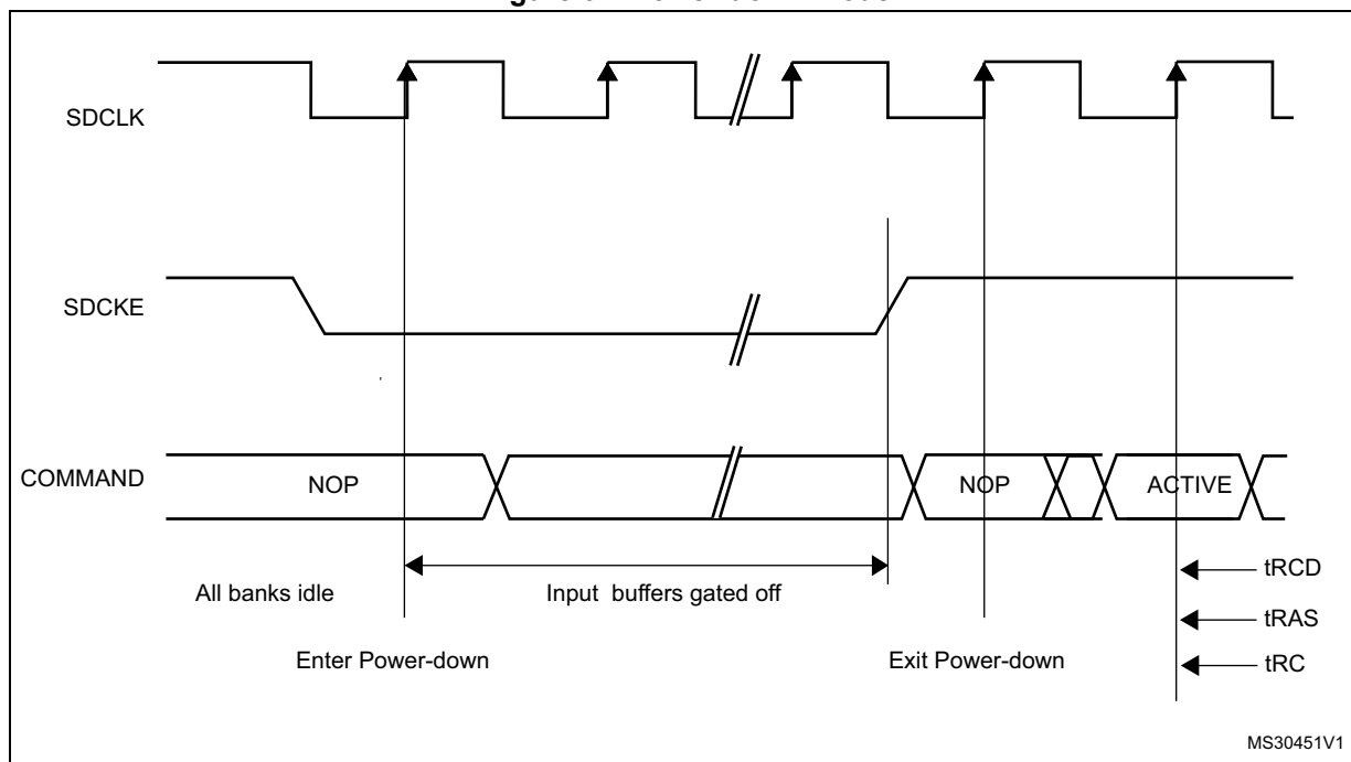
Figure 61. Power-down mode
