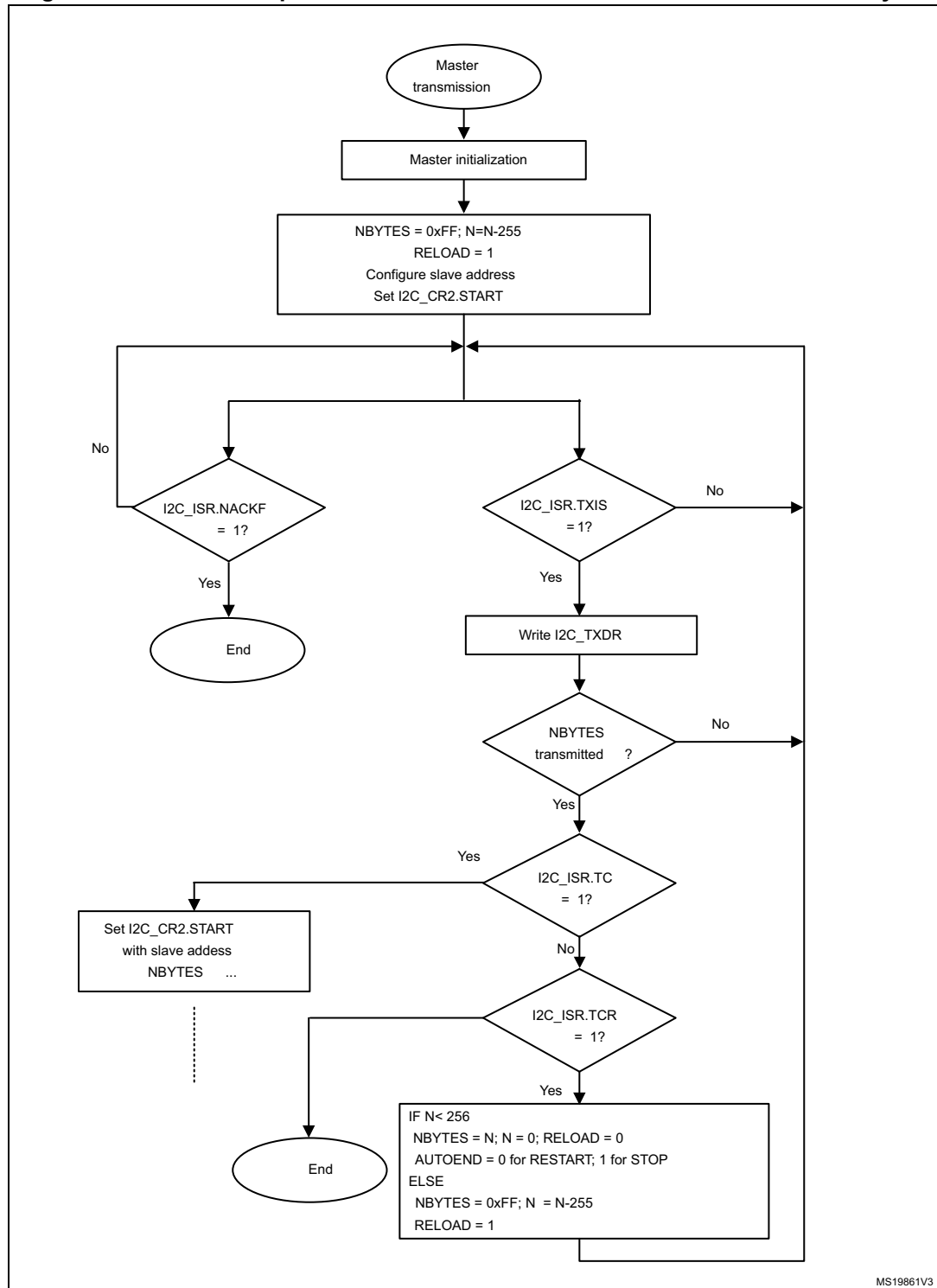
Figure 367. Transfer sequence flowchart for I2C master transmitter for N&gt;255 bytes
