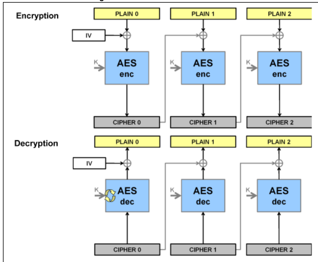
Figure 166. AES-CBC mode overview
