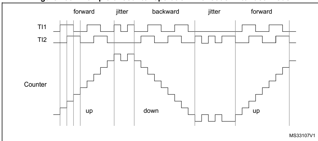
Figure 290. Example of counter operation in encoder interface mode
