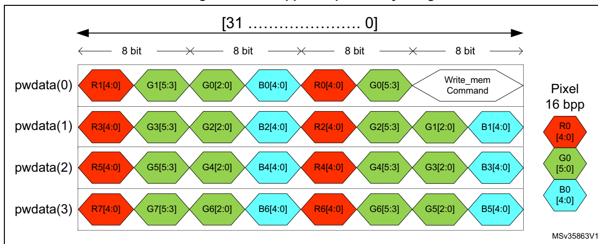
Figure 132. 16 bpp APB pixel to byte organization
