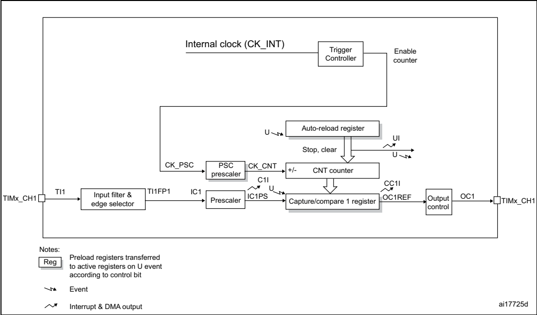
Figure 303. General-purpose timer block diagram (TIM10/TIM11/TIM13/TIM14)
