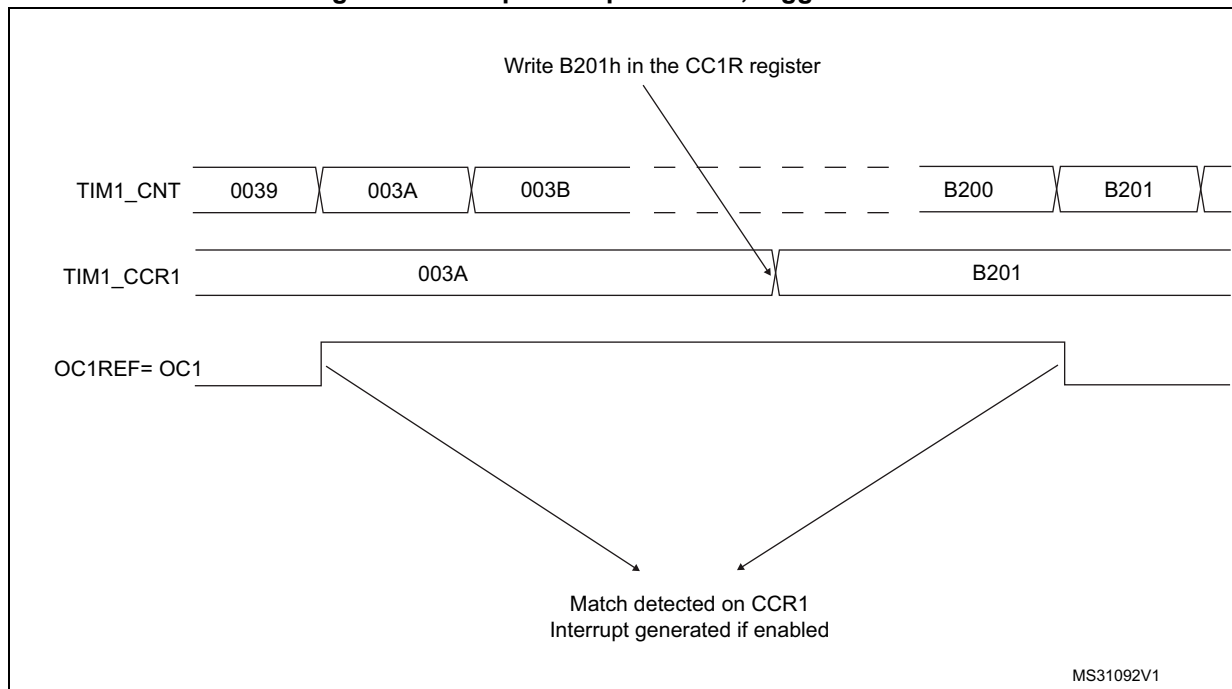
Figure 282. Output compare mode, toggle on OC1
