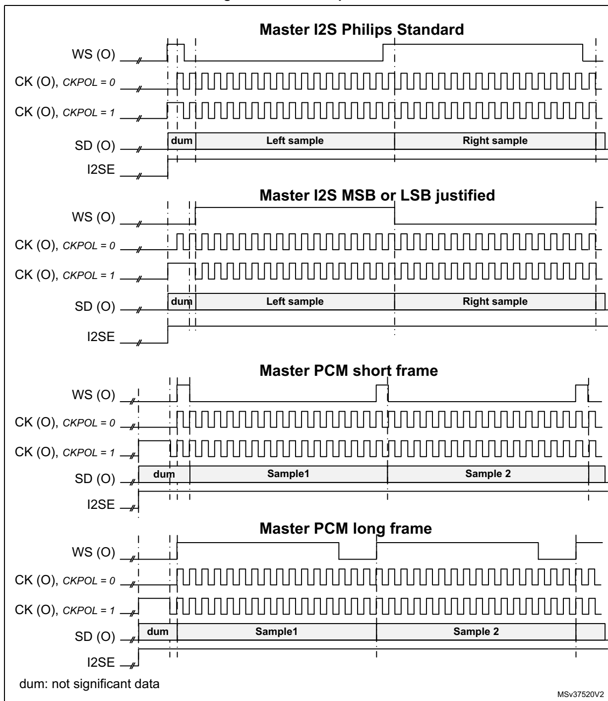
Figure 440. Start sequence in master mode
