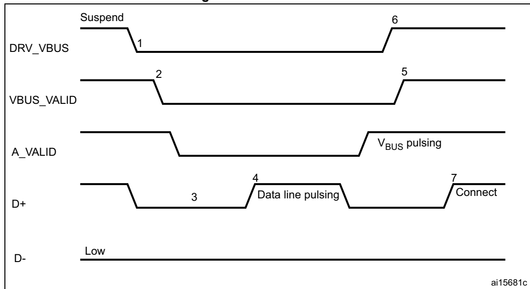
Figure 537. A-device SRP
