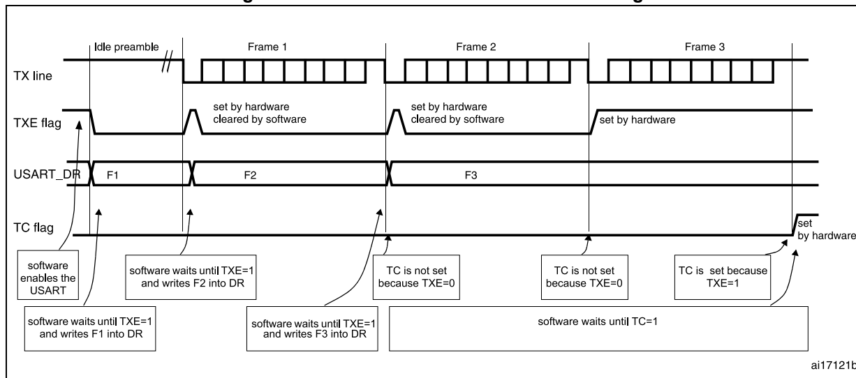
Figure 383. TC/TXE behavior when transmitting
