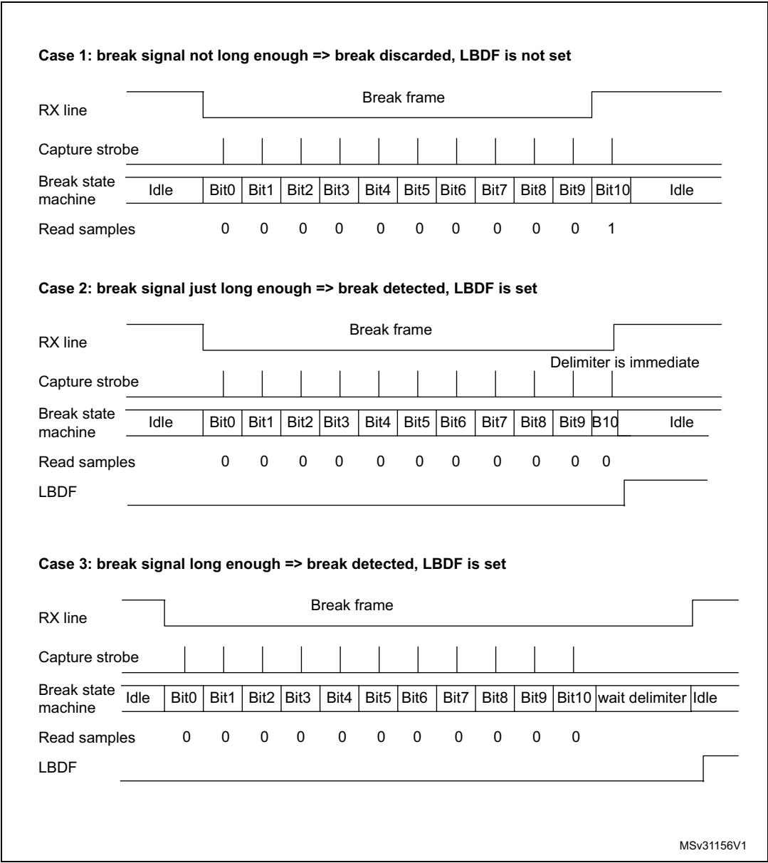
Figure 389. Break detection in LIN mode (11-bit break length - LBDL bit is set)
