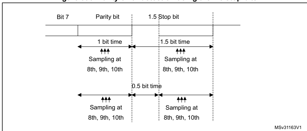
Figure 396. Parity error detection using the 1.5 stop bits
