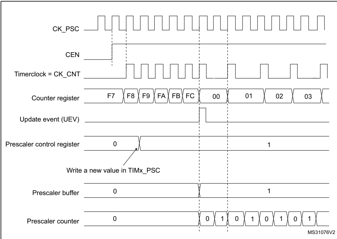
Figure 329. Counter timing diagram with prescaler division change from 1 to 2
