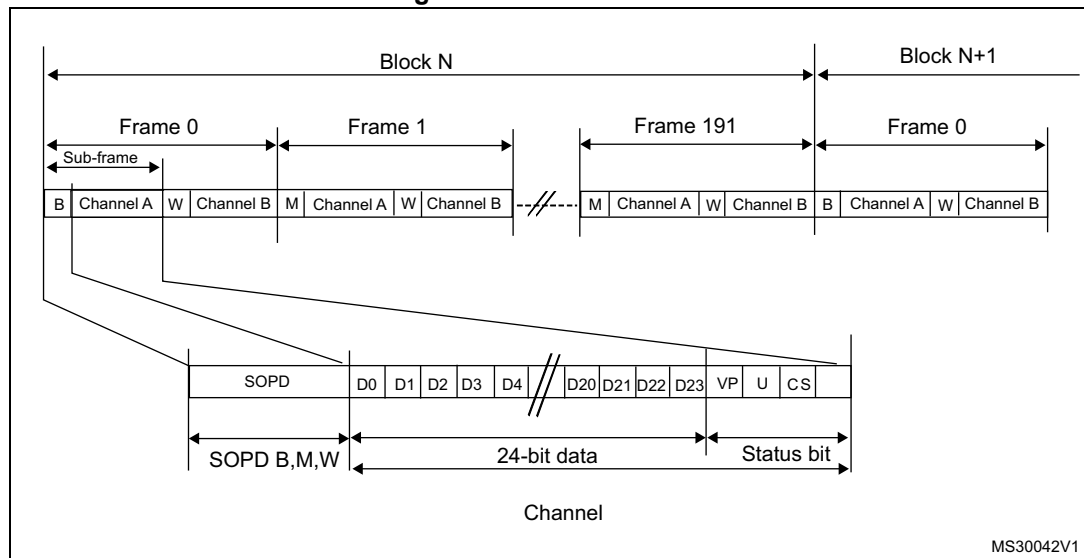
Figure 452. SPDIF format
