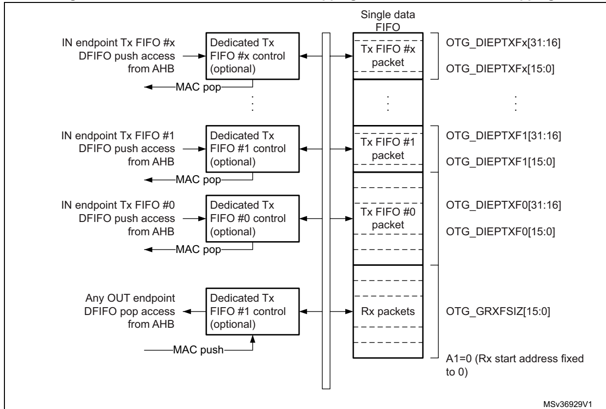
Figure 516. Device-mode FIFO address mapping and AHB FIFO access mapping
