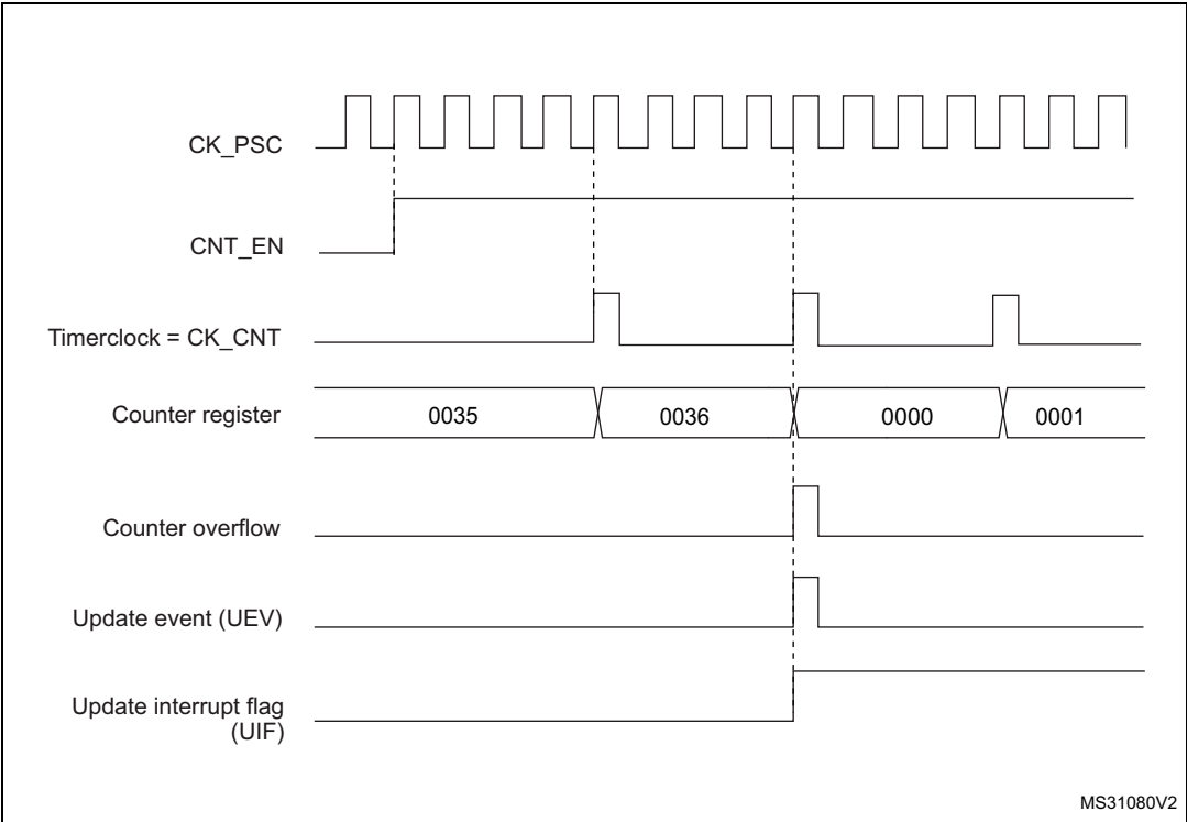
Figure 333. Counter timing diagram, internal clock divided by 4
