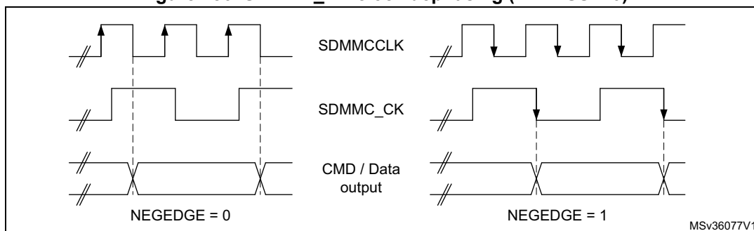
Figure 486. SDMMC_CLK clock dephasing (BYPASS = 0)
