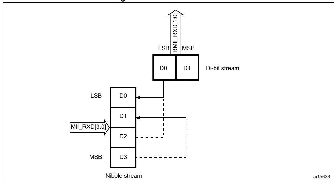
Figure 557. Receive bit order
