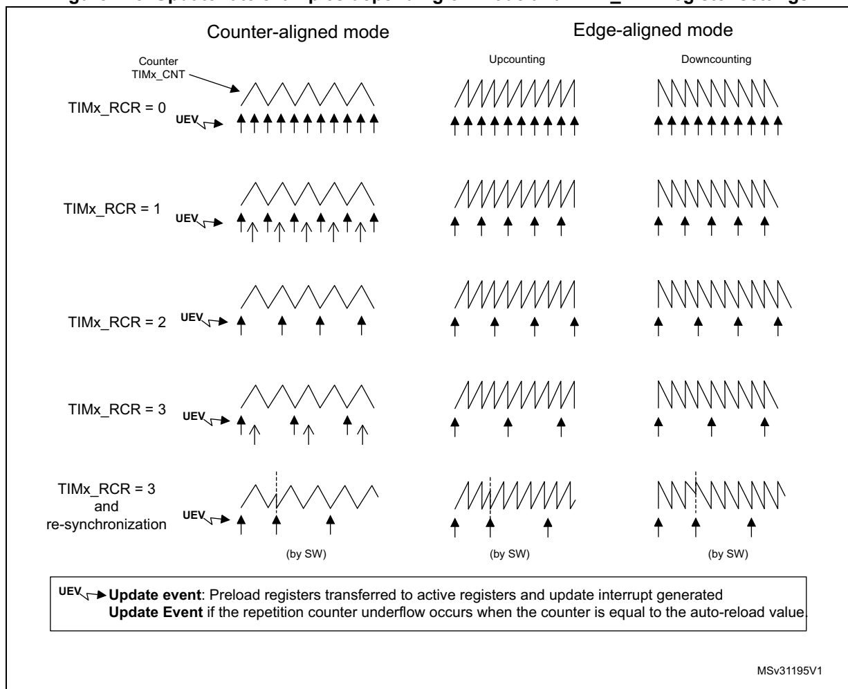
Figure 215. Update rate examples depending on mode and TIMx_RCR register settings
