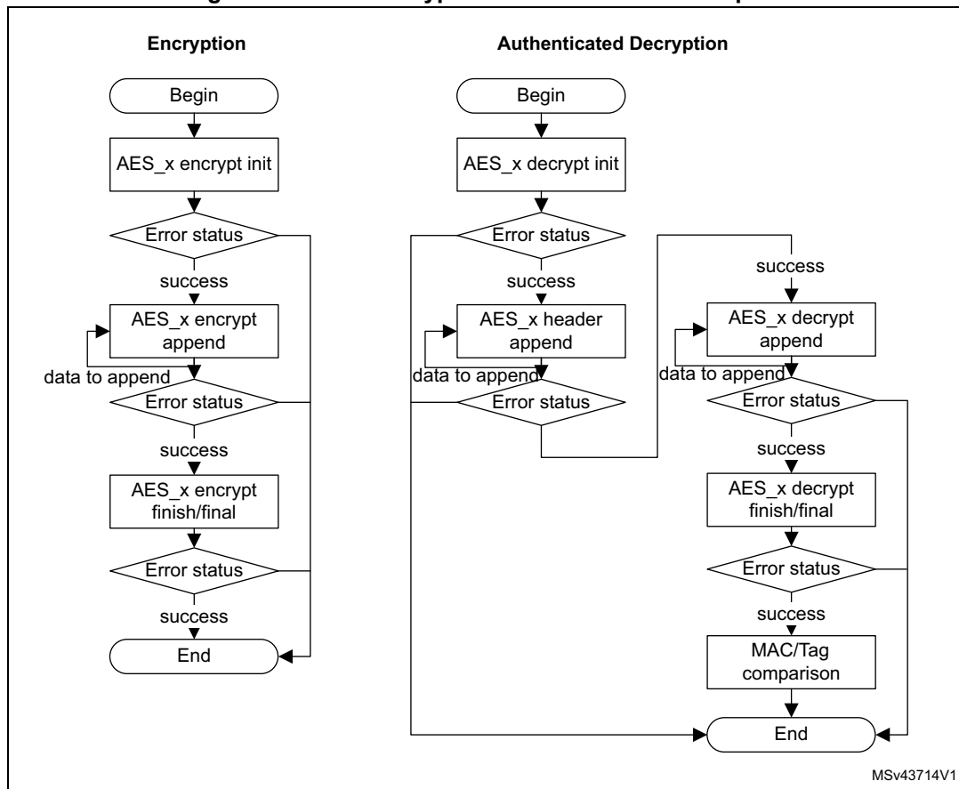
Figure 172. STM32 cryptolib AES flowchart examples
