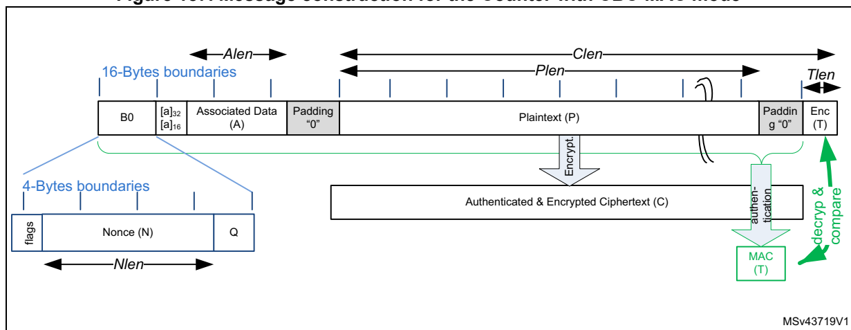
Figure 187. Message construction for the Counter with CBC-MAC mode
