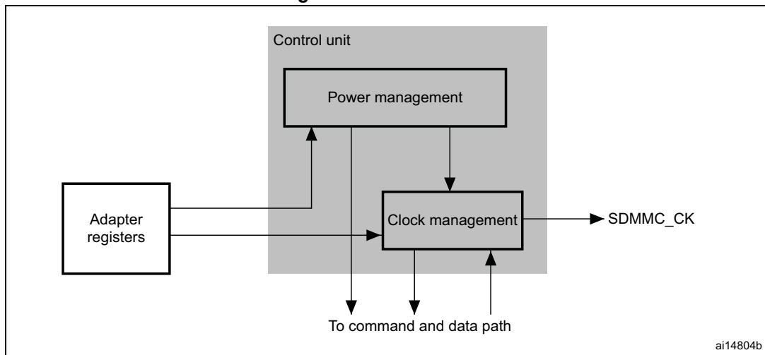
Figure 485. Control unit
