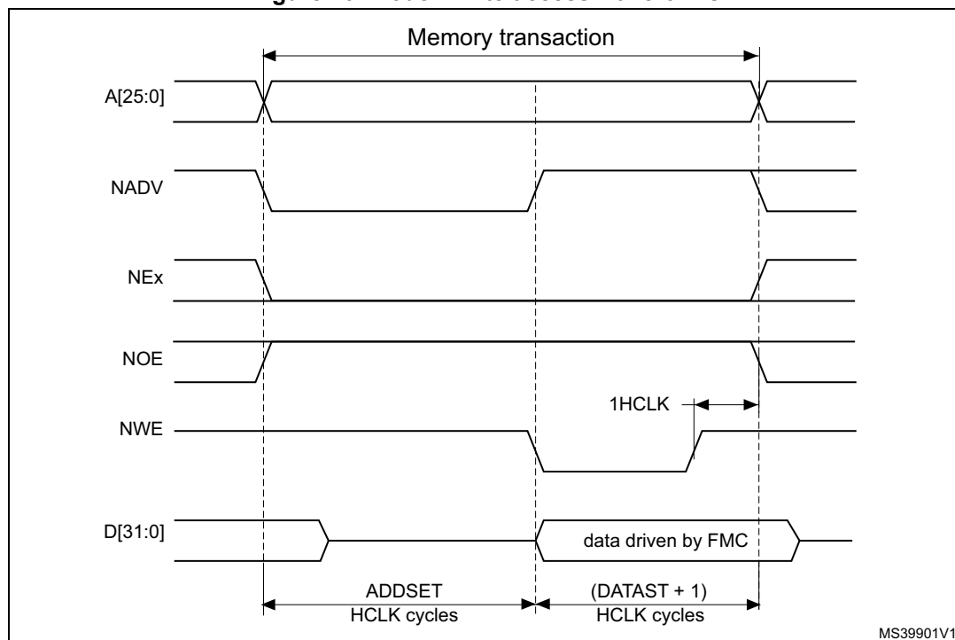
Figure 40. Mode2 write access waveforms
