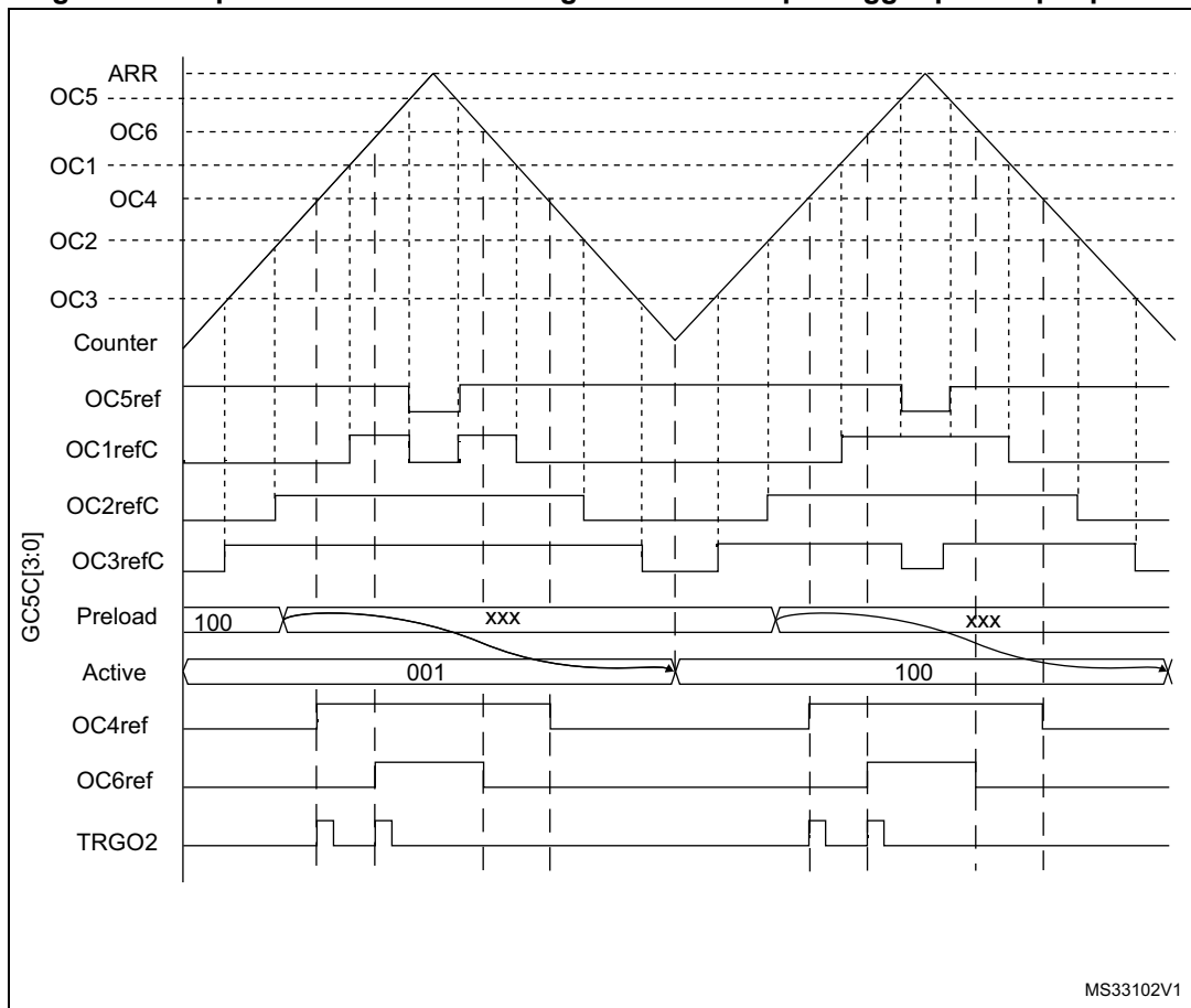
Figure 233. 3-phase combined PWM signals with multiple trigger pulses per period
