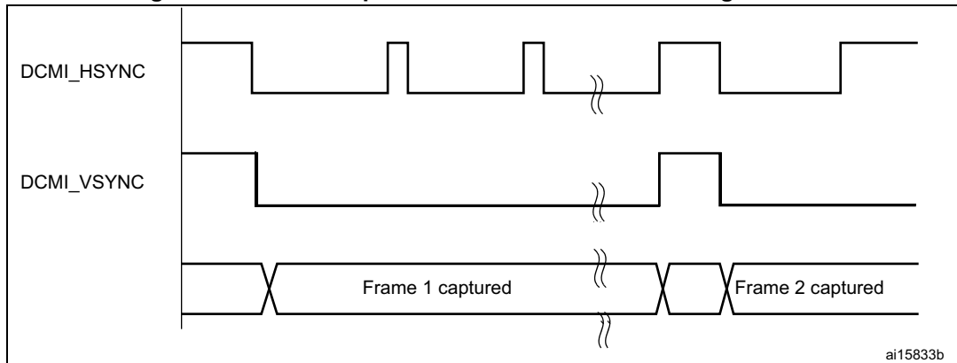
Figure 115. Frame capture waveforms in continuous grab mode
