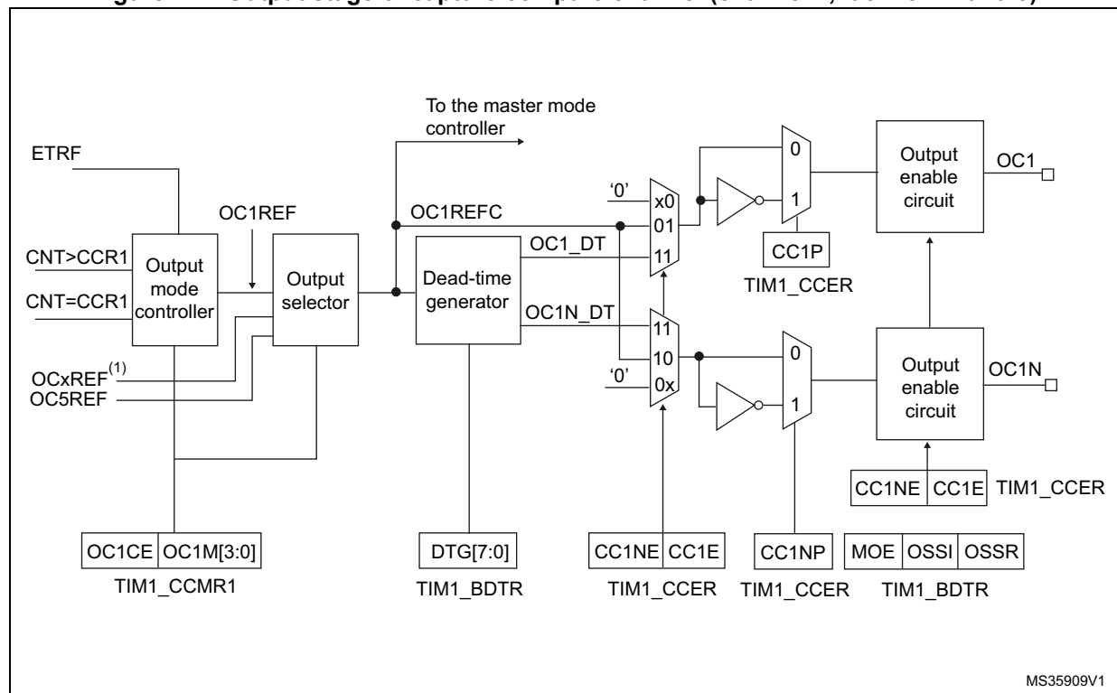
Figure 224. Output stage of capture/compare channel (channel 1, idem ch. 2 and 3)
