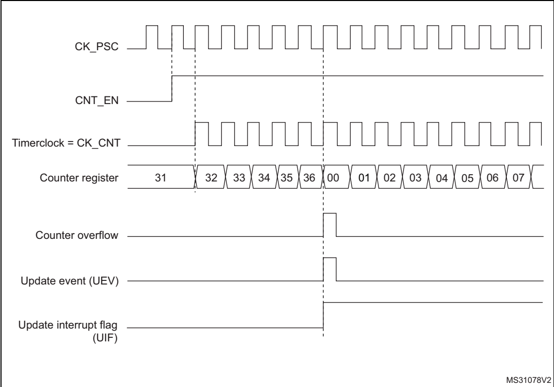
Figure 198. Counter timing diagram, internal clock divided by 1
