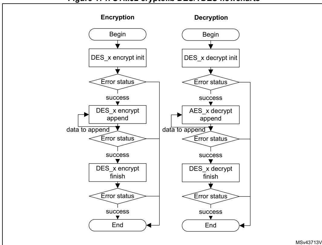
Figure 171. STM32 cryptolib DES/TDES flowcharts
