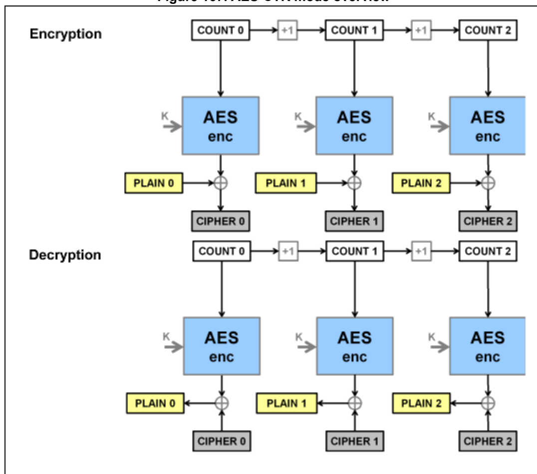
Figure 167. AES-CTR mode overview
