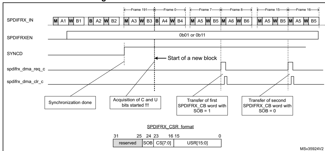
Figure 471. Channel/user data format
