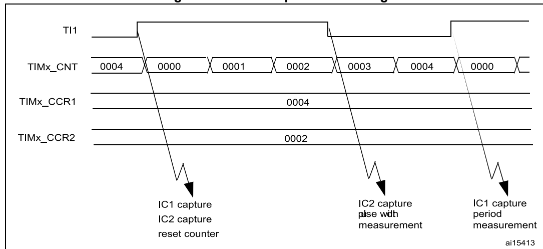
Figure 227. PWM input mode timing
