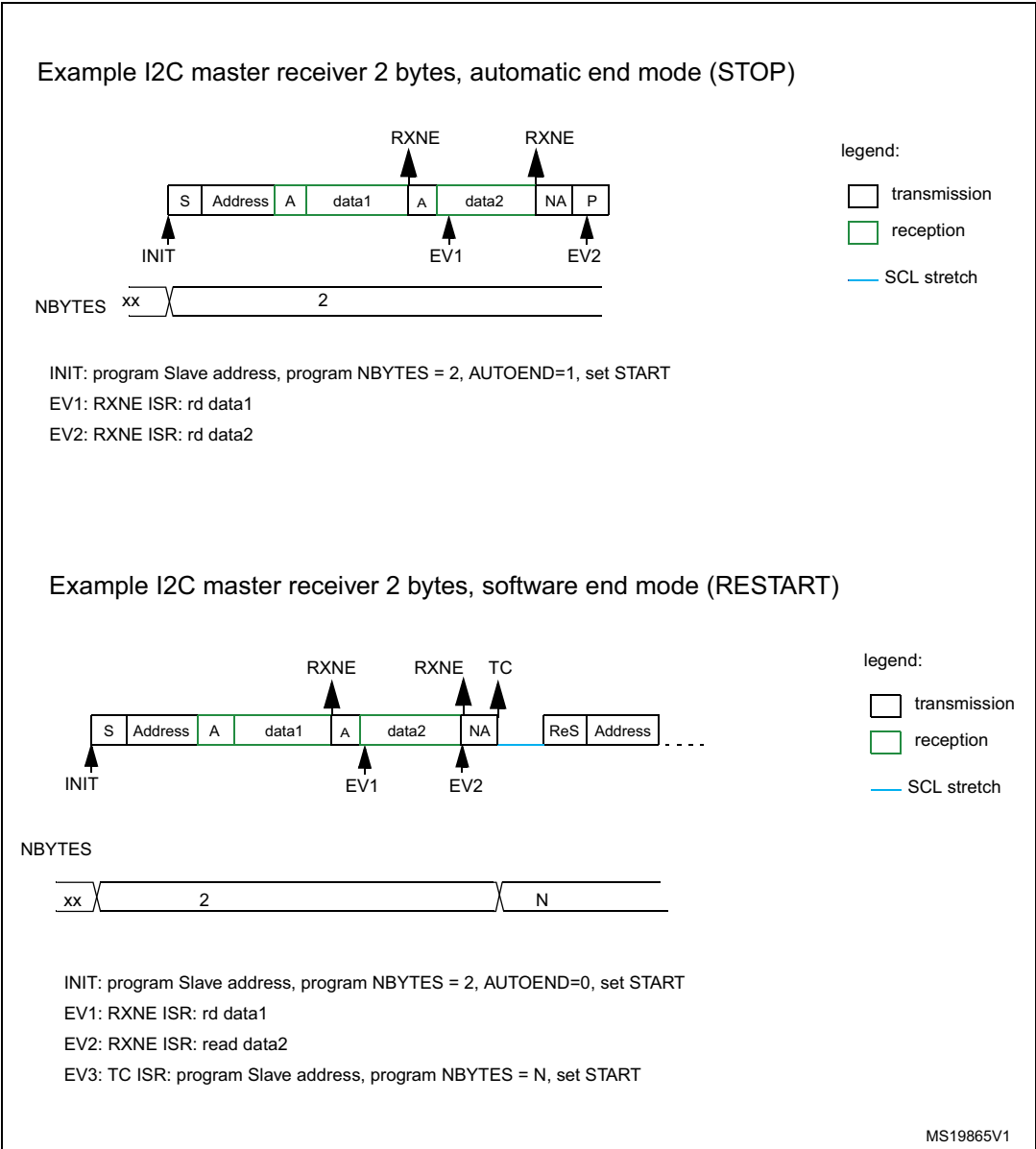
Figure 371. Transfer bus diagrams for I2C master receiver
