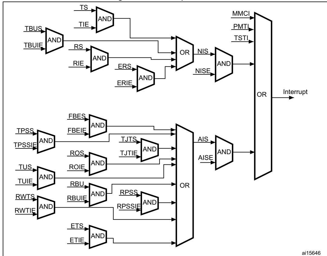
Figure 575. Interrupt scheme
