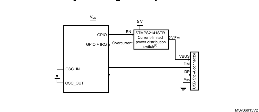
Figure 513. USB_FS host-only connection
