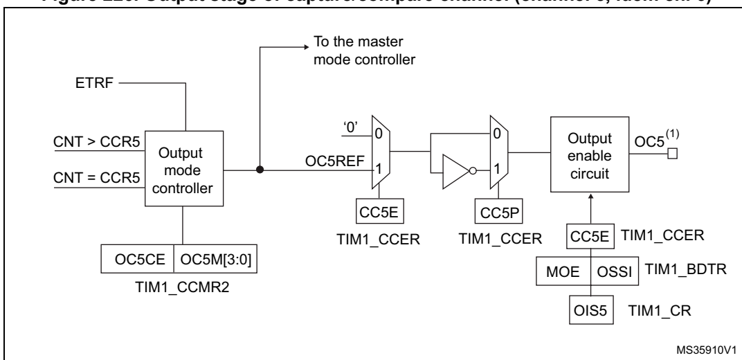
Figure 226. Output stage of capture/compare channel (channel 5, idem ch. 6)
