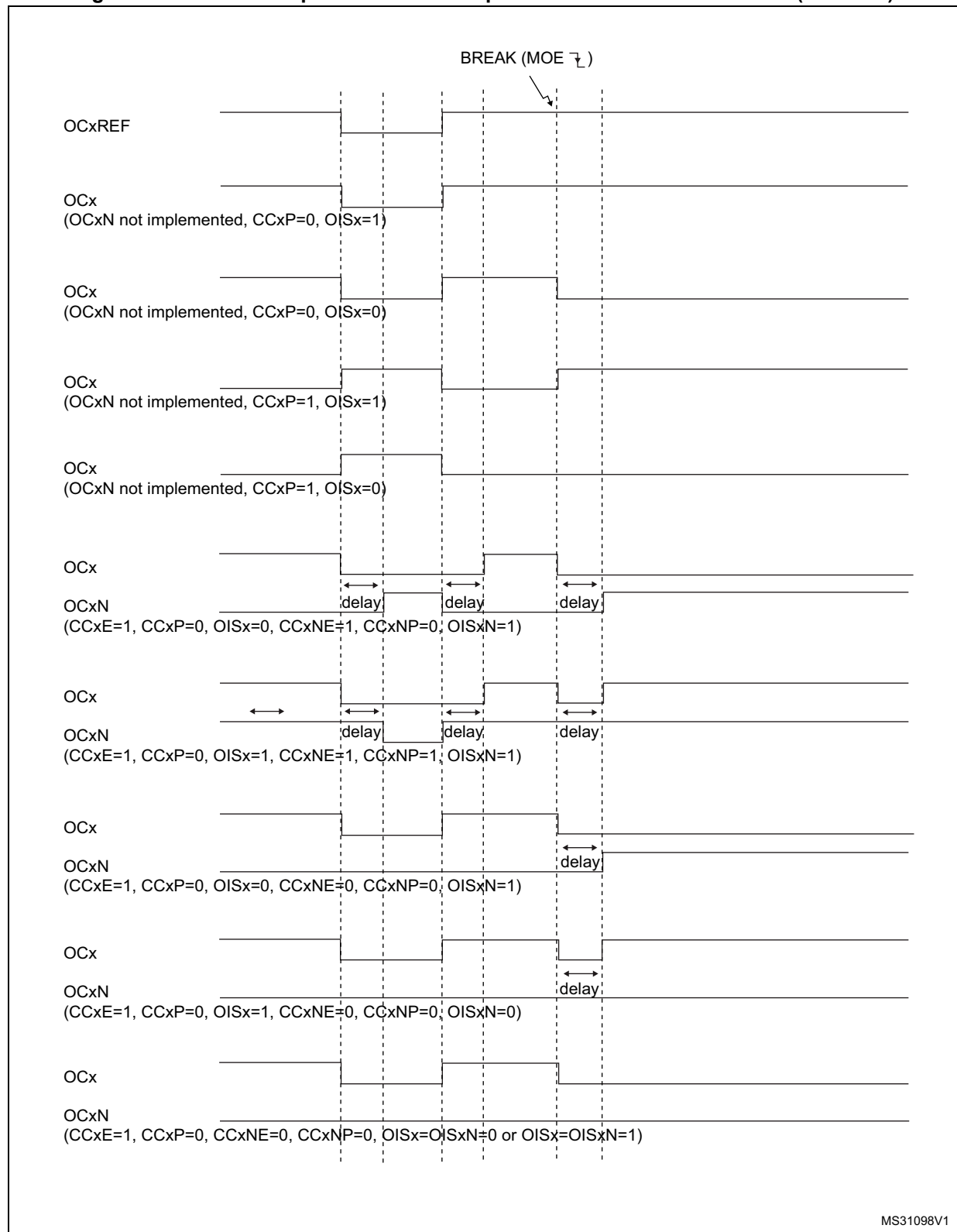
Figure 238. Various output behavior in response to a break event on BRK (OSS1 = 1)
