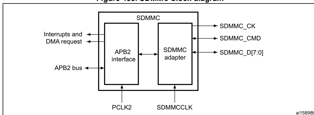
Figure 483. SDMMC block diagram
