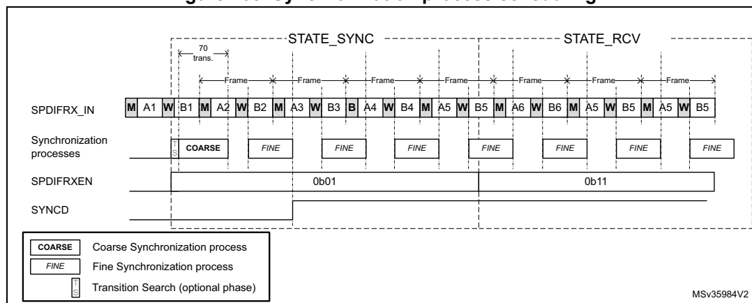
Figure 468. Synchronization process scheduling
