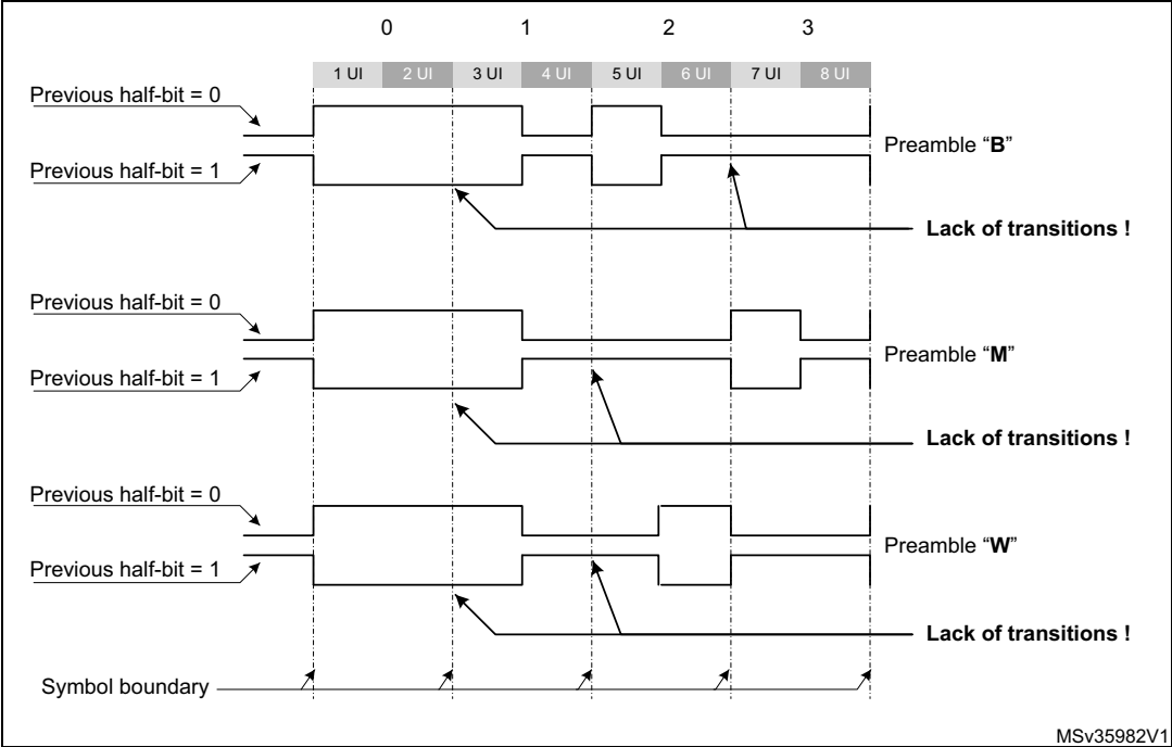
Figure 462. S/PDIF Preambles
