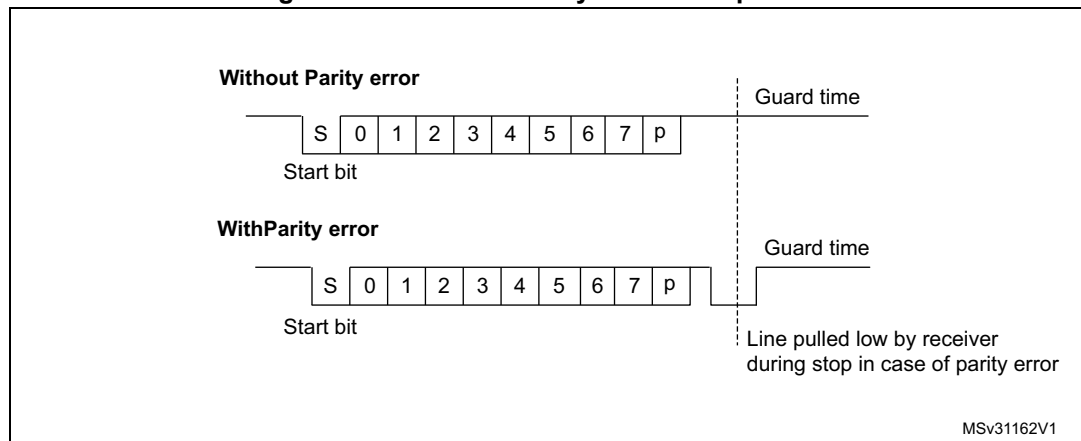
Figure 395. ISO 7816-3 asynchronous protocol
