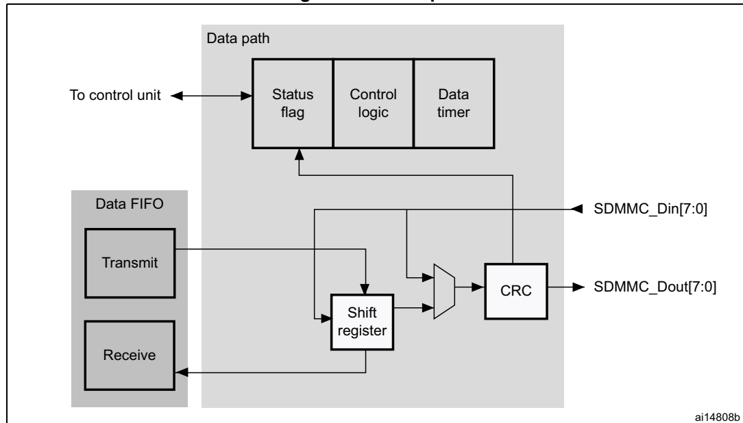
Figure 490. Data path
