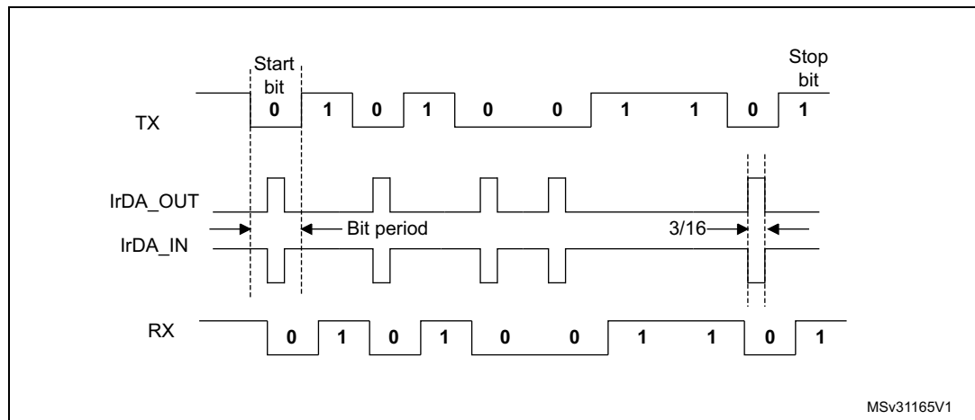
Figure 398. IrDA data modulation (3/16) -Normal Mode
