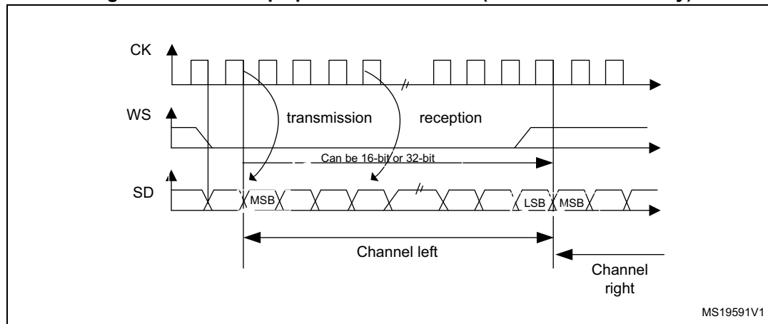
Figure 423. I 2 S Philips protocol waveforms (16/32-bit full accuracy)
