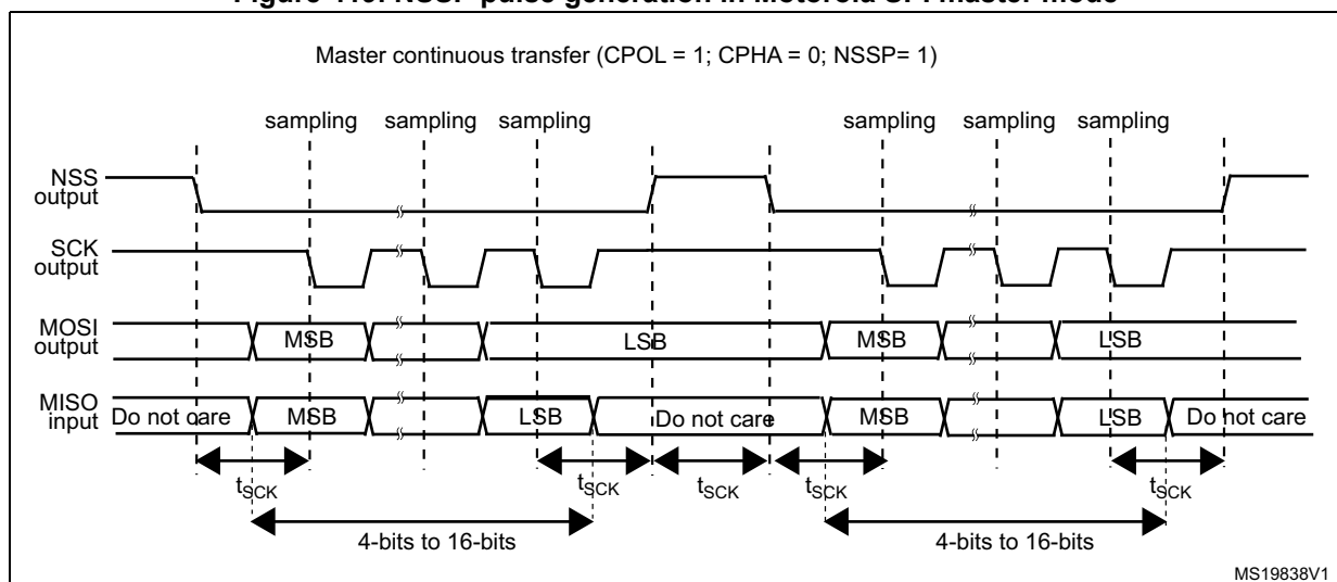
Figure 419. NSSP pulse generation in Motorola SPI master mode
