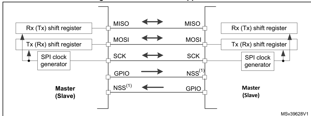
Figure 410. Multi-master application
