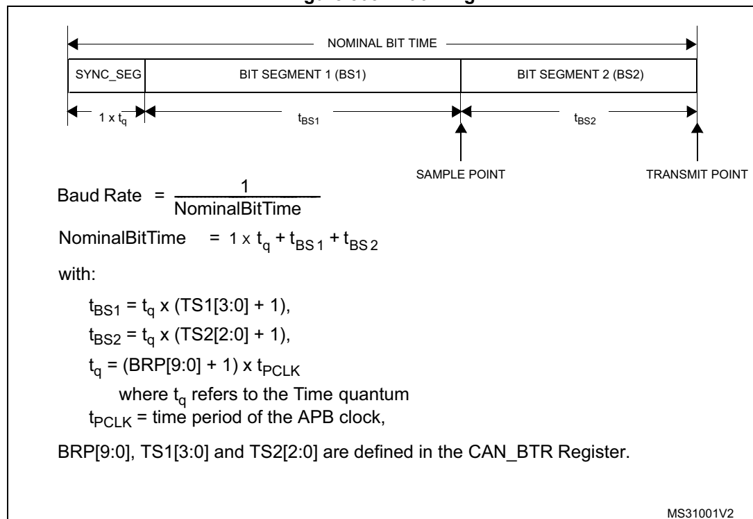
Figure 505. Bit timing
