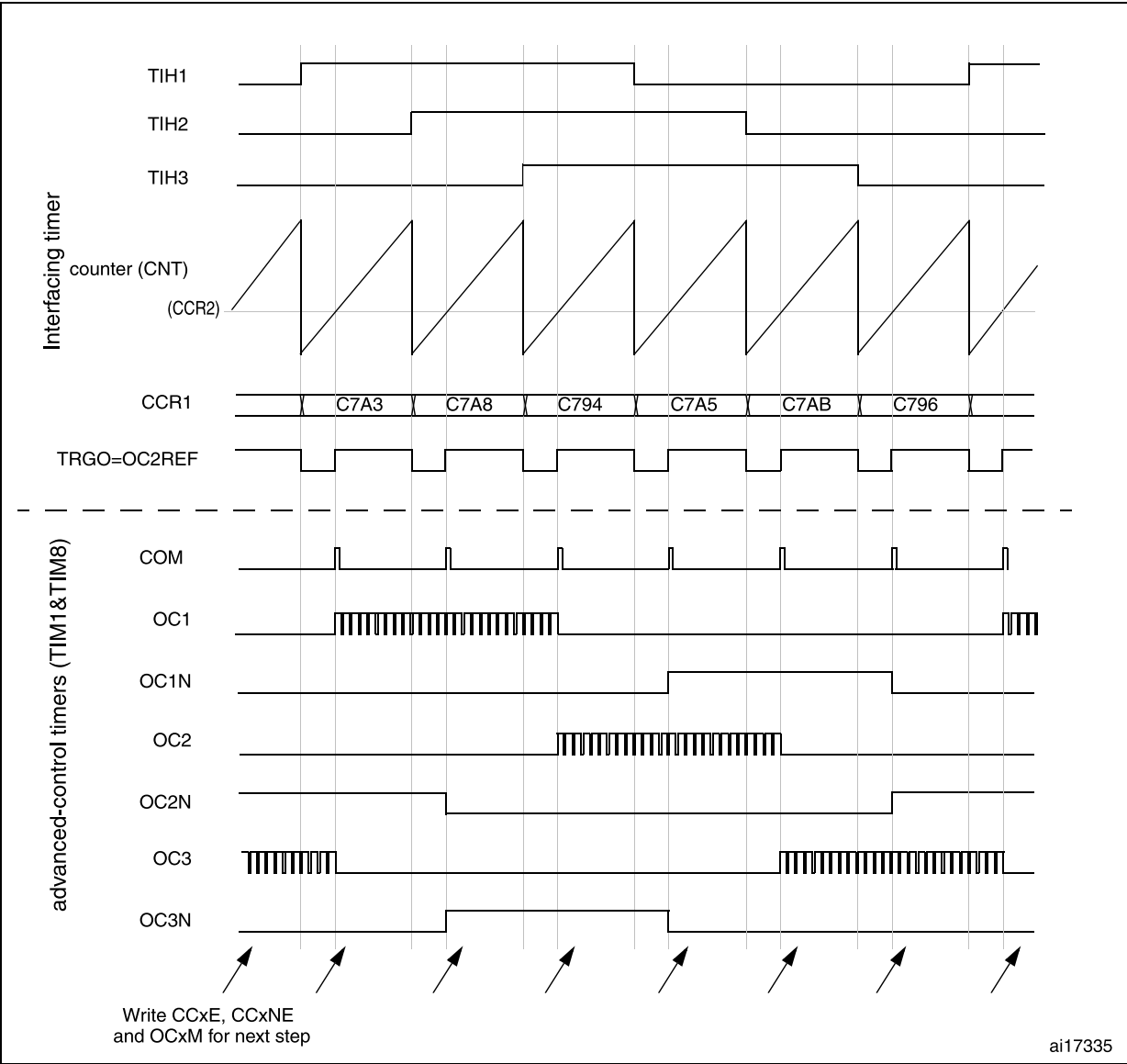
Figure 248. Example of Hall sensor interface
