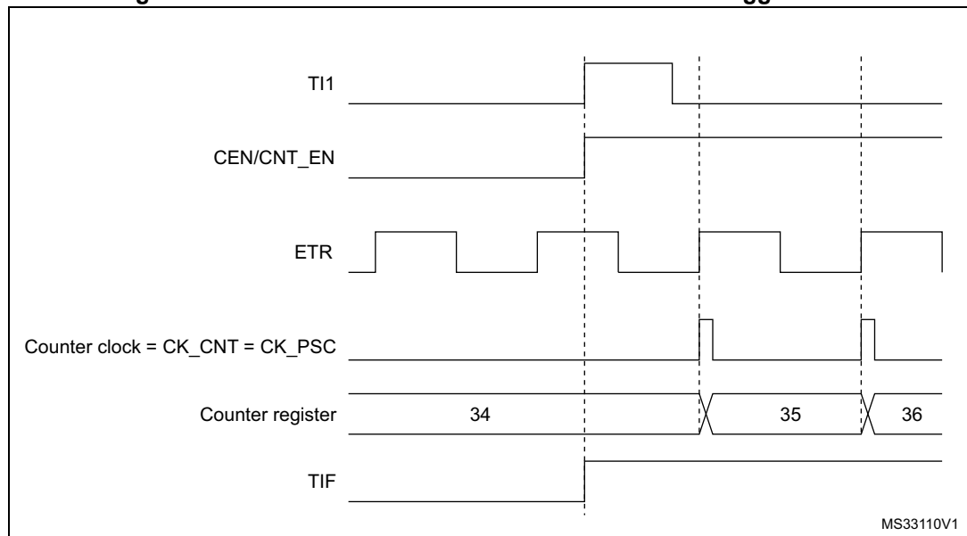
Figure 252. Control circuit in external clock mode 2 + trigger mode
