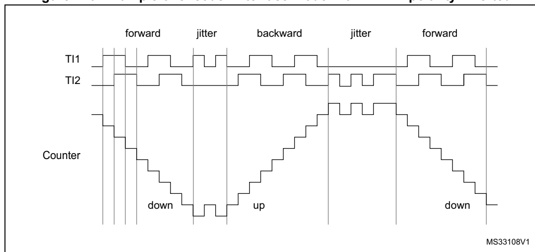
Figure 246. Example of encoder interface mode with TI1FP1 polarity inverted.
