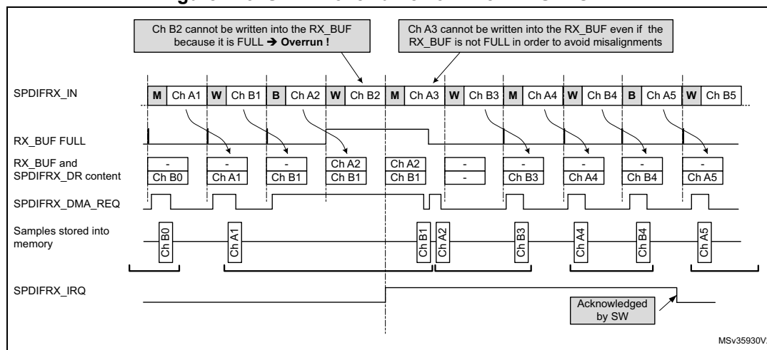
Figure 473. S/PDIF overrun error when RXSTEO = 1
