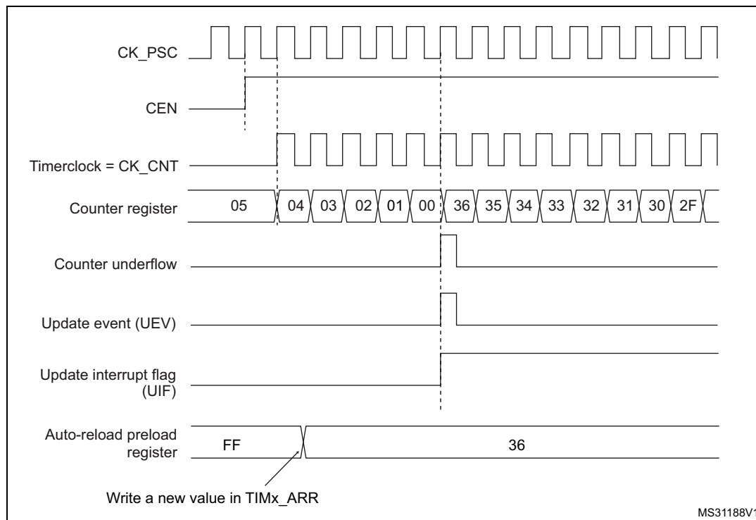
Figure 266. Counter timing diagram, Update event when repetition counter is not used
