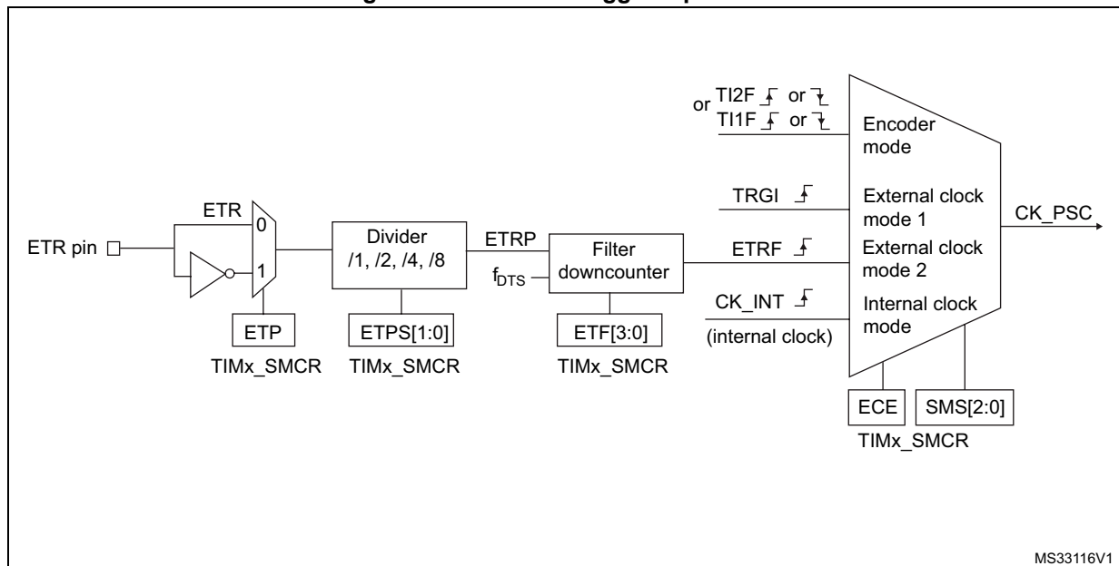
Figure 276. External trigger input block
