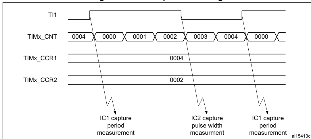
Figure 318. PWM input mode timing
