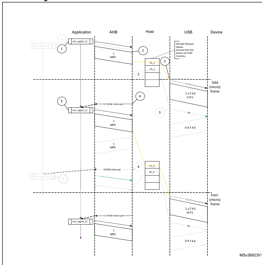
Figure 531. Normal isochronous OUT transaction - DMA mode
