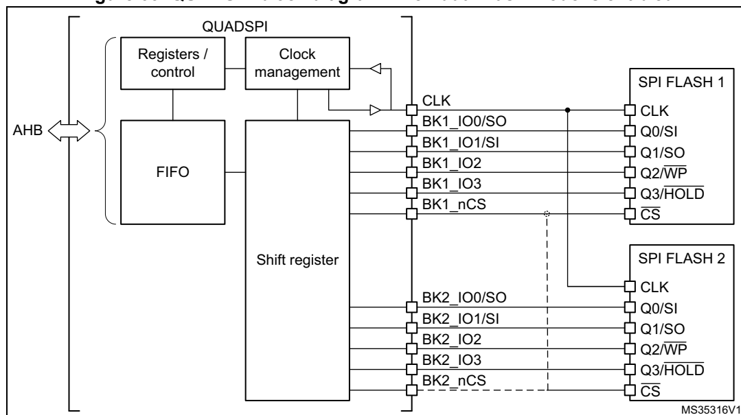
Figure 63. QUADSPI block diagram when dual-flash mode is enabled
