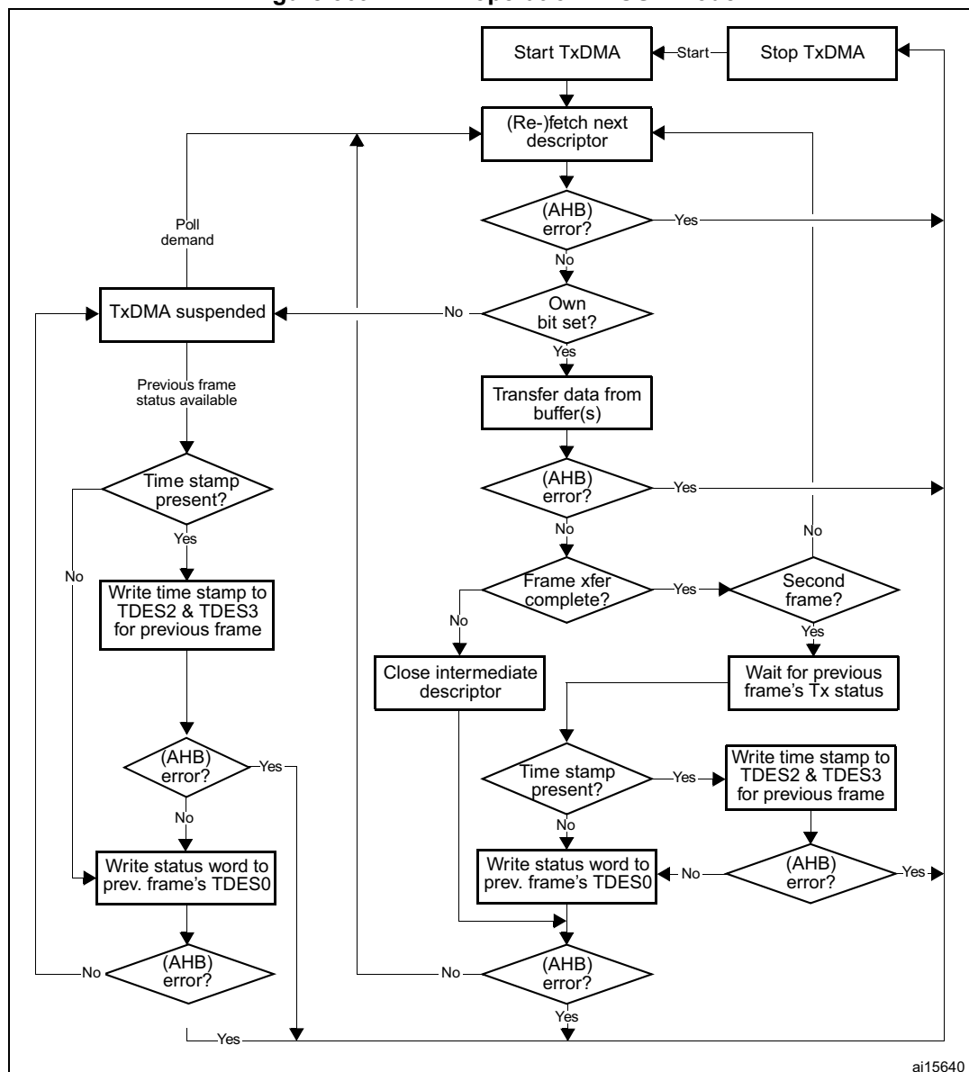
Figure 569. TxDMA operation in OSF mode
