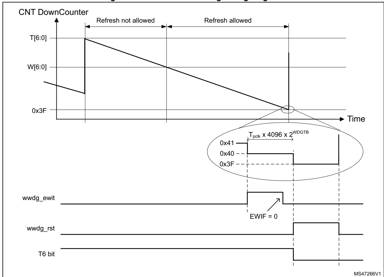
Figure 347. Window watchdog timing diagram
