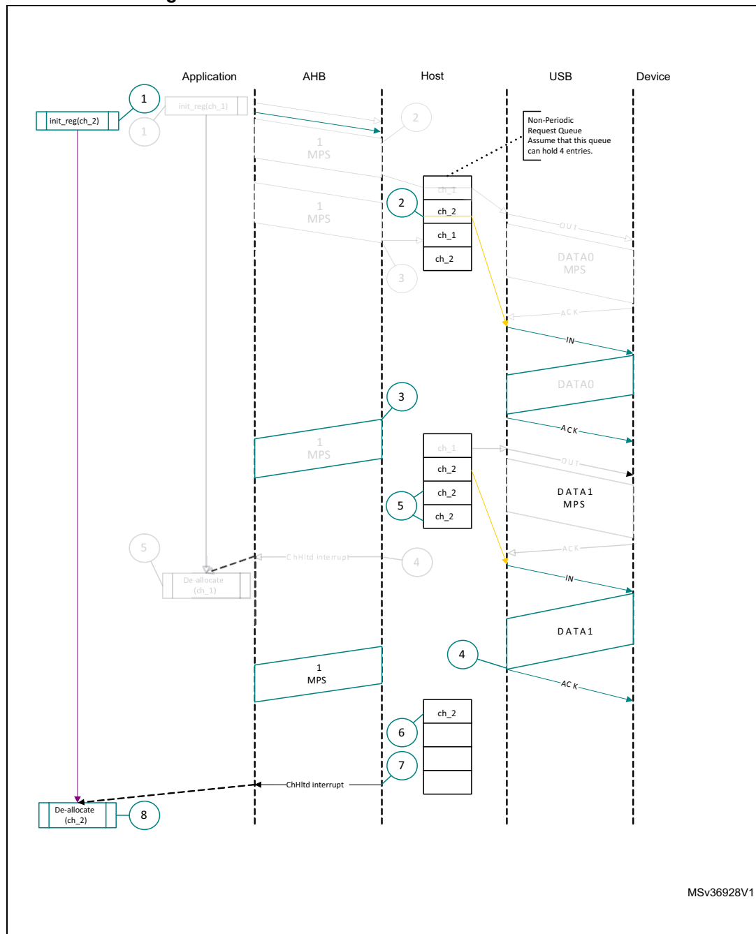
Figure 528. Normal bulk/control IN transaction - DMA
