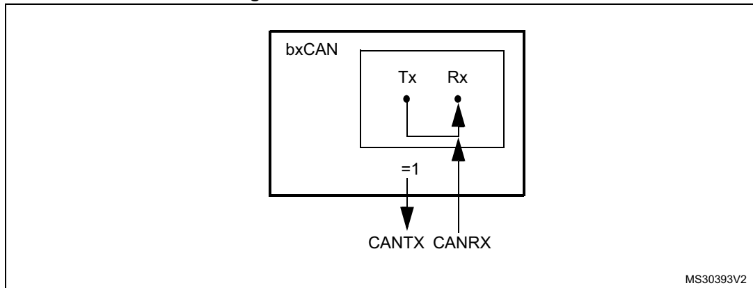
Figure 496. bxCAN in silent mode
