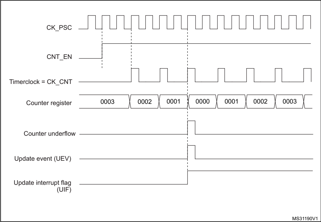
Figure 210. Counter timing diagram, internal clock divided by 2
