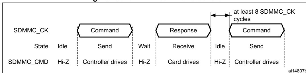
Figure 489. SDMMC command transfer
