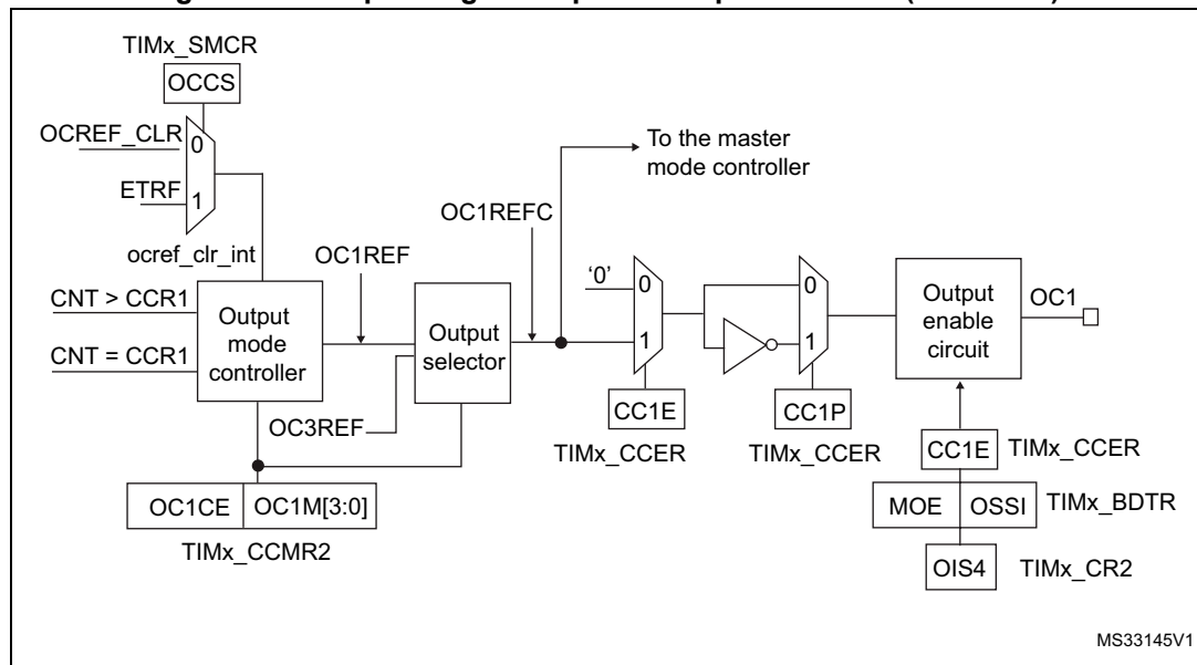
Figure 280. Output stage of capture/compare channel (channel 1)
