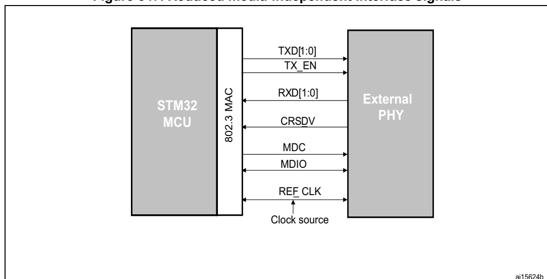
Figure 547. Reduced media-independent interface signals
