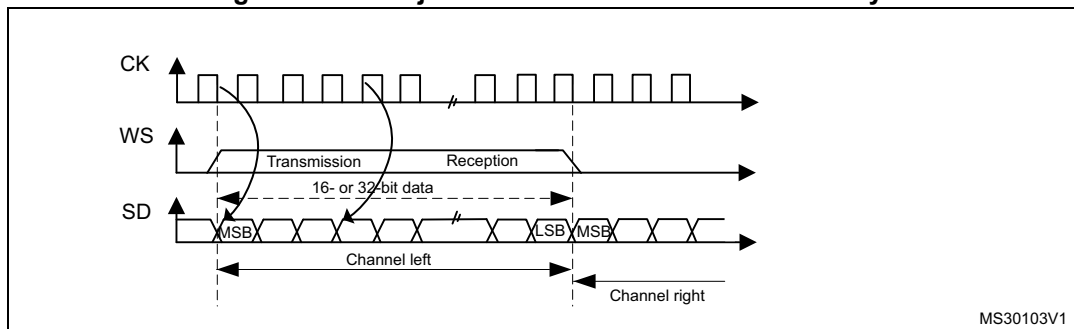
Figure 432. LSB justified 16-bit or 32-bit full-accuracy
