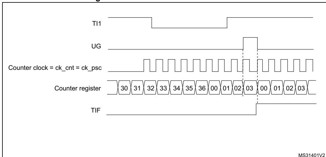
Figure 325. Control circuit in reset mode
