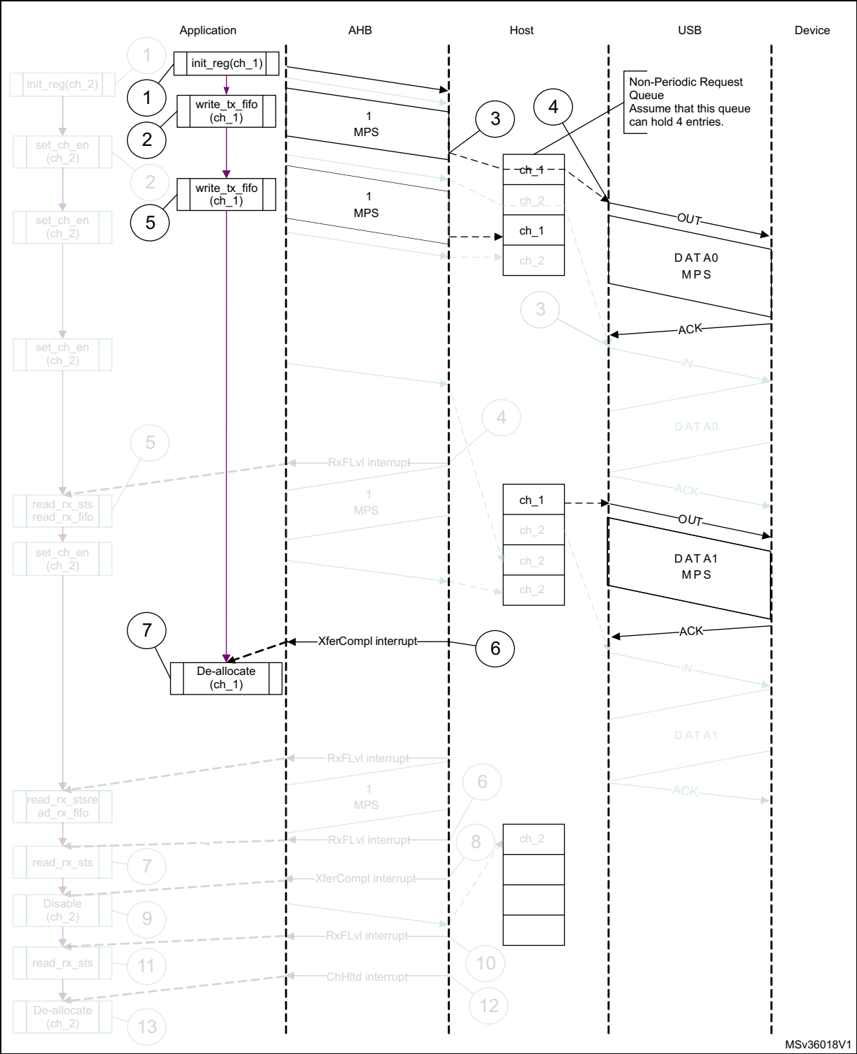
Figure 521. Normal bulk/control OUT/SETUP
