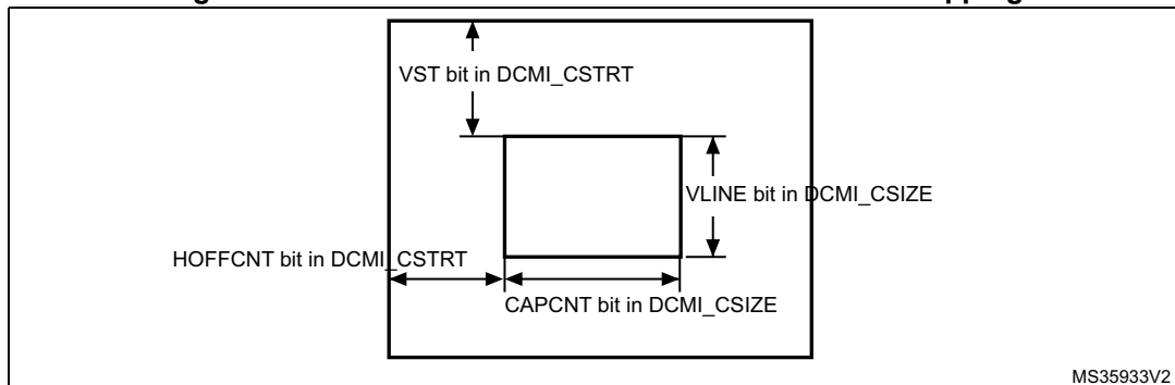
Figure 116. Coordinates and size of the window after cropping
