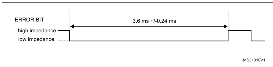
Figure 584. Error bit timing
