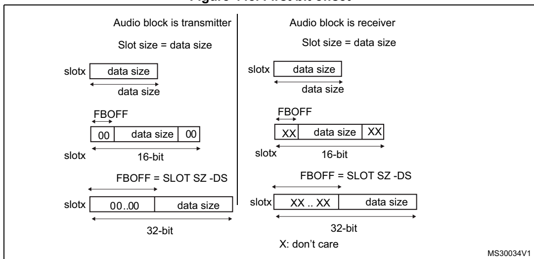
Figure 448. First bit offset
