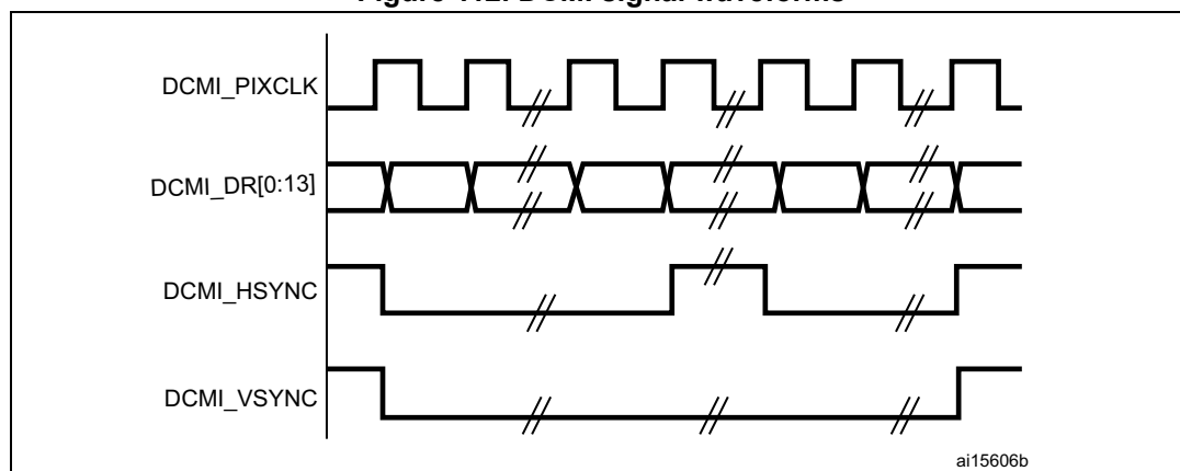
Figure 112. DCMI signal waveforms
