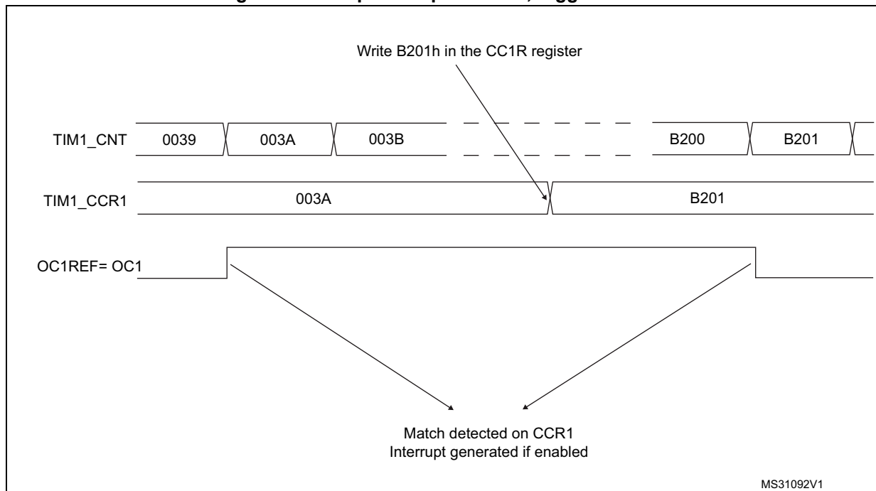
Figure 228. Output compare mode, toggle on OC1
