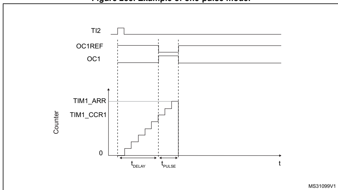
Figure 288. Example of one-pulse mode.
