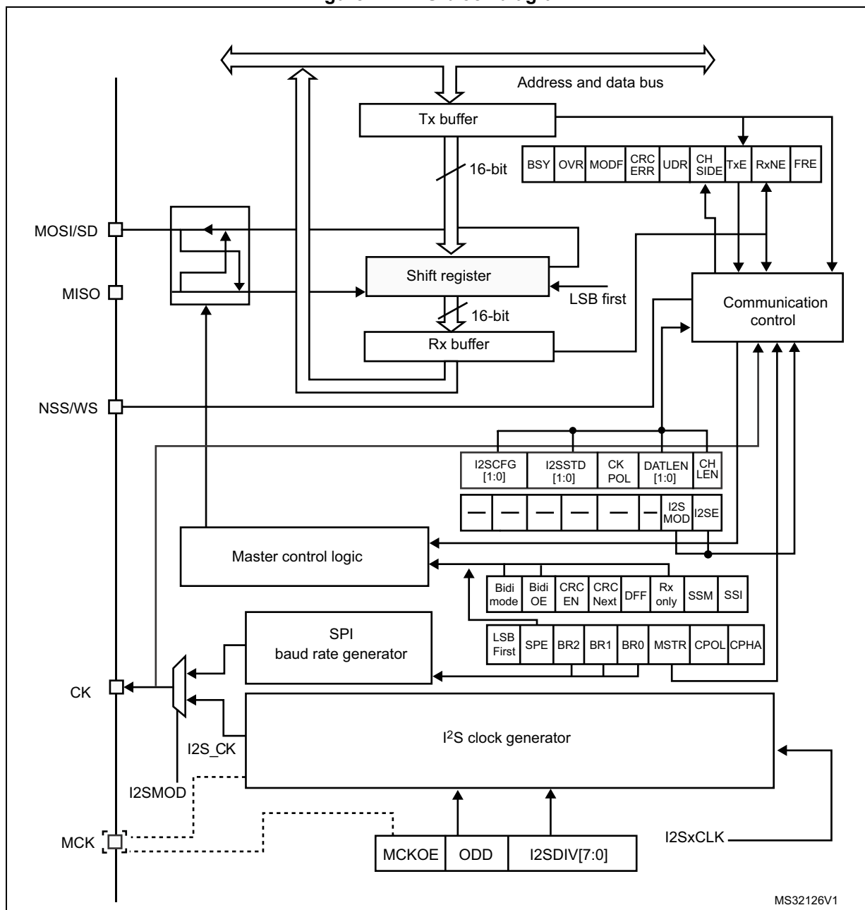
Figure 421. I 2 S block diagram
