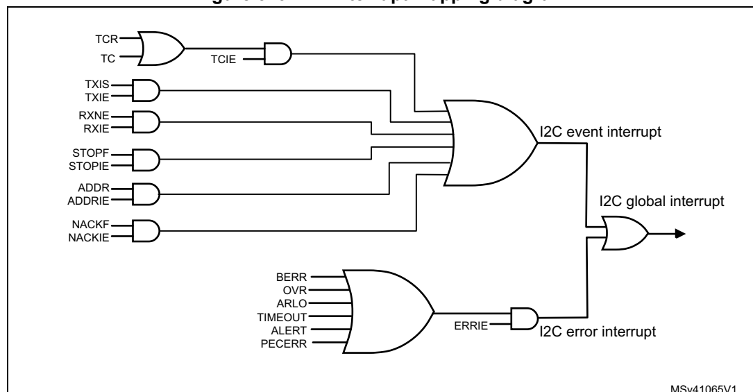
Figure 379. I2C interrupt mapping diagram
