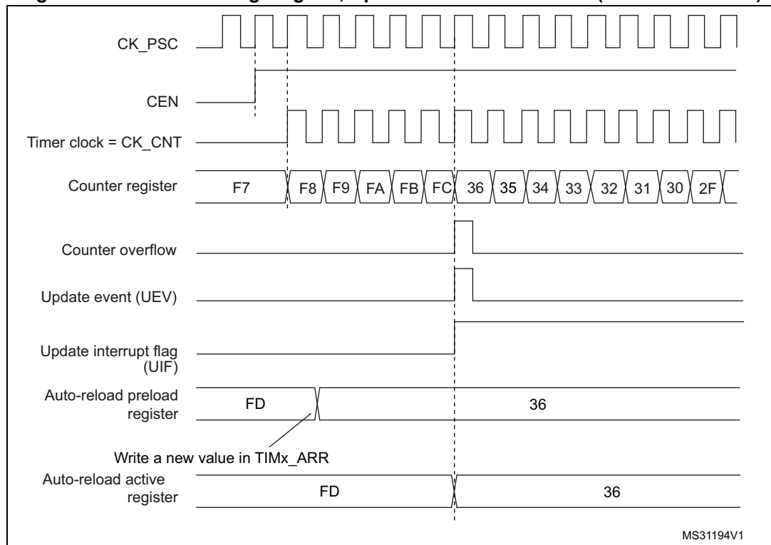
Figure 272. Counter timing diagram, Update event with ARPE=1 (counter overflow)
