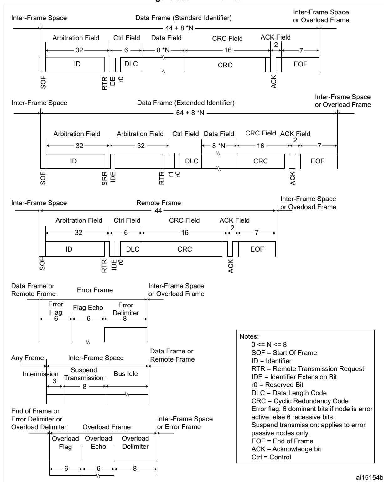
Figure 506. CAN frames
