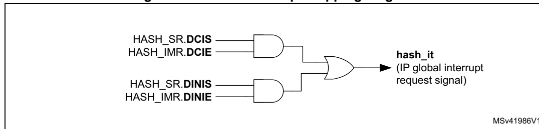
Figure 194. HASH interrupt mapping diagram
