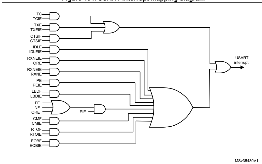
Figure 404. USART interrupt mapping diagram
