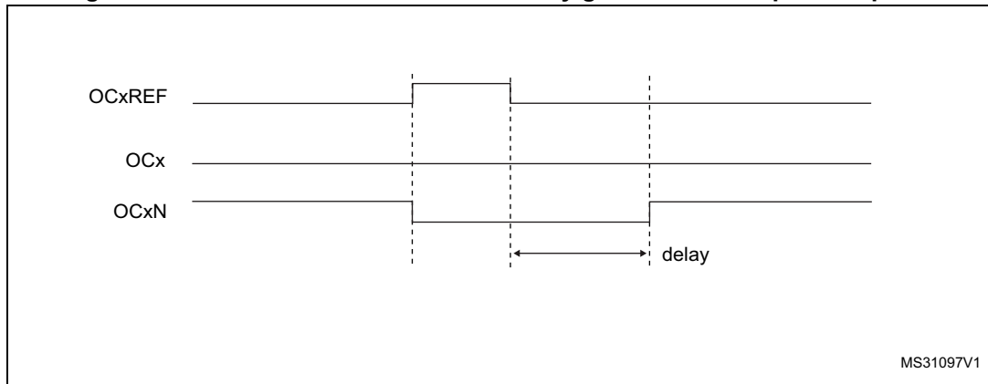
Figure 236. Dead-time waveforms with delay greater than the positive pulse
