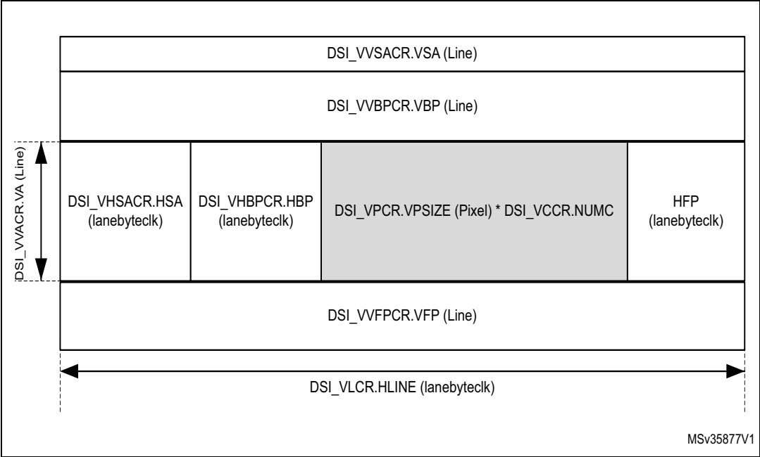
Figure 160. Frame configuration registers
