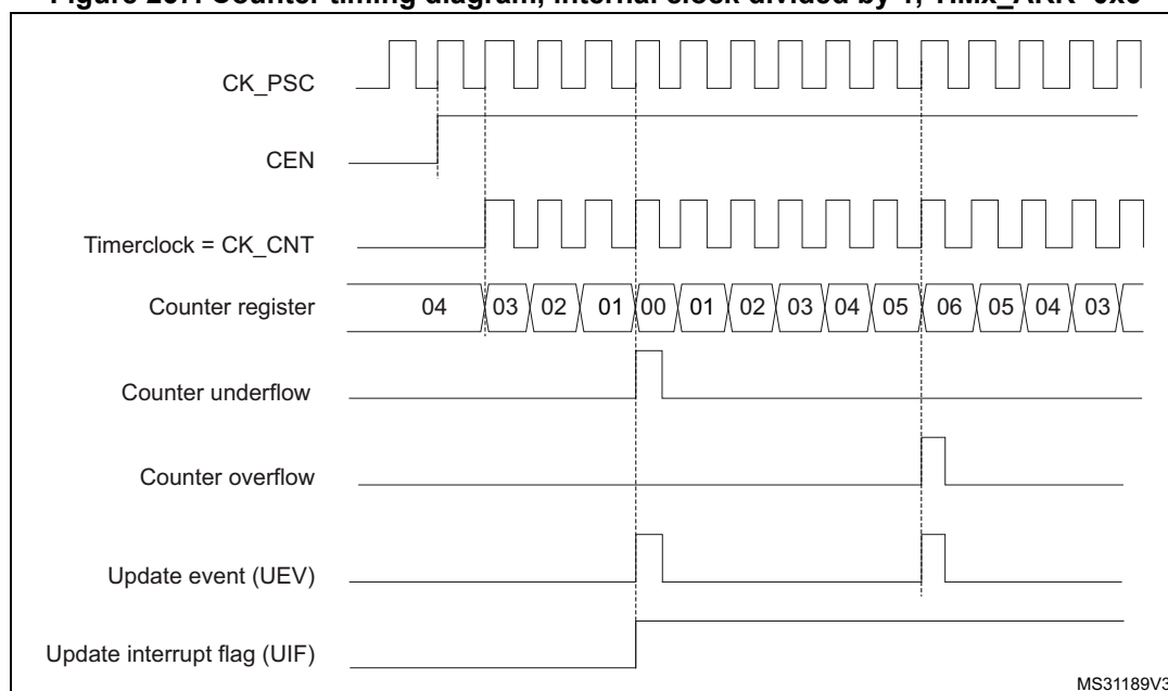
Figure 267. Counter timing diagram, internal clock divided by 1, TIMx_ARR=0x6
