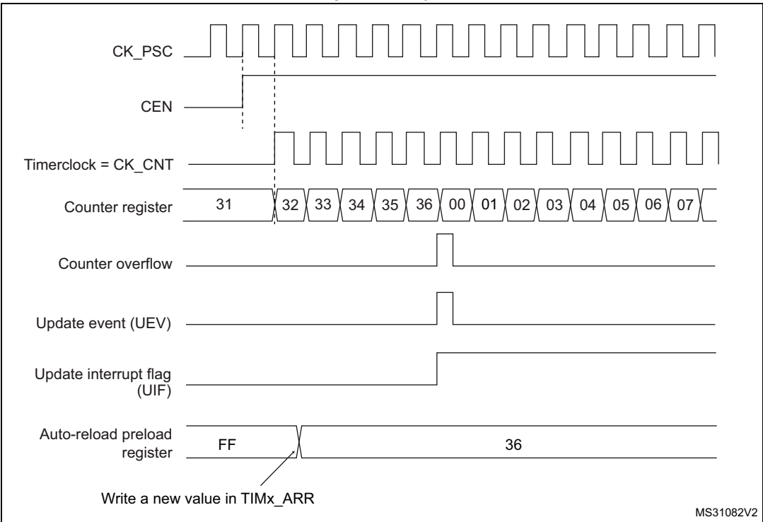
Figure 335. Counter timing diagram, update event when ARPE = 0 (TIMx_ARR not preloaded)
