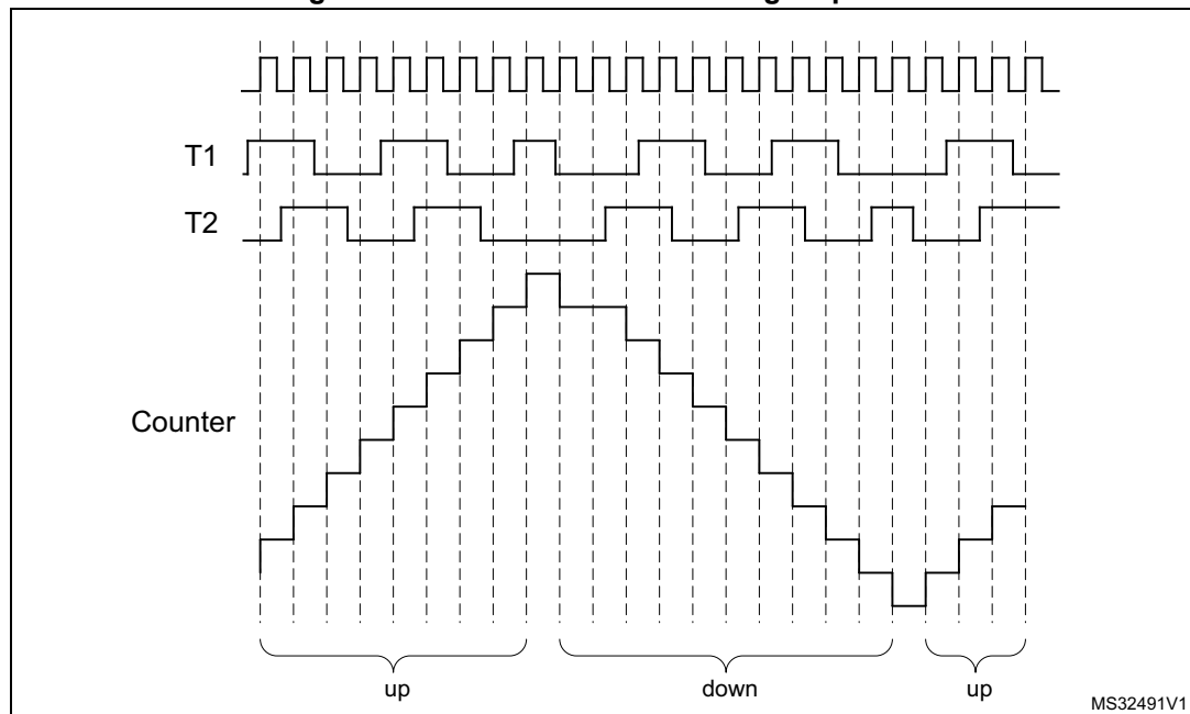
Figure 344. Encoder mode counting sequence
