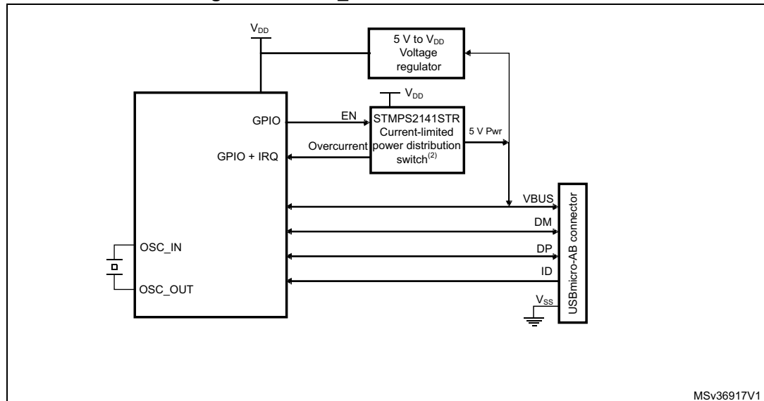
Figure 511. OTG_FS A-B device connection
