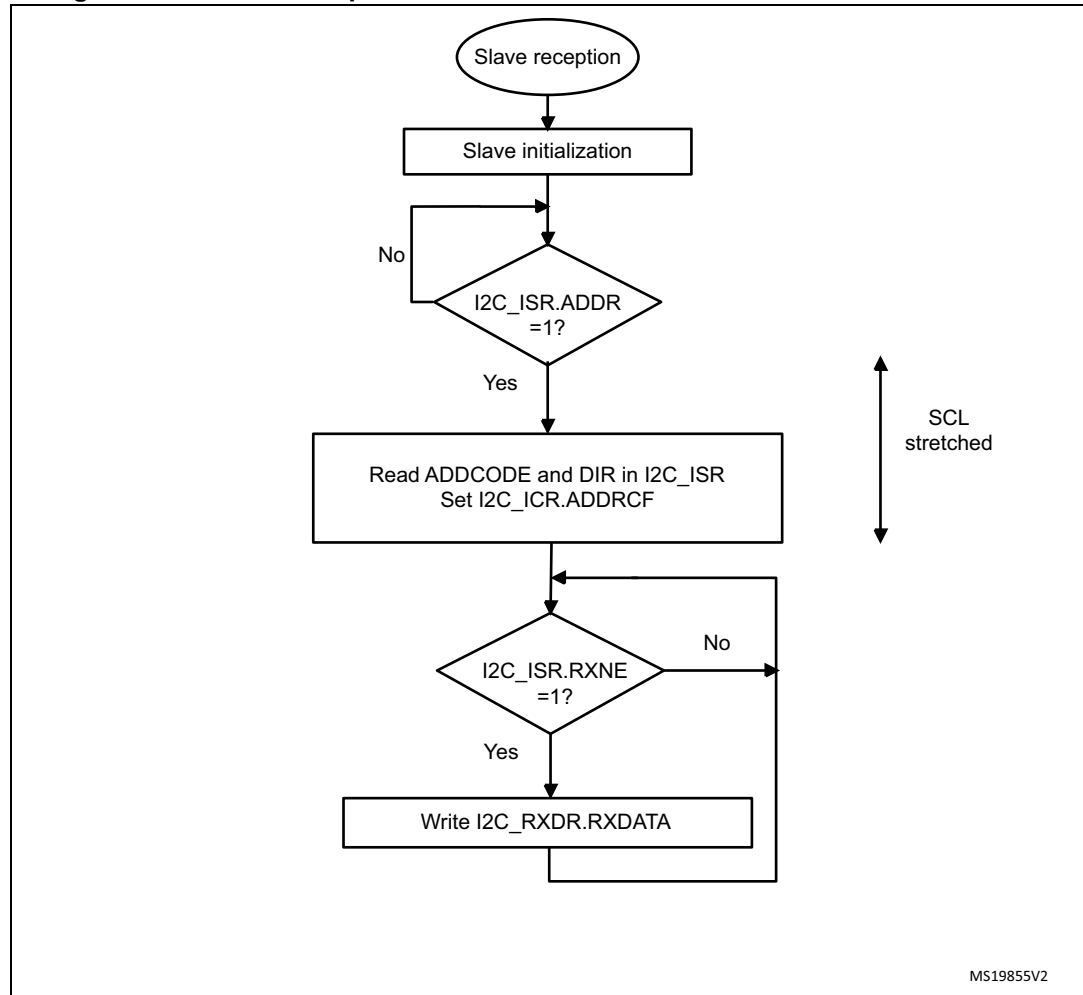
Figure 359. Transfer sequence flowchart for slave receiver with NOSTRETCH=0
