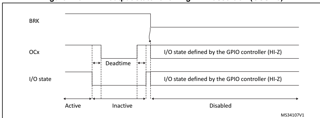
Figure 240. PWM output state following BRK assertion (OSSI=0)
