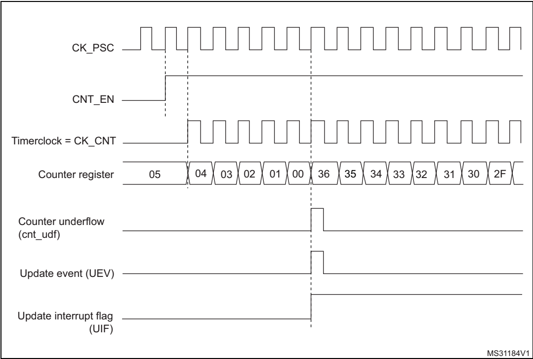
Figure 262. Counter timing diagram, internal clock divided by 1
