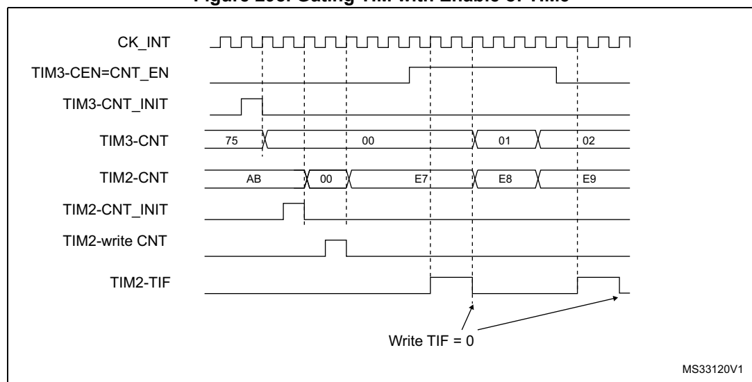
Figure 298. Gating TIM with Enable of TIM3
