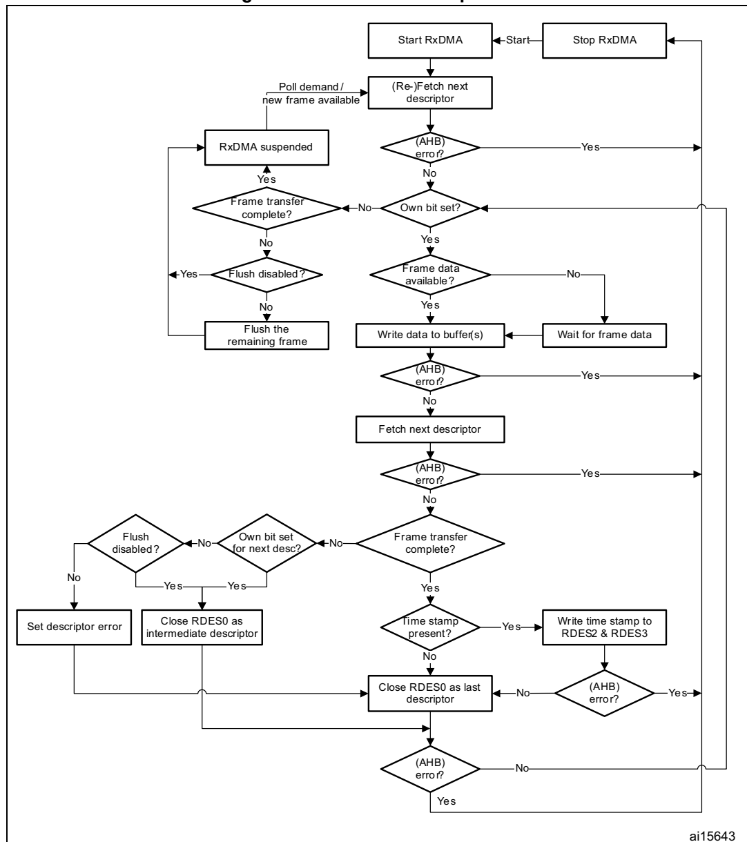
Figure 572. Receive DMA operation
