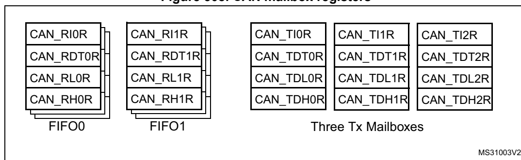
Figure 508. CAN mailbox registers
