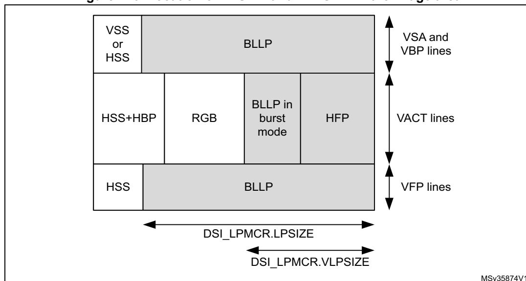
Figure 146. Location of LPSIZE and VLPSIZE in the image area
