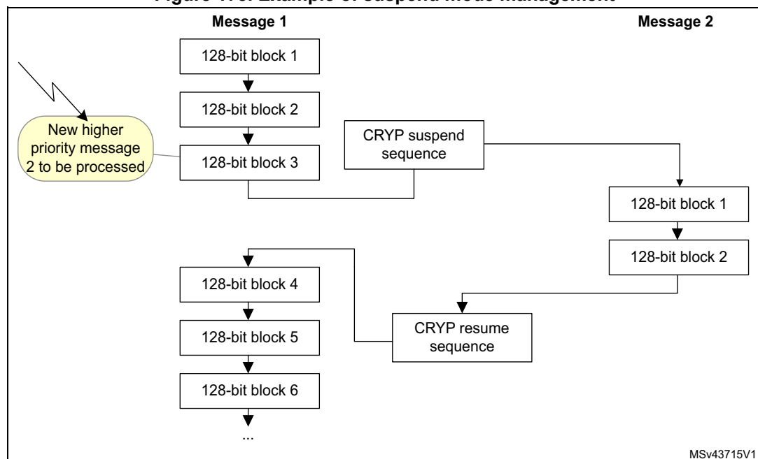
Figure 173. Example of suspend mode management
