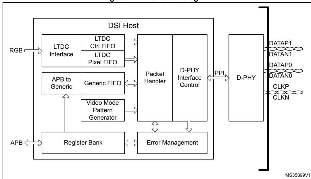
Figure 124. DSI block diagram
