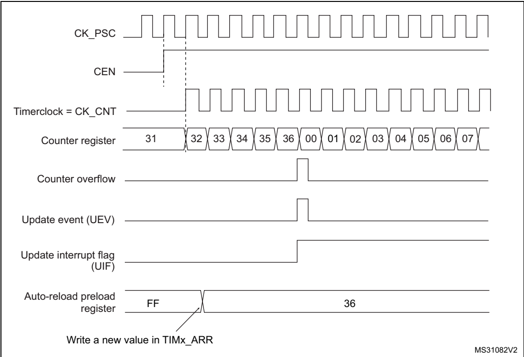
Figure 310. Counter timing diagram, update event when ARPE=0 (TIMx_ARR not preloaded)
