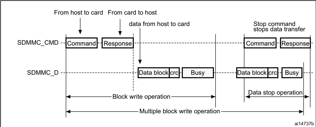
Figure 480. (Multiple) block write operation
