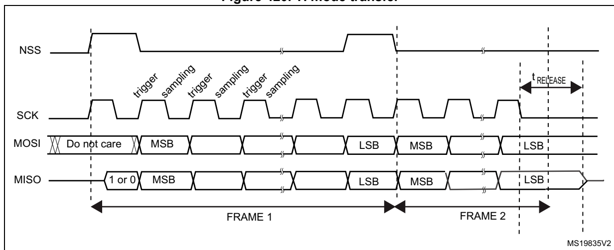
Figure 420. TI mode transfer
