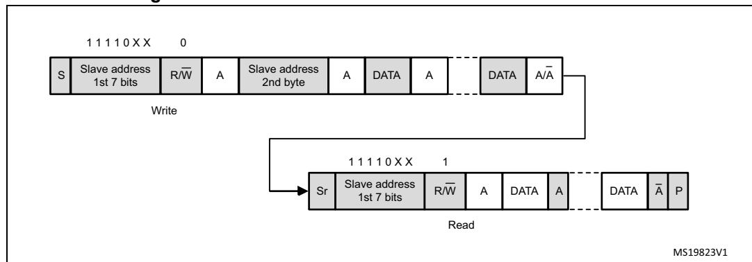
Figure 365. 10-bit address read access with HEAD10R=1
