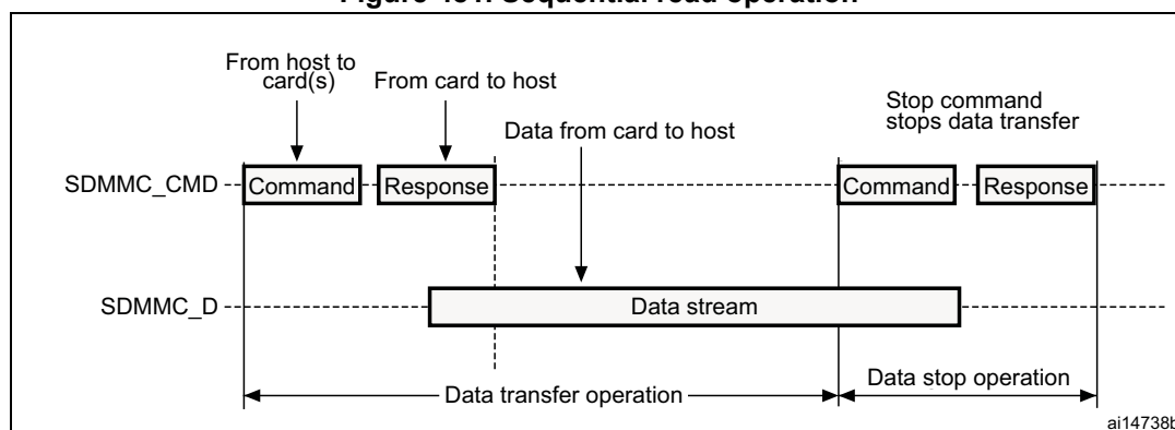
Figure 481. Sequential read operation
