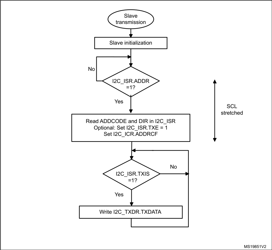
Figure 356. Transfer sequence flowchart for I2C slave transmitter, NOSTRETCH=0
