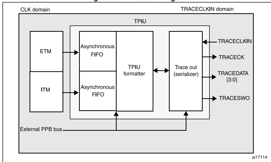
Figure 590. TPIU block diagram
