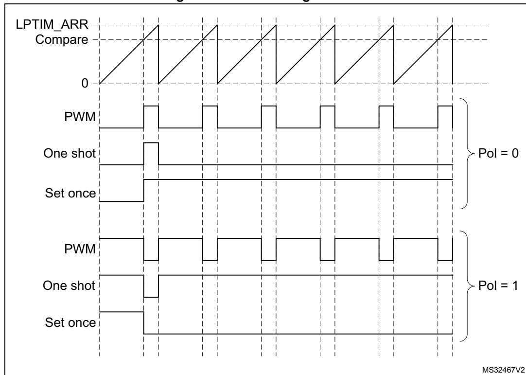
Figure 343. Waveform generation
