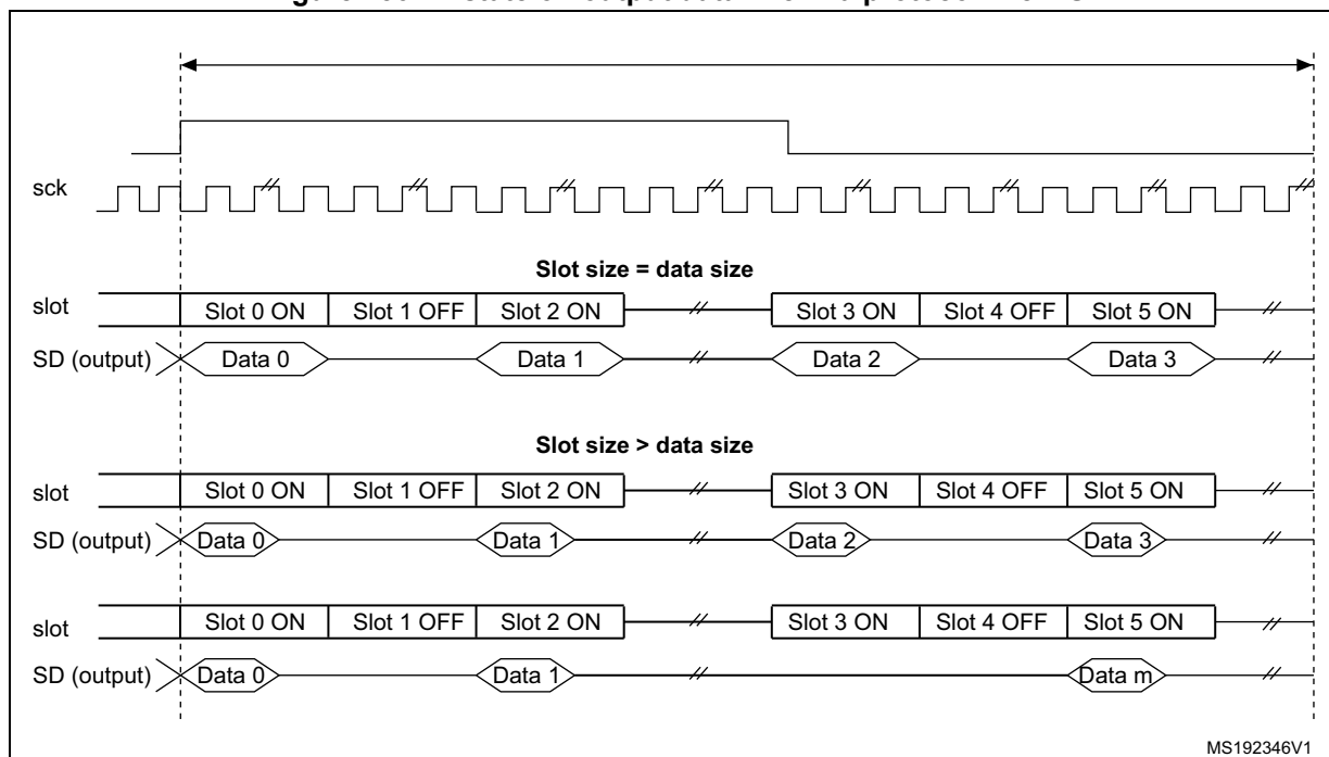
Figure 456. Tristate on output data line in a protocol like I2S
