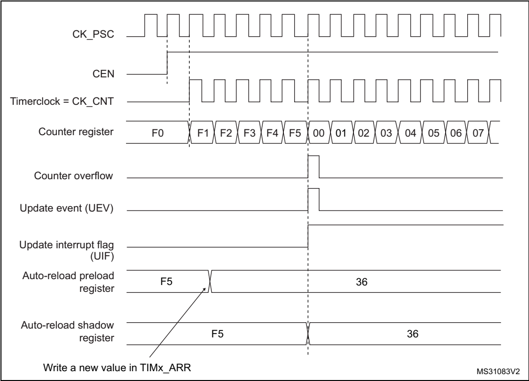
Figure 203. Counter timing diagram, update event when ARPE=1 (TIMx_ARR preloaded)
