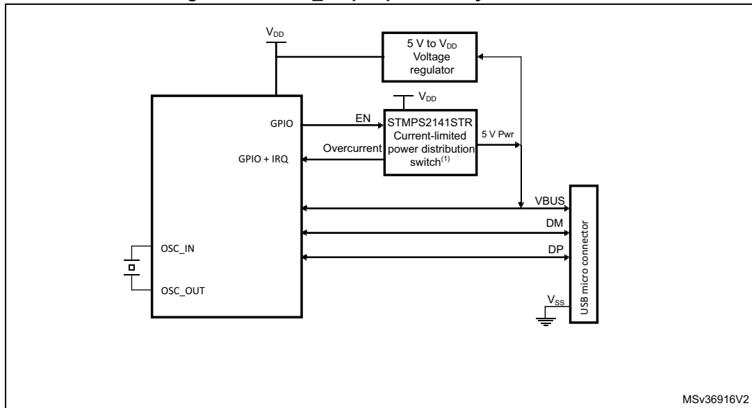
Figure 512. USB_FS peripheral-only connection
