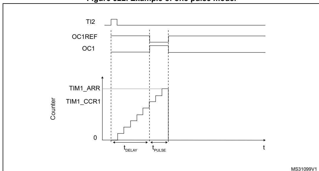
Figure 322. Example of one pulse mode.
