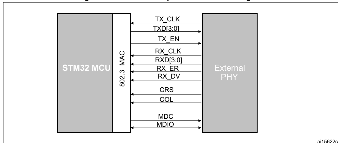
Figure 545. Media independent interface signals
