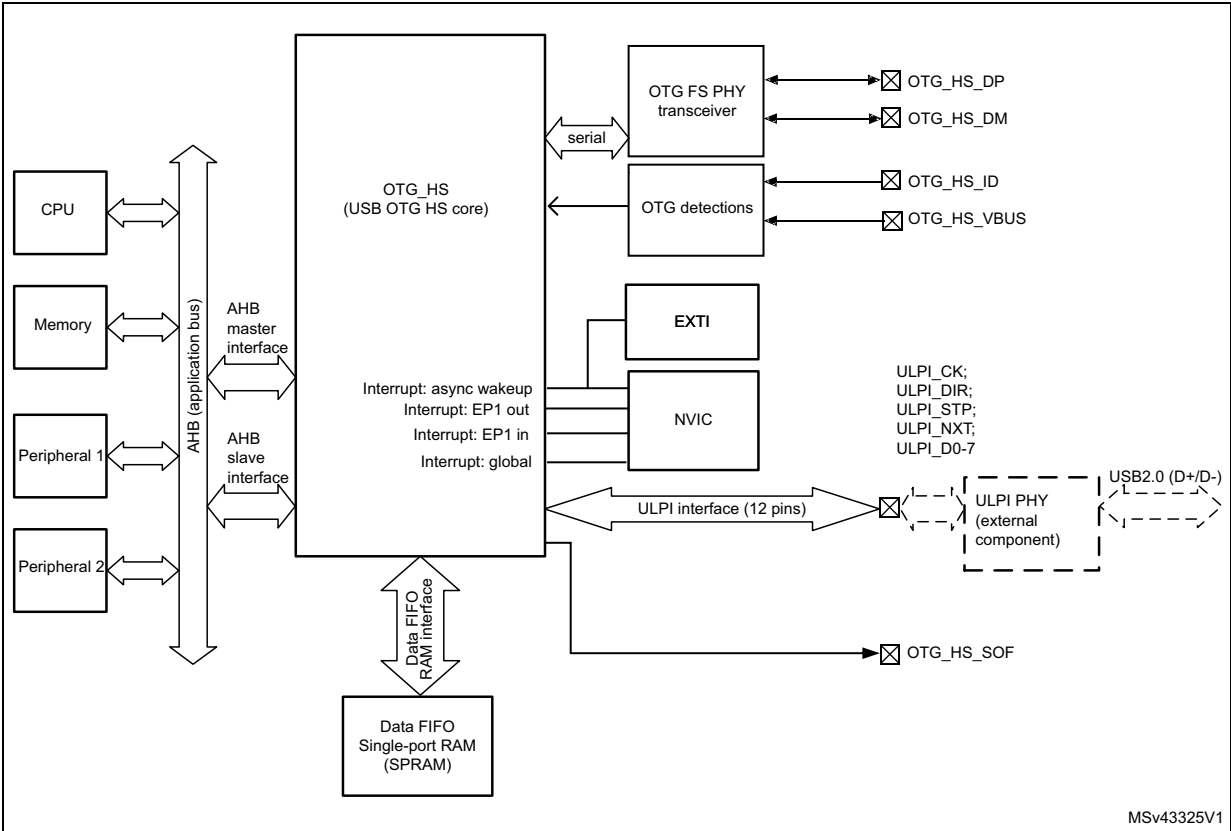
Figure 510. OTG high-speed block diagram
