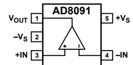
Figure 2. SOT23-5 (RJ-5)
