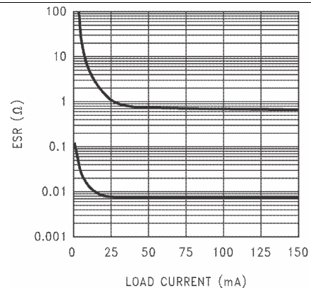
Figure 18. 2.2- \mu F Stable ESR Range for Output Voltage \leq 2.3 V
