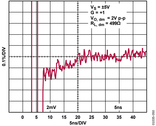
Figure 44. 0.1% Settling Time
