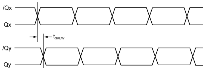
Figure 3. Output-to-Output Skew
