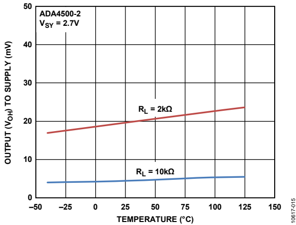
Figure 18. Output Voltage ( V_{OH} ) to Supply Rail vs. Temperature, V_{SY} = 2.7\text{ V}
