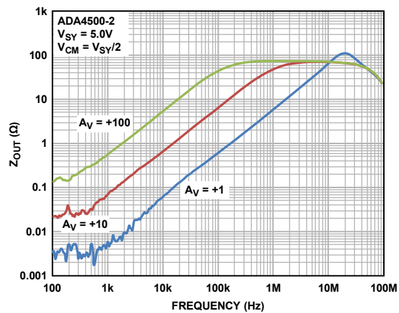
Figure 34. Closed Loop Output Impedance (Z OUT ) vs. Frequency, V SY = 5.0 V
