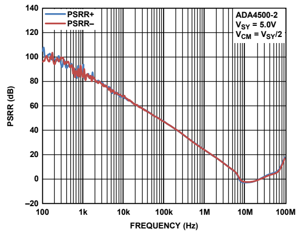
Figure 33. PSRR vs. Frequency, V SY = 5.0 V
