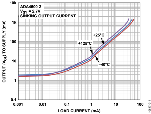
Figure 17. Output Voltage ( V_{OL} ) to Supply Rail vs. Temperature, V_{SY} = 2.7\text{ V}
