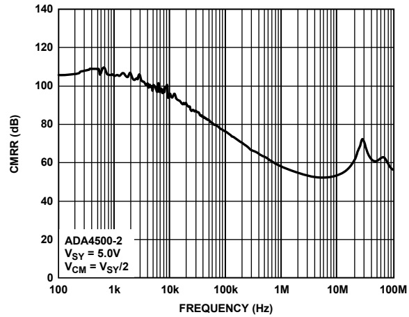
Figure 32. CMRR vs. Frequency, V SY = 5.0 V
