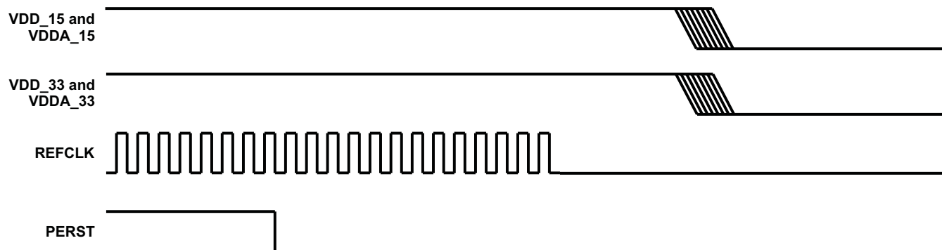
Figure 3-3. Power-Down Sequence
