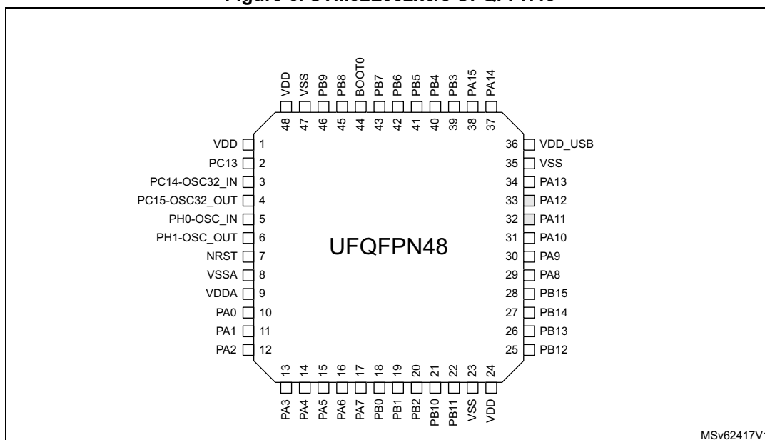
Figure 6. STM32L052x6/8 UFQFPN48
