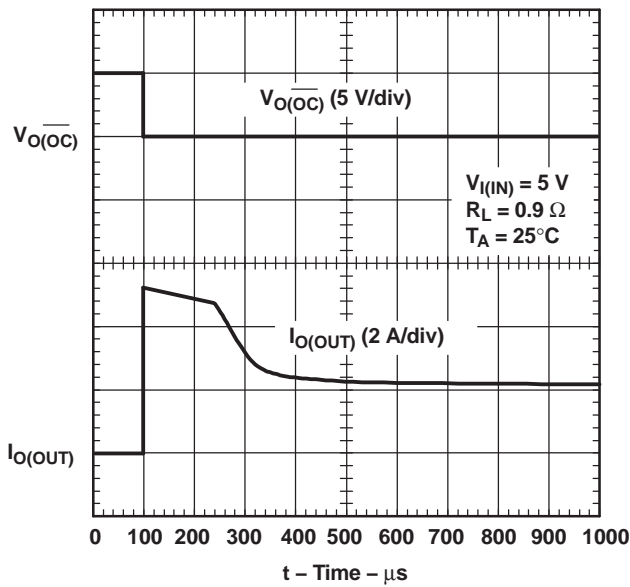
Figure 20. 0.9- \Omega Load Connected to an Enabled TPS2033 Device
