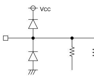
18pin (VOUT)
