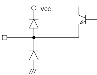
20pin (REF)
