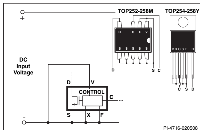
Figure 16a. Three Terminal Operation (VOLTAGE MONITOR and EXTERNAL CURRENT LIMIT Features Disabled. FREQUENCY Pin Tied to SOURCE or CONTROL Pin) for TOP254-258 Y Packages.
