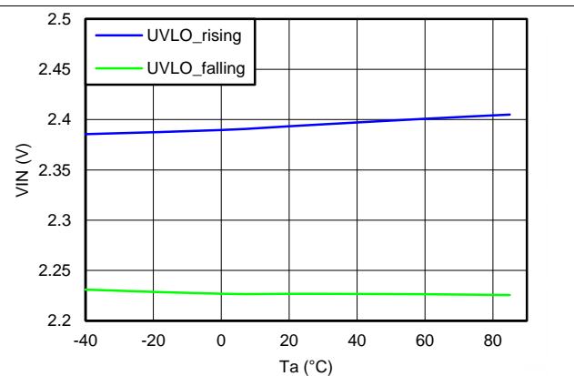
Figure 5. UVLO
