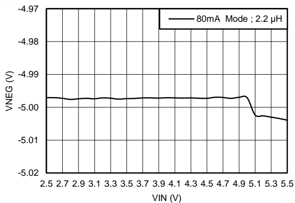
Figure 114. Line Regulation V NEG = -5.0 V — SYNC = HIGH
