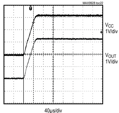
POWER-UP DELAY
