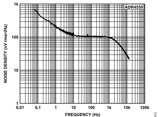
Figure 96. ADR4550 Output Noise Spectral Density
