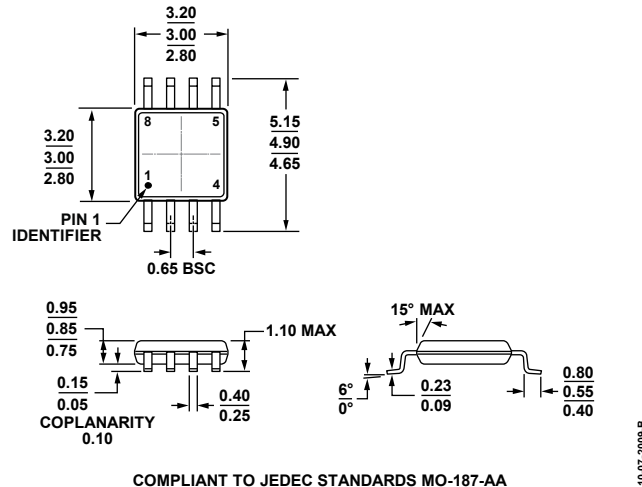
Figure 67. 8-Lead Mini Small Outline Package [MSOP] (RM-8) Dimensions shown in millimeters
