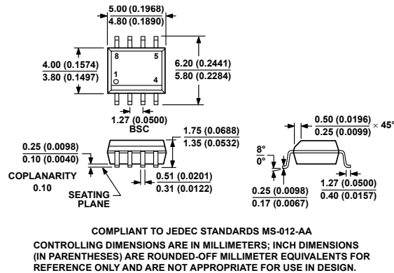
Figure 68. 8-Lead Standard Small Outline Package [SOIC_N] Narrow Body (R-8) Dimensions shown in millimeters and (inches)
