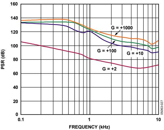
Figure 27. Positive PSR vs. Frequency, RTI
