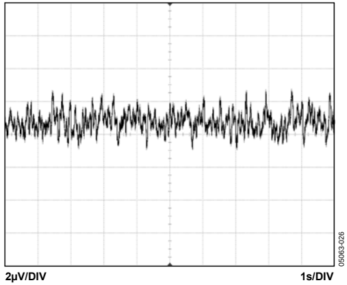
Figure 26. 0.1 Hz to 10 Hz RTI Voltage Noise, G = 100
