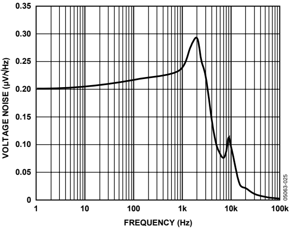
Figure 25. Voltage Noise Spectral Density vs. Frequency
