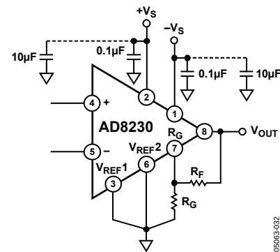
Figure 32. Gain Setting
