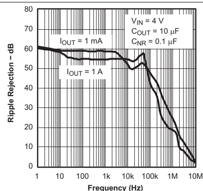
Figure 27. TPS79630 Ripple Rejection vs Frequency
