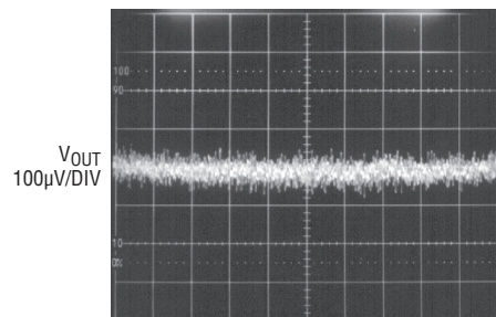
C OUT = 10µF I L = 100mA 1ms/DIV 1761 G48
