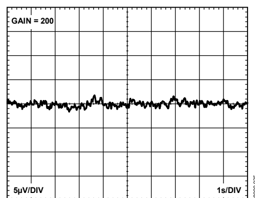
Figure 9. 0.1 Hz to 10 Hz RTI Voltage Noise
